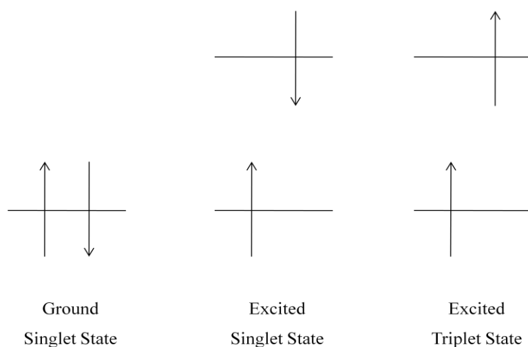
Figure 3.3 Electronic states; Singlet and Triplet state.
