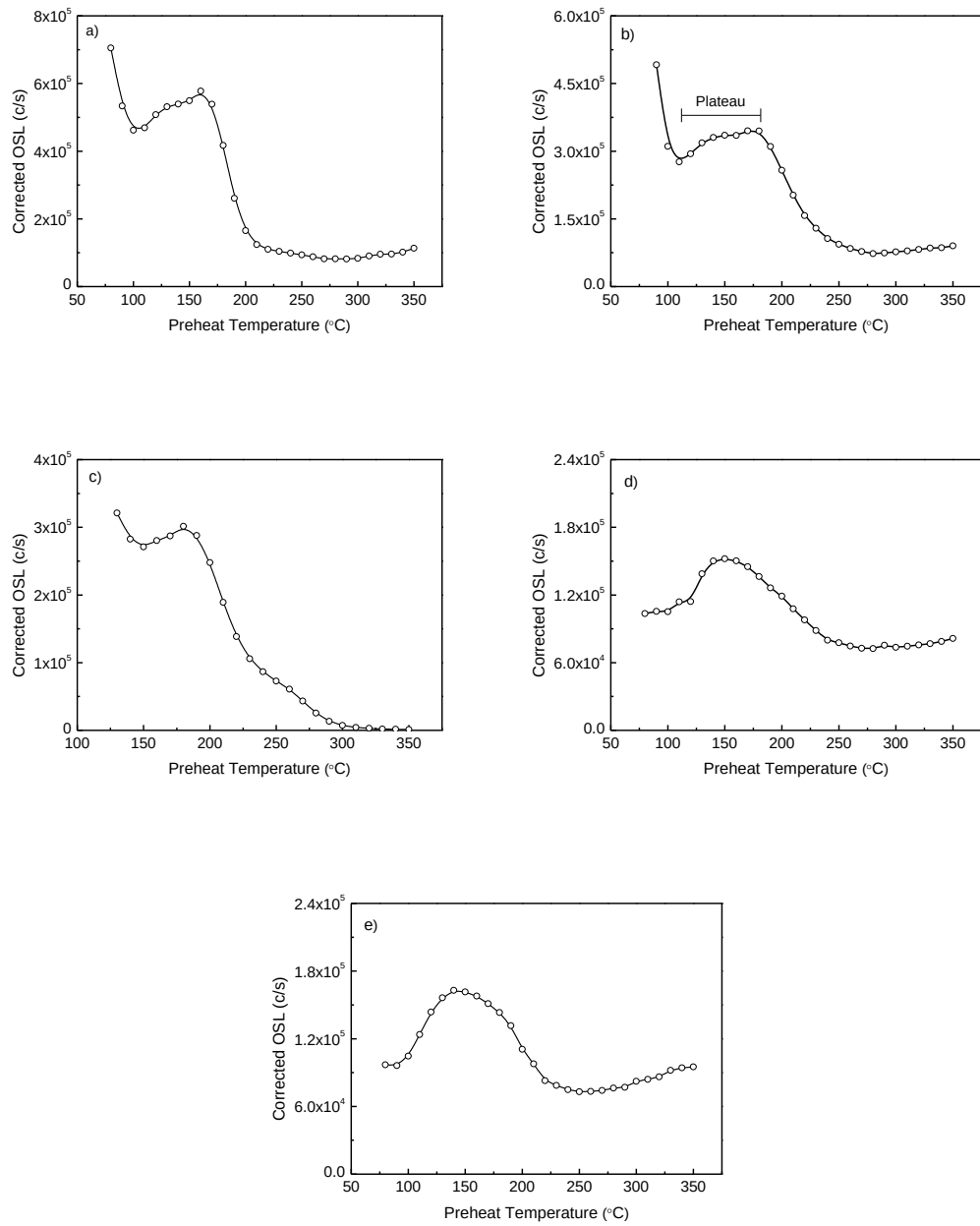
Figure 6.3 OSL responses of natural fluorites as a function of preheat temperature: a) Y-Fluorite, b) G-Fluorite, c) K-Fluorite, d) V-Fluorite, e) T-Fluorite.
