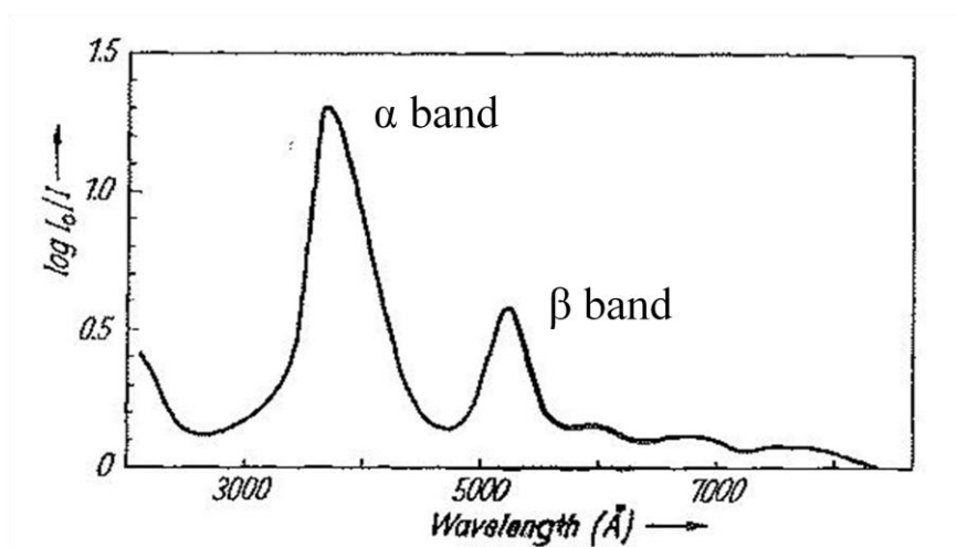
Figure 4.2 The optical absorption spectrum of an additively colored \text{CaF}_2 crystal at 300 °K (After, Arends, 1964).
