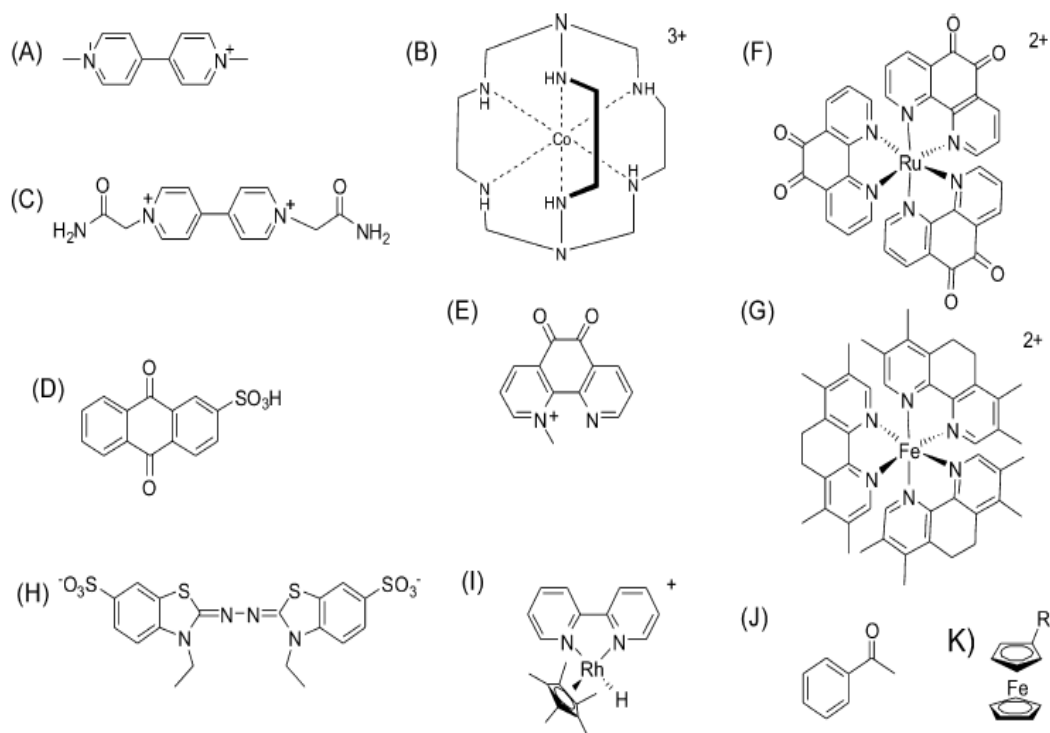
Figure 18: Substances used as electron shuttles (mediators) in electroenzymatic synthesis: (A) methyl viologen MV, (B) cobalt sepulchrate CoSep, (C) carboxamidomethyl viologen CAV, (D) anthraquinone 2-sulfonate AQ-2-S, (E) N-methyl-1,10-phenanthroline-5,6-dione, (F) tris(phenanthroline-5,6-dione)Ru(II), (G) tris(3,4,7,8-phenanthroline)Fe(II) Fe(tmphen)3, (H) 2,2'-azinobis(3-ethylbenzothiazoline)-6-sulfonate ABTS, (I) (2,2'-bipyridyl)(pentamethylcyclopentadienyl) rhodium complex, (J) acetophenone, (K) ferrocene derivatives
