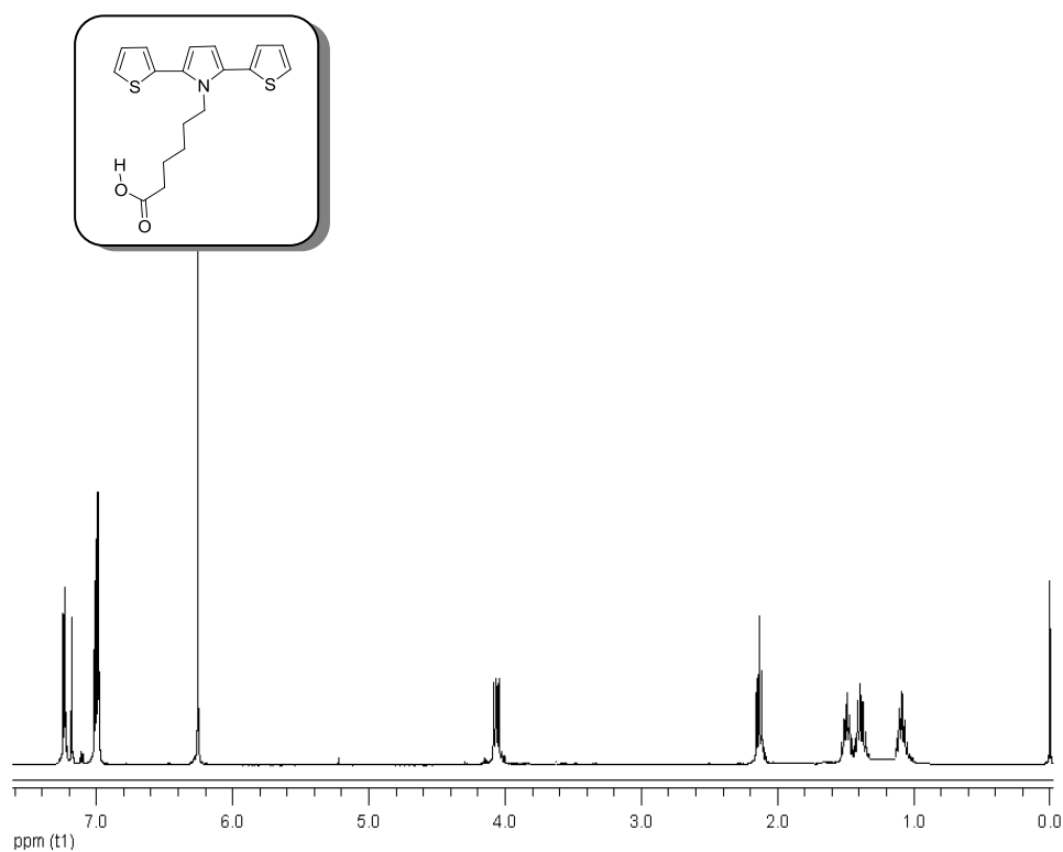
Figure A. 35 ^1\text{H} -NMR spectrum of (20)
