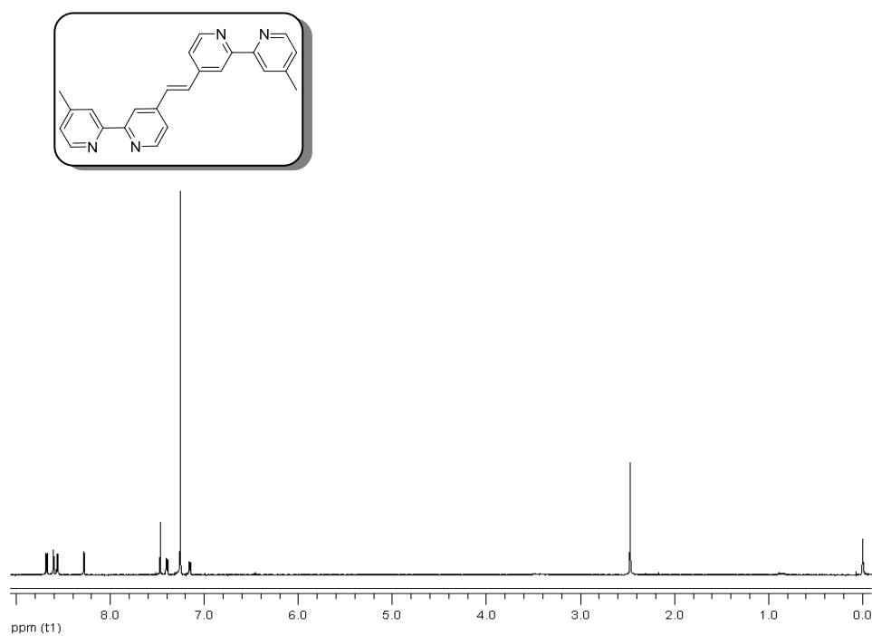
Figure A. 21 ^1\text{H} -NMR spectrum of (13)
