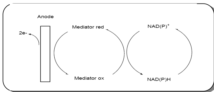
Figure 17: Indirect electrochemical method
