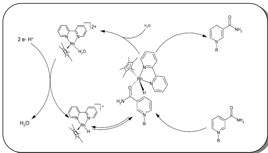
Figure 19: Mechanism of the regiospecific reduction of \text{NAD(P)}^+ by [\text{Cp}^*\text{Rh}(\text{bpy})(\text{H}_2\text{O})]^{2+} . The catalytically active Hydridorhodium complex [\text{Cp}^*\text{Rh}(\text{bpy})\text{H}]^+ is regenerated from its oxidized form either electrochemically (-750 mV vs Ag/AgCl) or via formate. The formation of an intermediate Rh-NAD complex was postulated to explain the high specificity of the hydride transfer .
