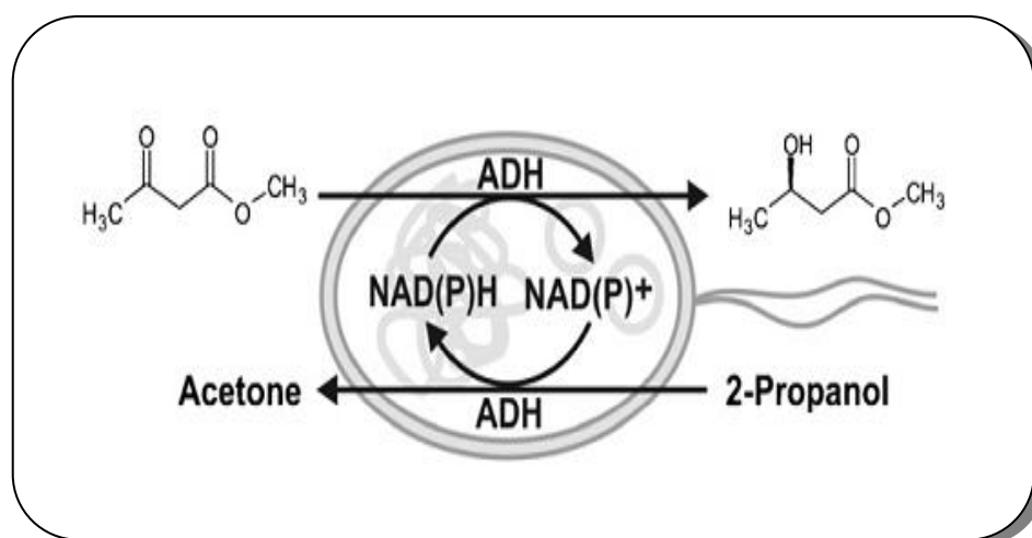
Figure 10: Reduction of methyl acetoacetate using alcohol dehydrogenase (ADH) in a substrate-coupled cofactor regeneration approach
