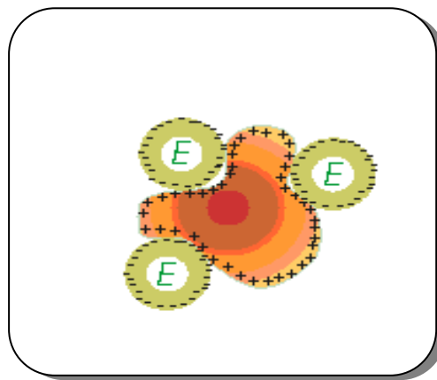
Figure 20: Enzyme (E) bound to a carrier by adsorption
