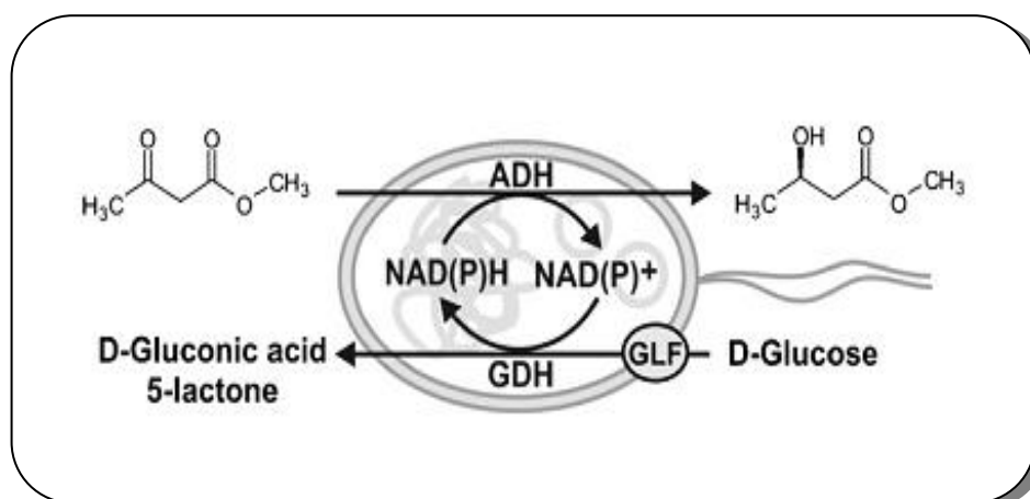
Figure 13: Reduction of methyl acetoacetate using alcohol dehydrogenase (ADH) with enzyme-coupled cofactor regeneration by glucose dehydrogenase (GDH).
