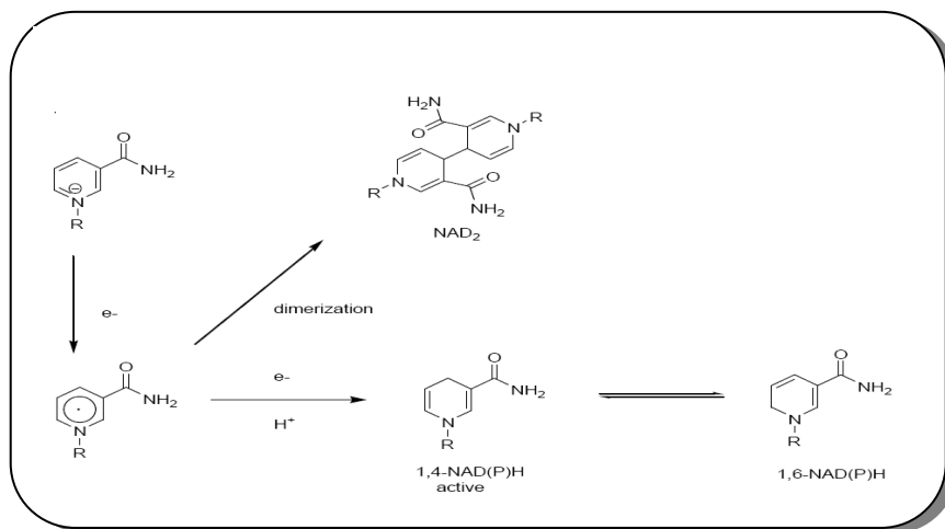
Figure 16: Formation of 1, 4-NAD (P) H and side products in direct electrochemical method
