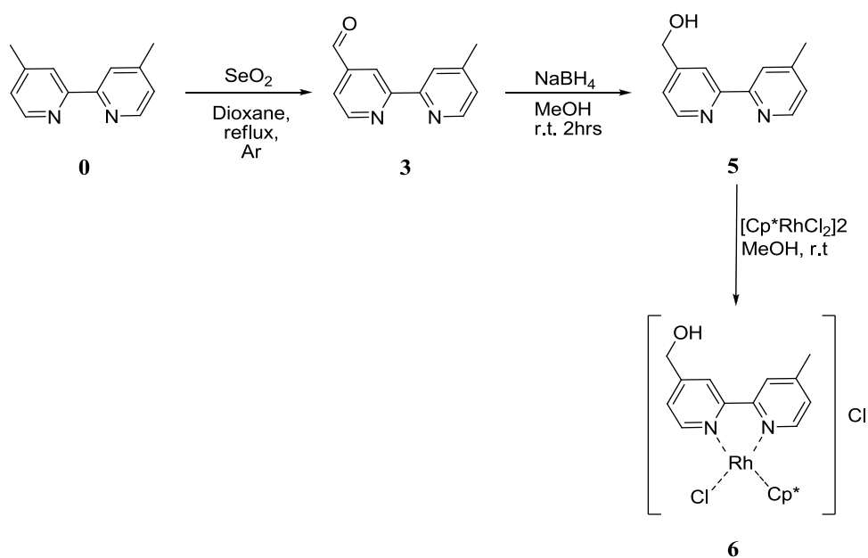
Figure 32: Synthesis of mediator 6
