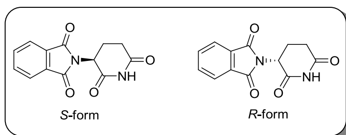
Figure 4: Enantiomers of thalidomide
