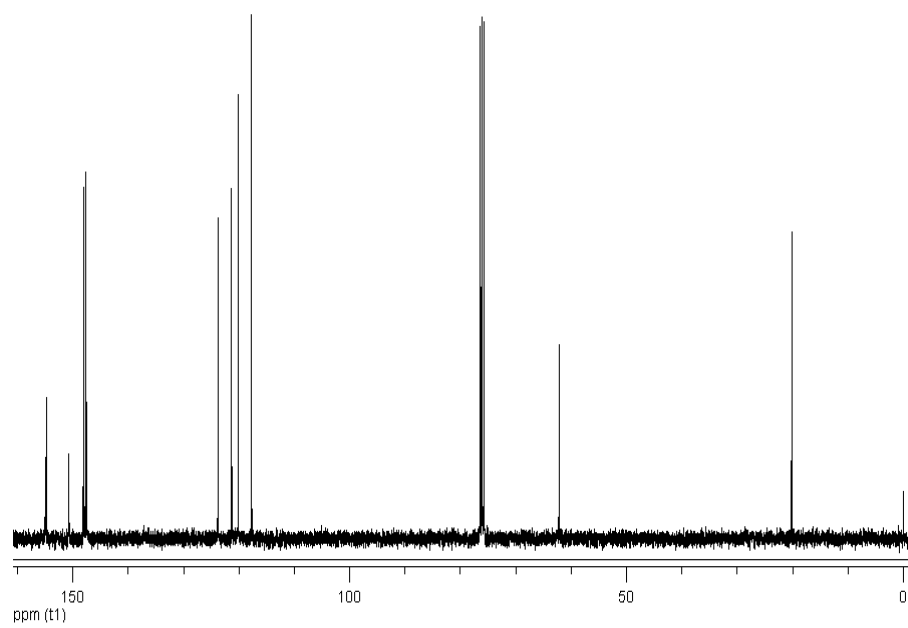
Figure A. 10 ^{13}\text{C} -NMR spectrum of (5)
