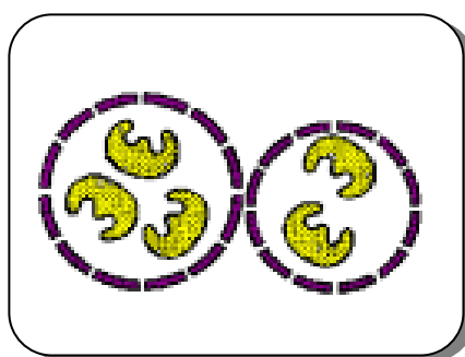
Figure 23: Enzyme confined in membrane
