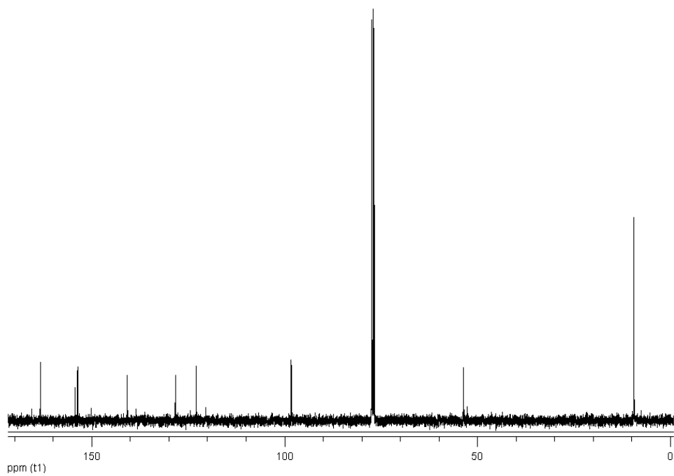
Figure A. 16 ^{13}\text{C} -NMR Spectrum of (9)
