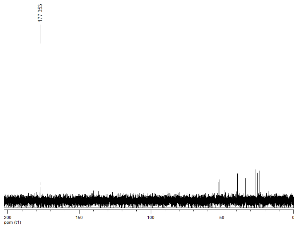
Figure A. 28 ^{13}\text{C} -NMR Spectrum of (16)
