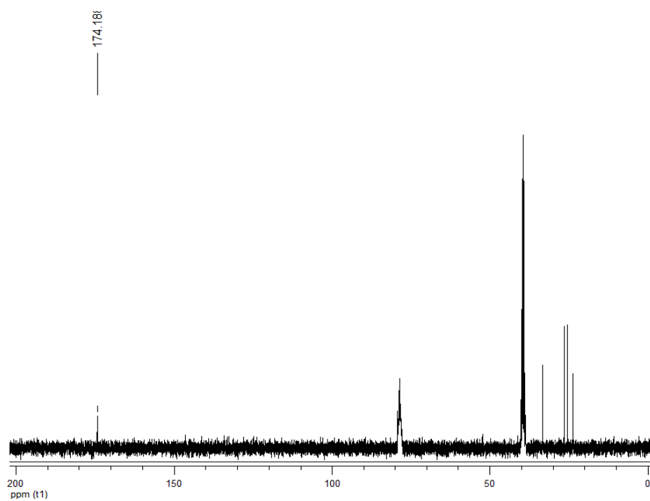
Figure A. 26 ^{13}\text{C} -NMR Spectrum of (15)
