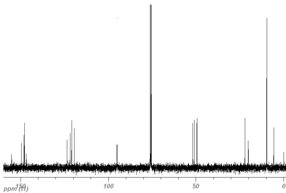
Figure A. 20 ^{13}\text{C} -NMR Spectrum of (11)
