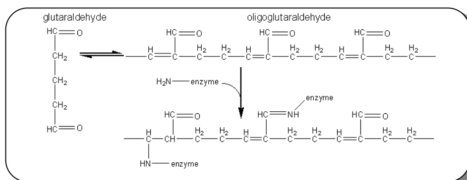
Figure 21: Coupling of glutaraldehyde with enzyme
