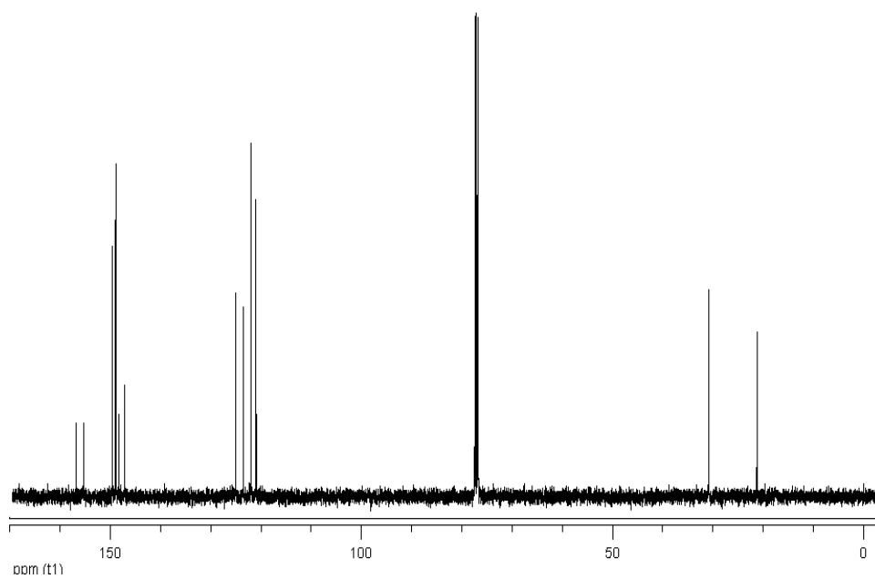
Figure A. 2 ^{13}\text{C} -NMR spectrum of (1)
