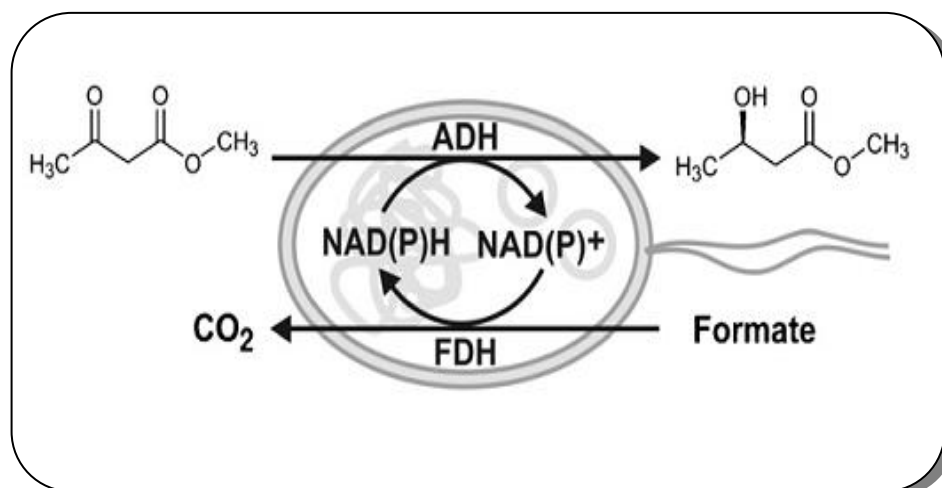
Figure 12: Reduction of methyl acetoacetate using alcohol dehydrogenase (ADH) with enzyme-coupled cofactor regeneration by formate dehydrogenase (FDH)
