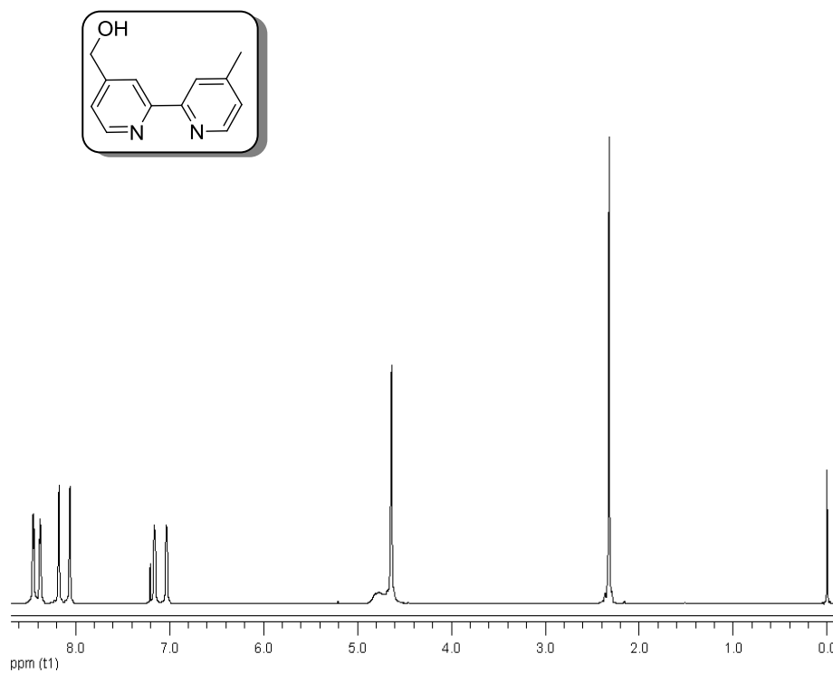
Figure A. 9 ^1\text{H} -NMR spectrum of (5)
