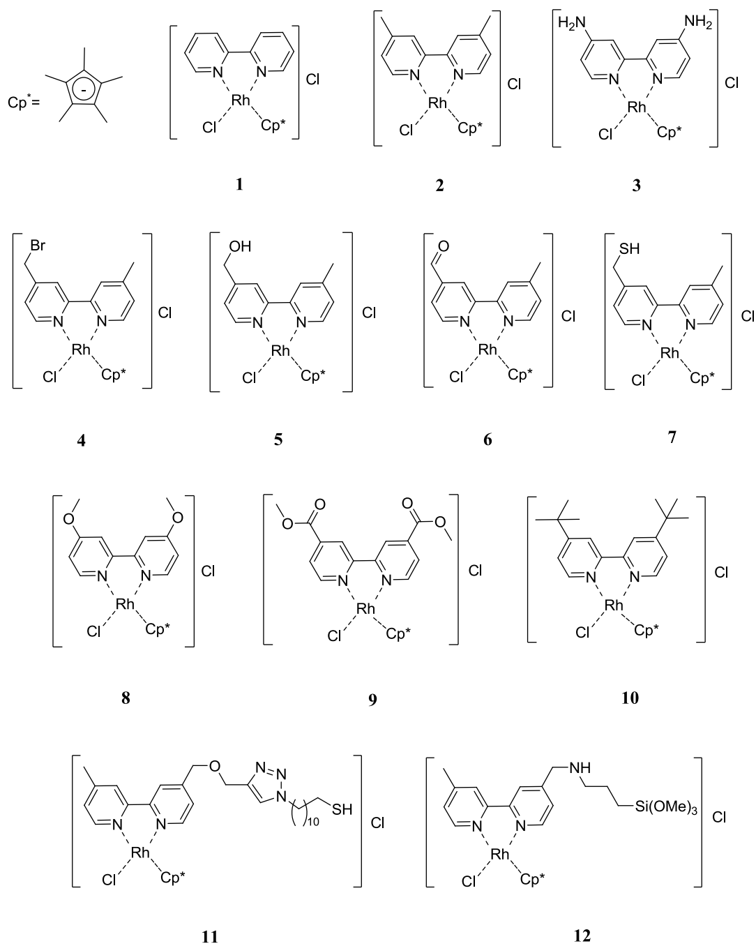
Figure 38: Bipyridine complex mediators
