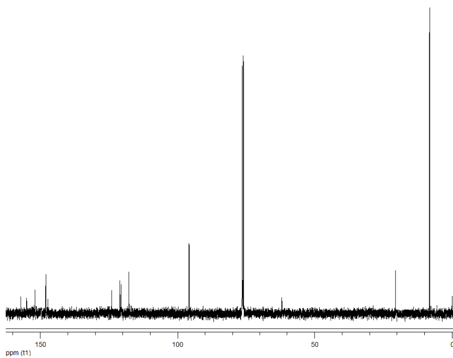
Figure A. 12 ^{13}\text{C} -NMR spectrum of (6)
