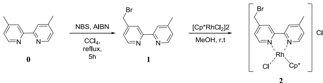
Figure 29: Synthesis of mediator 2
