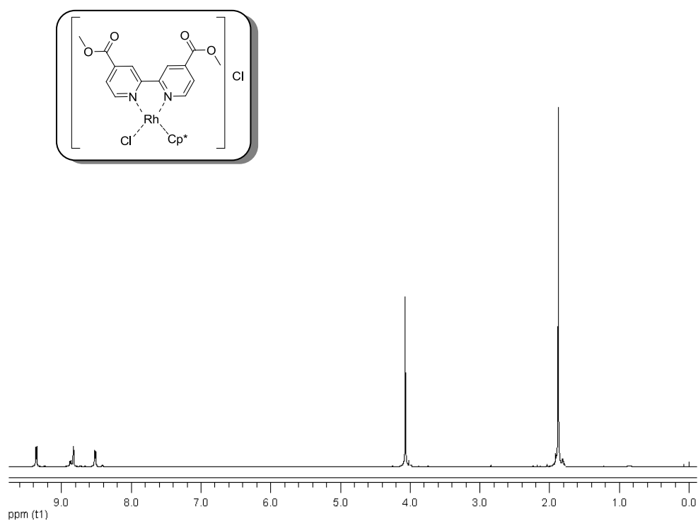
Figure A. 15 ^1\text{H} -NMR spectrum of (9)
