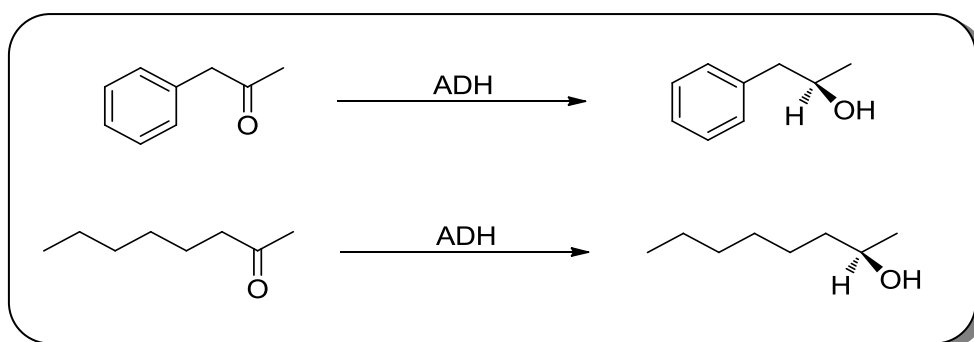
Figure 6: Reaction schemes for the synthesis of (R)-1-phenyl-2-propanol and (R)-2-octanol (ADH, alcohol dehydrogenase;
