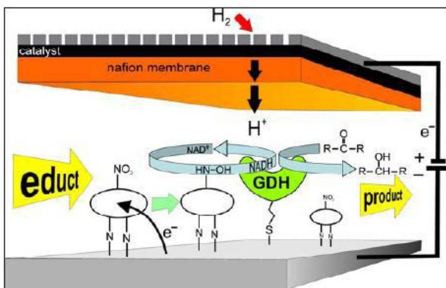
Figure 24: Model for electrochemical reactor
