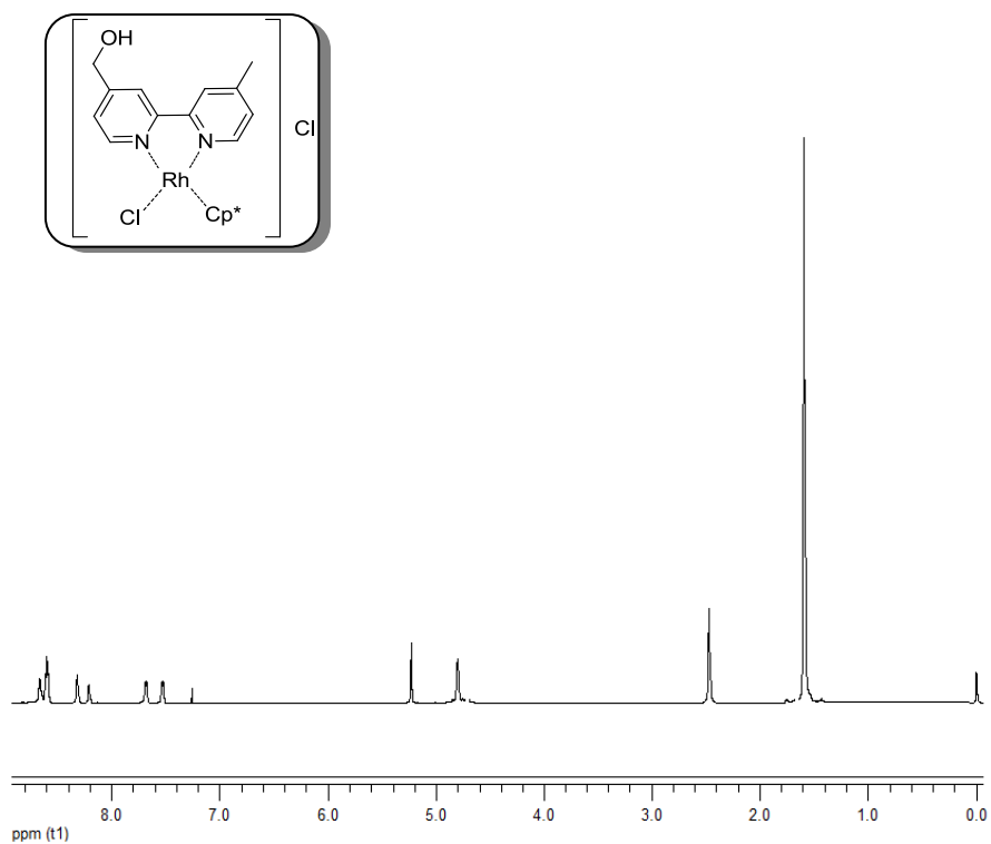
Figure A. 11 ^1\text{H} -NMR spectrum of (6)
