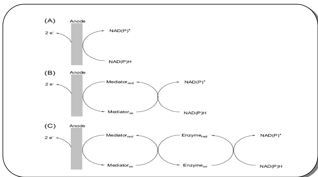
Figure 14: NAD (P) + -dependent oxidation reactions: (A) direct electrochemical regeneration, (B) indirect electrochemical regeneration, (C) enzyme-coupled electrochemical regeneration
