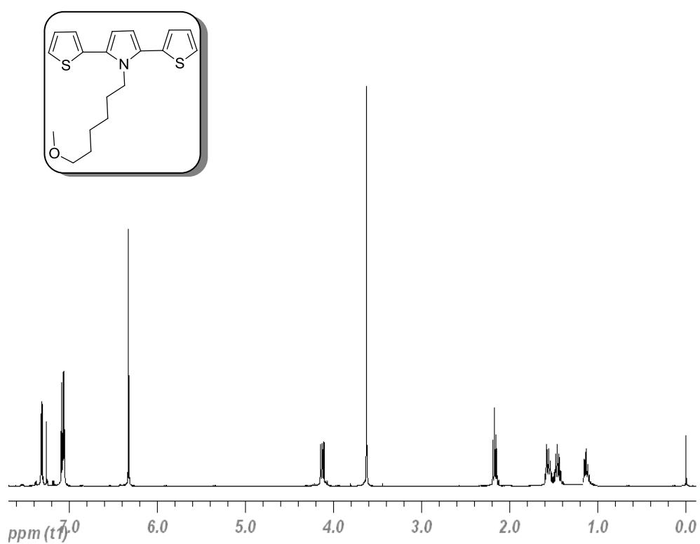
Figure A. 33 ^1\text{H} -NMR spectrum of (19)
