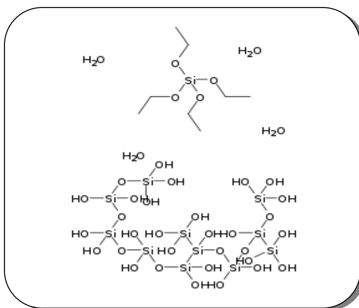
Figure 35: TEOS, water and polymerized Sol-gel
