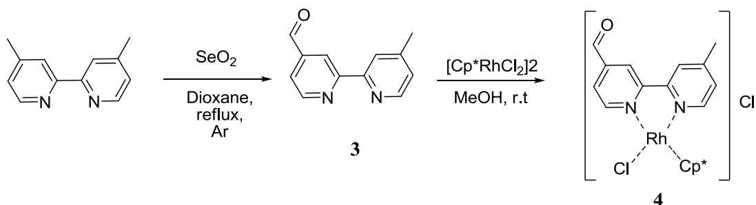
Figure 31: Synthesis of mediator 4
