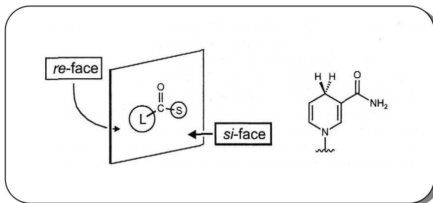
Figure 8: Delivery of the “hydride” from NADH to the re or si side of a prochiral ketone yielding either ( S )- or ( R )-alcohols. Depending on the dehydrogenase involved either the pro ( R )- or the pro ( S )-hydrogen at C-4 of the nicotinamide moiety of NAD(P)H is selectively transferred in the course of the reduction. L denotes the larger and S the smaller substituent at the central carbon.
