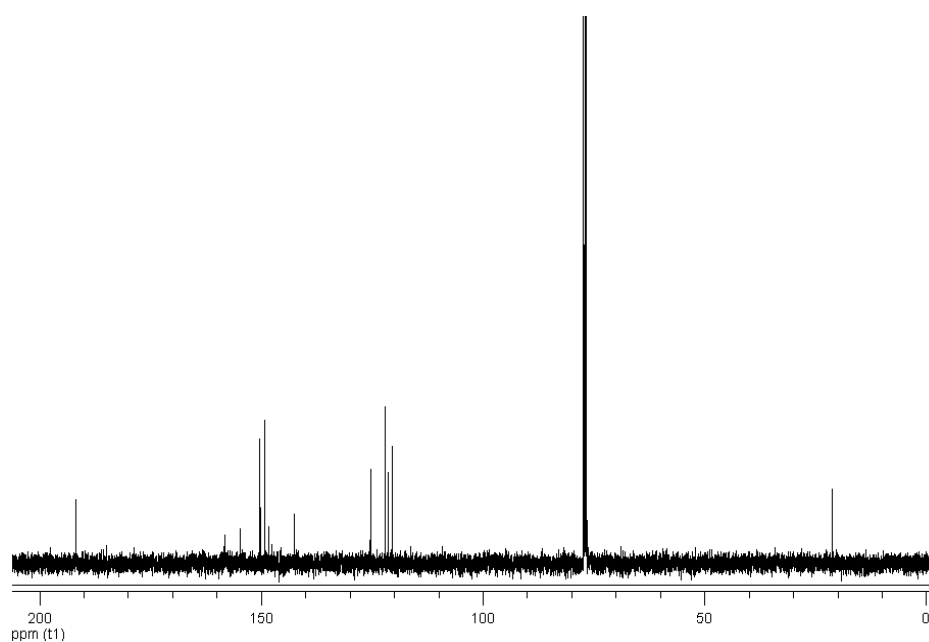
Figure A. 6 ^{13}\text{C} -NMR spectrum of (3)
