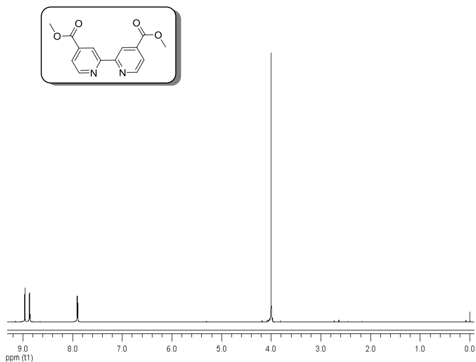
Figure A. 13 ^1\text{H} -NMR spectrum of (8)
