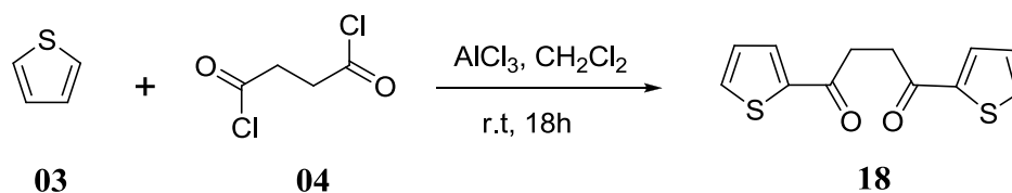
Figure 45: Synthesis of intermediate 18
