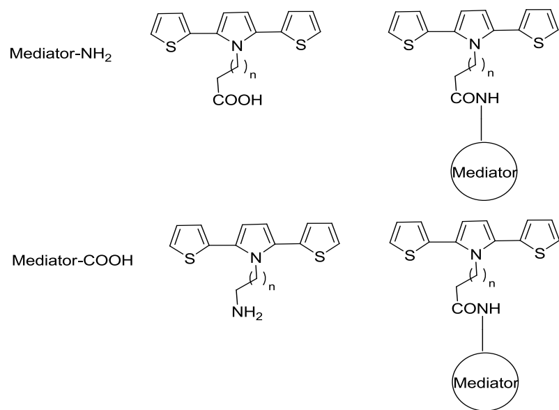
Figure 42: Reaction of the mediators with SNS monomer
