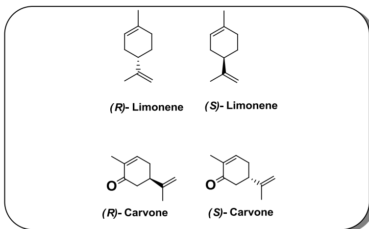
Figure 3: Enantiomers of limonene and carvone
