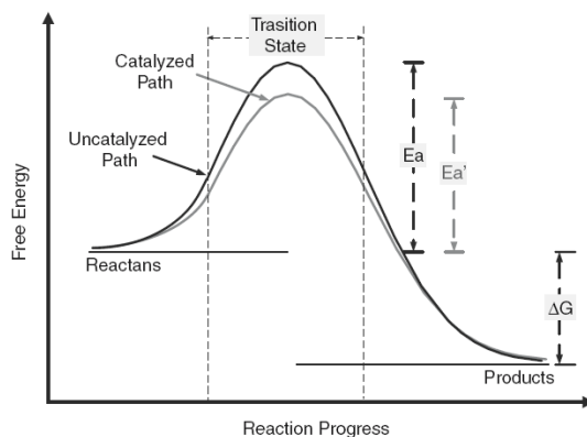
Figure 1: Mechanism of catalysis
