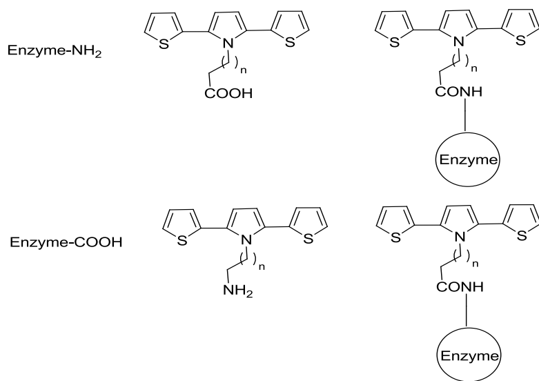
Figure 43: Reaction of the Enzymes with SNS monomer
