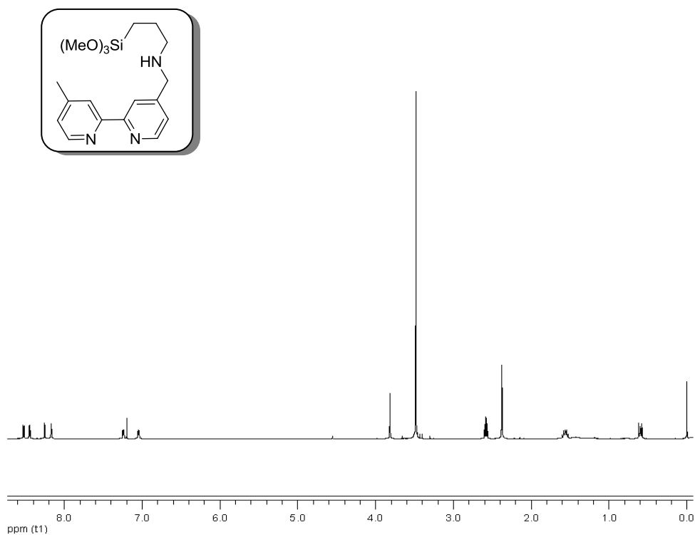
Figure A. 17 1 H-NMR spectrum of (10)
