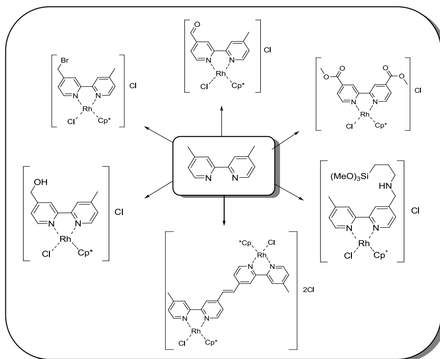
Figure 26: Synthesized pentamethylcyclopentadienyl rhodium bipyridine derivatives as mediators
