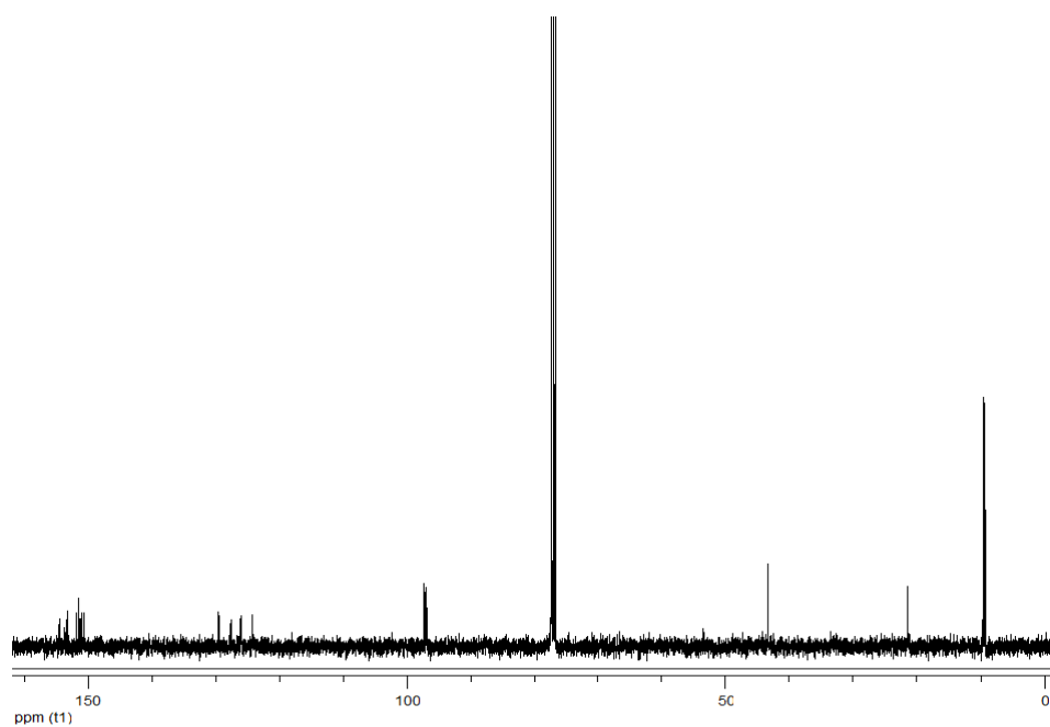
Figure A. 4 ^{13}\text{C} -NMR spectrum of (2)
