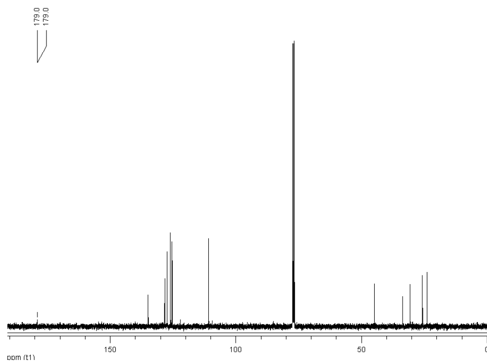
Figure A. 36 ^{13}\text{C} -NMR Spectrum of (20)
