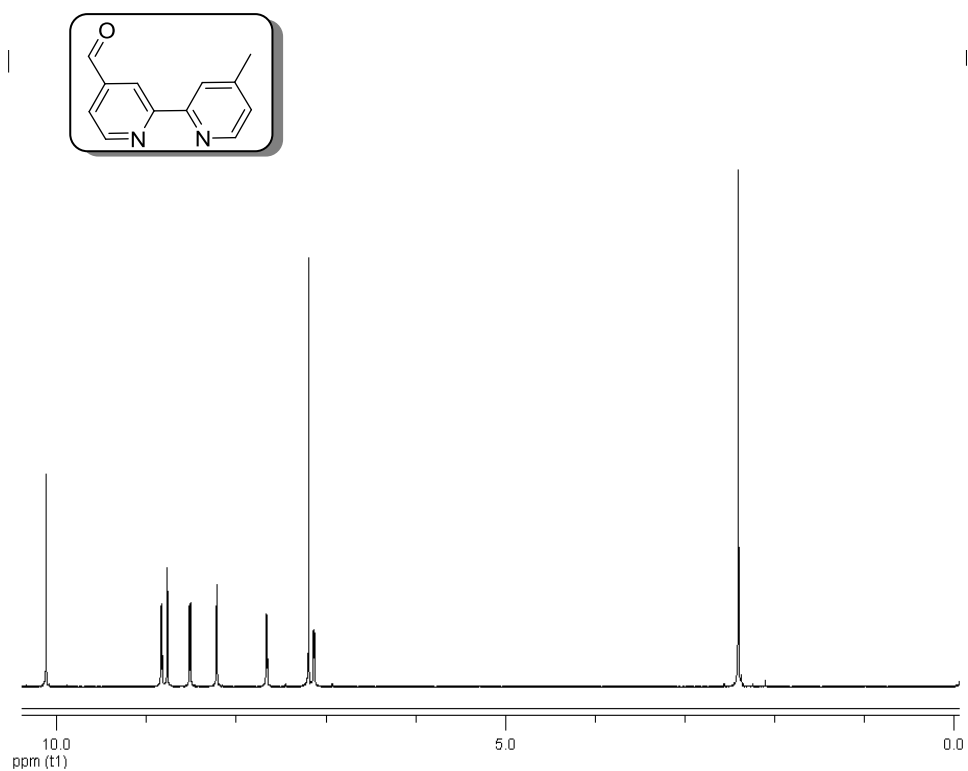
Figure A. 5 ^1\text{H} -NMR spectrum of (3)
