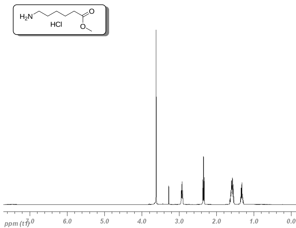
Figure A. 27 ^1\text{H} -NMR spectrum of (16)
