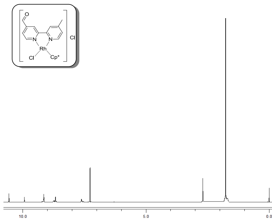
Figure A. 7 ^1\text{H} -NMR spectrum of (4)
