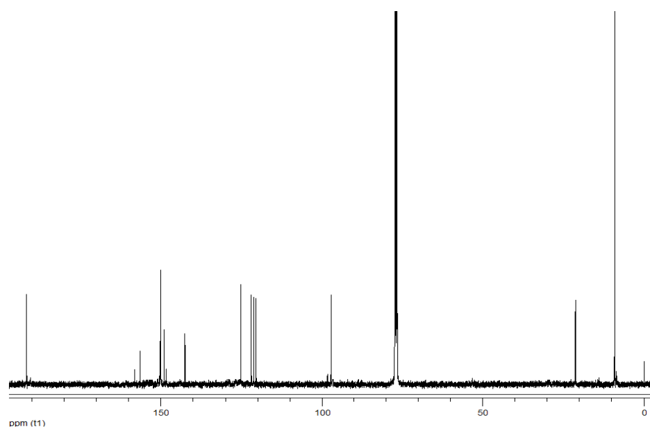
Figure A. 8 ^{13}\text{C} -NMR Spectrum of (4)
