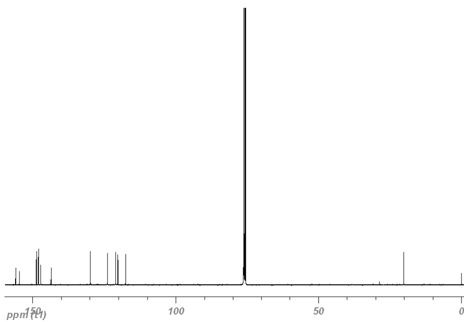
Figure A. 22 ^{13}\text{C} -NMR Spectrum of (13)
