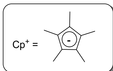
Figure 28: Pentamethylcyclopentadienyl anion
