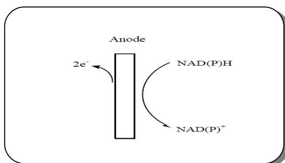
Figure 15: Direct electrochemical method
