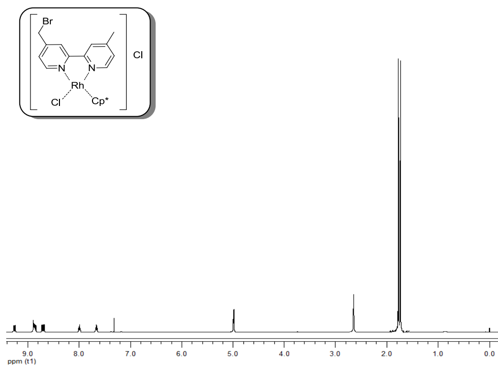
Figure A. 3 ^1\text{H} -NMR spectrum of (2)
