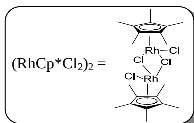
Figure 27: Rhodium complex
