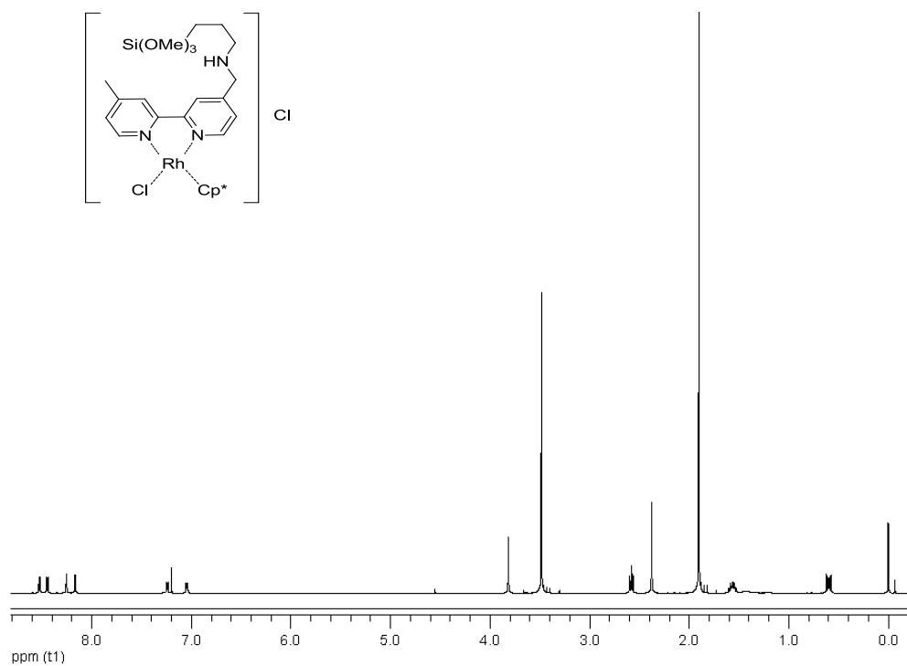
Figure A. 19 ^1\text{H} -NMR spectrum of (11)
