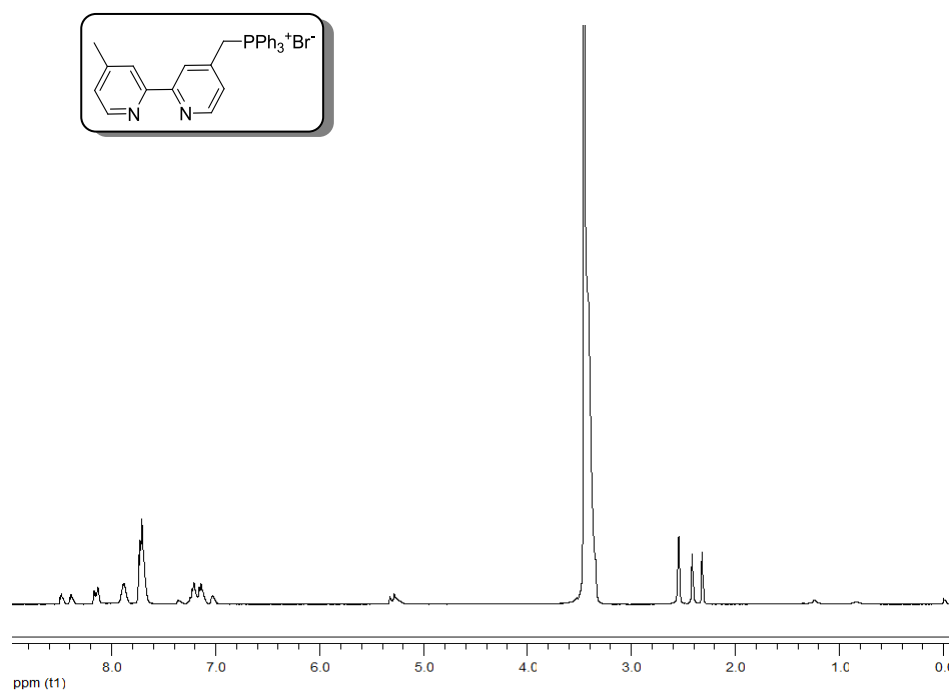
Figure A. 0 ^1\text{H} -NMR spectrum of (12)
