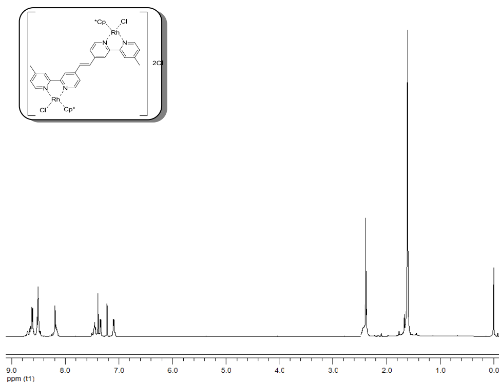
Figure A. 23 ^1\text{H} -NMR spectrum of (14)
