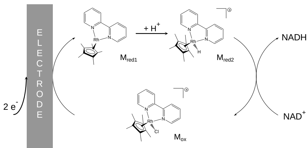
Figure 25: Mechanism of \text{NAD}^+ Reduction
