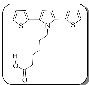
Figure 41: Conductive SNS monomer
