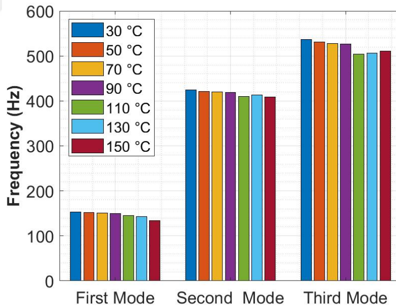
Figure 4.41: The Natural Frequencies of the Test Plate 3 with respect to Temperature ( 2^\circ\text{C/s} heating rate)
