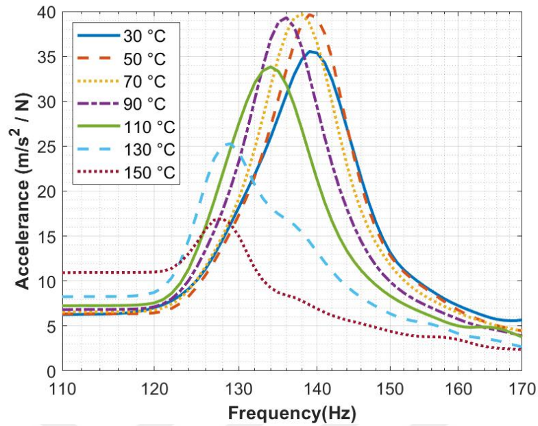
Figure 4.72: The Changes of the First Mode of the Test Plate 5 ( 1^\circ\text{C/s} heating rate)
