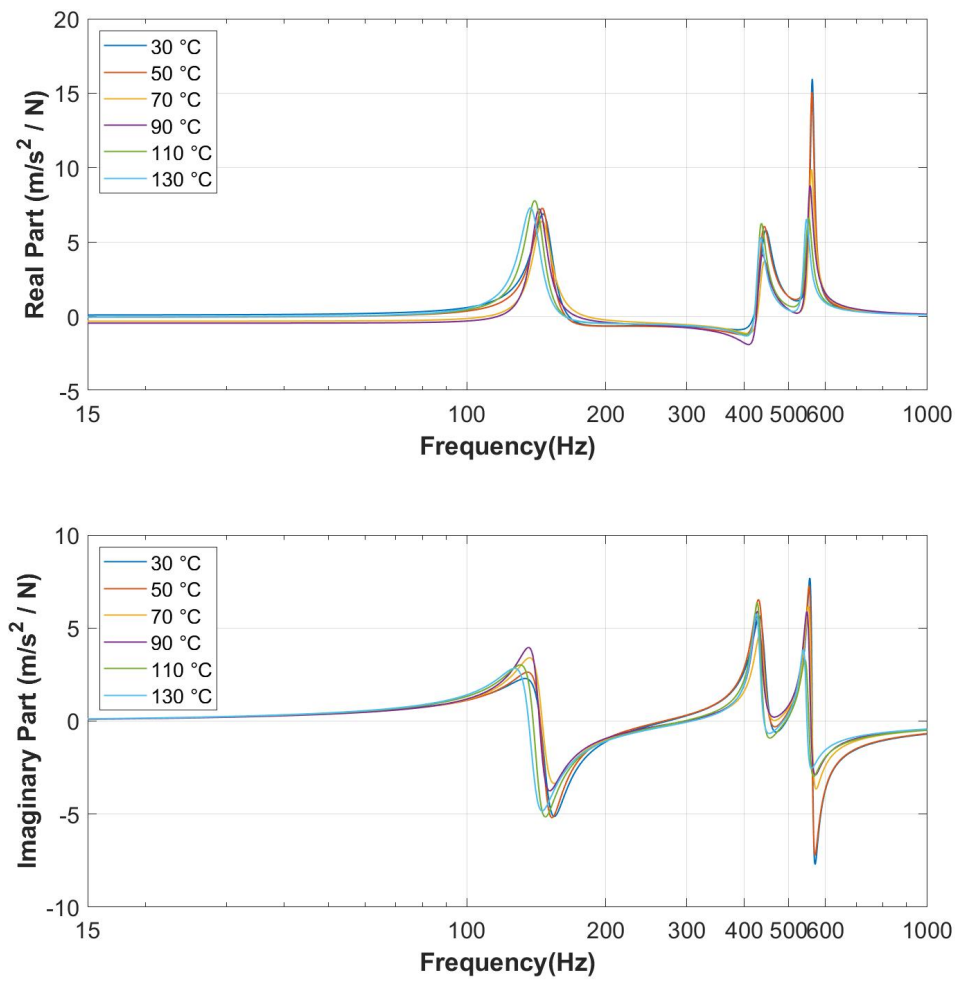
Figure 4.14: The Real and Imaginary Part of FRFs of the Test Plate 1 under Elevated Temperature ( 2^\circ\text{C/s} heating rate)
