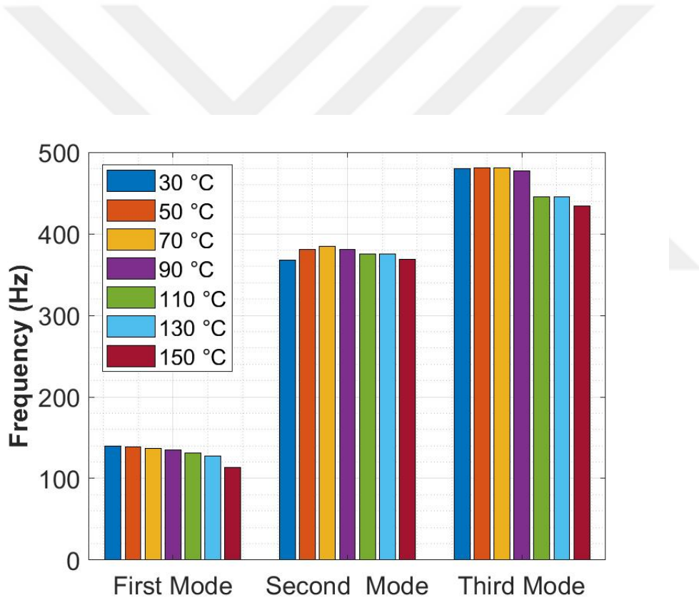
Figure 4.51: The Change of Natural Frequencies of the Test Plate 4 under Thermal Environment
