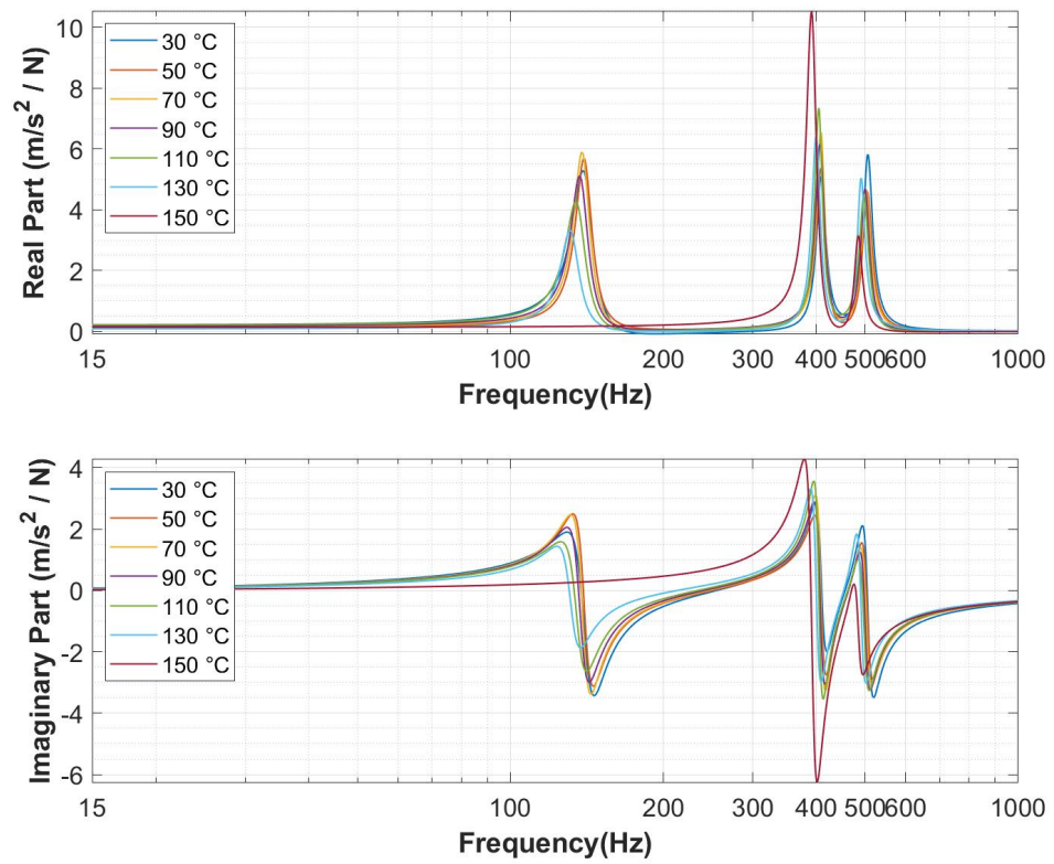
Figure 4.64: The Real and Imaginary Part of FRFs of the Test Plate 5 under Elevated Temperature ( 2^{\circ}\text{C/s} heating rate)
