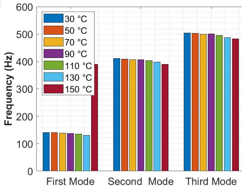
Figure 4.73: The Natural Frequencies of the Test Plate 5 with respect to Temperature ( 1^\circ\text{C/s} heating rate)
