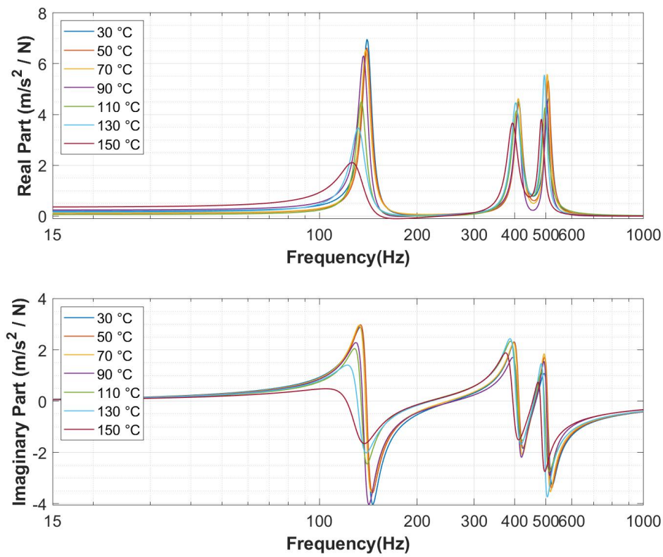
Figure 4.57: The Real and Imaginary Part of FRFs of the Test Plate 5 under Elevated Temperature ( 3^{\circ}\text{C/s} heating rate)
