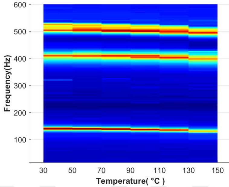
Figure 4.55: The Spectrogram of the Temperature dependent FRF changes of the Test Plate 5 ( 3^{\circ}\text{C/s} heating rate)
