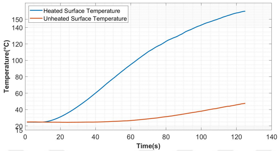
Figure 4.68: The Temperature values of the Test Plate 5 ( 1^{\circ}\text{C/s} heating rate)
