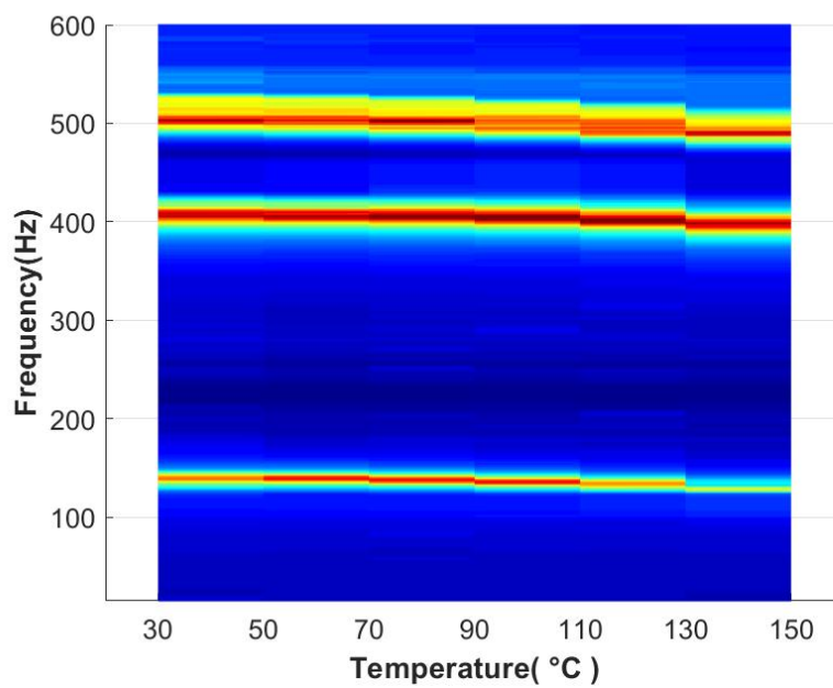
Figure 4.69: The Spectrogram of the Temperature Dependent FRF changes of the Test Plate 5 ( 1^{\circ}\text{C/s} heating rate)
