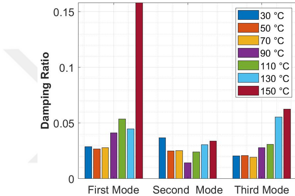
Figure 4.27: The Change of Damping Ratios of the Test Plate 2 under Thermal Environment
