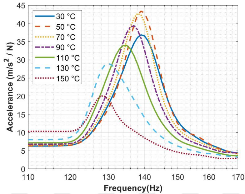
Figure 4.65: The Changes of the First Mode of the Test Plate 5 ( 2^\circ\text{C/s} heating rate)
