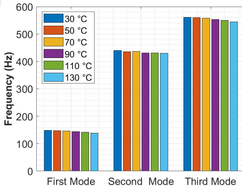
Figure 4.16: The Natural Frequencies of the Test Plate 1 with respect to Temperature ( 2^\circ\text{C/s} heating rate)
