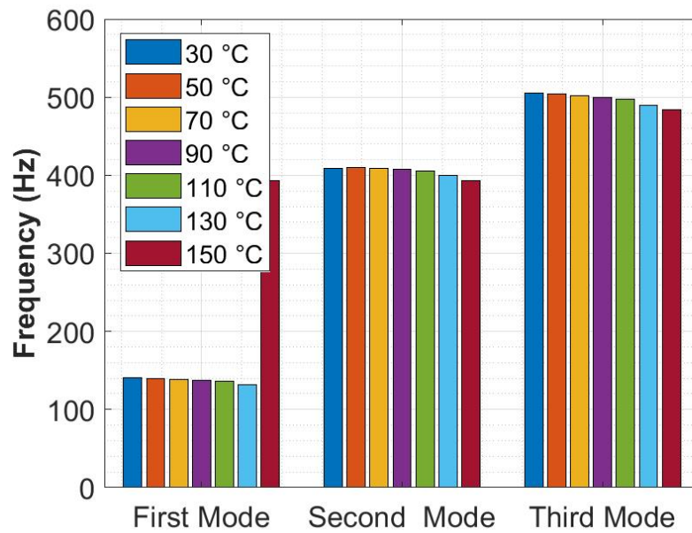
Figure 4.66: The Natural Frequencies of the Test Plate 5 with respect to Temperature ( 2^\circ\text{C/s} heating rate)
