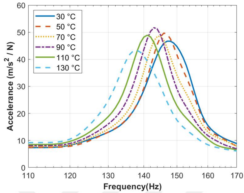
Figure 4.15: The Changes of the First Mode of the Test Plate 1 ( 2^\circ\text{C/s} heating rate)
