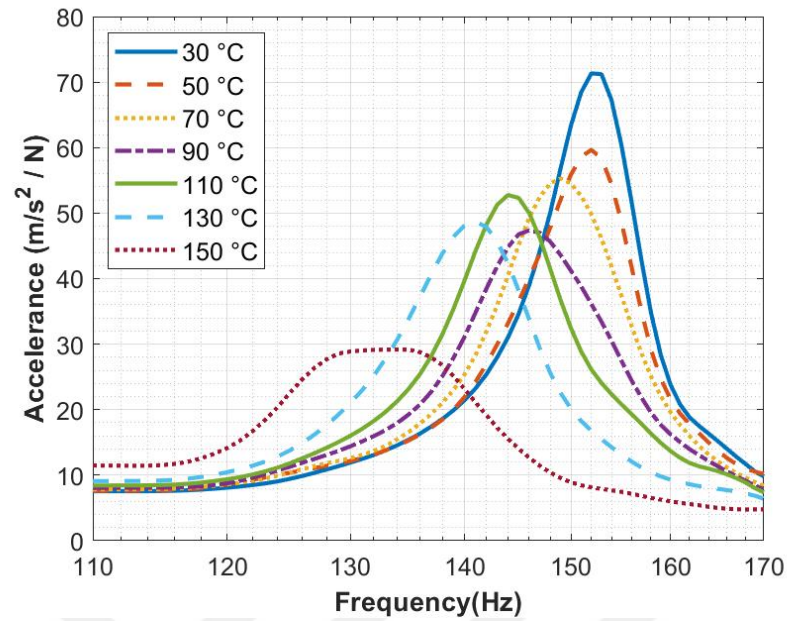
Figure 4.40: The Changes of the First Mode of the Test Plate 3 ( 2^\circ\text{C/s} heating rate)
