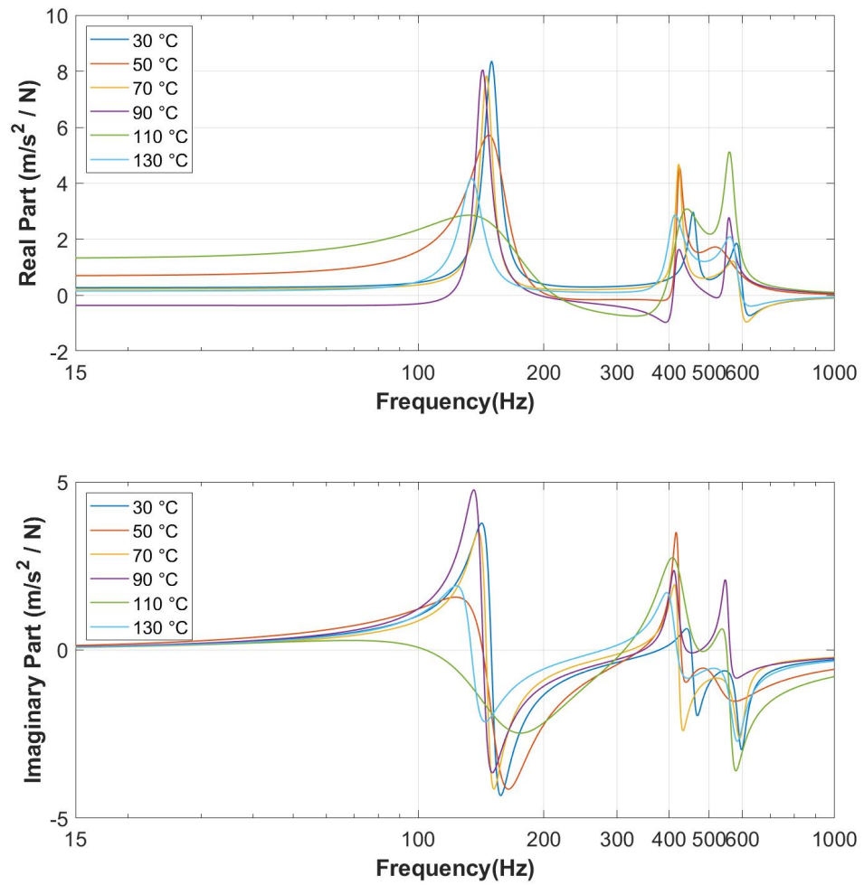
Figure 4.21: The Real and Imaginary Part of FRFs of the Test Plate 1 under the Elevated Temperature (1°C/s heating rate)
