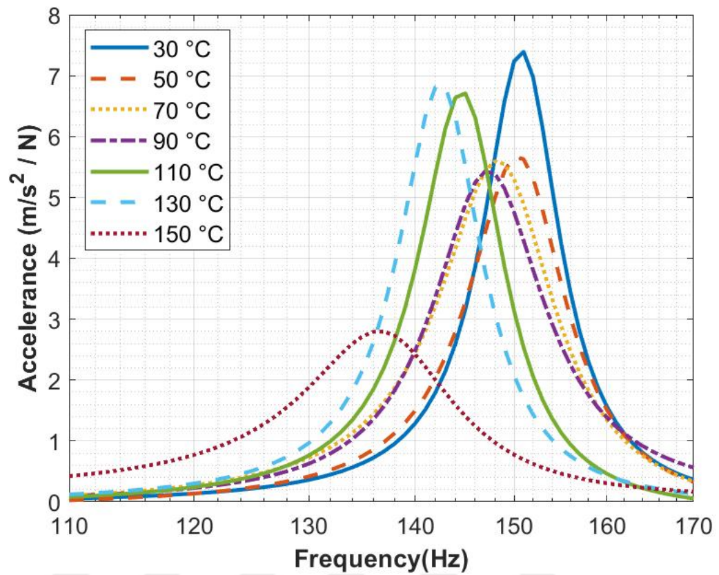
Figure 4.78: The Change of Vibration Response of the Test Plate 6 under Thermal Environment
