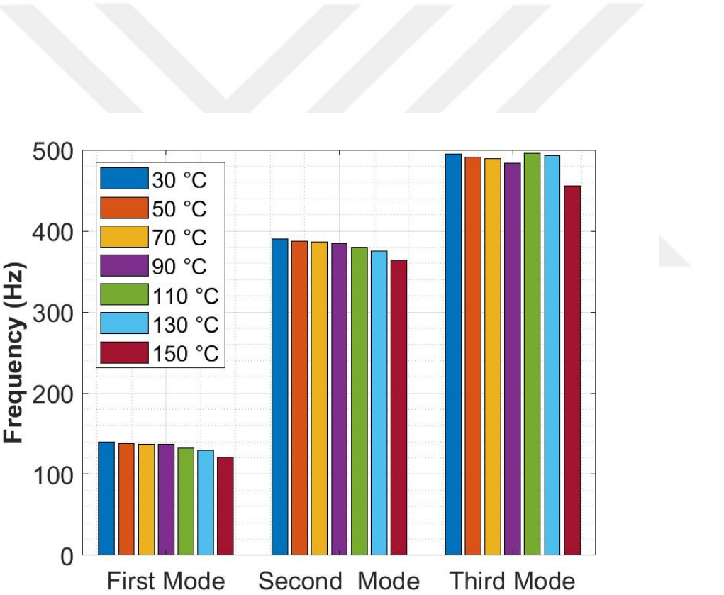
Figure 4.26: The Change of Natural Frequencies of the Test Plate 2 under the Thermal Environment
