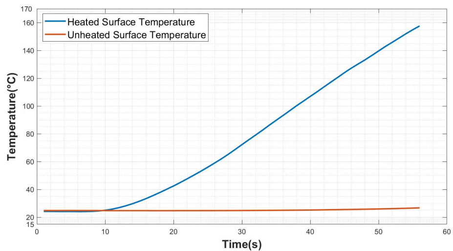
Figure 4.79: The Temperature values of the Test Plate 7 ( 3^{\circ}\text{C/s} heating rate)
