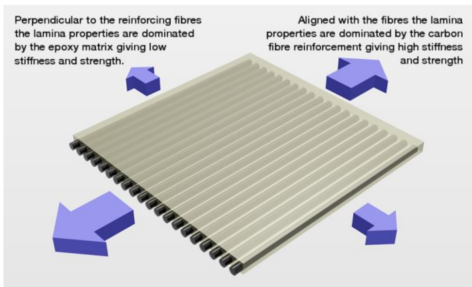
Figure 3.2: Lamina Directions [3]
