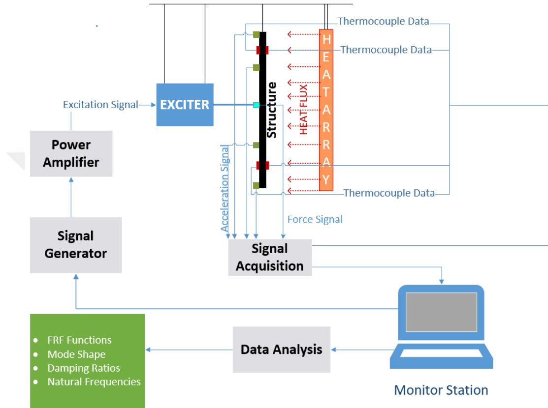
Figure 3.15: The Illustration of the Instrumentation of the Experimental Setup
