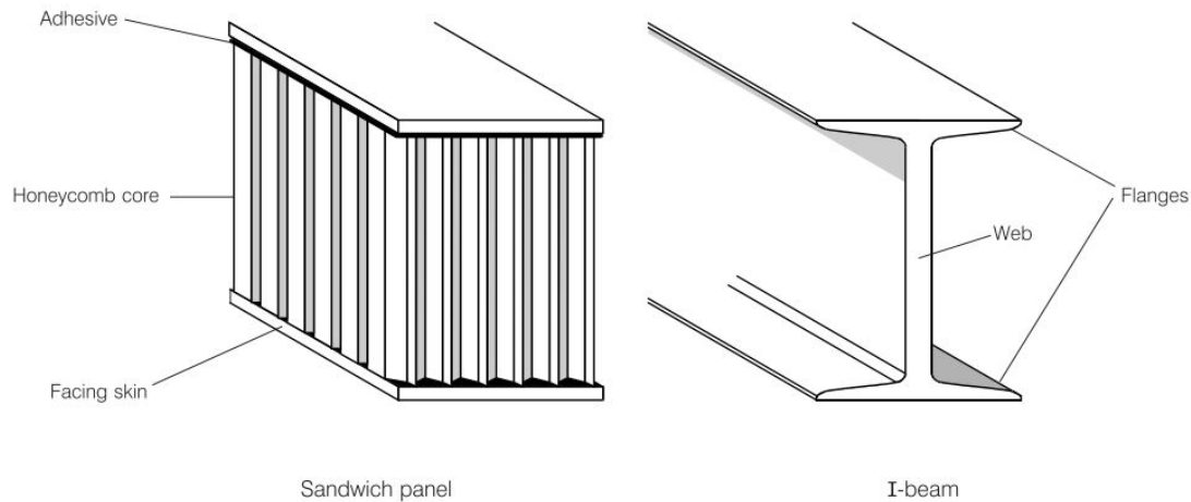
Figure 3.7: Hexagonal Core vs. I-Beam Structure[6]
