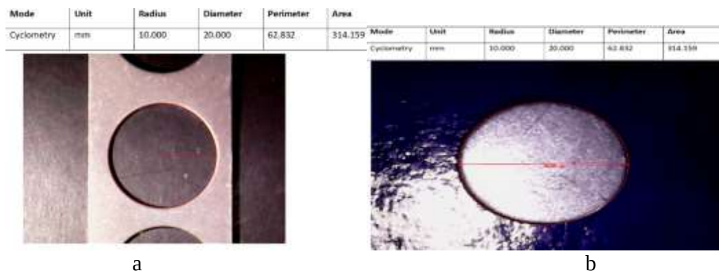
Figure 6.9. a) The effect of the punch 0^\circ on the product piercing, b) The effect of the punch 0^\circ on the product blanking.
