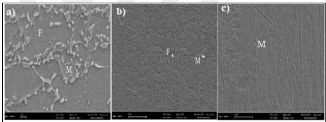
Figure 2.4. The microstructure of DP600 a) BM, b) HAZ and c) FZ [52].
