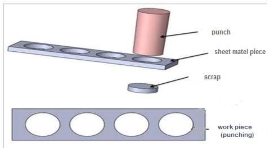
Figure 4.2. Punching sheet metal cutting operation (piercing) [86].
