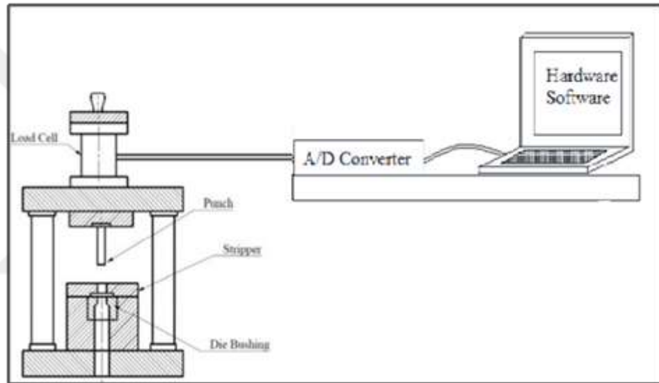
Figure 5.1. Schematic overview of the experimental set-up.
