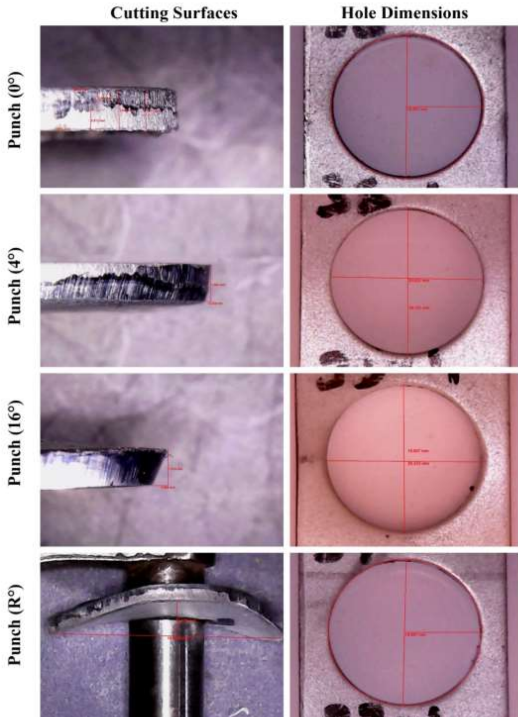
Figure 6.8. Cutting surfaces of punched parts with different punches and holes.
