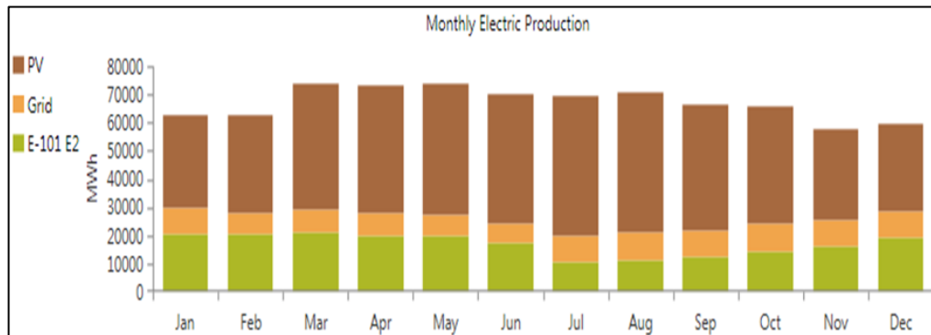
Figure 5.14. Monthly electric production for PV panels and wind turbine for MFZ HERS.
