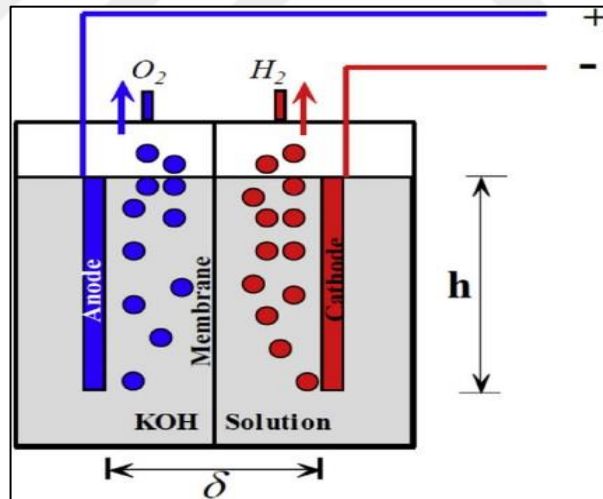
Figure 1.14. Electrolyzer Schematic [24].
