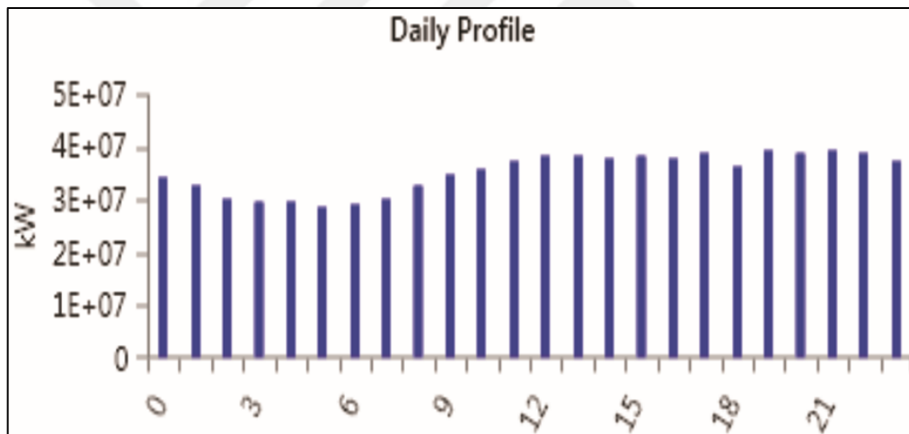
Figure 4.10. Hourly load profile for MFZ.
