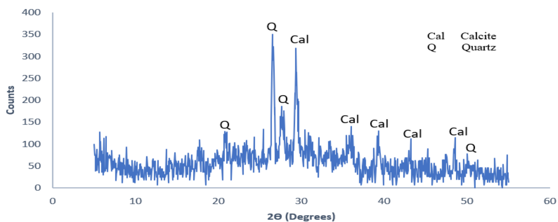
Figure 4.16. XRD analysis E-2 mixture after 28 days of ambient curing
