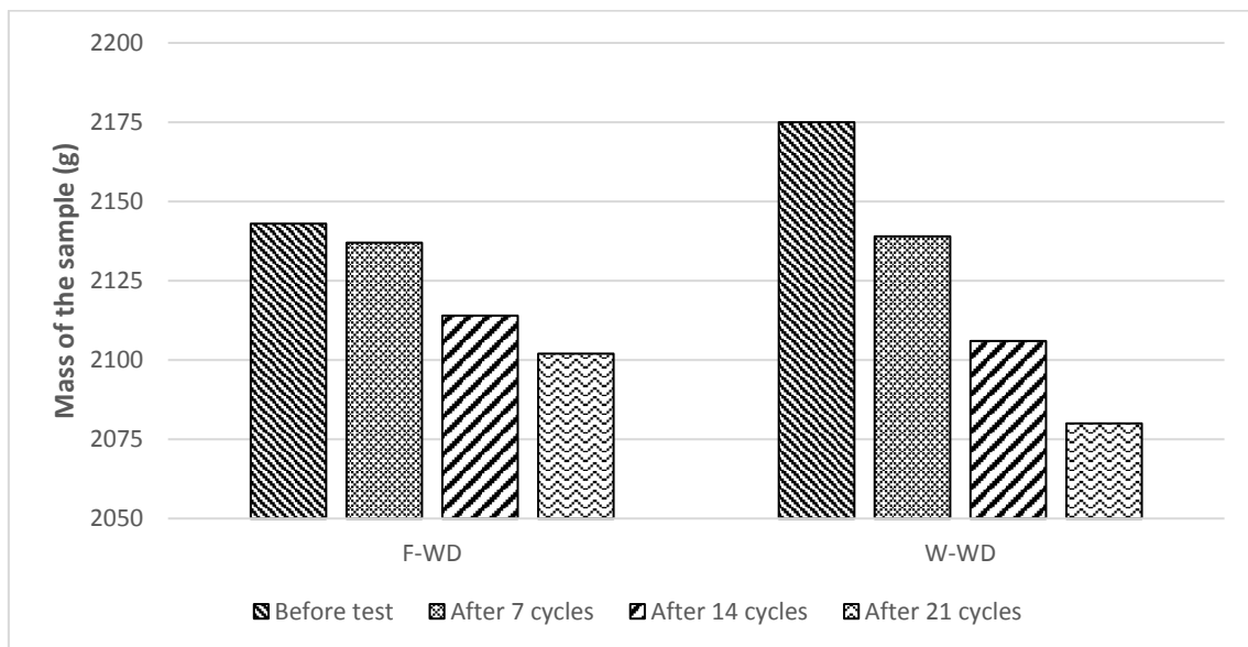
Figure 4.30. Masses of the samples for Wetting-Drying Cycles
