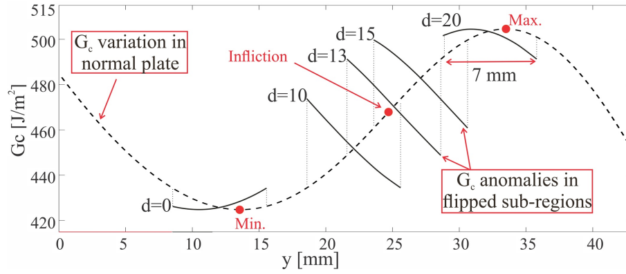
Figure 4.22: G_c variation in pristine (normal) plate and the plates with flipped sub-region
