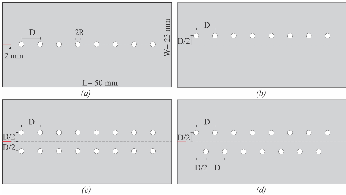
Figure 3.1: Geometric properties of homogeneous plates under dynamic loading with 2R=3L/100 and D=L/9
