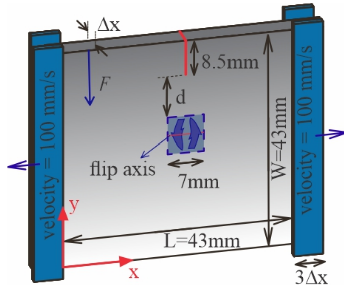
(a) Crack on stiff side
