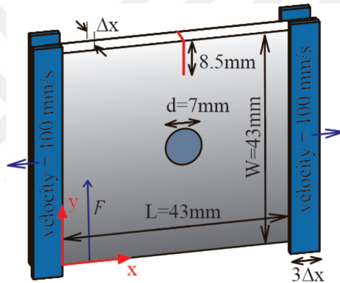
(b) Crack on compliant side
