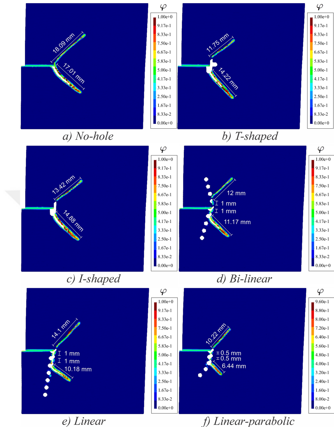
Figure 3.13: Crack surface and propagation length of the geometries under shear loading at 1350 th time-step
