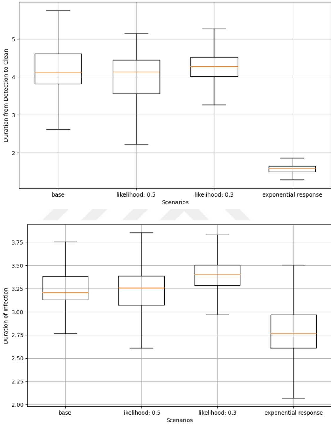
Figure 22. Boxplot of duration from detection to clean (top), Average infection duration (bottom)
