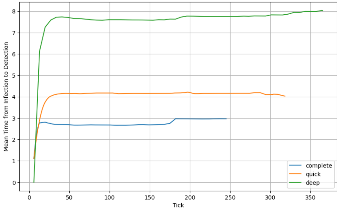
Figure 15. Average duration from infection to detected based on scan type
