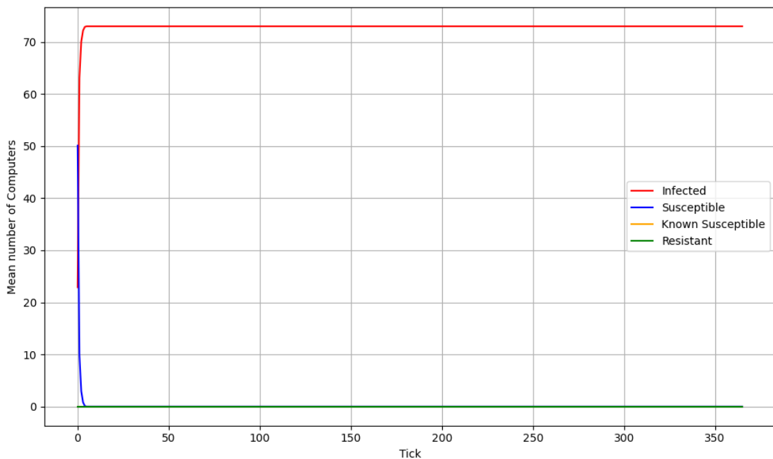
Figure 23. Number of components in each state for worst case scenario
