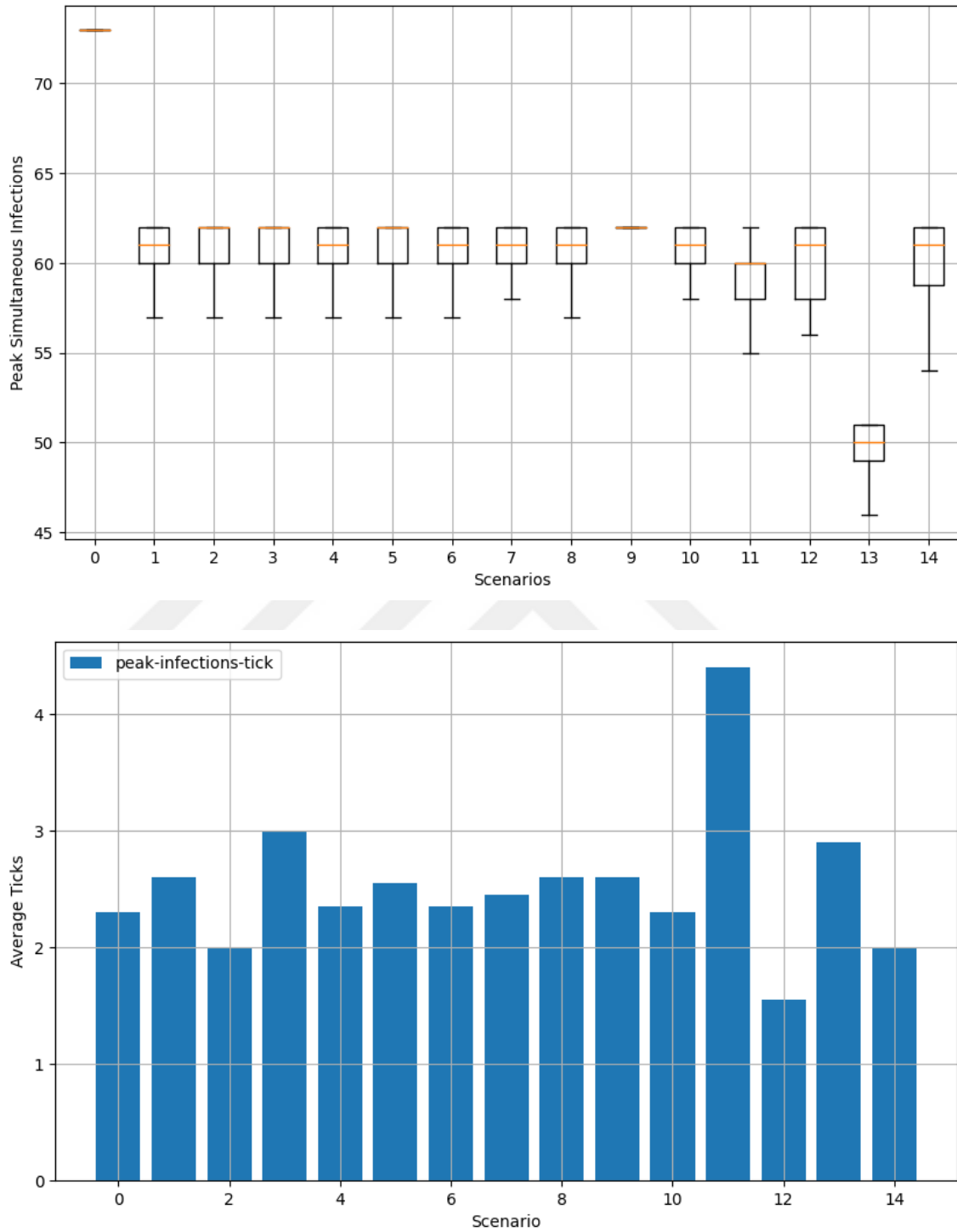
Figure 26. Peak simultaneous infections (top) and rate of spread (bottom) for all scenarios
