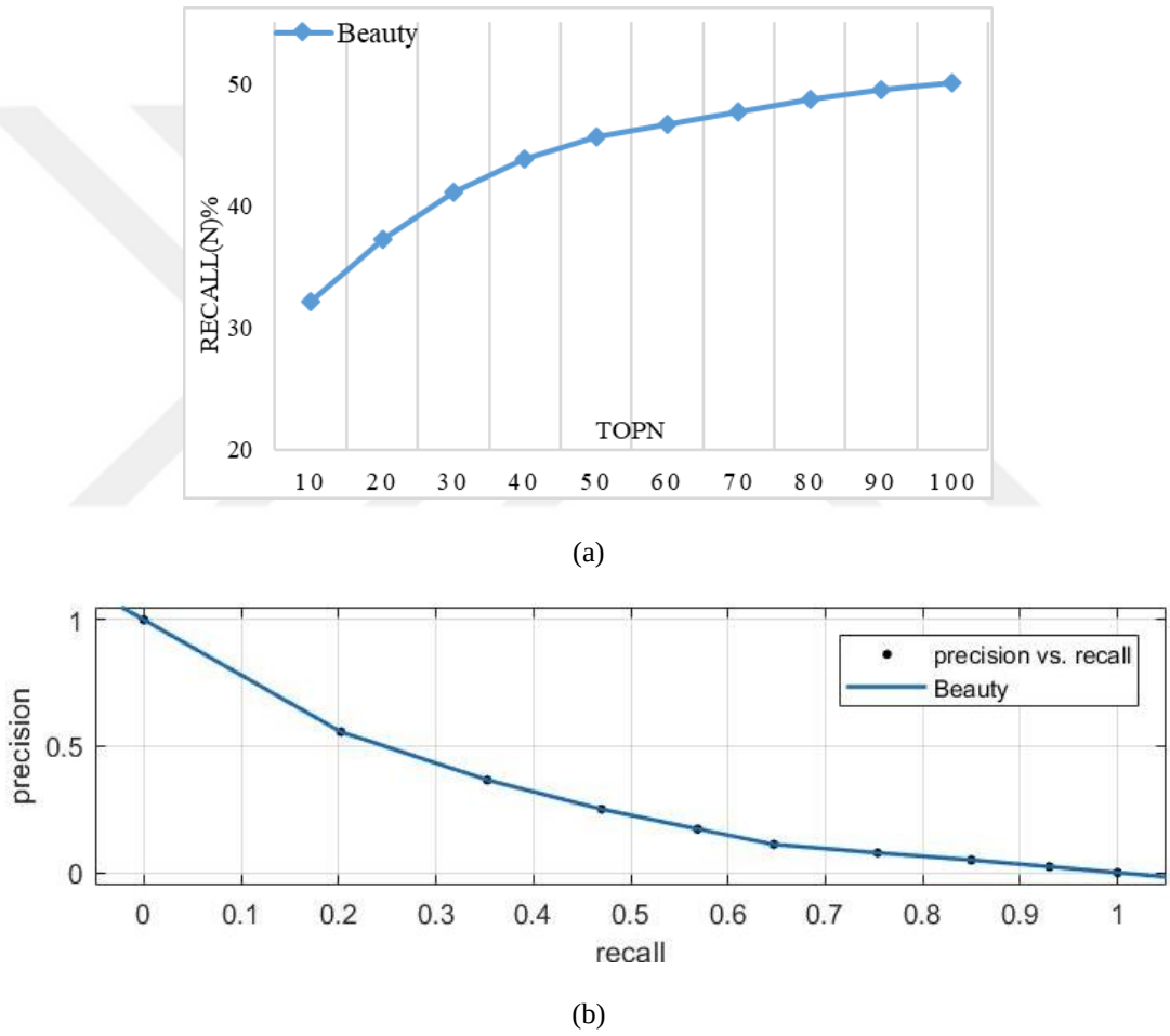
Figure 6.16. Beauty: (a) recall-at-N and (b) precision-versus-recall on all items
