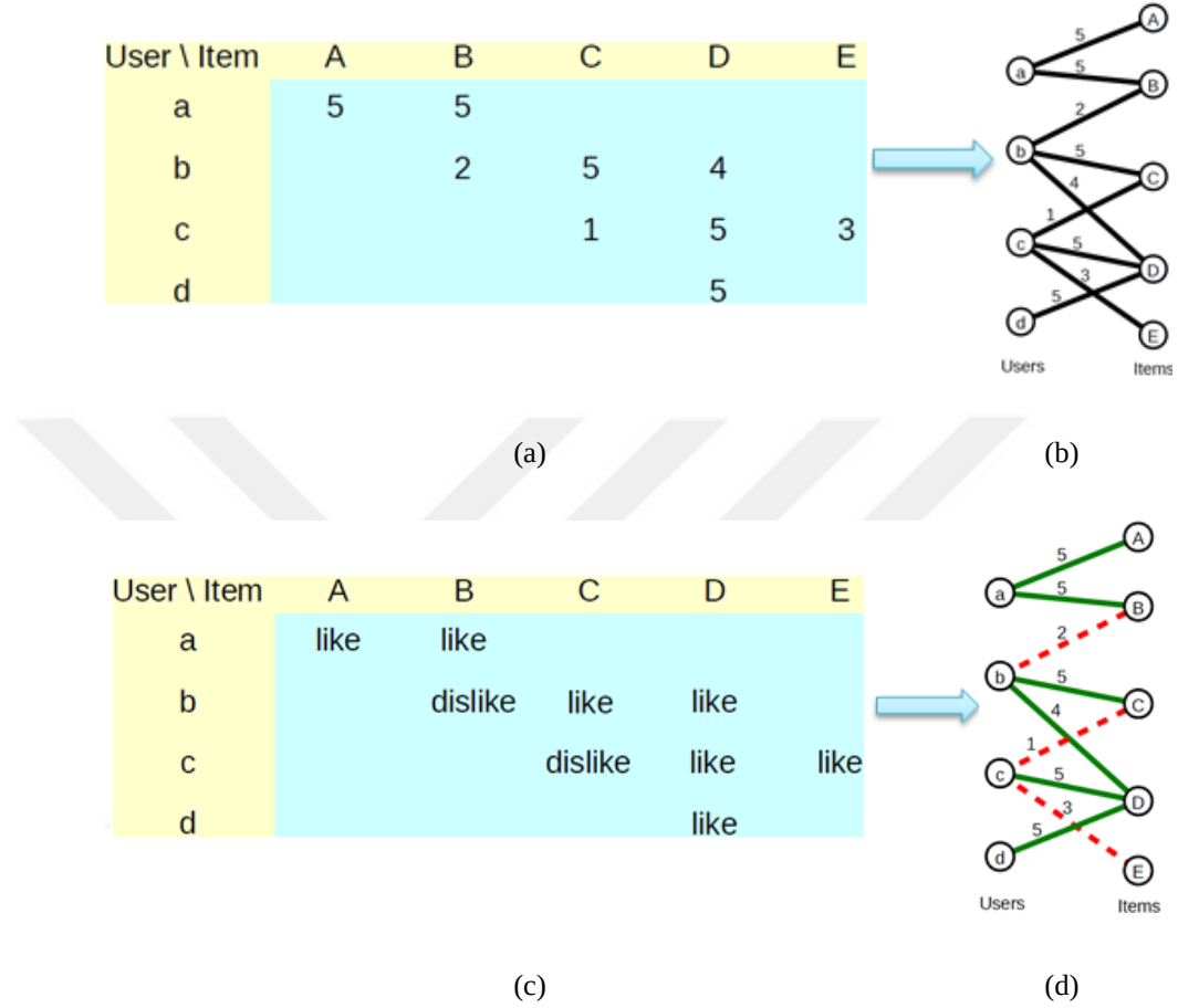
Figure 4.2. (a) User-item rating matrix (b) bipartite graph model (c) User-item relationship matrix, (d) bipartite signed graph (green links are represented as like, red-dash links are represented as dislike)
