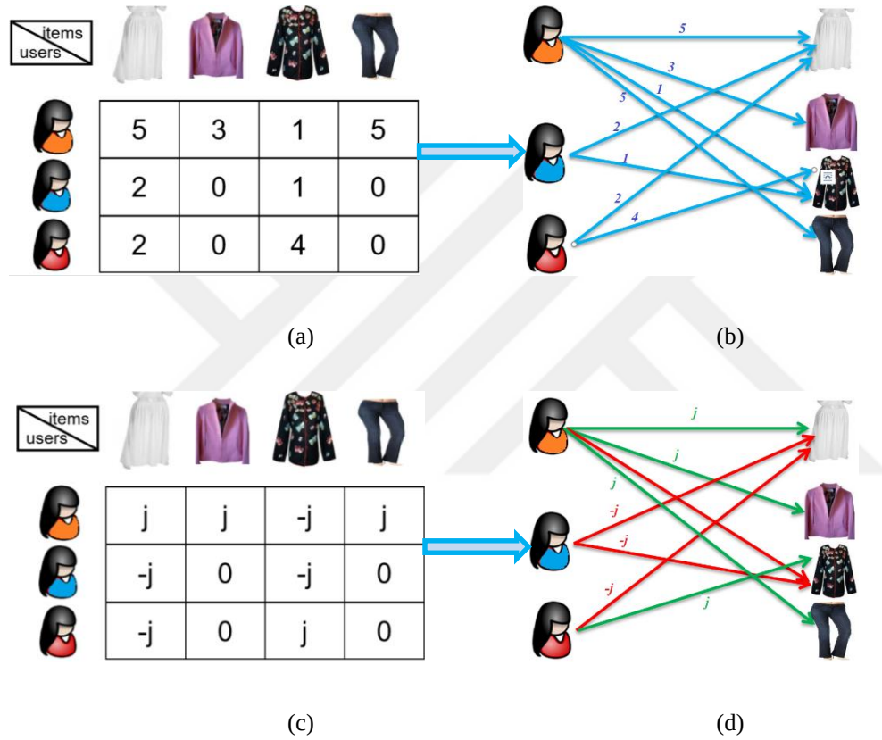
Figure 5.1. (a) User-item rating matrix, (b) bipartite graph model (c) rating conversion of rating matrix A_{UI} , (d) bipartite signed graph.
