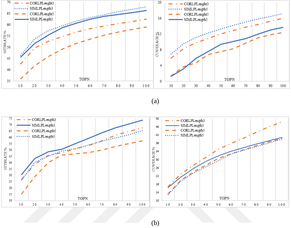
Figure 4.4. The hits rate and coverage comparison of SIMLP and CORLP with path length 3, 5 for topN recommendation on Hetrec (a) and MovieLens (b) datasets.
