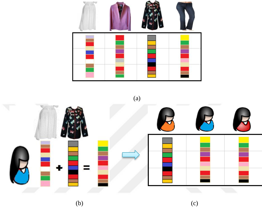
Figure 5.2. (a) Item-feature matrix, (b) the generation of a user feature vector (c) users feature matrix.
