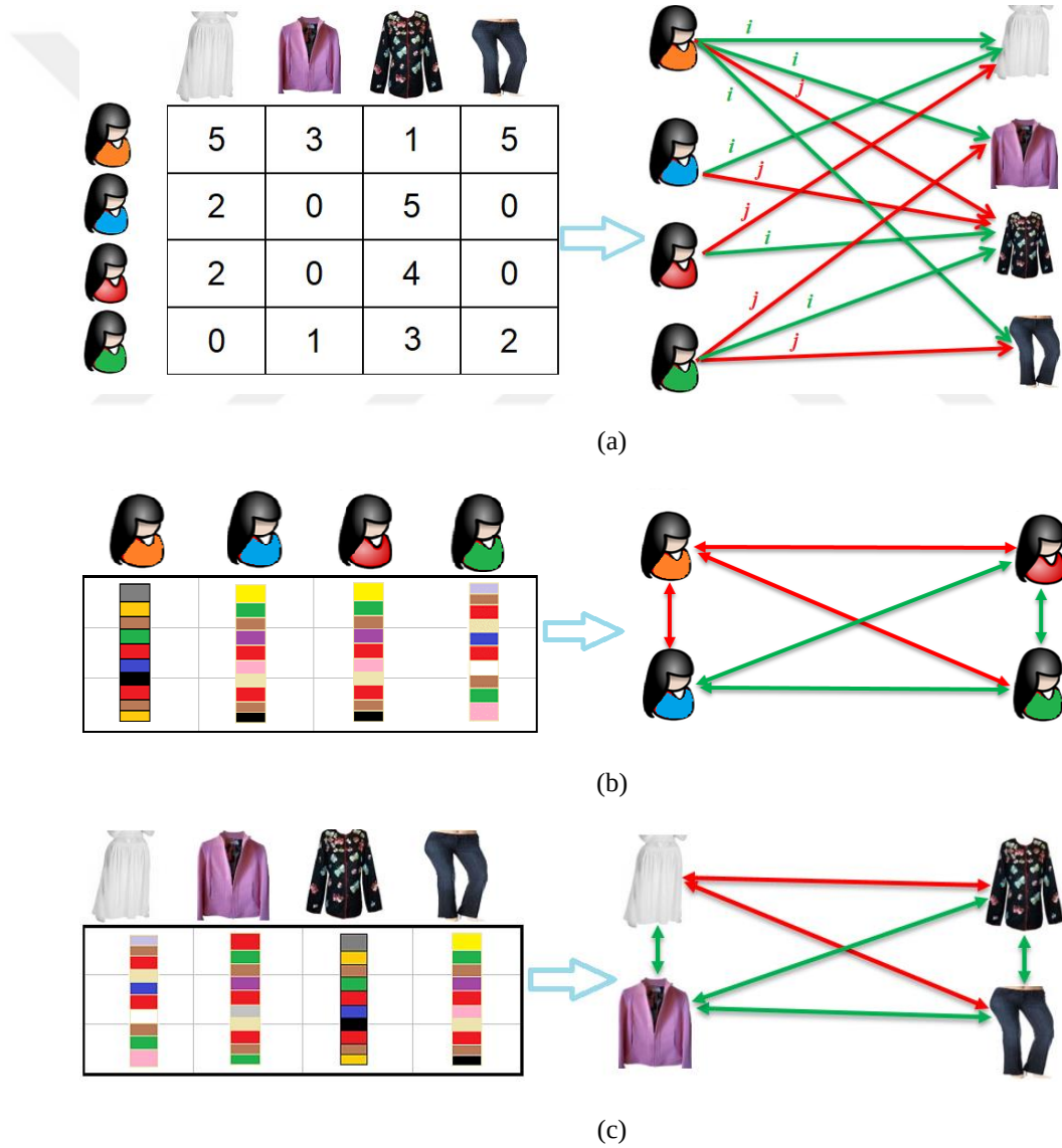
Figure 6.12. (a) User-item rating matrix and bipartite signed graph, (b) user-feature matrix and user-user relationship graph, (c) item-feature matrix and item - item relationship graph
