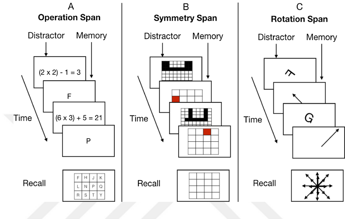
Figure 2. Flowchart of complex span tasks.
