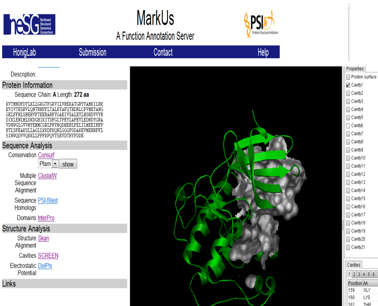
Figure 5.10. MarkUs visualization of Akt2 (PDB 1gzn).
