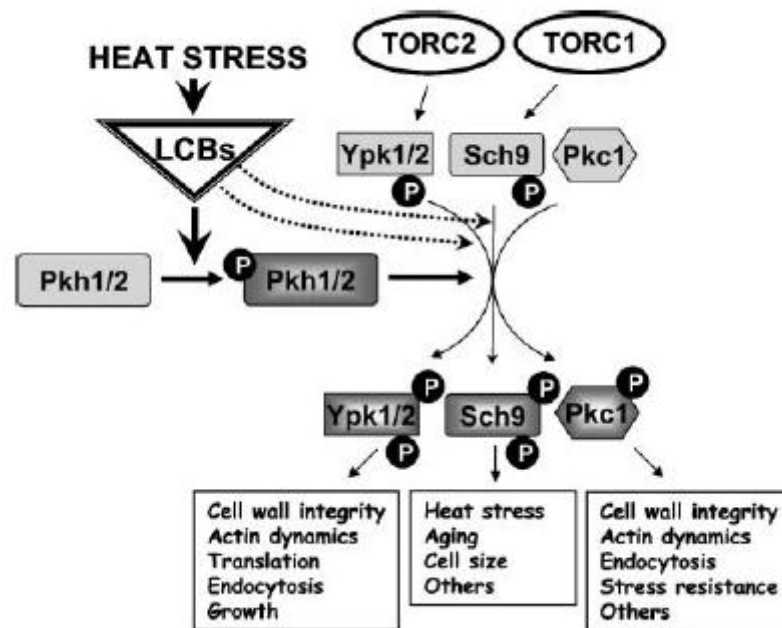
Figure 2.5. The signaling pathways controlled by long chain acid bases in S. cerevisiae (Dickson, 2008).
