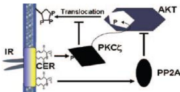
Figure 2.9. Regulation of Akt/PKB by ceramide (Holland and Summers, 2008).
