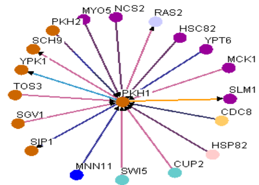
Figure 4.19.b. Genetic interaction of Pkh1p.
