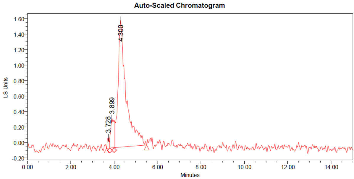
Figure 4.10. Lipid analysis of the deletion mutant of by HPLC (30 g/l initial glucose concentration).
