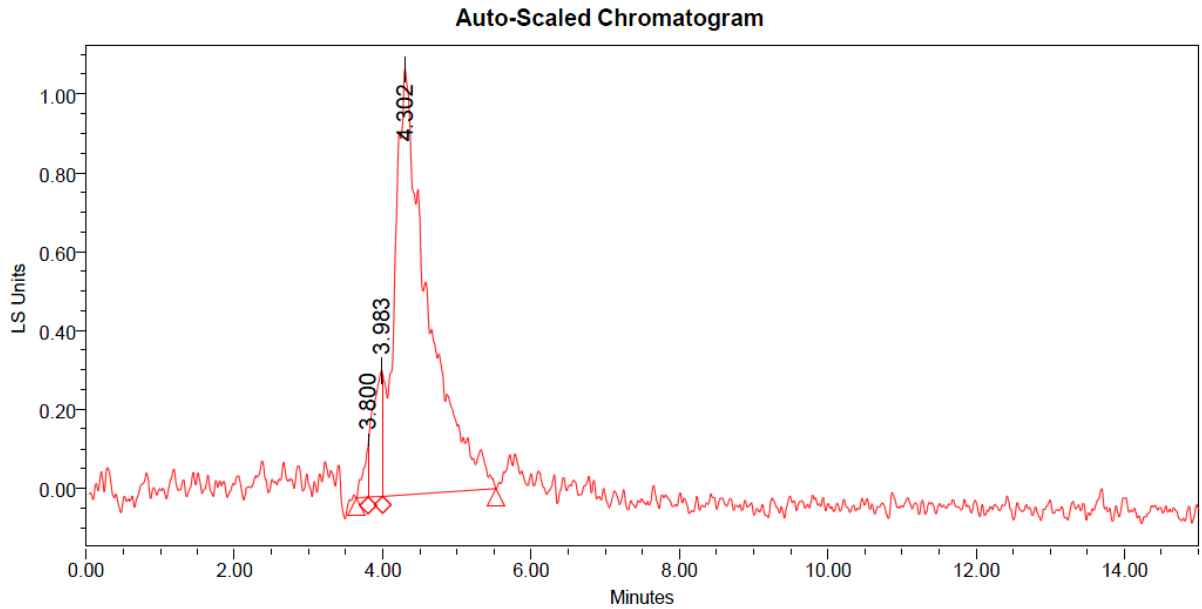
Figure 4.11. Lipid analysis of the deletion mutant of . By HPLC (30 g/l initial glucose concentration).
