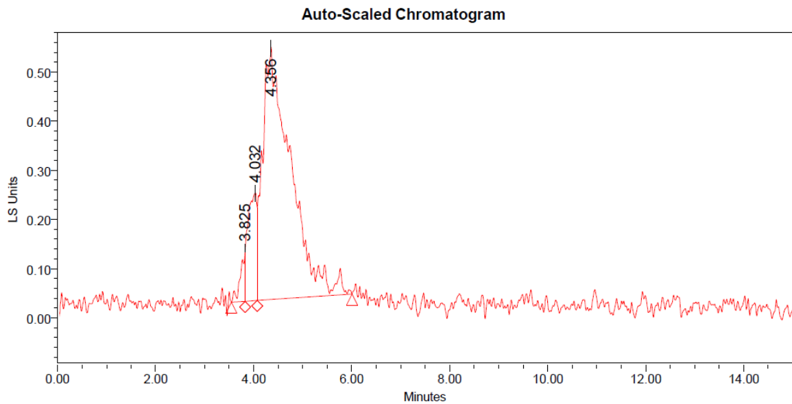
Figure 4.15. Lipid analysis of the deletion mutant of Y. lipolytica by HPLC (40 g/l initial glucose concentration).
