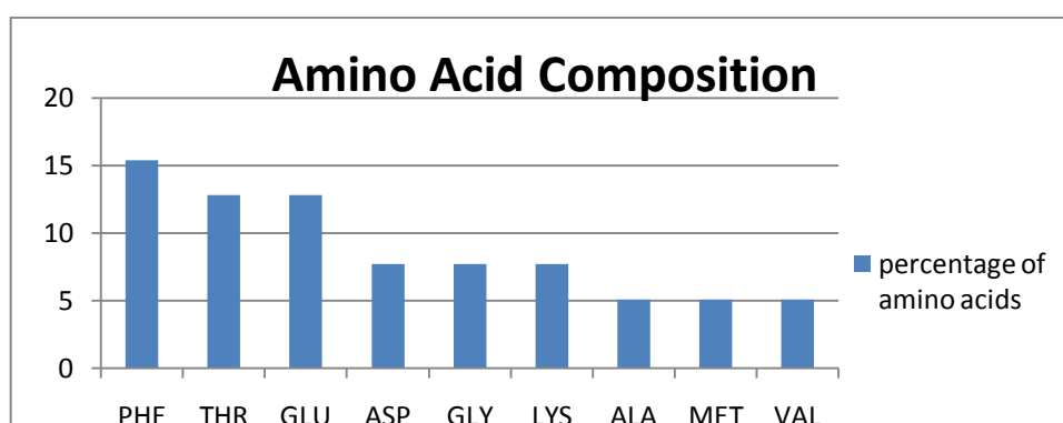
Figure 5.18. Amino acid composition of functional surface of Akt2 protein kinase domain (PDB 2jdr).
