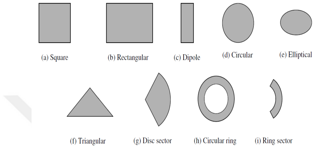
Figure 2.2. Representative shapes of microstrip patch element [10].
