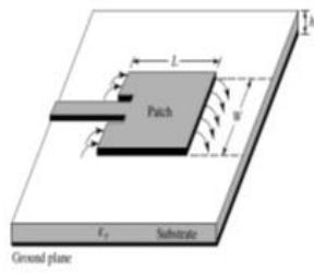
(a) Microstrip line feed
