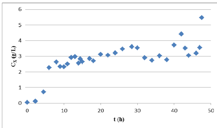
Figure 3.17 Fermentation with Continuous Fresh Medium Feed and Continuous Membrane Filtration. C_X , Biomass Concentration.
