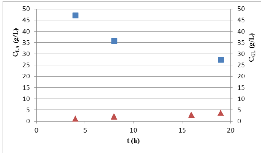
Figure 3.6 Lactic Acid Production (▲) and Glucose Consumption (■) for 5% Glucose, 0.5% Peptone, 0.5% Yeast Extract Medium for the Fermentation without pH Control. C LA , Lactic Acid Formation; C GL , Glucose Level.
