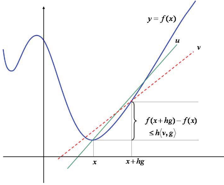
Figure 2.1: Quasiseccants for a one variable function
