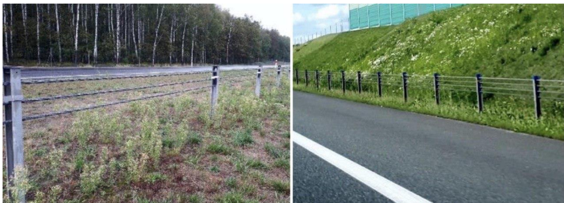
Figure 3.10. Cable barrier applications [90].
