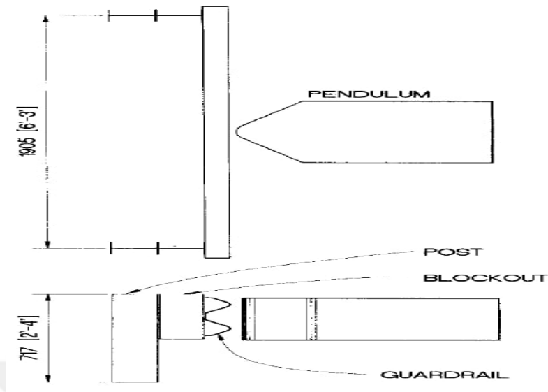
Figure 5.6. Configuration of 820 kg pendulum used in 1998 [126].
