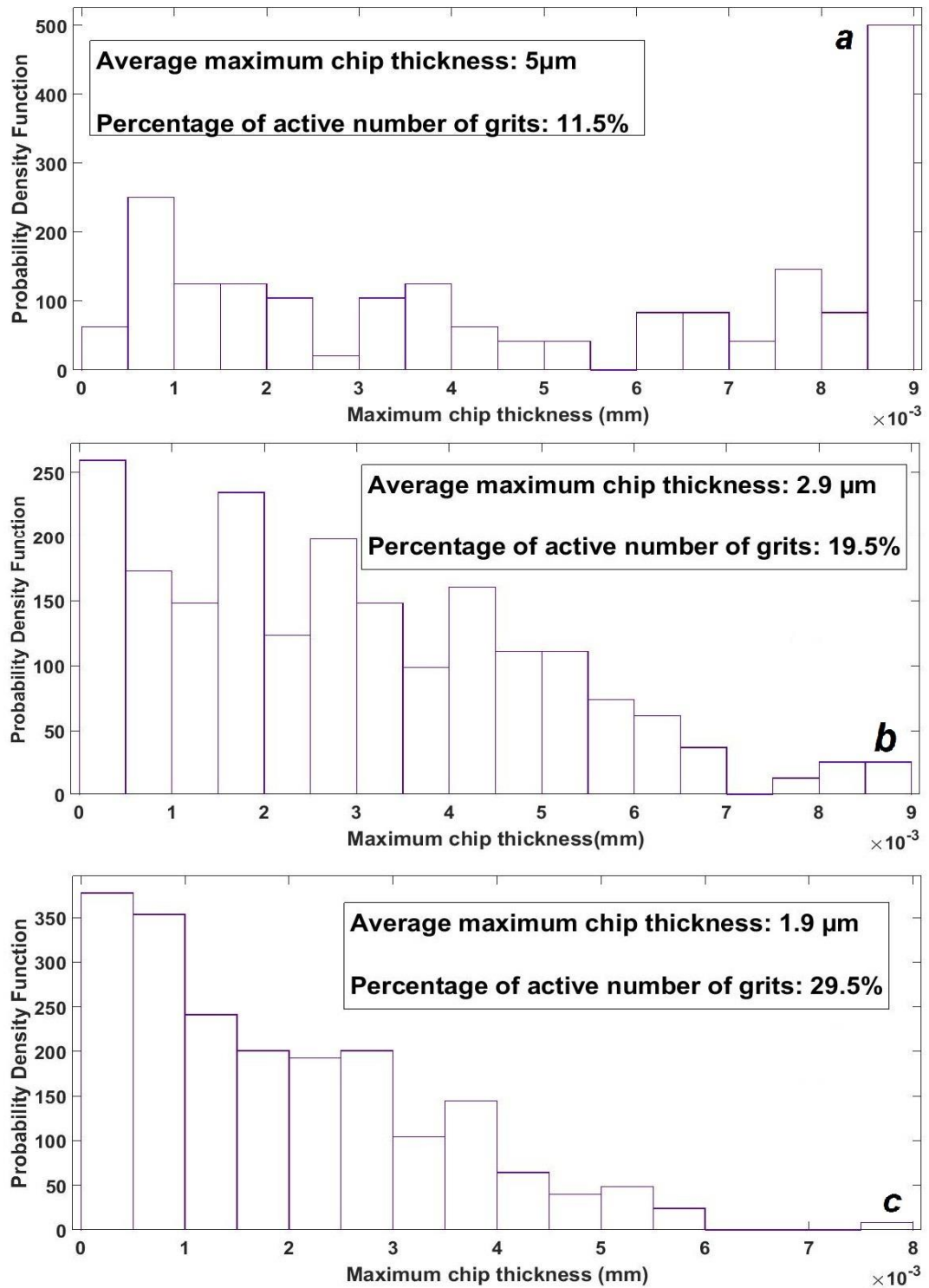
Figure 7-13 Probability density function of maximum chip thickness, depth of cut 0.08mm, feed rate 0.05 mm/rev for wheel 1 (a), wheel 4 (b) and wheel 5 (c)
