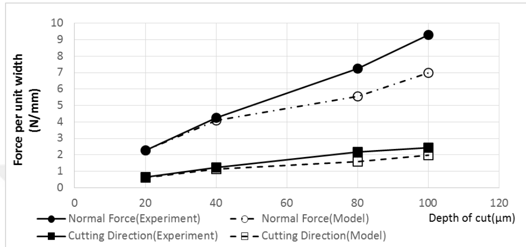
Figure 7-20 Grinding force per unit width in the cutting and normal direction for wheel 3 at different depth of cuts, feed 0.1 mm/rev, run out 10 μm
