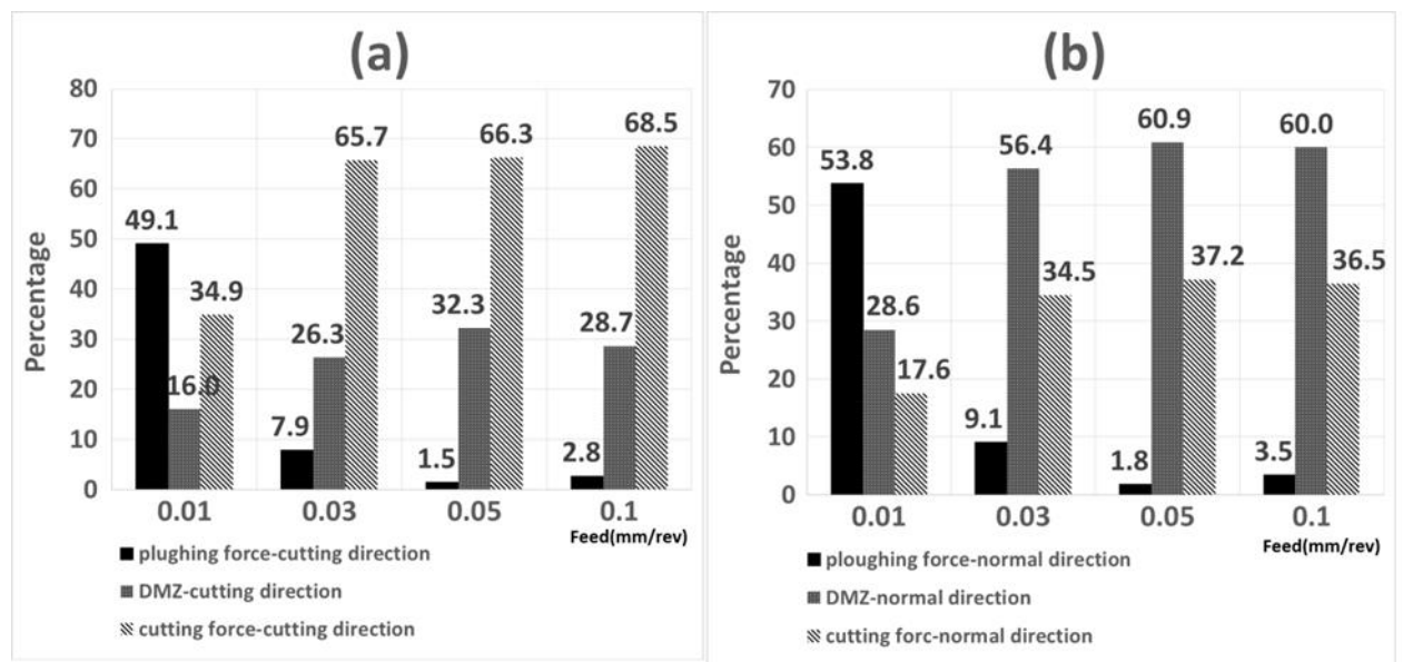
Figure 7-16 Contribution of force parts in the cutting direction (a) and normal direction (b) for wheel 1 at different feed rate, depth of cut 0.08 \mu\text{m} , run out 10 \mu\text{m}
