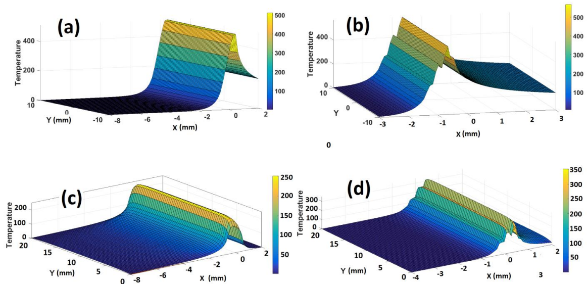
Figure 4-7 3D temperature profile of the workpiece in different cases: a) constant heat source in dry condition (adiabatic boundary conditions at walls) b) periodic heat source in dry condition c) constant heat source in wet condition (convective boundary condition at walls) d) periodic heat source in wet condition
