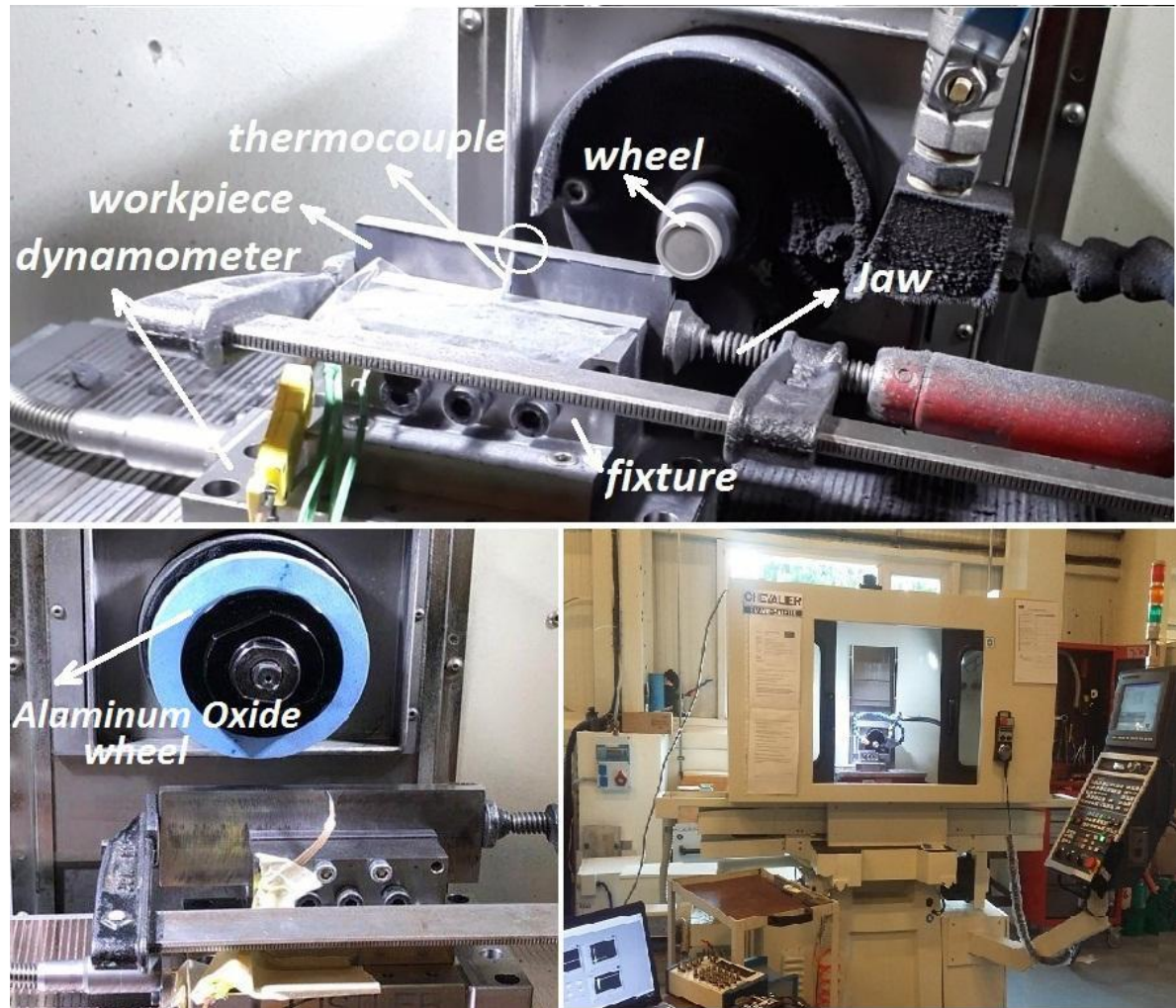
Figure 6-11 Experimental setup and devices for temperature model verification
