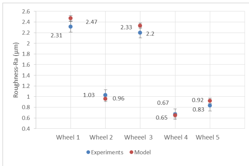
Figure 7-8 Surface roughness value ( R_a ) perpendicular to the cutting direction for wheel 1 to 5 at different feed rates (0.01 to 0.1 mm/rev) and depth of cuts (0.02 to 0.1 mm)
