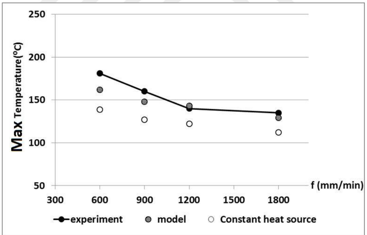
Figure 7-27 Maximum temperature in dry condition at different feed rates using aluminum oxide wheel where the depth of cut was 6 μm and the cutting speed was 10.4 m/sec.
