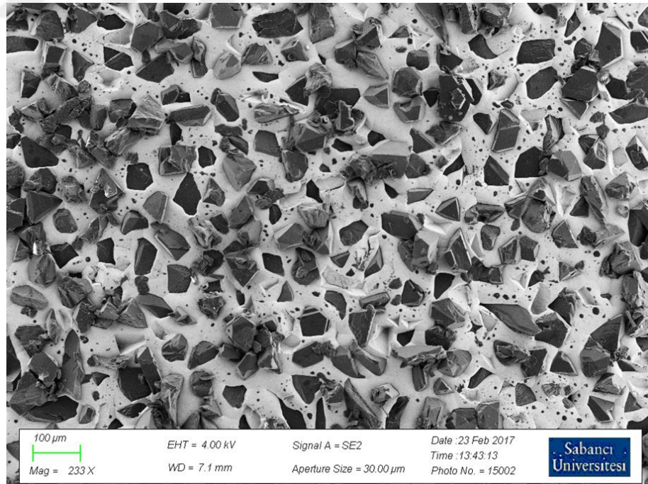
Figure 2-1 SEM photo of an electroplated CBN grinding wheel
