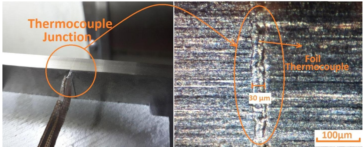
Figure 6-12 Thermocouple junction
