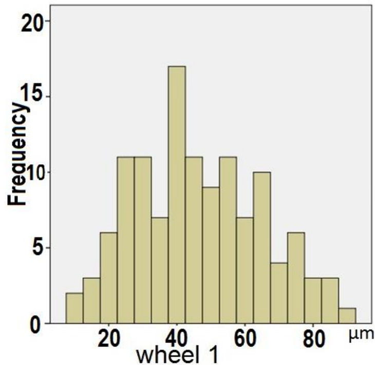
Figure 7-1 height distribution of the grit for wheel 1
