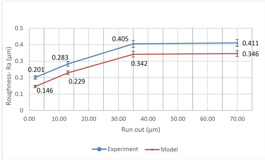
Figure 7-12 Surface roughness values parallel to the cutting direction for wheel 2 at different run out, feed rate 0.14mm/rev, depth of cut 0.08 mm
