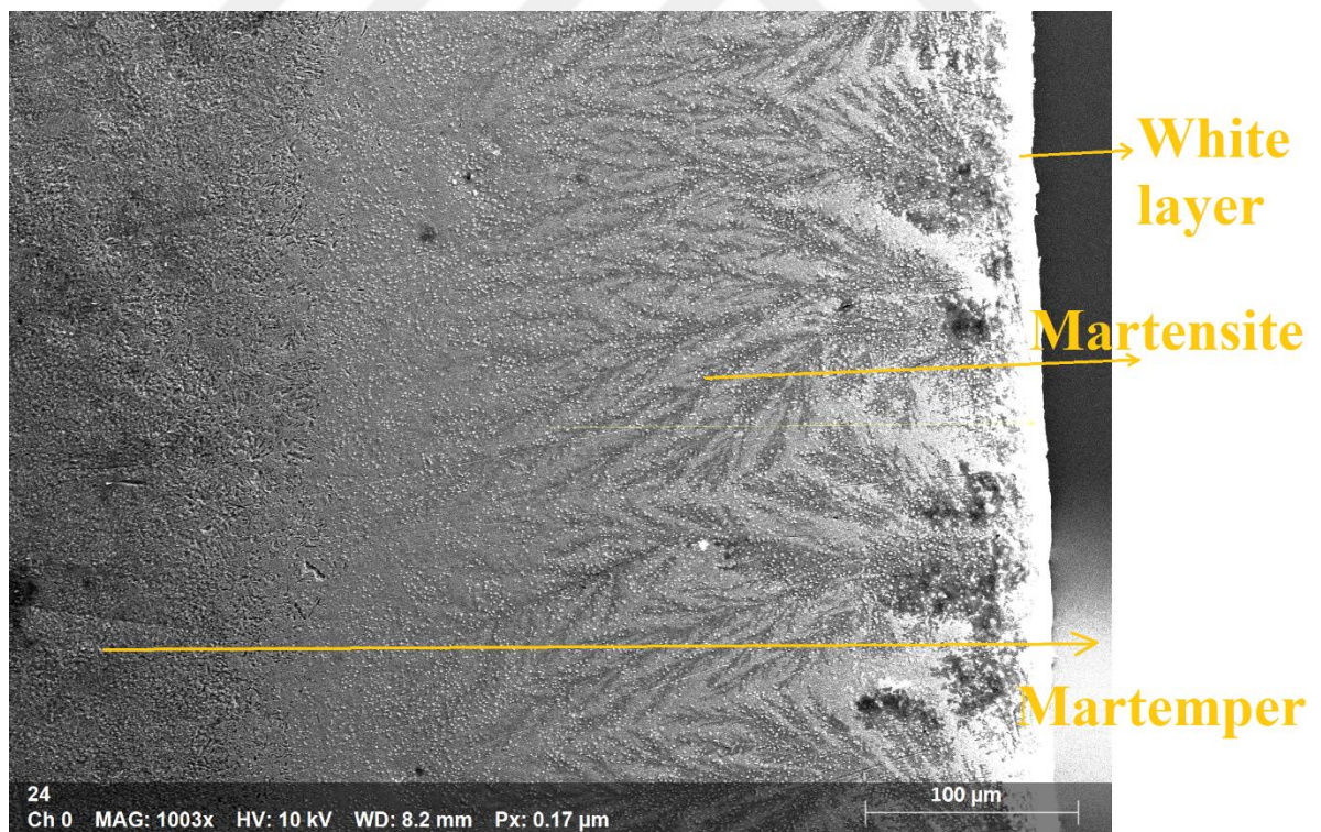
Figure 7-35 Cross section of a sample after grinding in absence of oxygen
