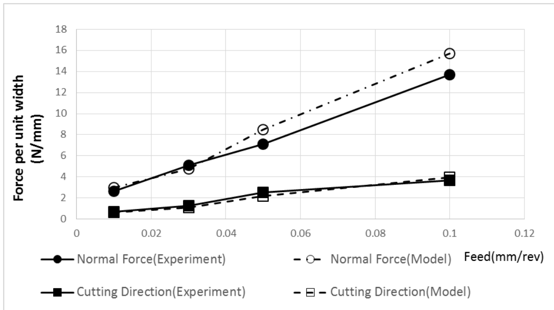
Figure 7-15 Grinding force per unit width in the cutting and normal direction for wheel 1, depth of cut 80 \mu\text{m} , run out 10 \mu\text{m}
