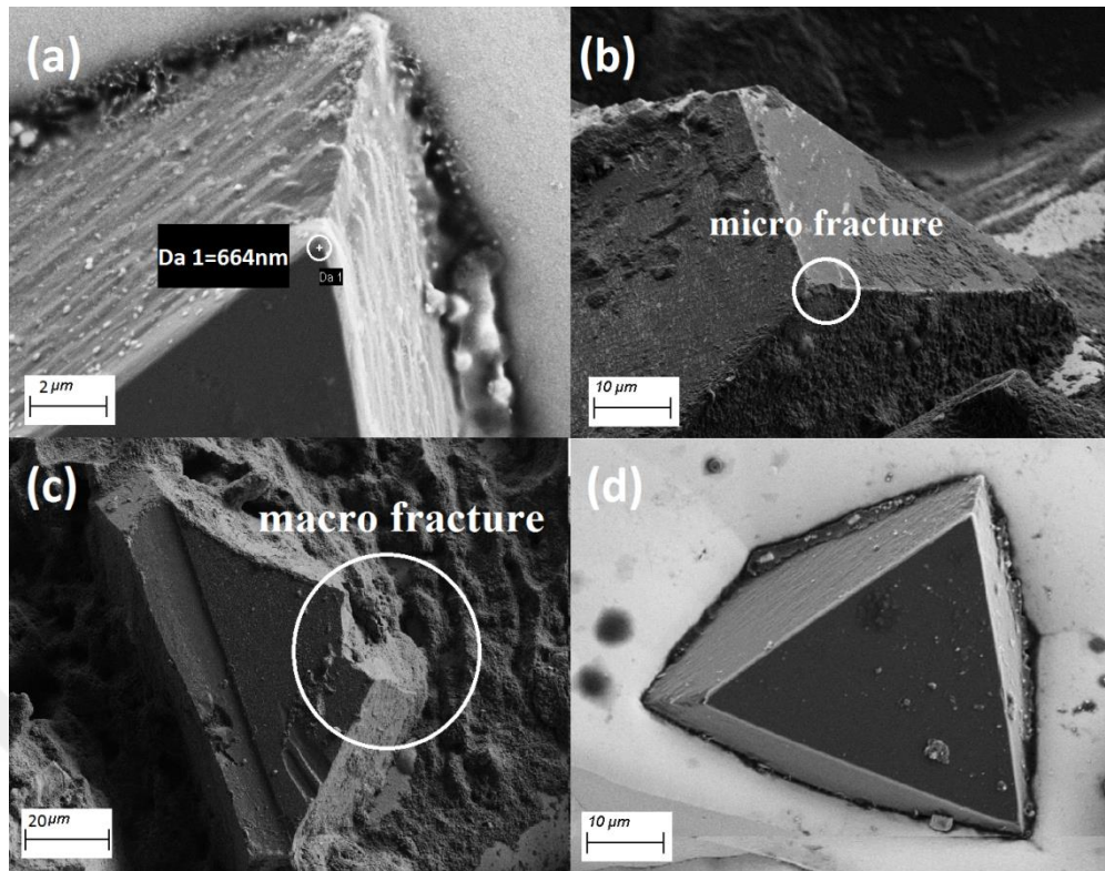
Figure 6-5 SEM photos of single CBN grits, a) a sharp grit with edge radii of 0.6\ \mu\text{m} , b) fracture wear at the tip, c) fracture wear changing the clearance angle, d) grit with a flat surface
