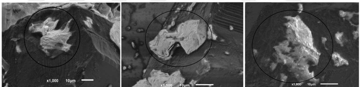
Figure 6-6 SEM photos of CBN grits with sticking material on the rake face
