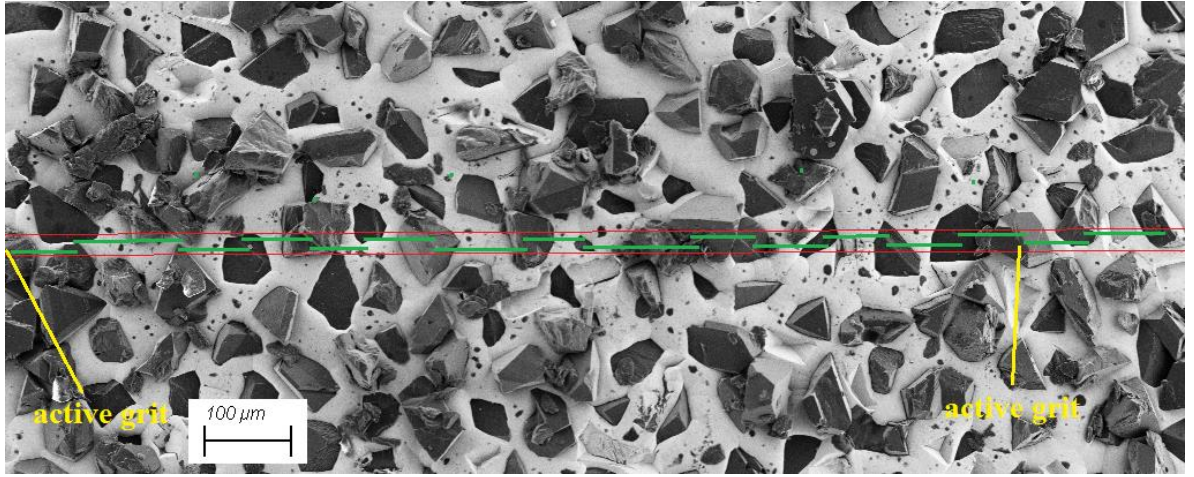
Figure 2-3 sample wheel discretization on a single layer CBN wheel
