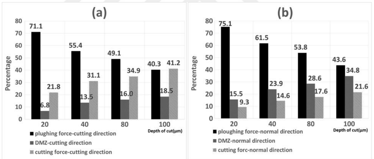
Figure 7-19 Contribution of force parts in the cutting direction (a) and normal direction (b) for wheel 1 at different depth of cuts, feed 0.01 mm/rev, run out 10 μm
