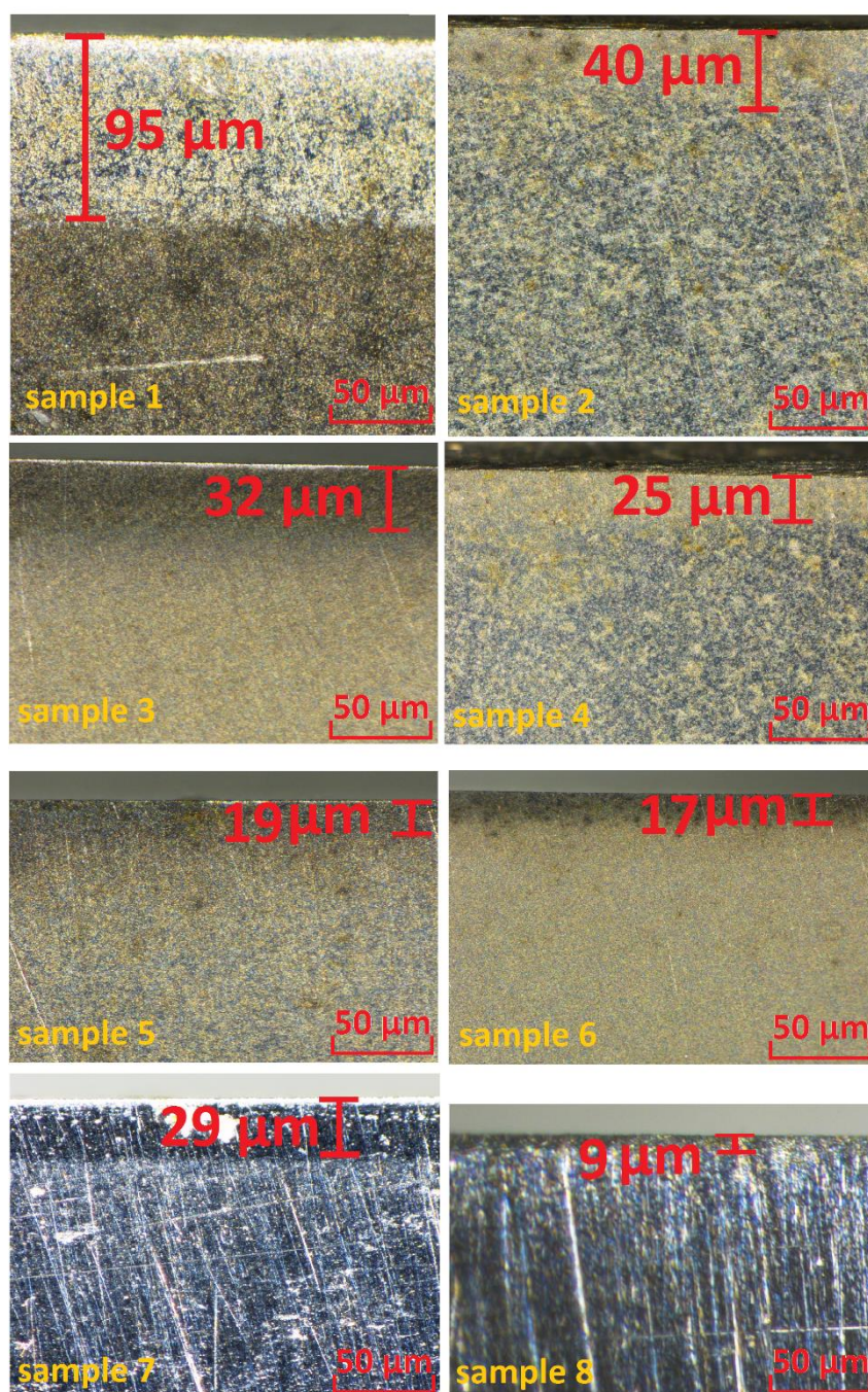
Figure 7-29 Cross-sections of the workpiece samples.
