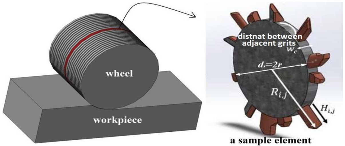
Figure 2-2 Discretization of grinding wheel along the radial direction
