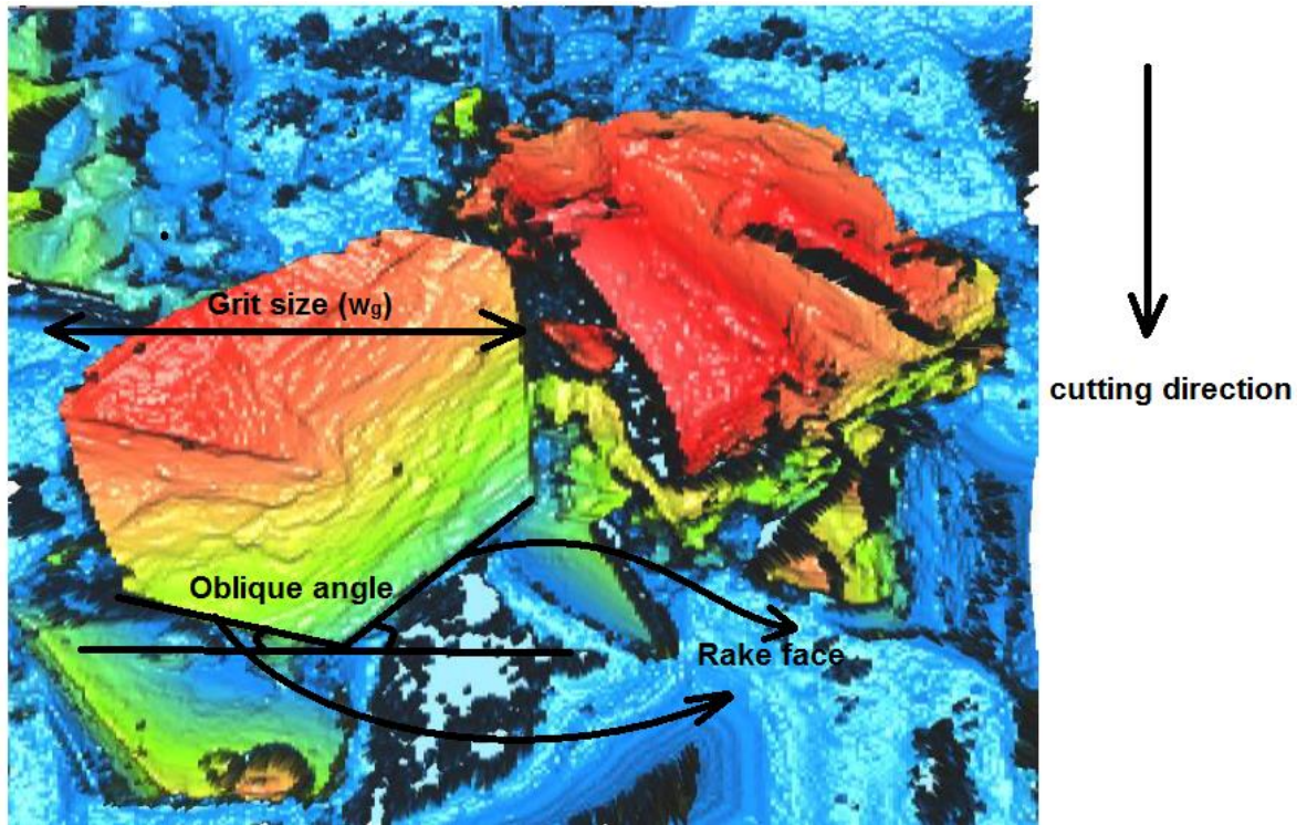
Figure 6-7 2D view of the grit (top view) grit size and oblique angles can be identified easily from this view
