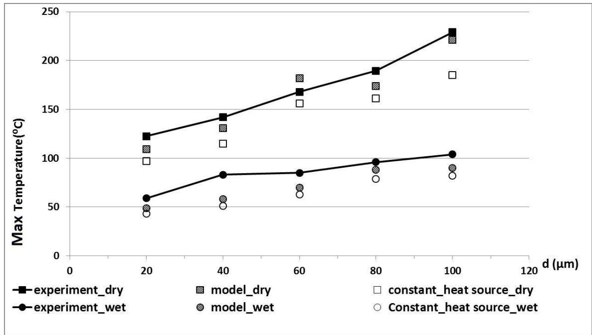
Figure 7-24 Maximum temperature in dry condition using CBN wheel at different depth of cuts, feed rate 600mm/min, cutting speed 29 m/sec
