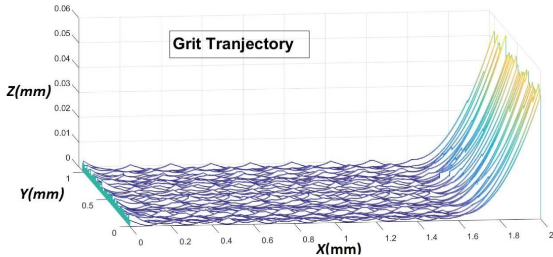
Figure 2-9 Grit trajectory) at feed 0.25 mm/rev, depth of cut 0.08 mm
