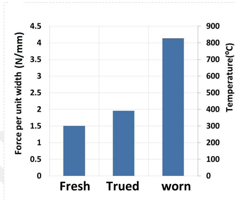
Figure 4-13 Tangential Grinding force per unit width and Temperature for Inconel 718 workpiece material using a CBN electroplated wheel in fresh, trued and worn conditions, depth of cut 20\text{ }\mu\text{m} , feed rate 2800\text{ mm/min} , cutting speed 15\text{ m/sec} , run out 10\text{ }\mu\text{m}
