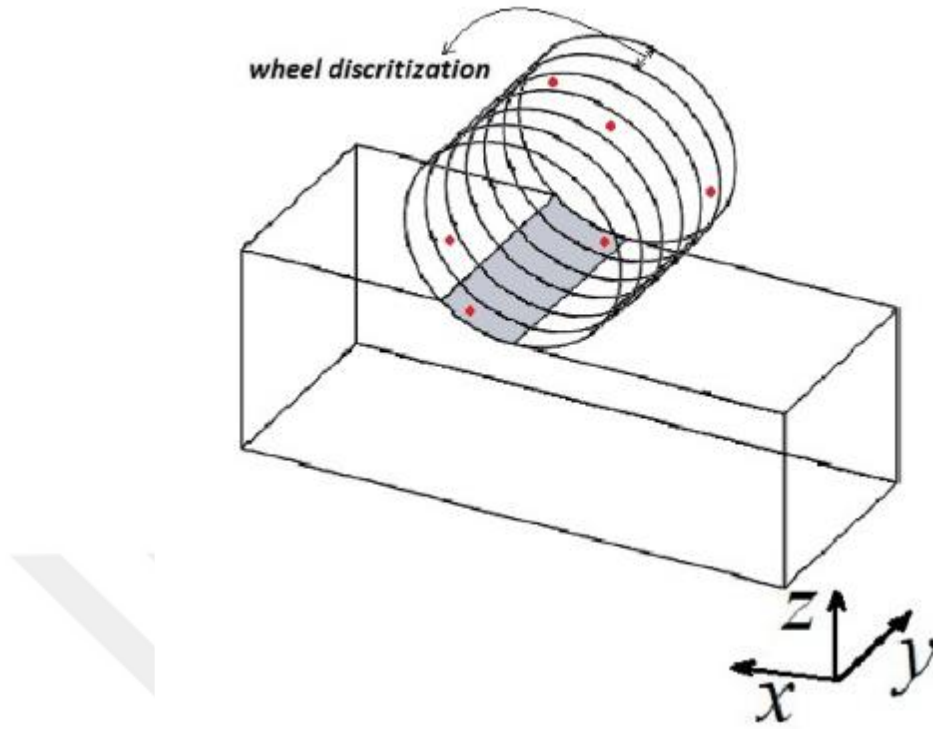
Figure 4-6 wheel discretization and position of the active grits
