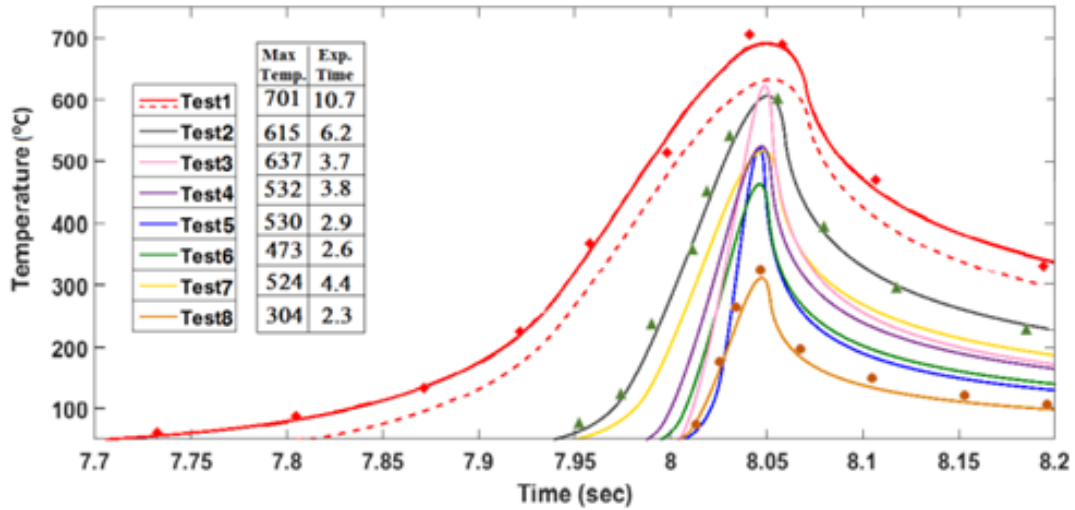
Figure 7-30 Temperature profiles of the samples.
