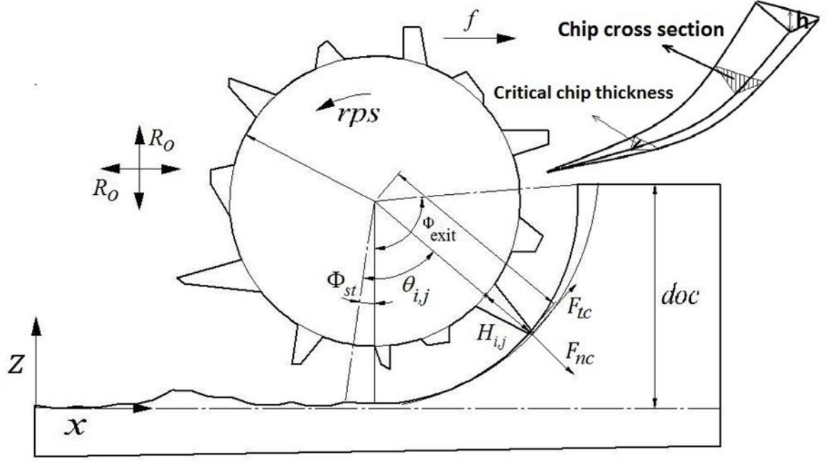
Figure 3-2 cutting force for a single grit
