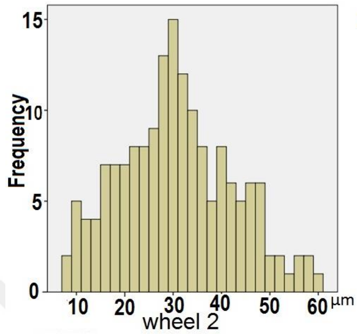
Figure 7-2 height distribution of the grit for wheel 2
