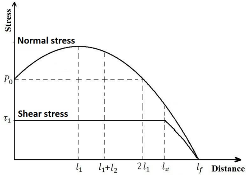
Figure 3-4 Normal and shear stress profiles on the flank face
