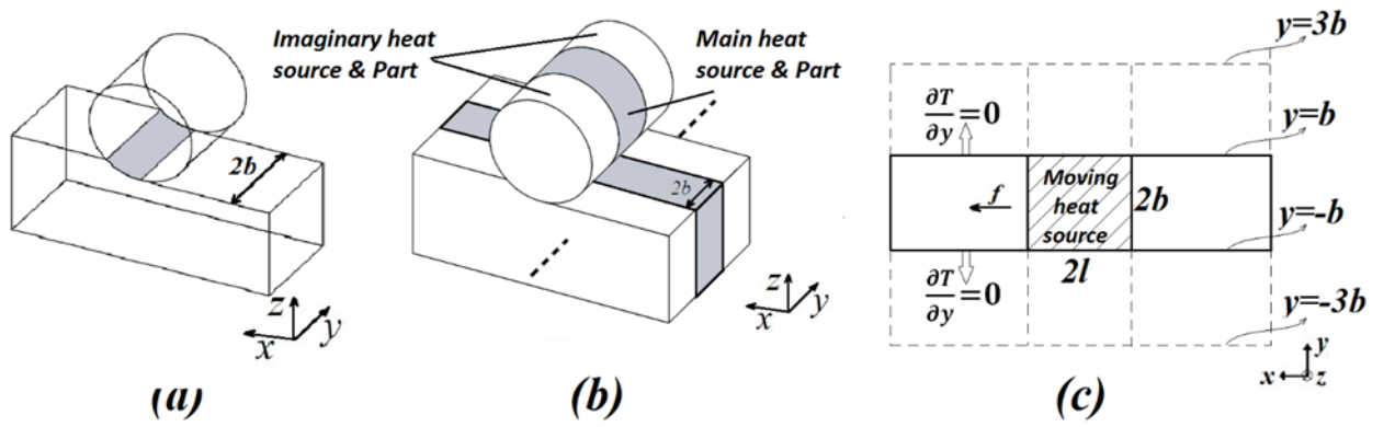
Figure 4-2 a) Rectangular heat source on a body with a finite width b) main and imaginary heat source and workpiece c) 2D view of the workpiece
