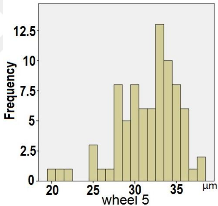
Figure 7-5 height distribution of the grit for wheel 5
