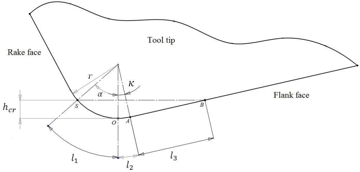
Figure 3-3 grit tip considering edge radius in the third deformation zone
