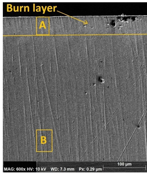
Figure 7-31 SEM photo of sample 2
