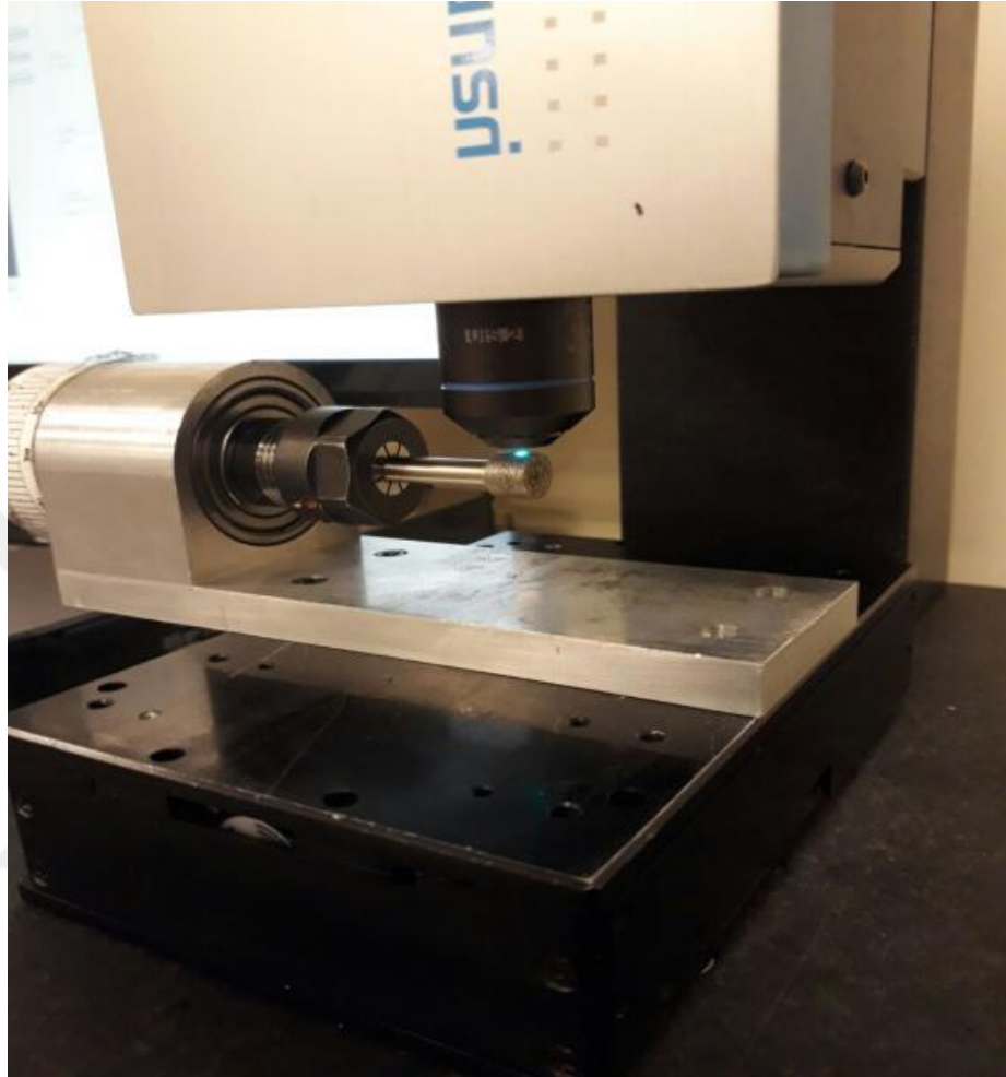
Figure 6-1 μsurf NanoFocus microscope and apparatus enable 360 ° access to the wheel
