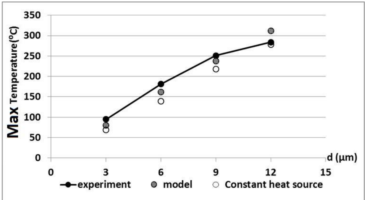
Figure 7-26 Maximum temperature in dry condition using aluminum oxide wheel at different depths of cut, and feed rate of 600mm/min and forcutting speed 10.4 m/sec
