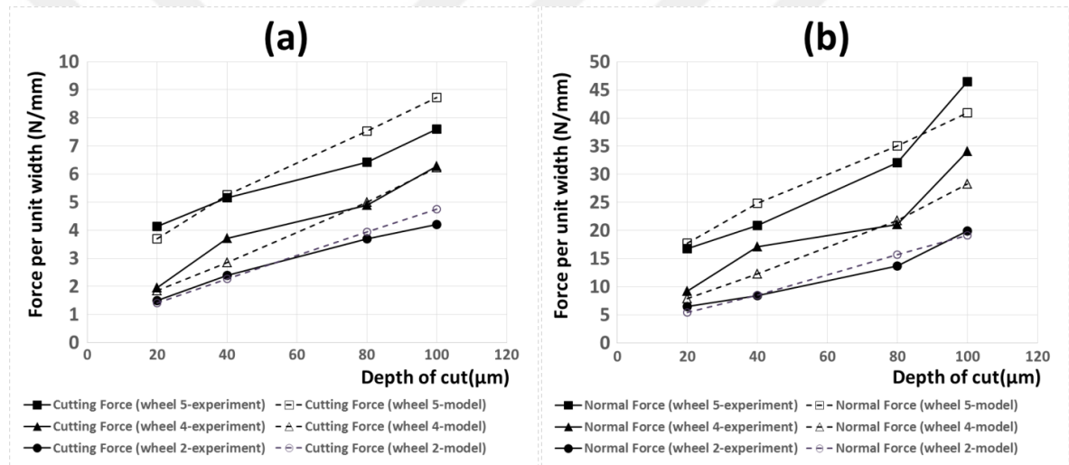
Figure 7-21 Grinding force per unit width in the cutting direction (a) and normal direction (b) for wheel 2 (fresh), 4 (trued) and 5 (worn) at different depth of cuts, feed 0.1 mm/rev, run out 10 μm
