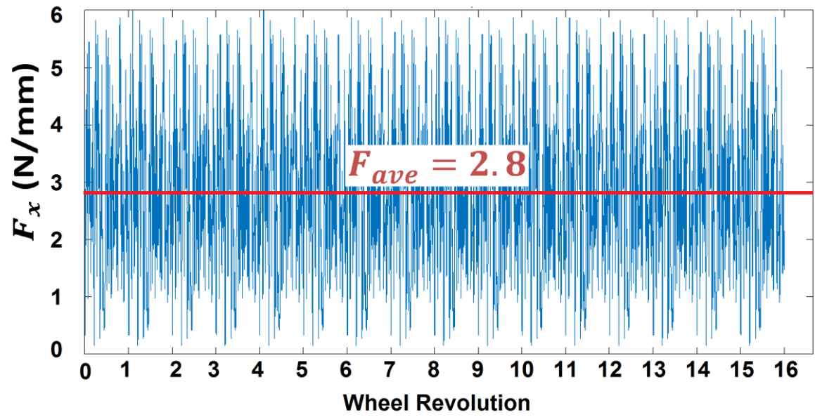
Figure 4-5 Horizontal grinding force per unit width for a dressed aluminum wheel, wheel diameter 40mm, wheel rpm 6000, feed 1000 mm/min, depth of cut 0.06 mm, workpiece material: bearing steel, grit height standard deviation 8 \mu\text{m} , grit width of cut standard deviation 4 \mu\text{m}
