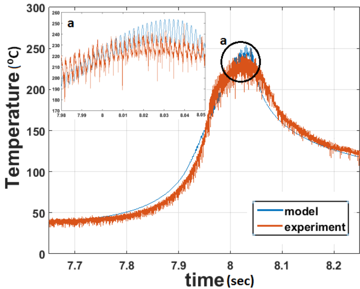
Figure 7-23 Temperature signal collected using CBN wheel, under dry condition with depth of cut of 100\ \mu\text{m} , feed rate of 600\text{mm/min} and cutting speed of 29\text{ m/sec}
