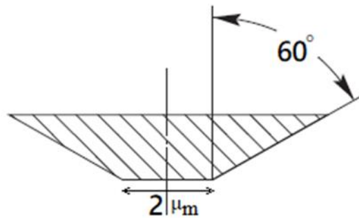
Figure 2-7 Cross-section of the grit with average parametric values
