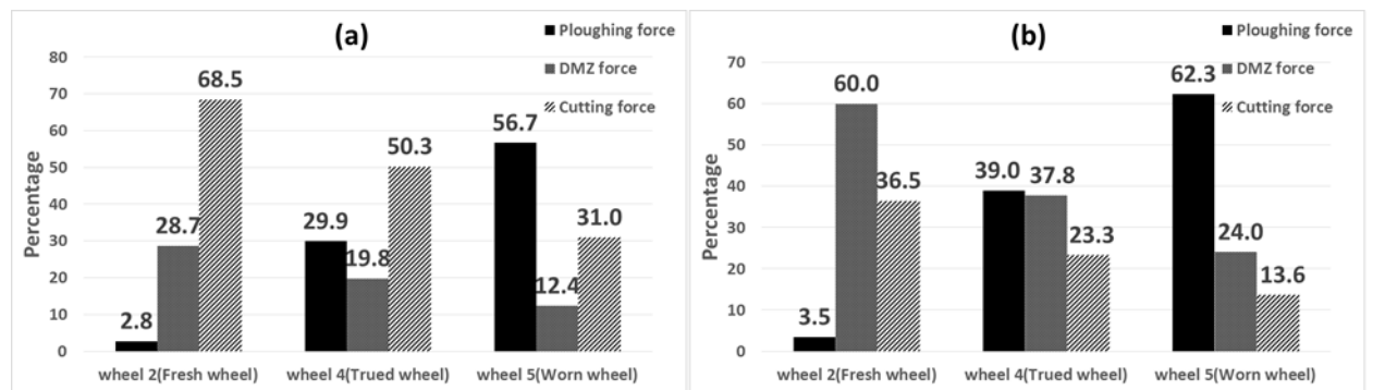
Figure 7-22 Contribution of force parts in the cutting direction (a) and normal direction (b) for the fresh, trued and worn wheels, depth of cut 0.08 μm, feed 0.1 mm/rev run out 10 μm
