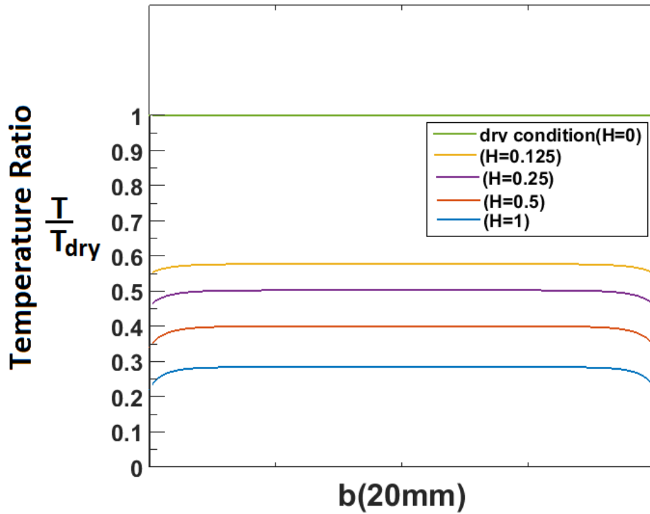
Figure 4-12 Effect of cooling convection factor on temperature of the bearing steel workpiece slab, L=0.98 ,
