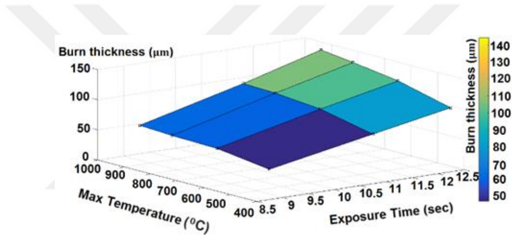
Figure 5-2 Burn thickness vs. exposure time and maximum temperature for AISI 52100 workpiece material and aluminum oxide wheel.
