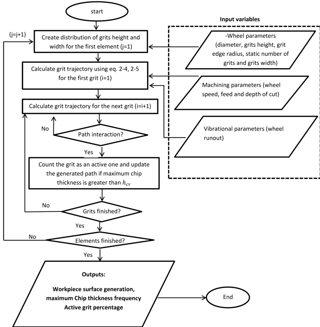
Figure 2-8 Algorithm of simulation code for workpiece surface generation
