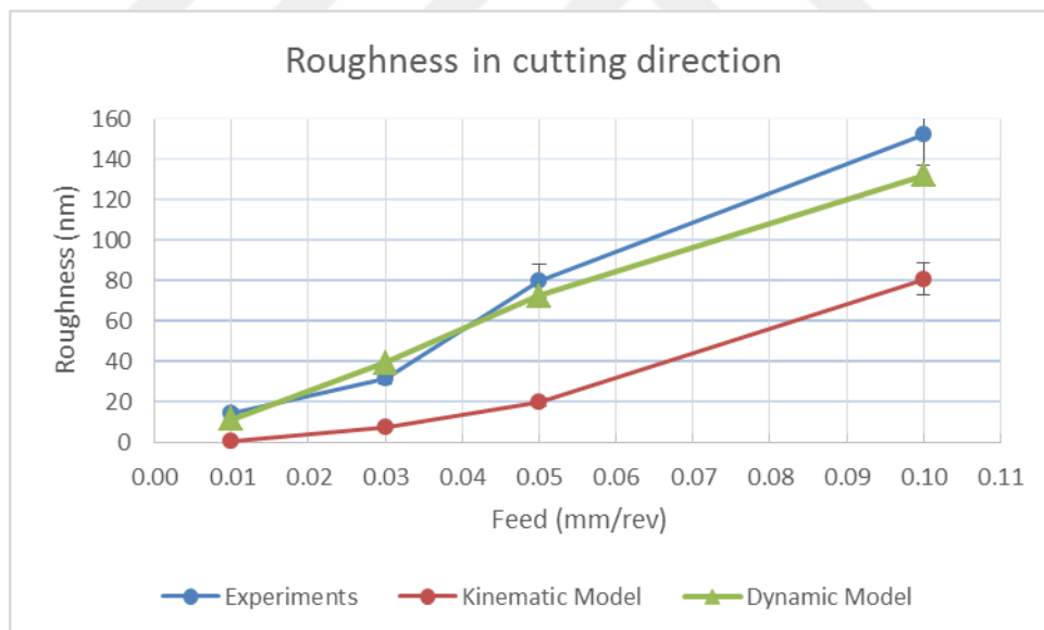
Figure 7-10 Surface roughness values parallel to the cutting direction for wheel 4 at different feed rates, 10 micron wheel run out, 40 micron depth of cut
