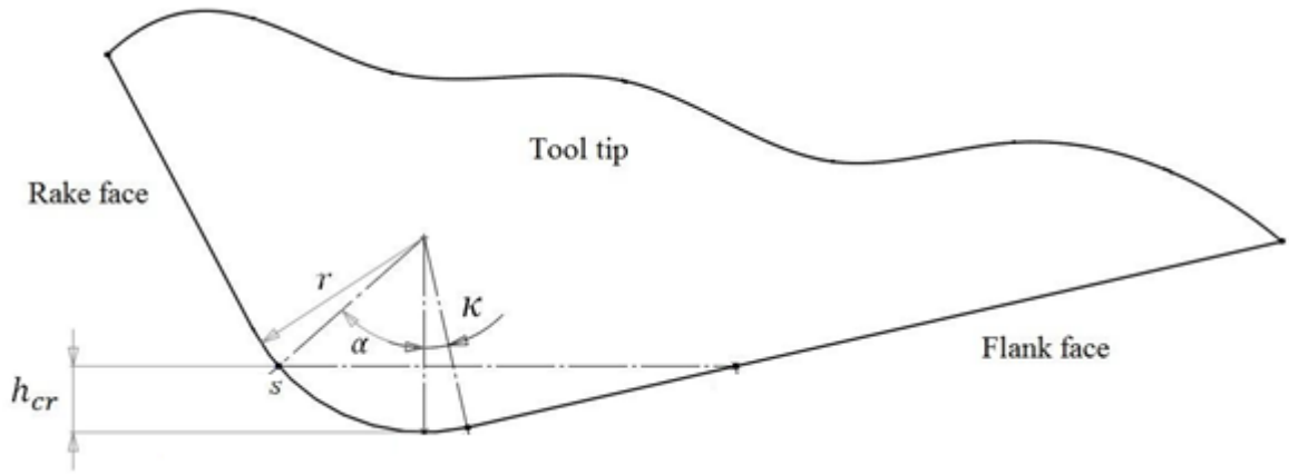
Figure 2-6 Tool tip considering edge radius in the third deformation zone
