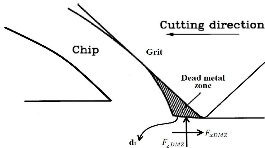
Figure 3-6 formation of the dead metal zone
