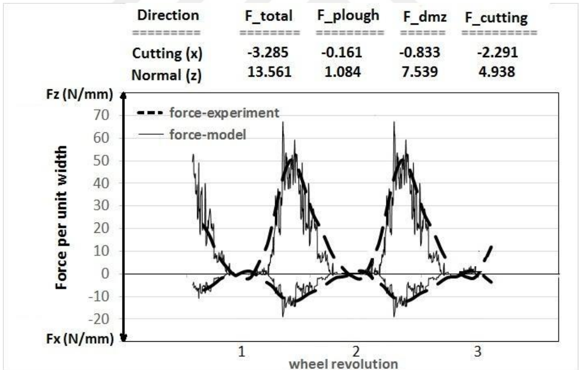
Figure 7-14 Grinding force per unit width in the cutting and normal direction for wheel 1, depth of cut 80\text{ }\mu\text{m} , feed 0.1\text{ mm/rev} , run out 10\text{ }\mu\text{m}
