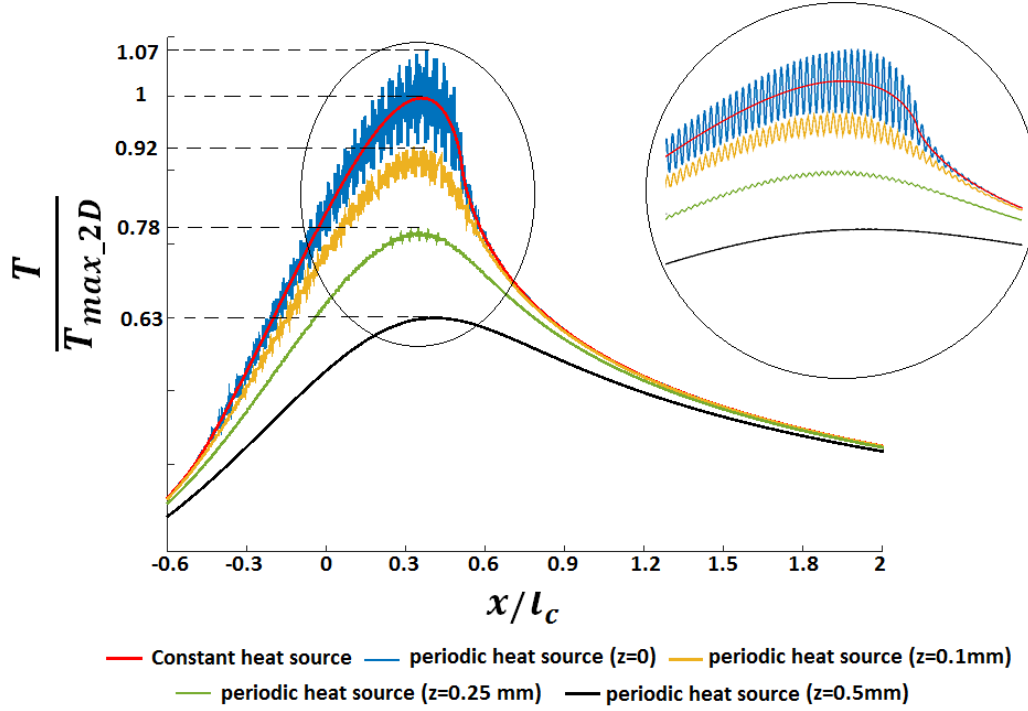
Figure 4-9 temperature profiles of the slab in feed direction along the middle of slab considering different heat sources for a bearing hardened steel workpiece material at different z levels
