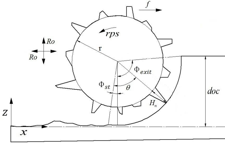
Figure 2-4 Schematic of wheel-workpiece interaction in surface grinding
