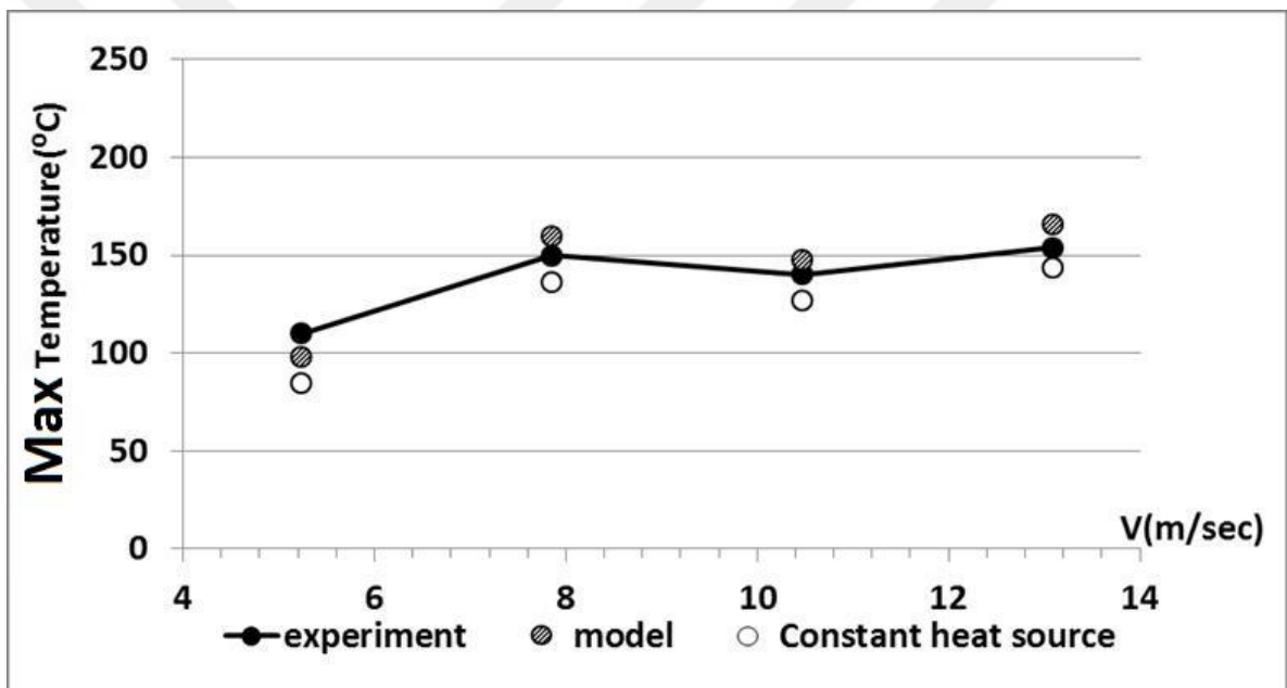
Figure 7-28 Maximum temperature in dry condition at different cutting speed using aluminum oxide wheel, depth of cut 6 \mu\text{m} , feed rate 1200 mm/min
