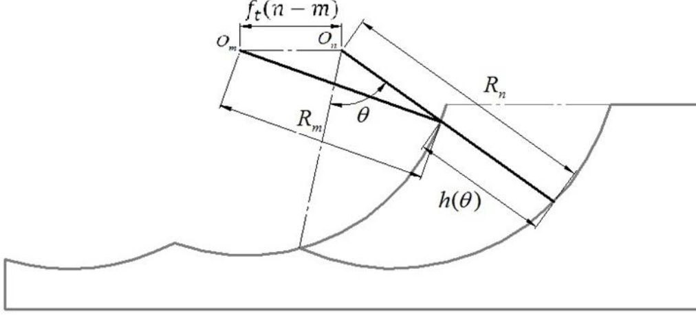
Figure 2-5 Instantaneous chip thickness in grinding
