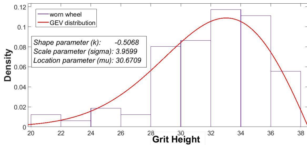
Figure 7-7 Probability density function of grit height for the worn wheel (wheel 5)
