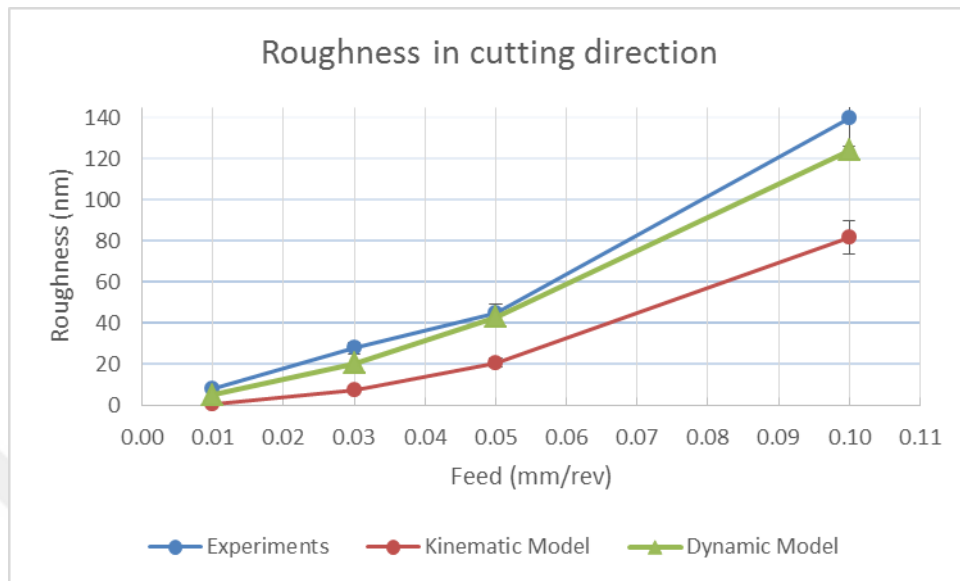
Figure 7-9 Surface roughness values parallel to the cutting direction for wheel 1 at different feed rates, 10 micron wheel run out, 40 micron depth of cut
