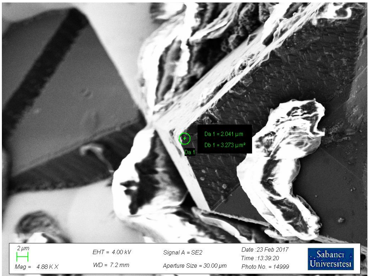
Figure 6-4 SEM photo of a grit showing the edge radius
