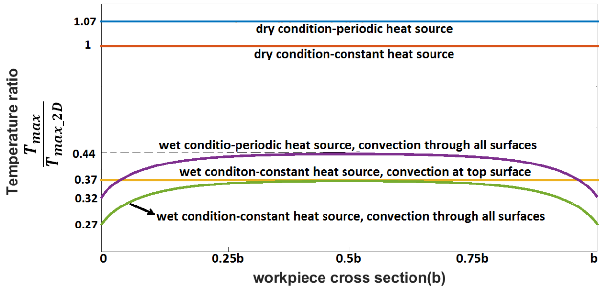
Figure 4-8 maximum temperature of the workpiece along the cross section of the workpiece considering different boundary conditions and different heat source for a bearing hardened steel workpiece material, coolant convective factor h=0.07 \text{ W/mm}^2\text{K} , b=10\text{mm} , L=0.23
