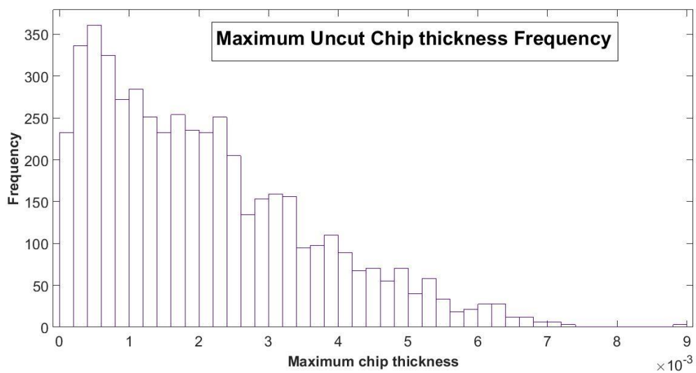
Figure 2-10 chip thickness frequency at feed 0.25 mm/rev, depth of cut 0.08 mm
