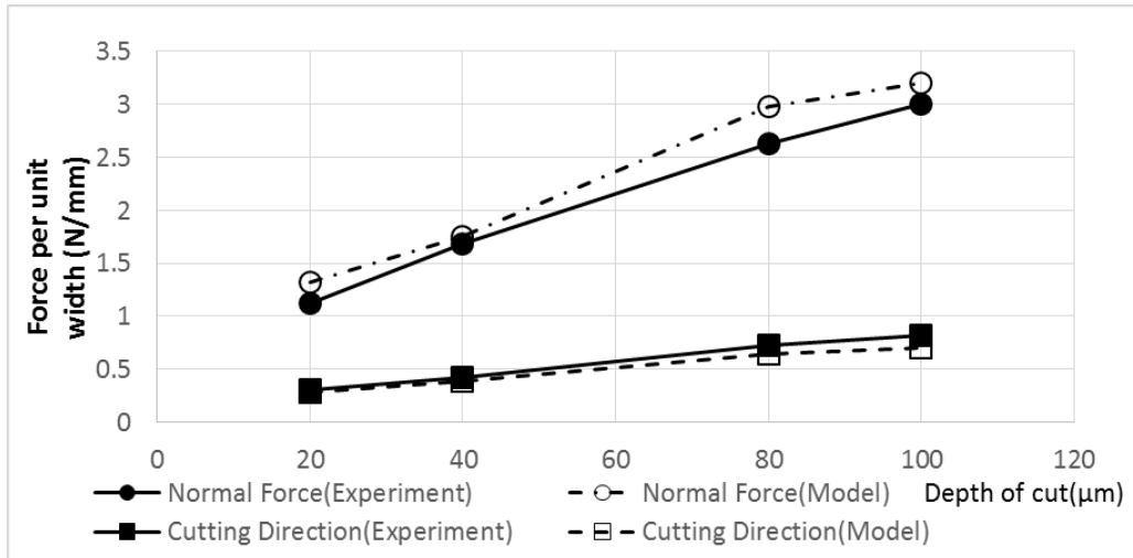
Figure 7-18 Grinding force per unit width in the cutting and normal direction for wheel 2 at different depth of cuts, feed 0.01 mm/rev, run out 10 μm
