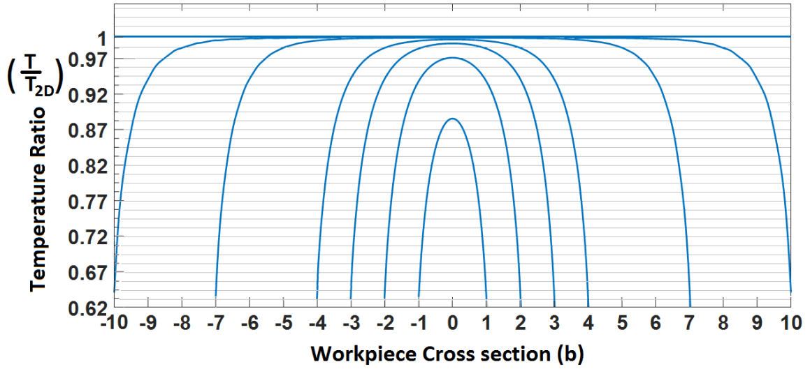
Figure 4-11 Temperature distribution along the cross section of the workpiece considering different workpiece width considering bearing hardened steel workpiece material, coolant convective factor h=0.07 \text{ W/mm}^2\text{K} , L=0.97
