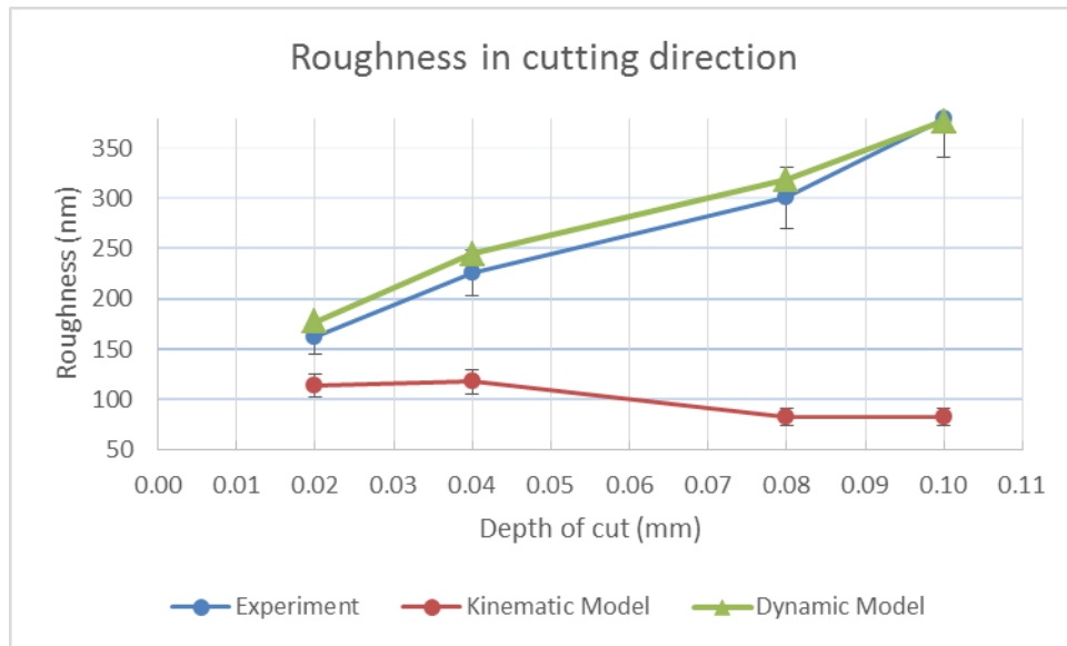
Figure 7-11 Surface roughness values parallel to the cutting direction for wheel 5 at different depth of cut, 10 micron wheel run out, 0.1 mm/rev feed rate
