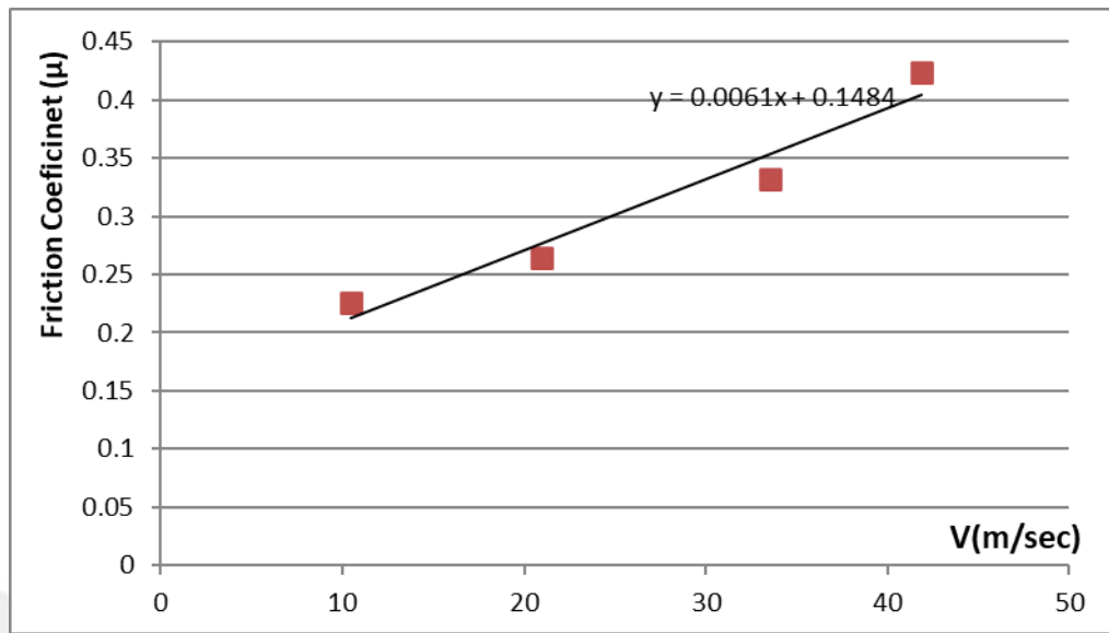
Figure 6-10 Relation between sliding coefficient of friction and cutting speed
