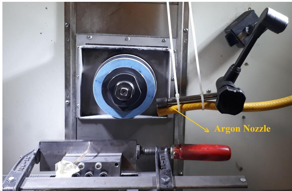
Figure 7-34 Setup of experiment to perform grinding test in absence of oxygen
