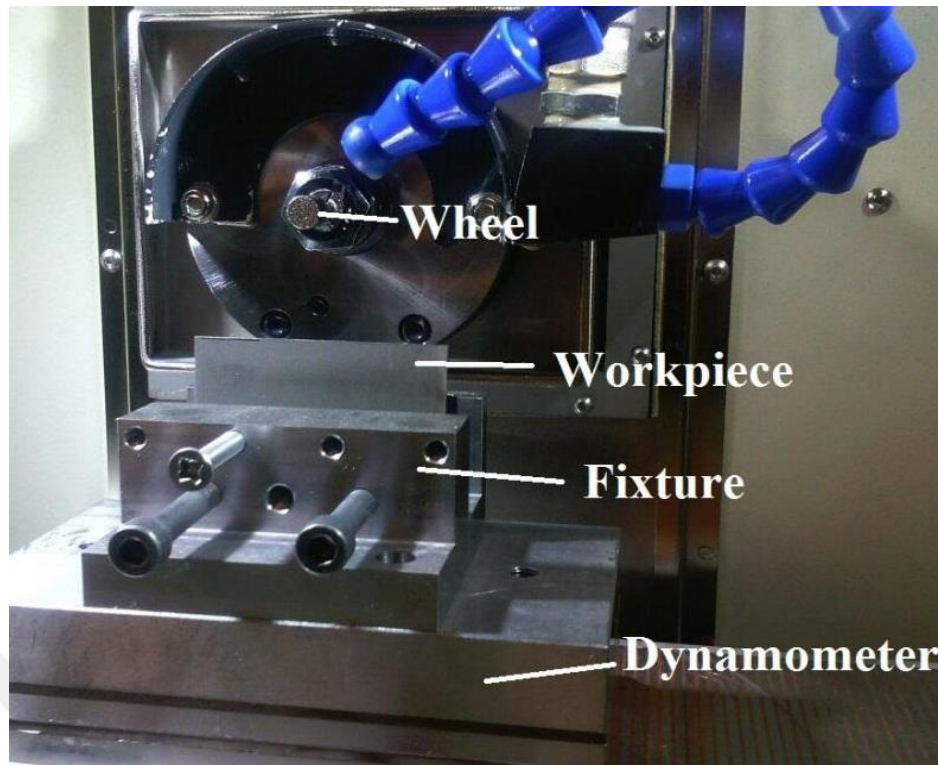
Figure 6-9 Experimental setup for force model verification
