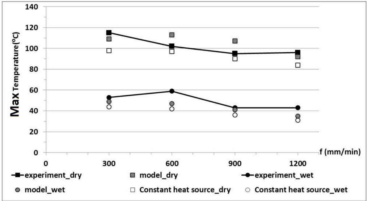
Figure 7-25 Maximum temperature in dry and wet conditions at different feed rates, depth of cut 20 \mu\text{m} , cutting speed 29 m/sec
