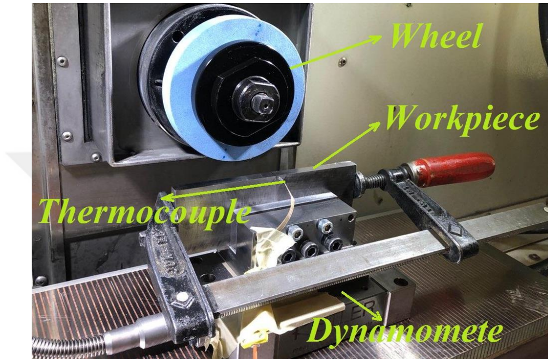
Figure 6-13 setup of the experiment for burn tests
