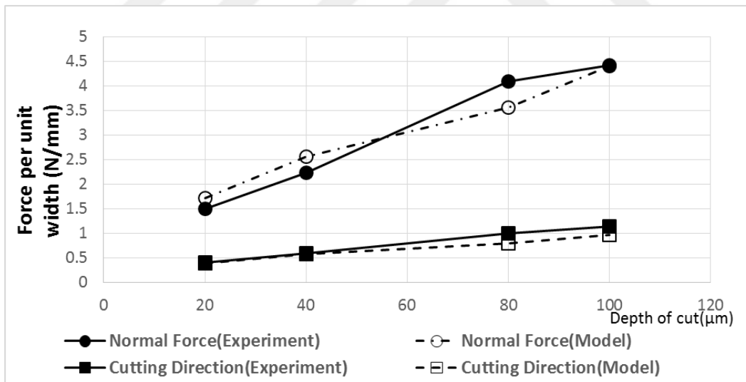
Figure 7-17 Grinding force per unit width in the cutting and normal direction for wheel 1 at different depth of cuts, feed 0.01 mm/rev, run out 10 μm
