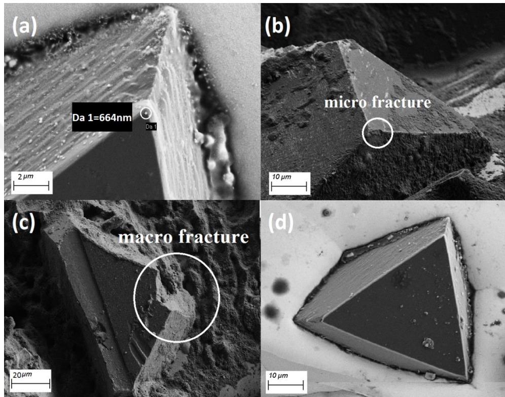
Figure 3-5 SEM photos of single CBN grits, a) a sharp grit with edge radii of 0.6 \mu\text{m} , b) fracture wear at the tip, c) fracture wear changing the clearance angle, d) grit with a flat surface
