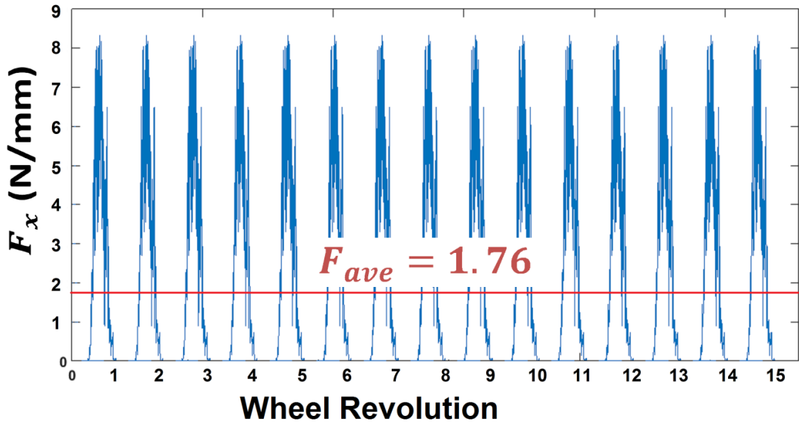
Figure 4-4 Horizontal grinding force per unit width for a CBN single layer wheel, run out 5\ \mu\text{m} , wheel diameter 20mm, wheel rpm 12000, feed 2000 mm/min, depth of cut 0.04mm, workpiece material: bearing steel, grit height standard deviation 10\ \mu\text{m} , grit width of cut standard deviation 3\ \mu\text{m}
