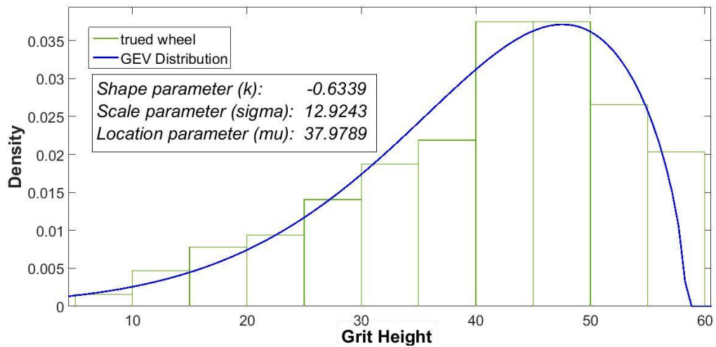
Figure 7-6 Probability density function of grit height for the trued wheel (wheel 4)
