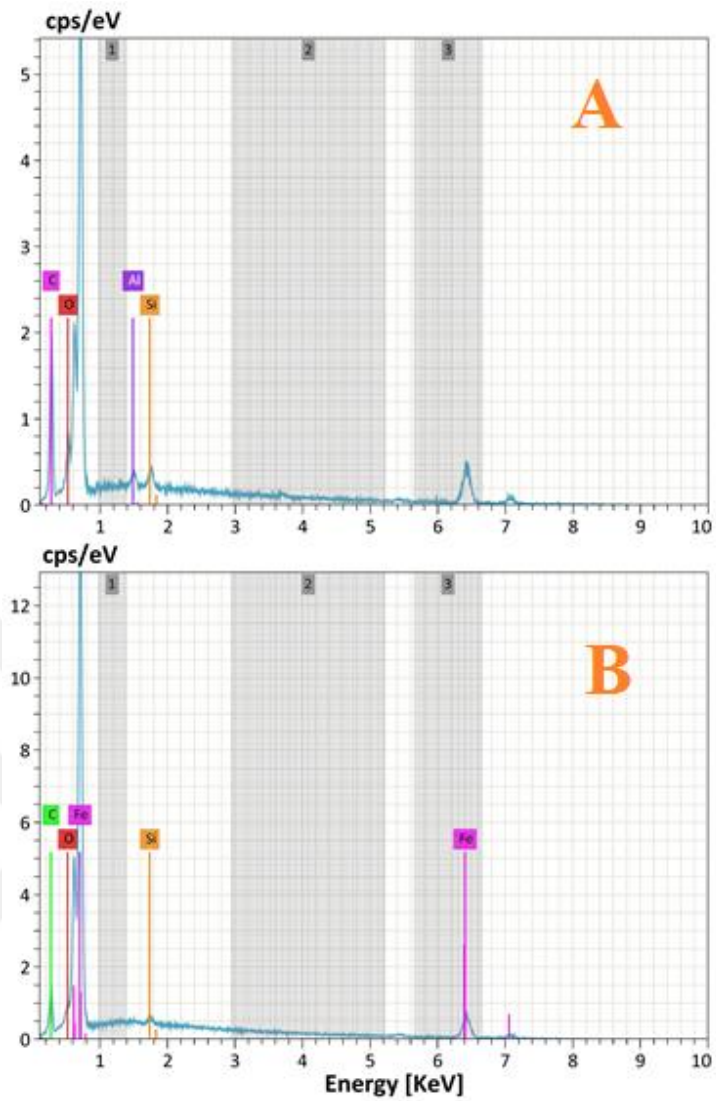
Figure 7-32 EDS analyze of sample 2 in two areas: A (Burn layer) and B(Bulk area)
