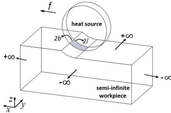
Figure 4-1 rectangular heat source in semi-infinite workpiece in grinding
