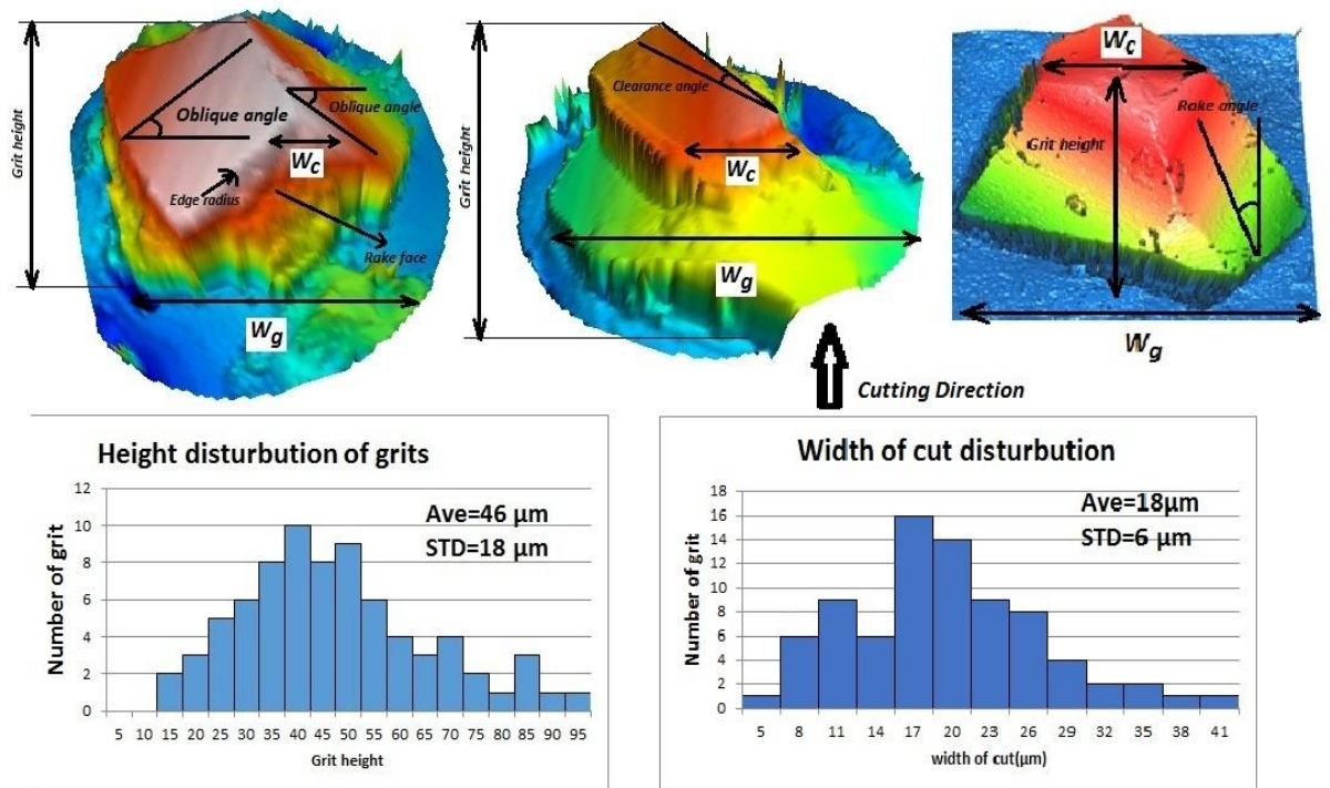
Figure 6-2 some grit picture and relevant geometric parameters along with height and width of cut distribution as two main parameters for kinematic-geometrical model
