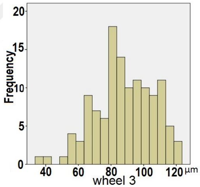
Figure 7-3 height distribution of the grit for wheel 3
