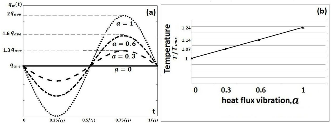
Figure 4-10 Effect of heat source fluctuation on the maximum temperature a) heat source profile for 1 wheel revolution, b) maximum temperature corresponding to each heat source at wet grinding condition, h=0.07 W/mm 2 K, L=1.4
