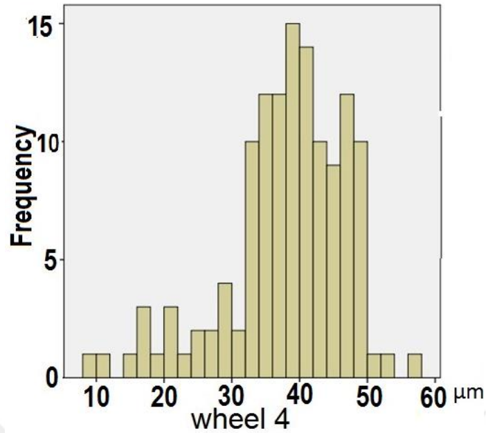
Figure 7-4 height distribution of the grit for wheel 4
