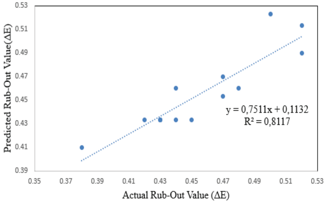
Figure 5.4. Regression Plot of Rub-Out (ΔE) for RAL 9010
