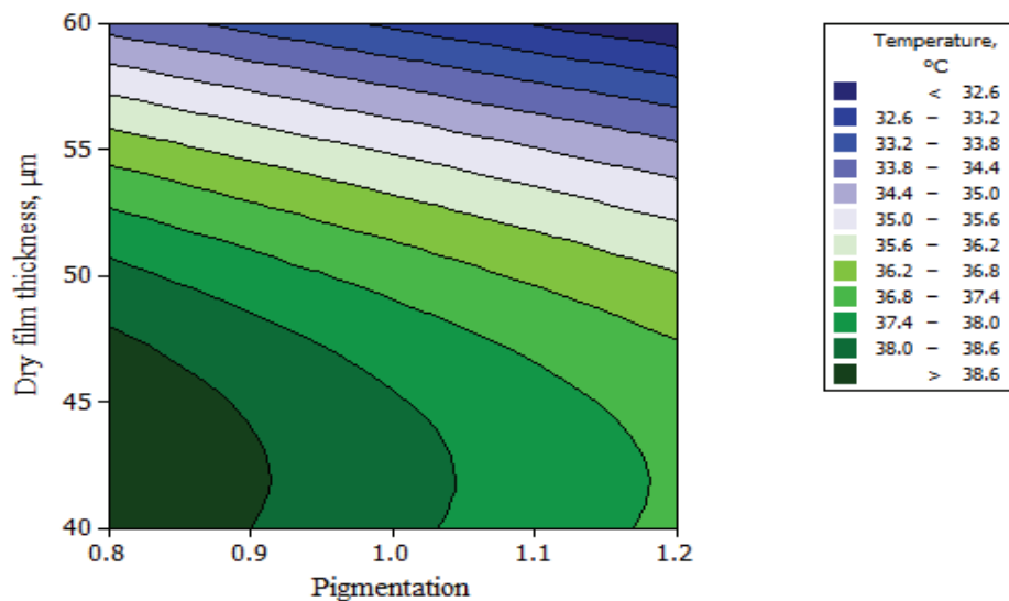
Figure 5.31. Contour Plot of \Delta Temperature ( ^{\circ}\text{C} ) vs. Dry Film Thickness ( \mu\text{m} ) and Pigmentation
