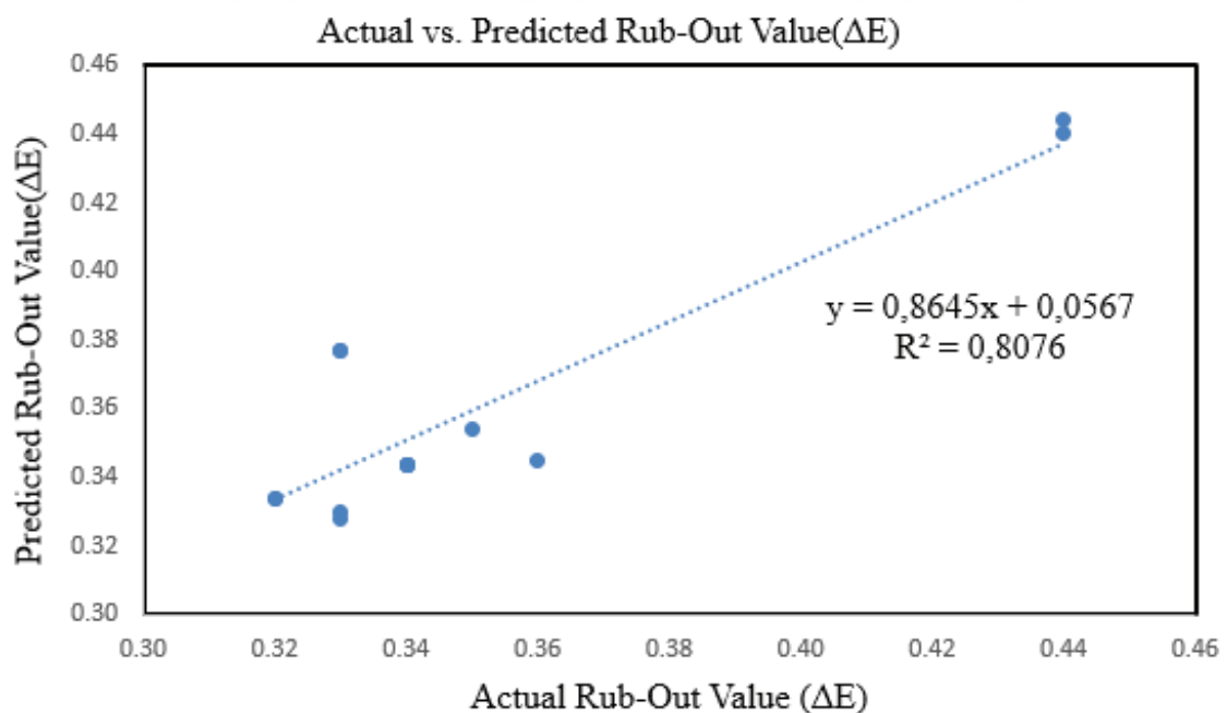
Figure 5.26. Regression Plot of Rub-Out ( \Delta E ) for RAL 9011
