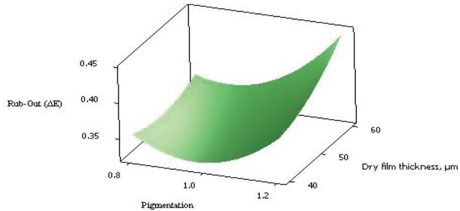
Figure 5.30. 3D Surface Plot of Rub-Out vs. Dry Film Thickness ( \mu\text{m} ) and Pigmentation
