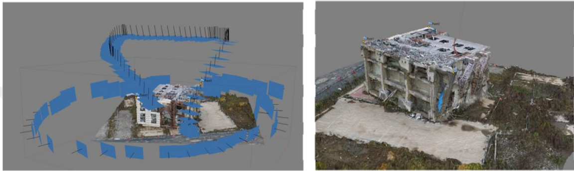
Figure 3.14. Estimated camera positions (left) and generated 3D model from both aerial and ground photos (right) (Yamazaki et al., 2015).
