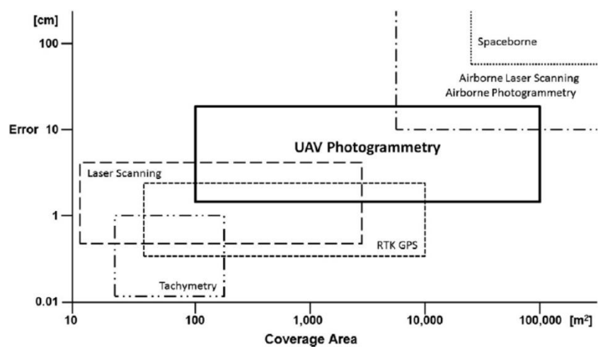
Figure 3.2. UAV applications for surveying tasks (Siebert and Teizer, 2014).
