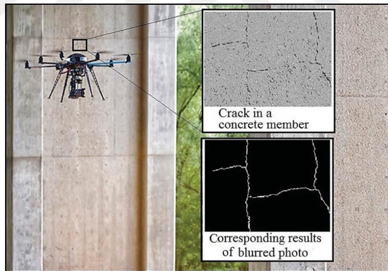
Figure 3.13. Detecting concrete cracks using drones (Li and Liu, 2018).
