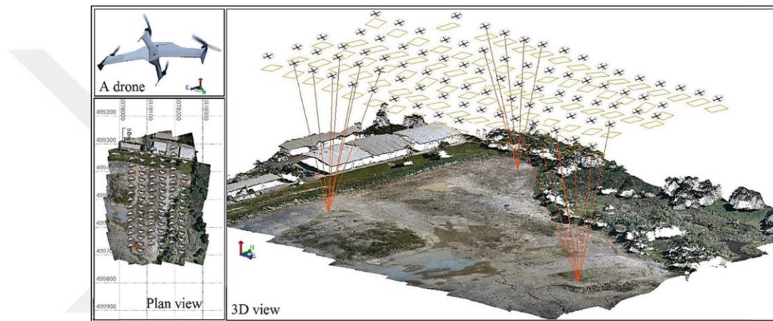
Figure 3.1. Drone-based photogrammetry (Li and Liu, 2018).
