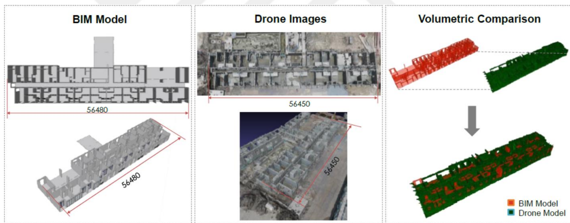
Figure 3.9. Volumetric comparison between construction plan and on-site progress (Anwar et al., 2018).
