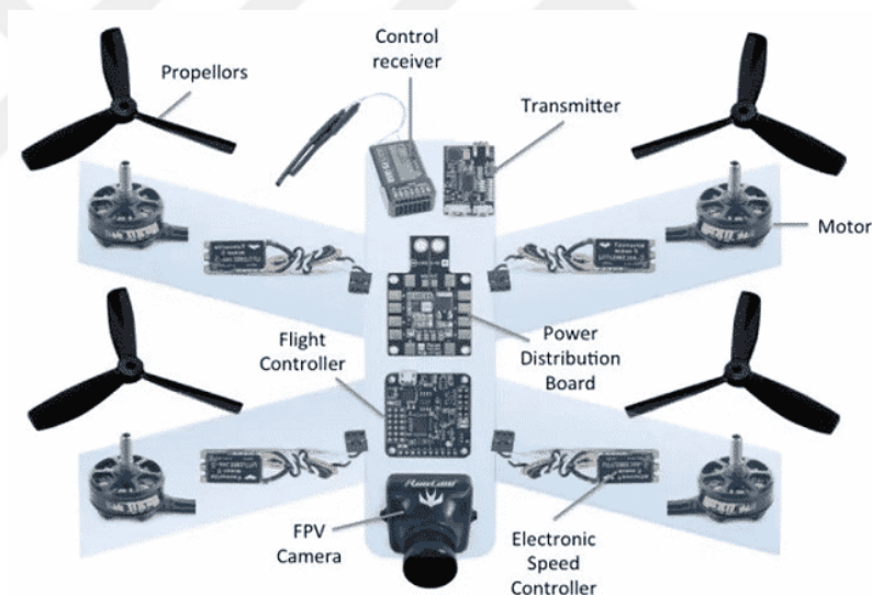
Figure 2.14. Components of a UAV system (Electricalfundablog).
