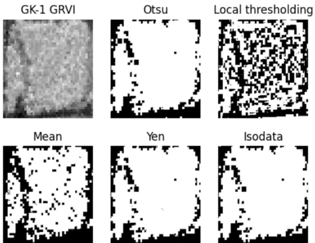
Figure 5.19: GK-1 GRVI Thresholds
