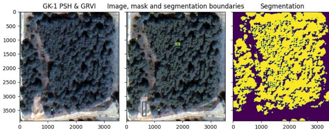
Figure 5.8: GK-1 Pan-Sharpener image and GRVI results with RF.
