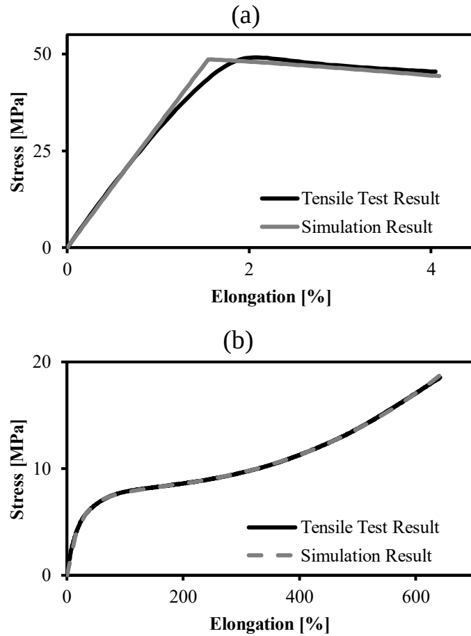
Figure 2.18. The tensile test result versus simulation result graph for (a) PLA and (b) TPU specimens.
