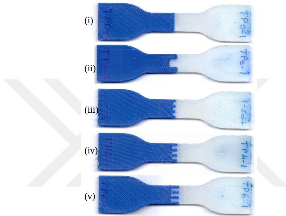
Figure 2.4. Flat interface specimen (TP0) (i), shear test specimen (ii), and combed specimens having (iii) 2 mm (iv) 4 mm (v) 6 mm comb lengths. Blue parts are printed with PLA and white parts with TPU filament.
