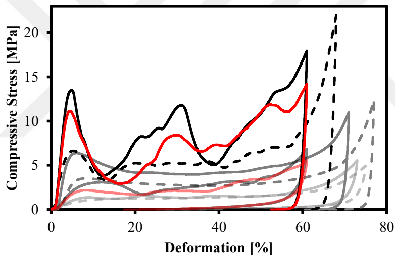
Figure 3.11. Compressive test results of the honeycomb (black), gyroid (gray), and Voronoi (red) infill patterns for both PA and PAHT CF15 specimens.
