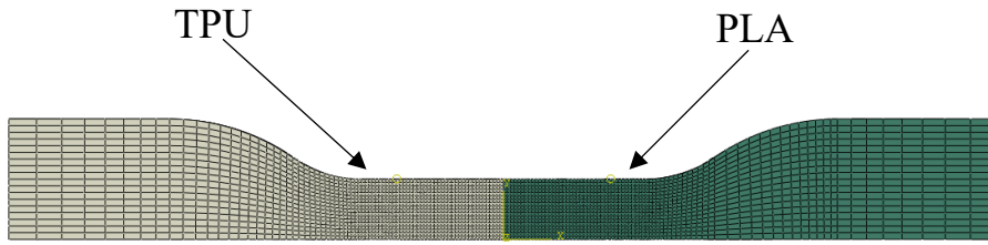
Figure 2.6. Screenshot of discretized flat interface specimen, half of the specimen was modeled using symmetry boundary conditions.
