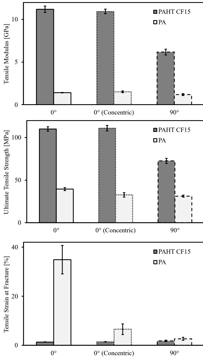
Figure 3.10. Tensile modulus, ultimate tensile strength, and tensile strain at fracture values of the PA and PAHT CF15 specimens for concentric infill, 0°, and 90° raster angles.
