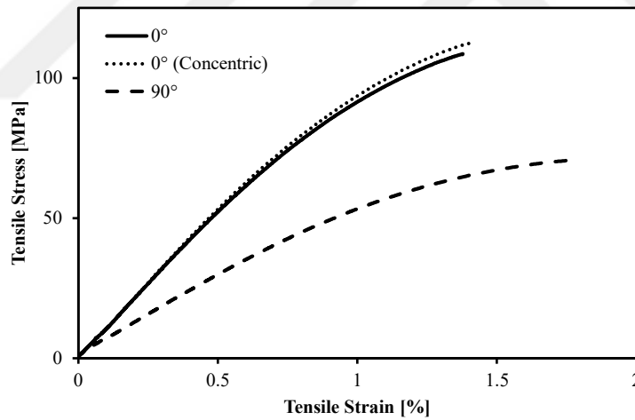
Figure 3.6. Tensile stress versus tensile strain plot of PAHT CF15 specimens for concentric infill, 0^\circ , and 90^\circ raster angles.
