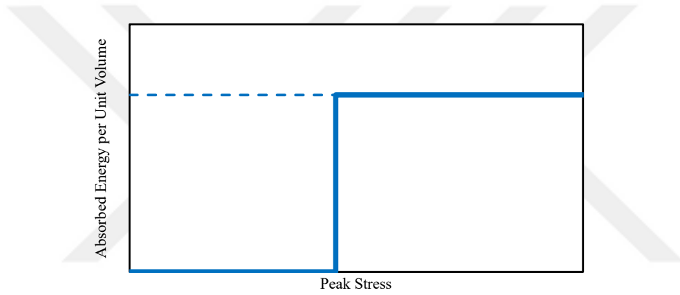
Figure 3.4. Absorbed energy per unit volume versus peak stress diagram of an ideal energy absorber.
