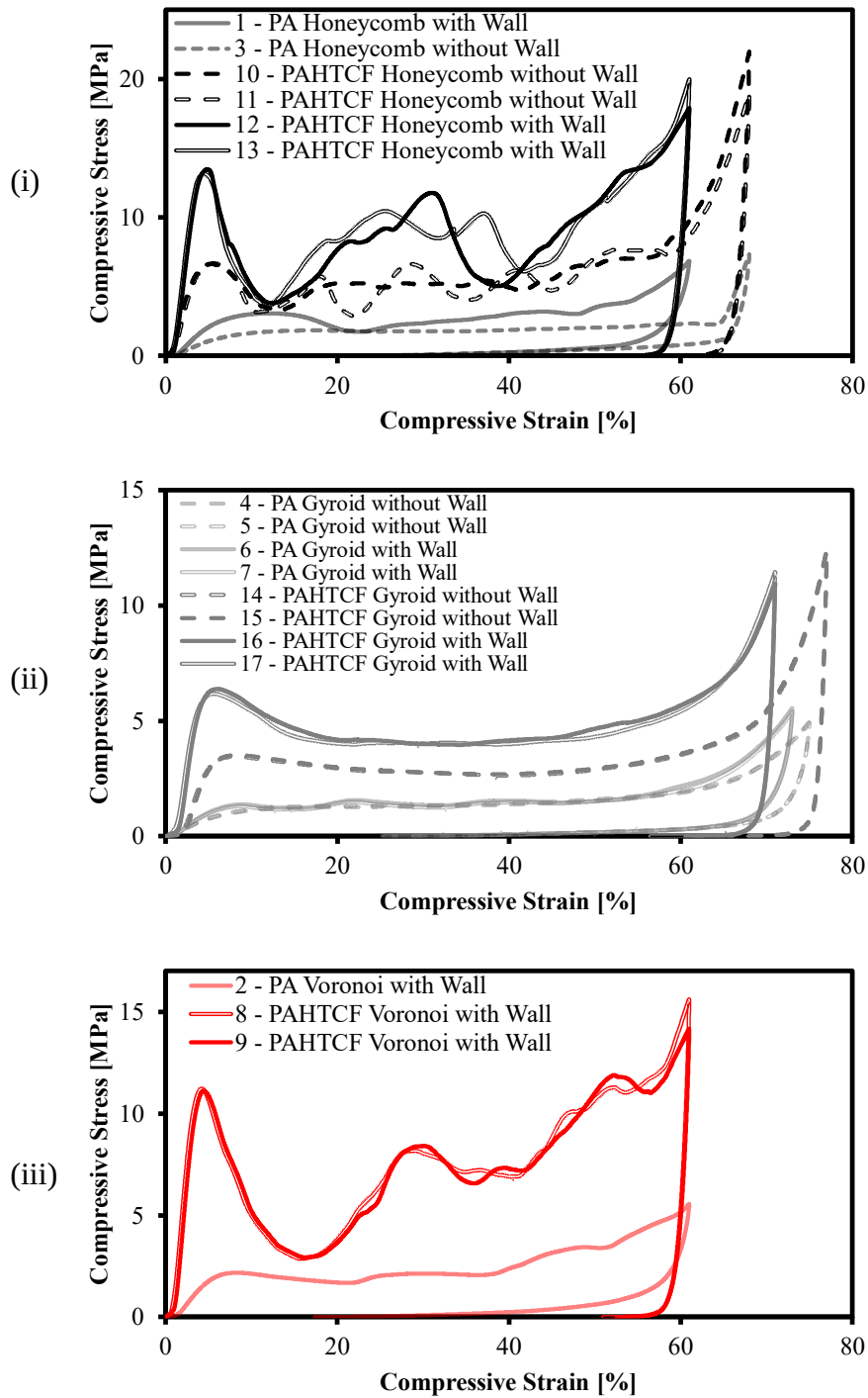
Figure 3.12. Compressive test results of (i) honeycomb, (ii) gyroid, (iii) Voronoi infill patterns for both PA and PAHT CF15 materials.
