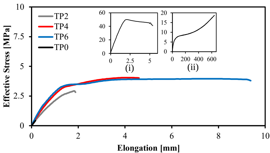
Figure 2.13. Effective stress versus tensile deformation response of the combed specimens having 0, 2, 4, and 6 mm comb lengths. The insets are (i) stress versus percent elongation graph of the PLA tensile test specimen and (ii) stress versus percent elongation graph of the TPU specimen.
