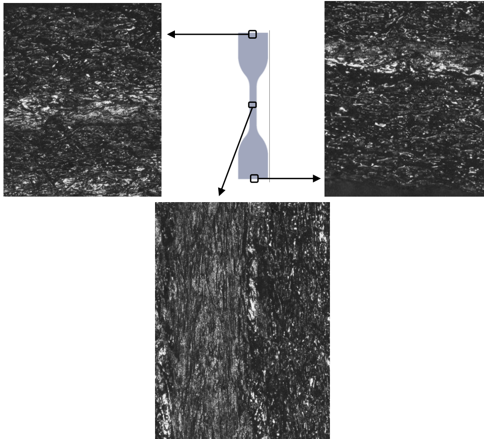
Figure 3.8. The optical microscopy image showing the top surface of a concentric infill tensile test specimen.
