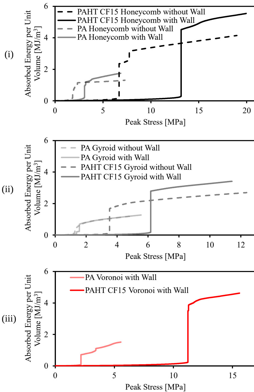
Figure 3.13. Peak stress versus absorbed energy per unit volume graph of compressive test specimens printed using (i) honeycomb, (ii) gyroid, and (iii) Voronoi infill with and without wall.
