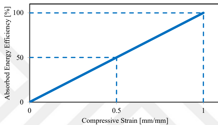
Figure 3.5 Absorbed energy efficiency versus compressive strain graph for an ideal energy absorber.
