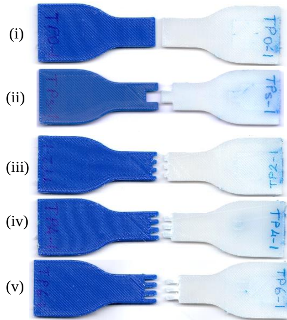
Figure 2.10. The photographs of multi-material specimens after the uniaxial tensile tests. The flat interface (i), shear test specimen (ii), and combed specimens having (iii) 2 mm (iv) 4 mm (v) 6 mm comb lengths.
