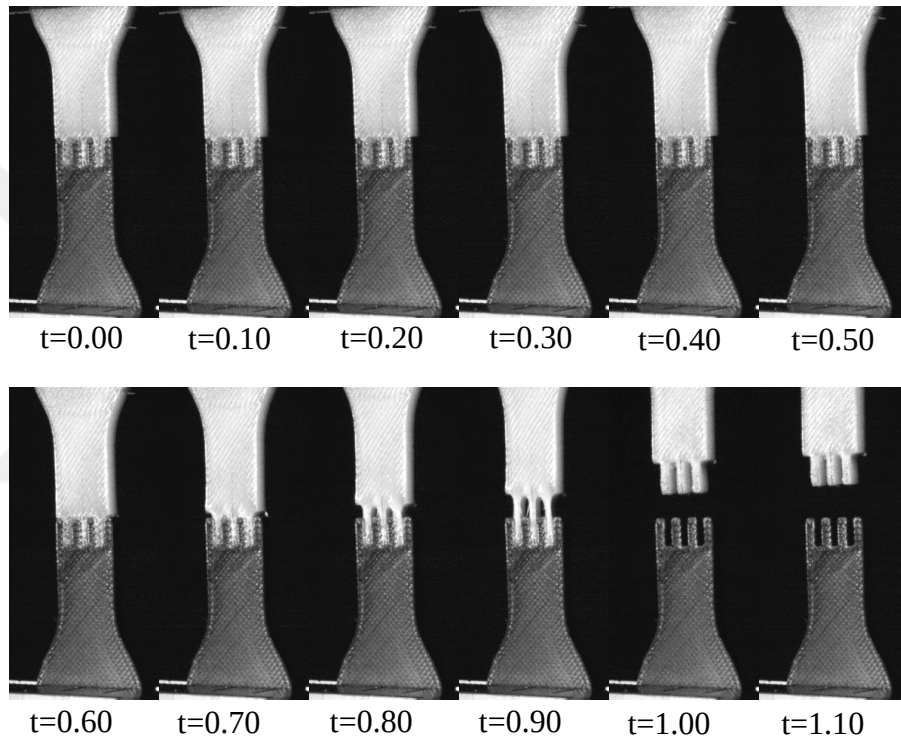
Figure 2.16. The snapshots from the tensile test video of the multi-material combed tensile test specimen with a comb length of 6 mm.
