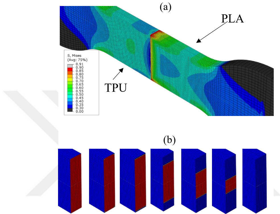
Figure 2.19. (a) The Von-Mises stress state of the flat interface specimen just before the crack initiation (b) Snippets showing the progression of the cohesive contact loss at interface surface of the TPU specimen. The red regions show a bonded contact, and the blue regions indicate those not in contact.
