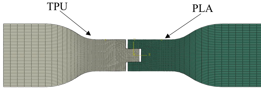
Figure 2.7. Screenshot of the discretized tensile shear test specimen, half of the specimen is modeled using symmetry boundary conditions.
