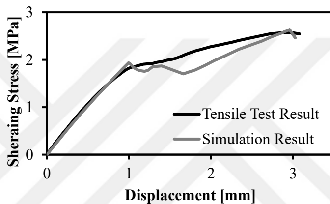
Figure 2.21. Tensile test result versus simulation result graph for the shear test specimen.
