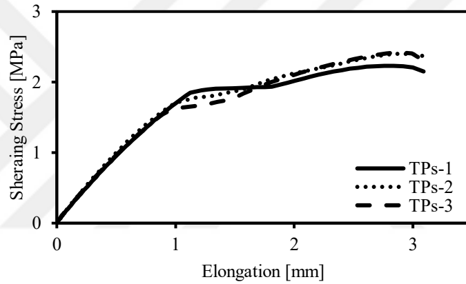
Figure 2.14. Stress versus elongation diagram of the shear stress test specimens. Shearing stress is calculated using the total interfacial area. The elongation value shows the total tensile elongation of the tensile test specimen in the gage length.
