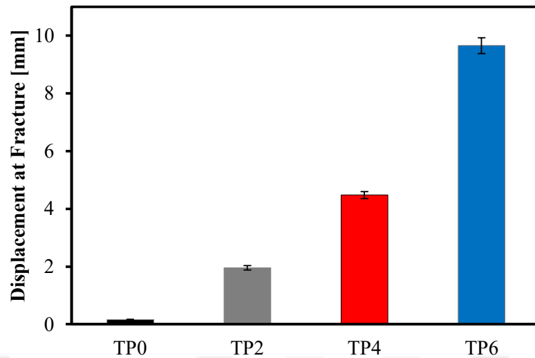
Figure 2.12. Displacement at fracture of the comb interface specimens having 0, 2, 4, and 6 mm comb lengths.
