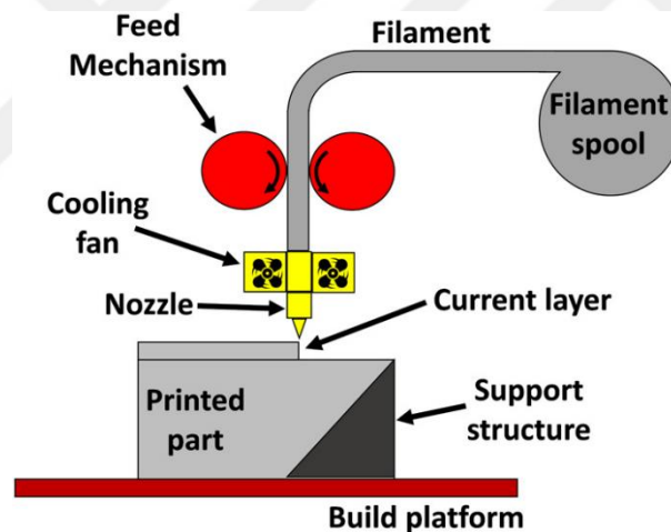
Figure 1.1. Schematic illustration of a typical FFF 3D printer [23].
