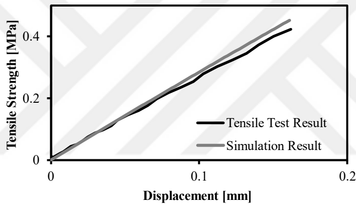
Figure 2.20 Tensile test result versus simulation result graph for TP0 specimen.
