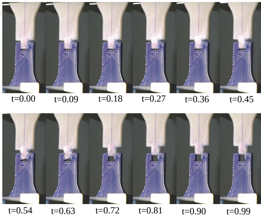
Figure 2.15. The snippets from the tensile test video of the multi-material shear tensile test specimen. The blue markings are drawn with a pen for alignment and to use in the post-processing of the video.
