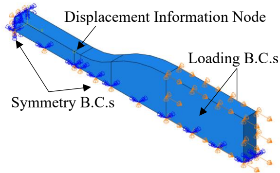
Figure 2.5. The screenshot showing the boundary conditions used in the simulations of PLA and TPU specimens.
