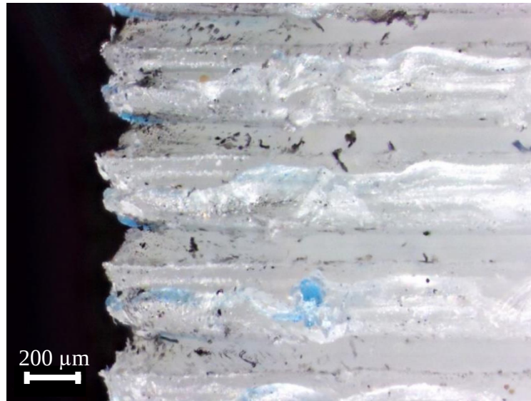
Figure 2.17. Optical microscopy image of a fractured interface of TPU part of the dogbone tensile shear test specimen.
