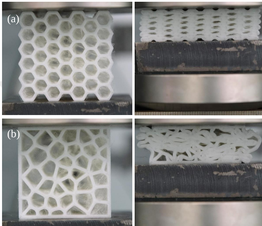
Figure 3.15. The photographs of the (a) best and (b) worst performing specimens.
