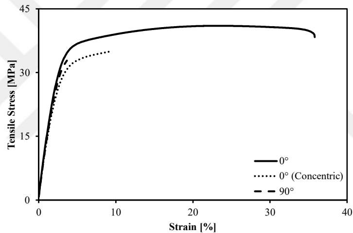
Figure 3.7. Tensile test results of PA specimen tensile test specimens, for concentric infill, 0°, and 90° raster angles.
