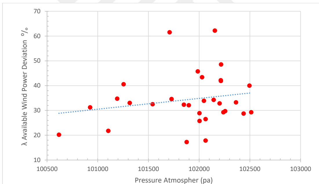
Figure B.3.4 Wind power deviation with atmospheric pressure
