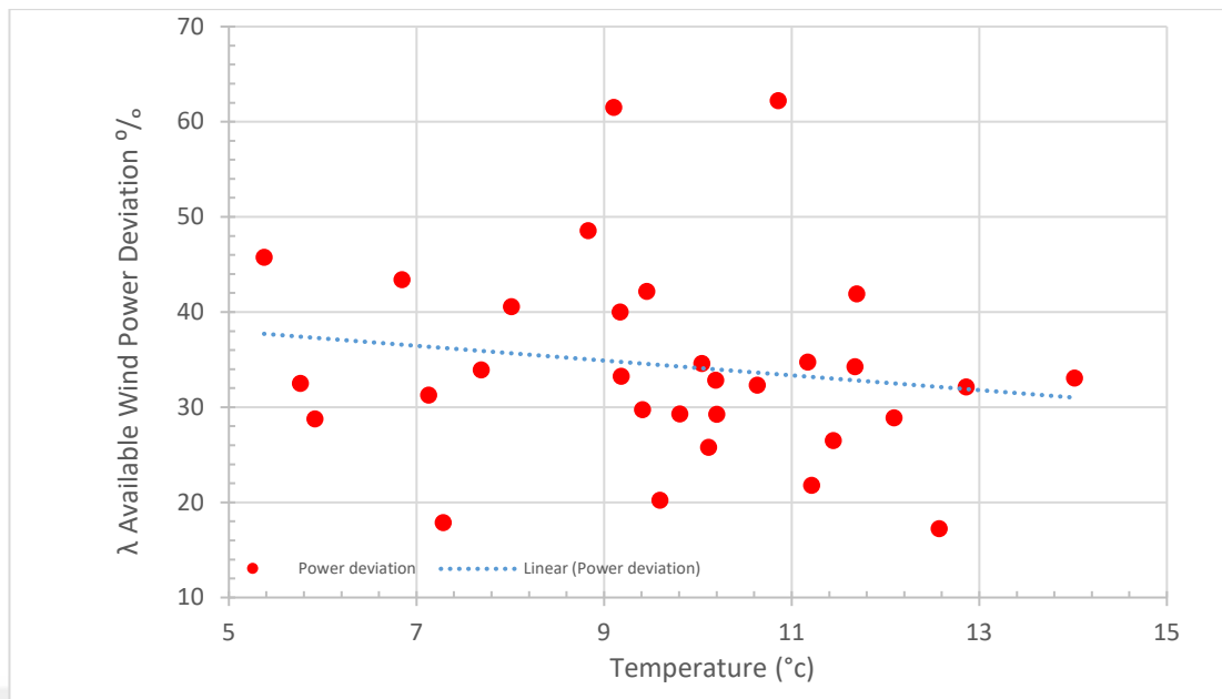
Figure B.3.3 Wind power deviation with temperature
