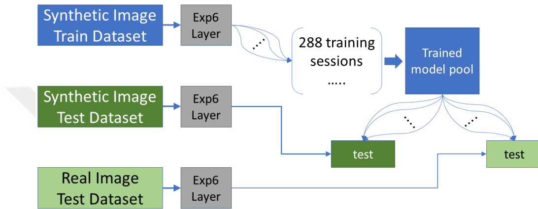
Figure 4.11 Experiment 6 train and test scenario schematic representation.
