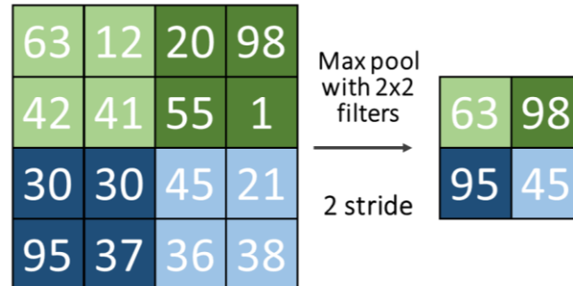
Figure 2.10 Max pooling process and result.
