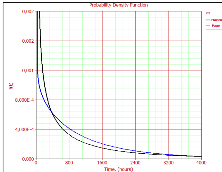
Figure A.40 PDF curves of Bucket – Ringbolt
