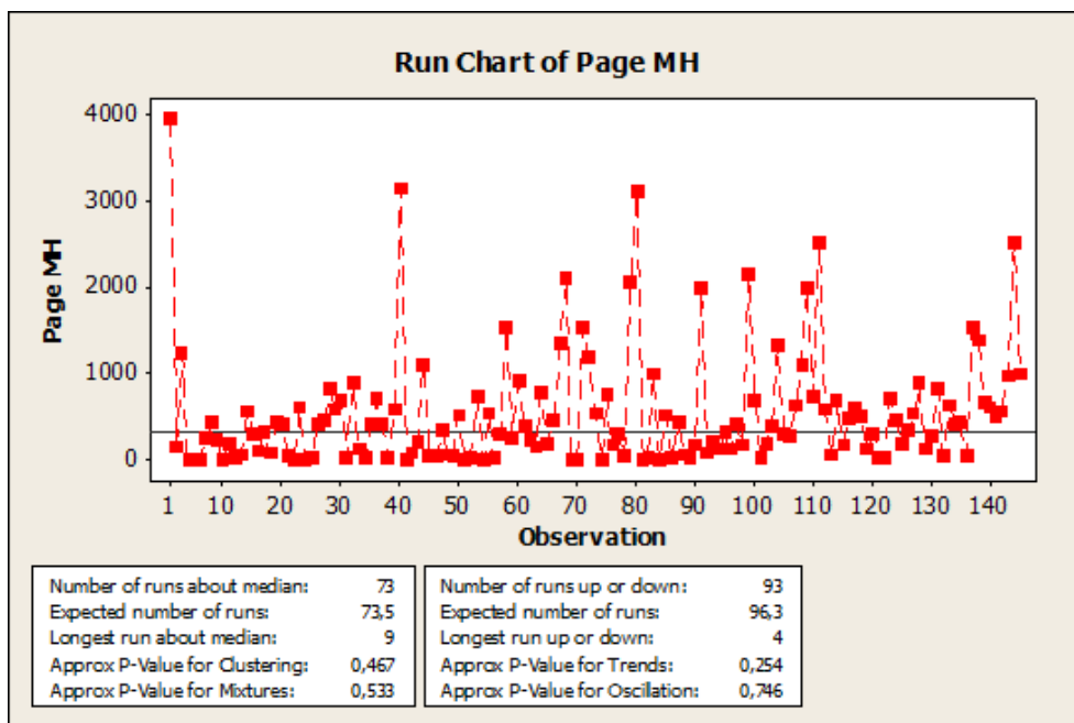
Figure A.14 Runs chart for Page's machinery house
