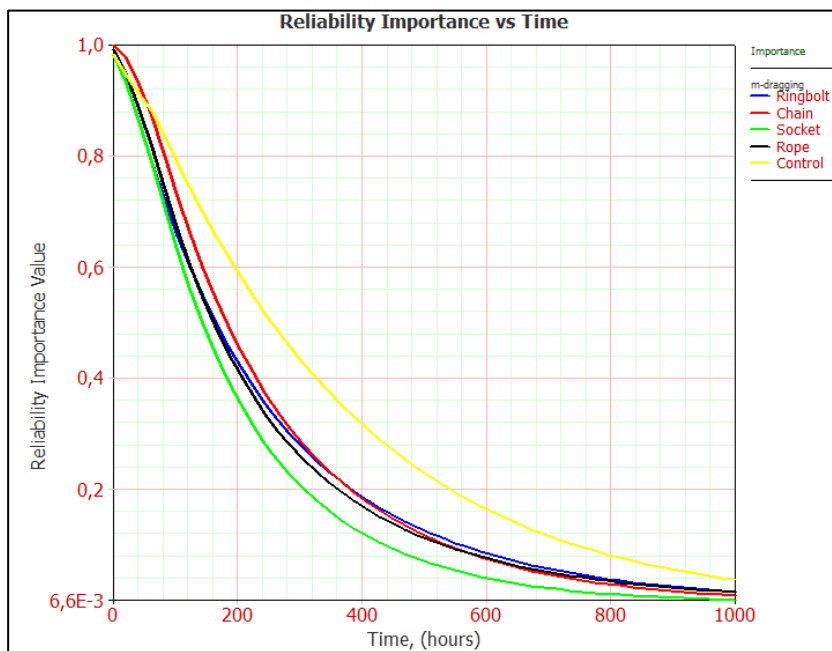
Figure A.22 Changes in importance values with time (Marion-Drugging)
