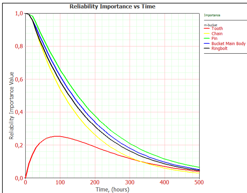
Figure A.46 Changes in importance values with time (Marion-Bucket)
