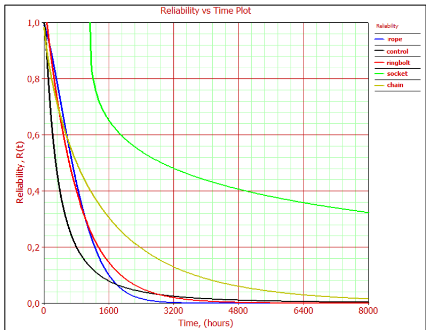
Figure A.20 Reliability curves of components (Marion-Dragging)
