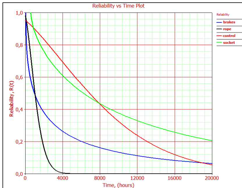
Figure A.28 Reliability curves of components (Page-Hoisting)
