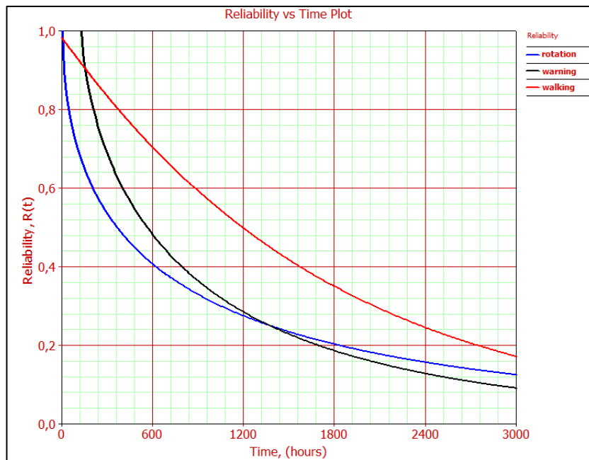
Figure A.52 Reliability curves of components (Page-Movement)
