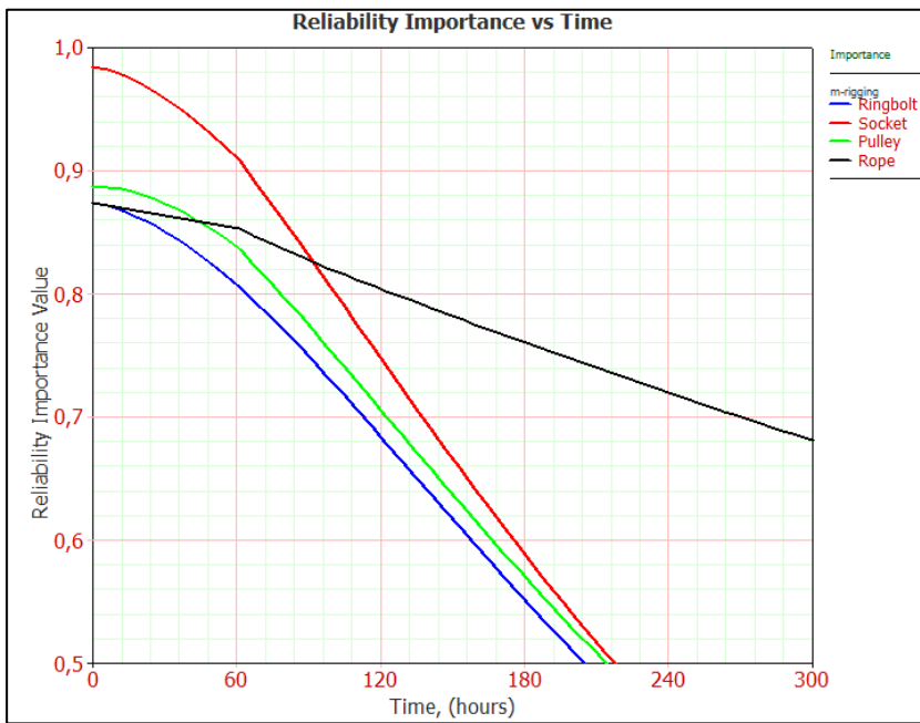
Figure A.37 Changes in importance values with time (Marion-Rigging)
