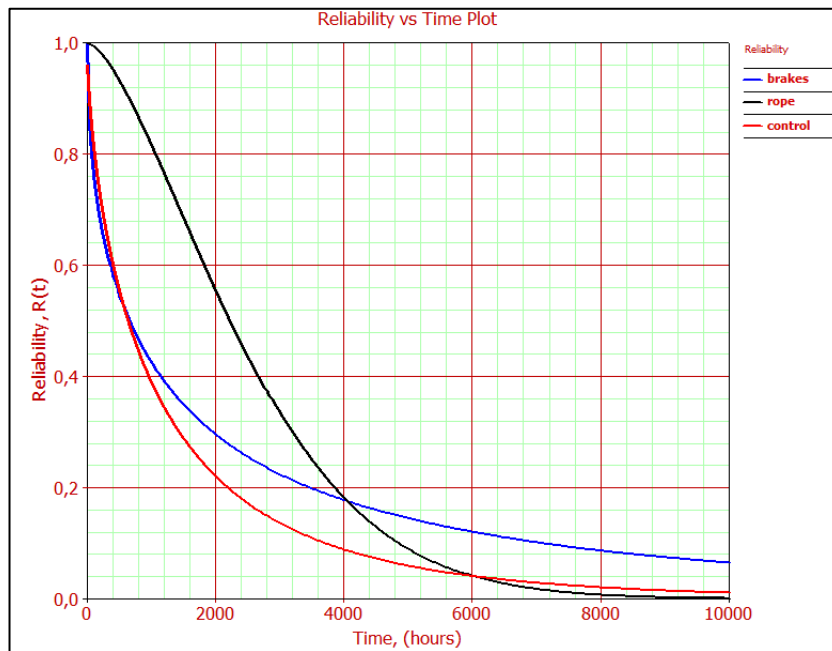
Figure A.27 Reliability curves of components (Marion-Hoisting)
