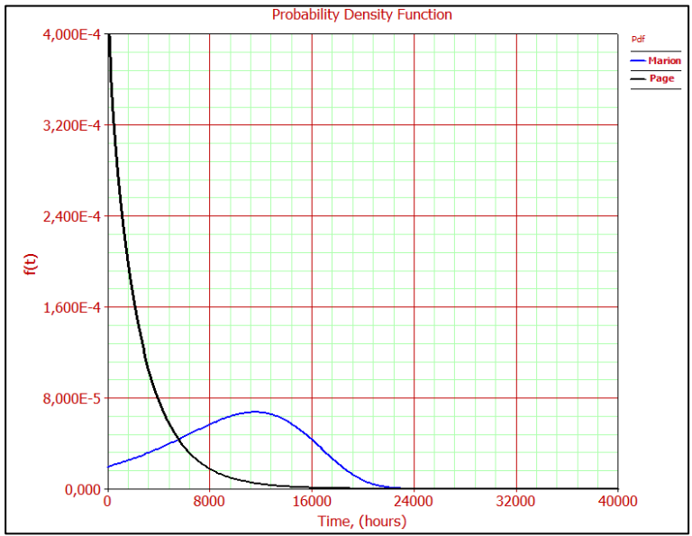
Figure A.34 PDF curves of Rigging - Socket
