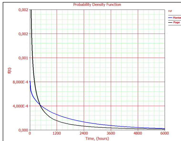
Figure A.48 PDF curves of Movement – Rotation
