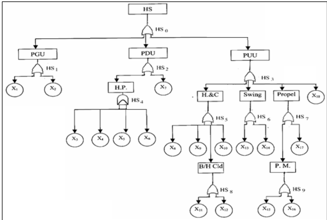
Figure 2.4 Fault tree representation of the system (Samanta et al. , 2002)
