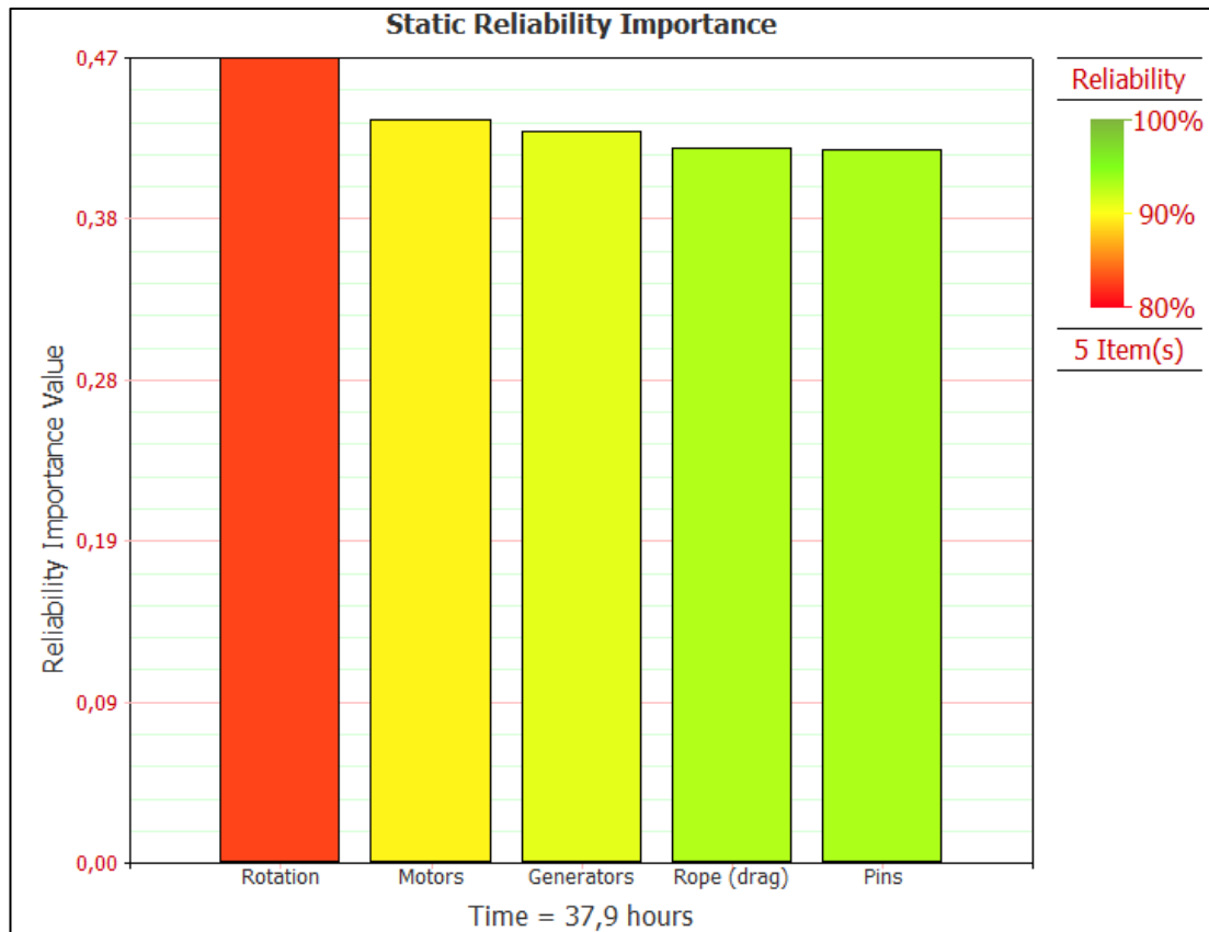
Figure 4.18 5 components with highest RI values at Page's mean life
