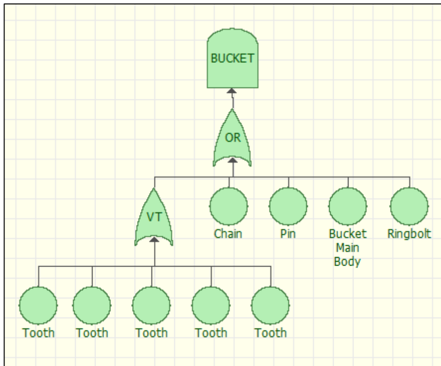
Figure 4.10 Fault tree representation of bucket units
