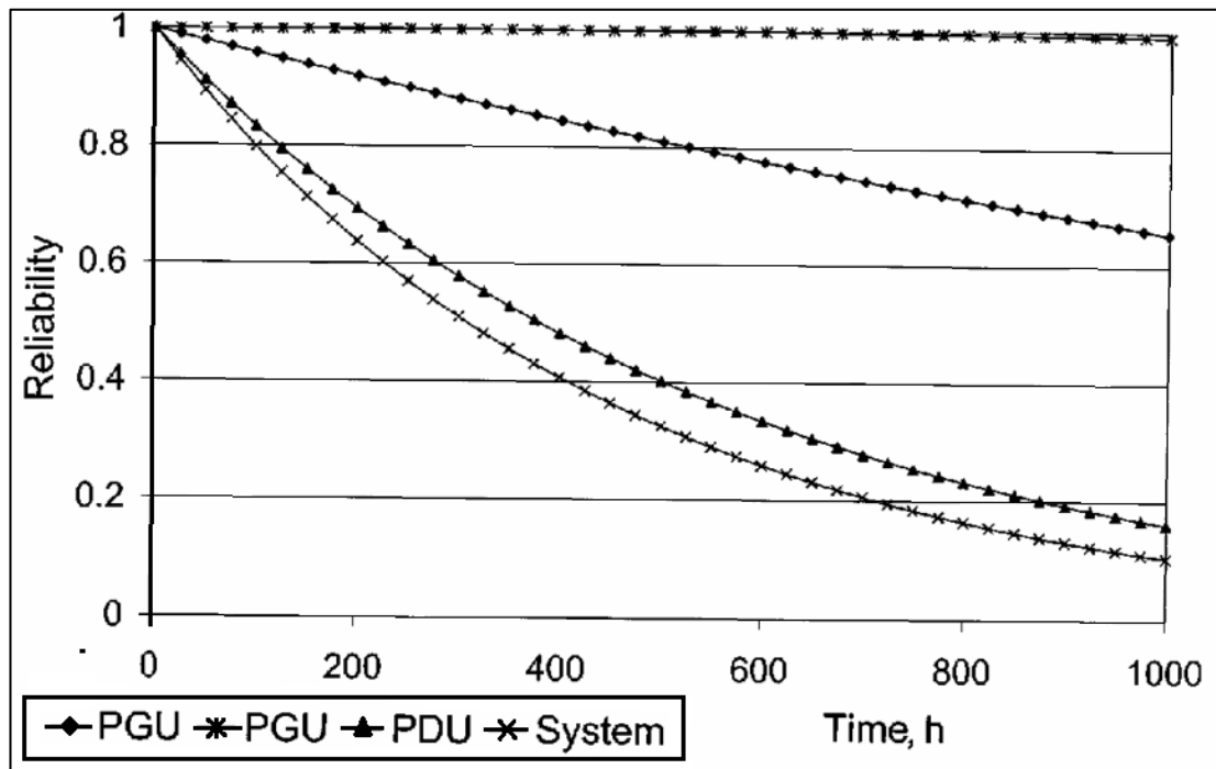
Figure 2.6 Reliability changes with time for the shovel and the subsystems (Samanta et al. , 2002)
