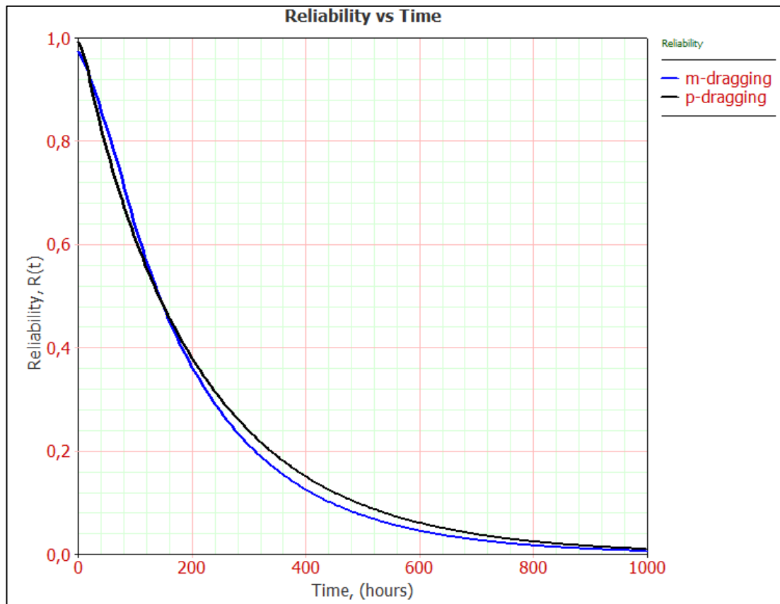
Figure 4.5 Reliability graph of dragging units
