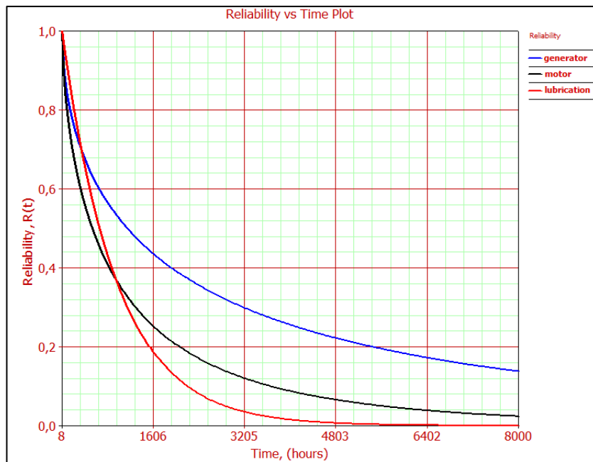
Figure A.60 Reliability curves of components (Page-Machinery House)
