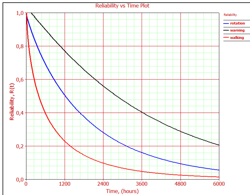
Figure A.51 Reliability curves of components (Marion-Movement)
