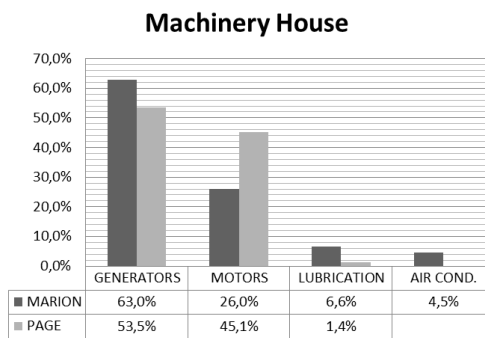
Figure A.2 Ratio of component downtimes to total unit downtimes
