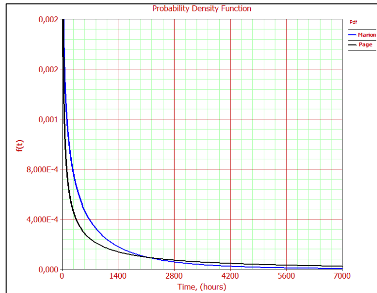
Figure A.55 PDF curves of Machinery House – Generators
