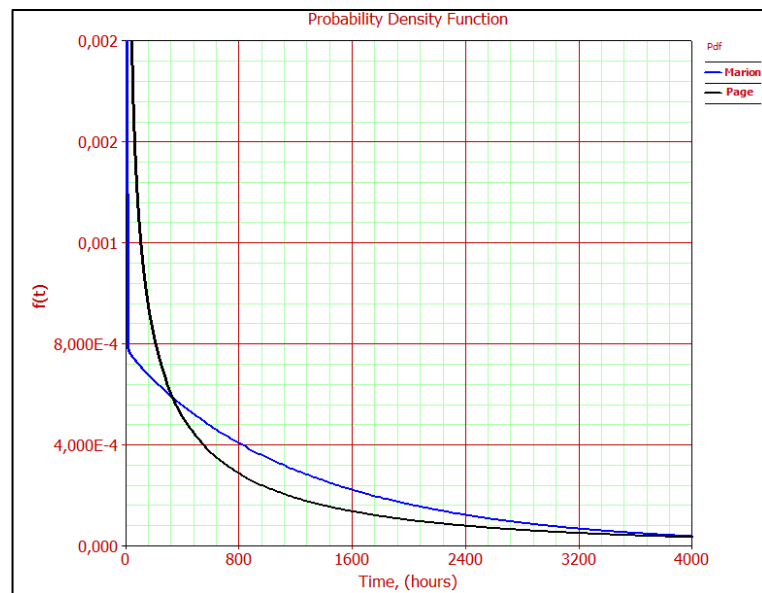
Figure A.56 PDF curves of Machinery House – Motors
