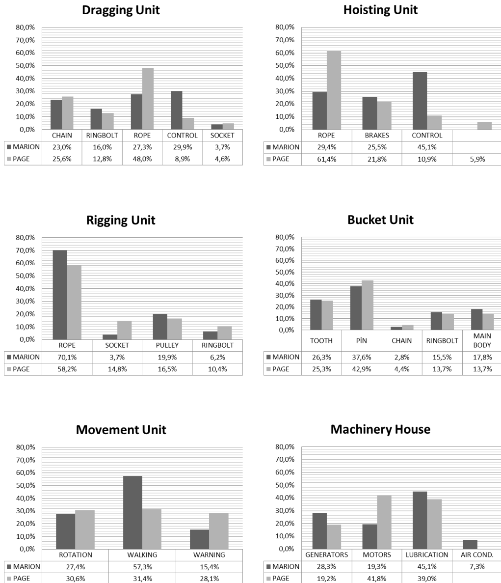
Figure A.1 Ratio of components' number of failures to total number of failures
