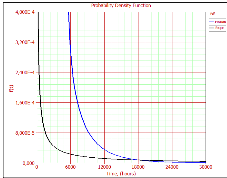
Figure A.43 PDF curves of Bucket – Chains
