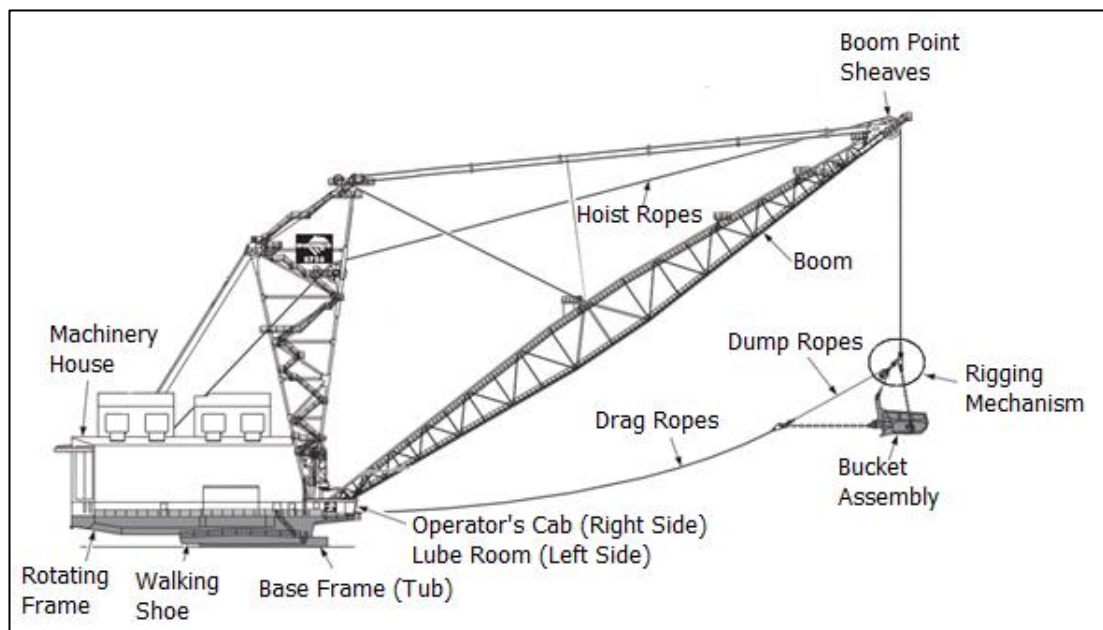
Figure 4.1 Main components of a dragline (modified from Oresome Resources, n.d.)
