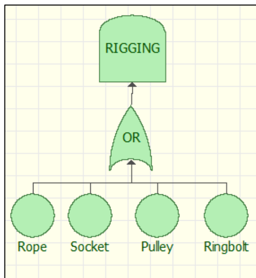
Figure 4.8 Fault tree representation of rigging units
