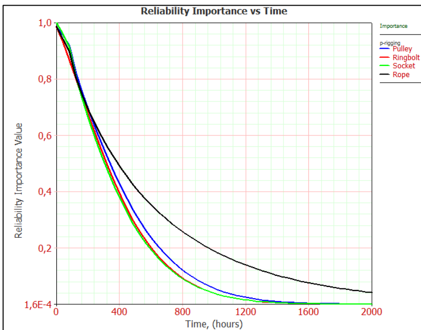
Figure A.38 Changes in importance values with time (Page-Rigging)
