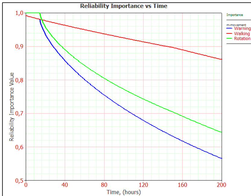
Figure A.53 Changes in importance values with time (Marion-Movement)
