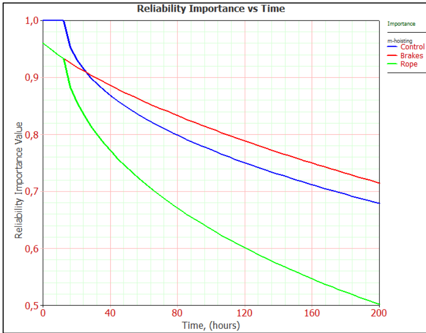
Figure A.29 Changes in importance values with time (Marion-Hoisting)
