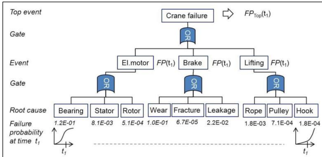
Figure 2.10 Fault tree representation of the crane system (Halme and Aikala, 2012)
