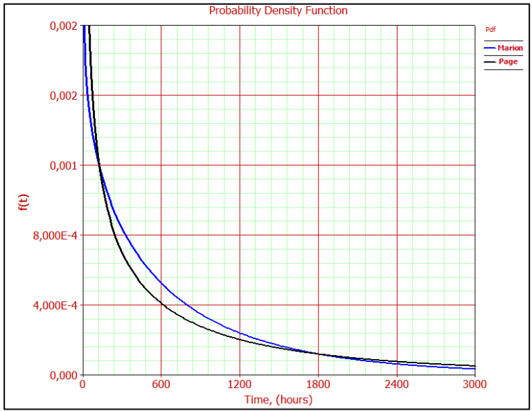
Figure A.41 PDF curves of Bucket – Teeth
