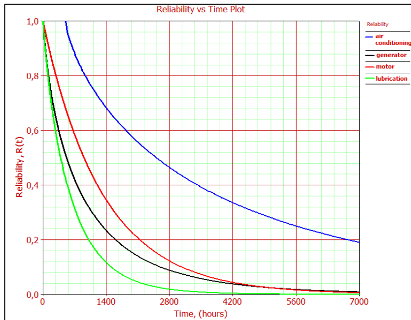
Figure A.59 Reliability curves of components (Marion-Machinery House)
