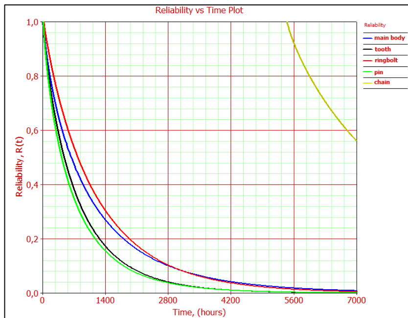
Figure A.44 Reliability curves of components (Marion-Bucket)
