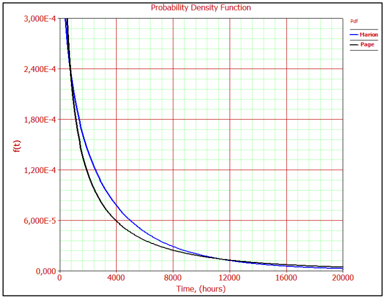
Figure A.33 PDF curves of Rigging – Ringbolt
