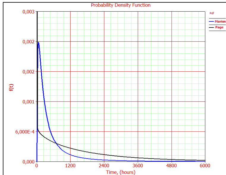
Figure A.16 PDF curves of Dragging - Control
