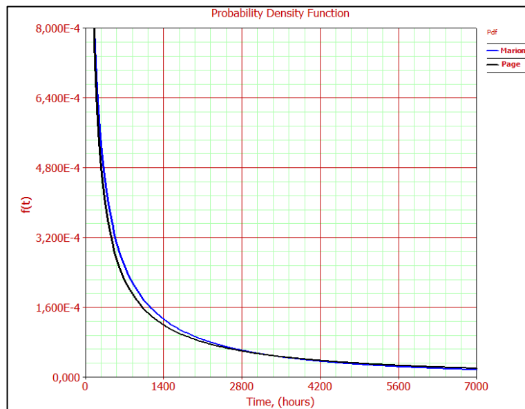
Figure A.24 PDF curves of Hoisting - Brakes
