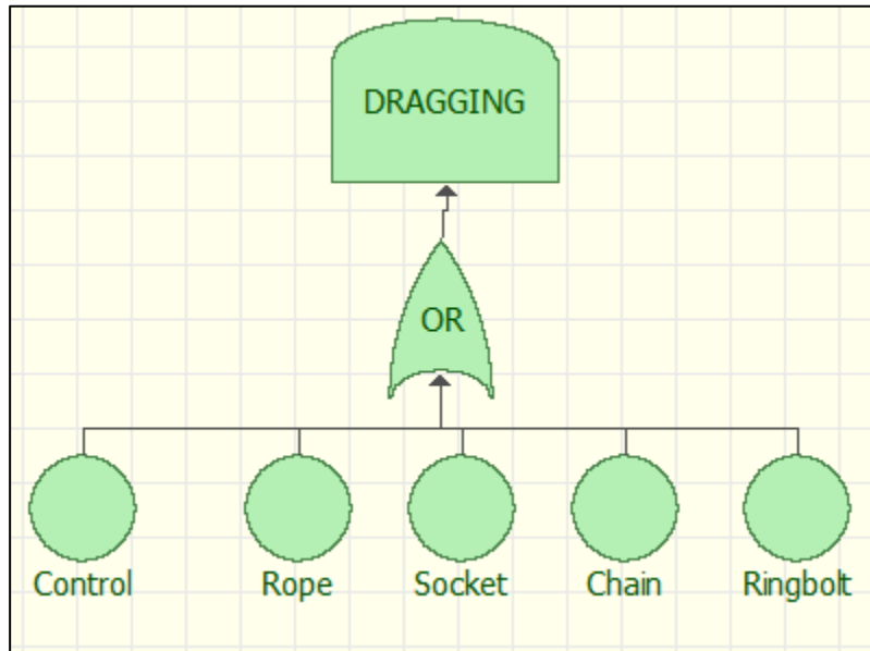
Figure 4.4 Fault tree representation of dragging units
