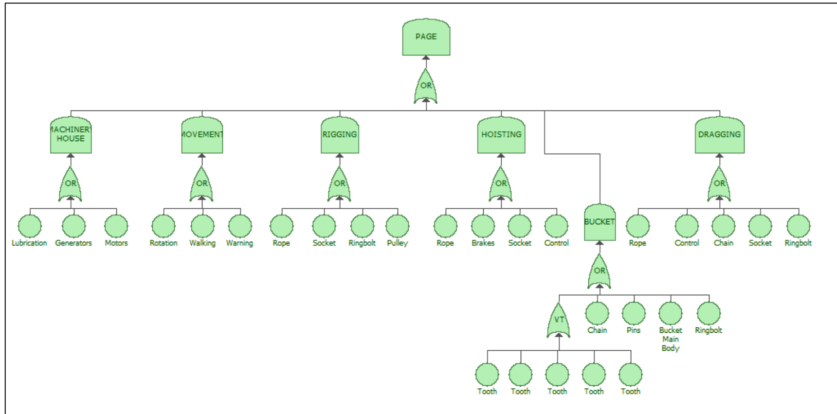
Figure 4.16 Fault tree representation of the dragline system (PAGE)
