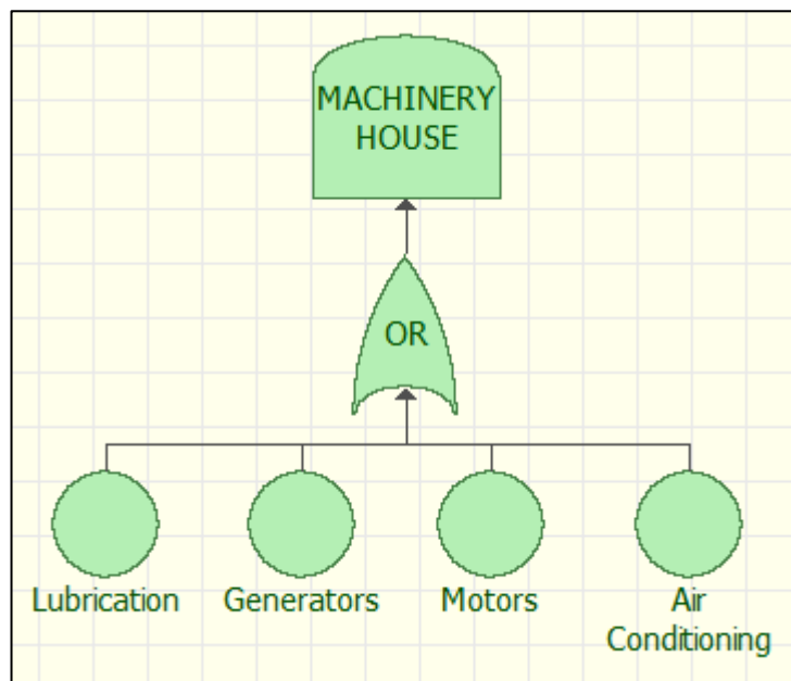
Figure 4.14 Fault tree representation of machinery houses
