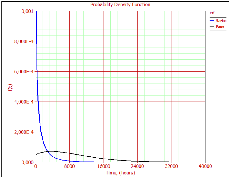
Figure A.26 PDF curves of Hoisting - Control
