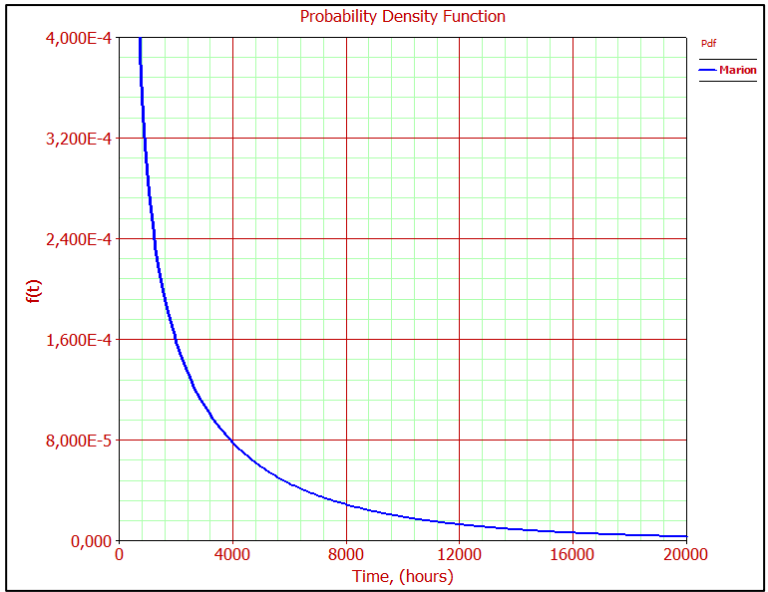
Figure A.58 PDF curves of Machinery House – Air Conditioning
