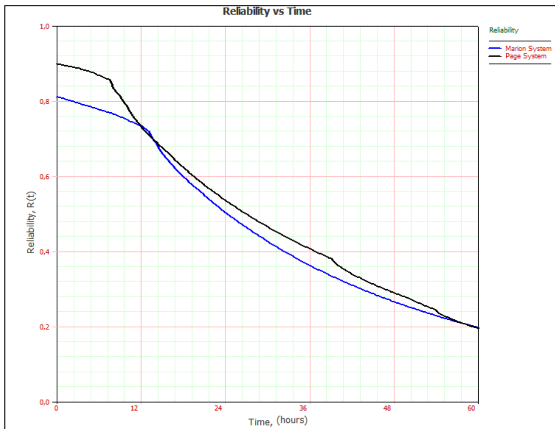
Figure 4.17 Reliability graph of the draglines
