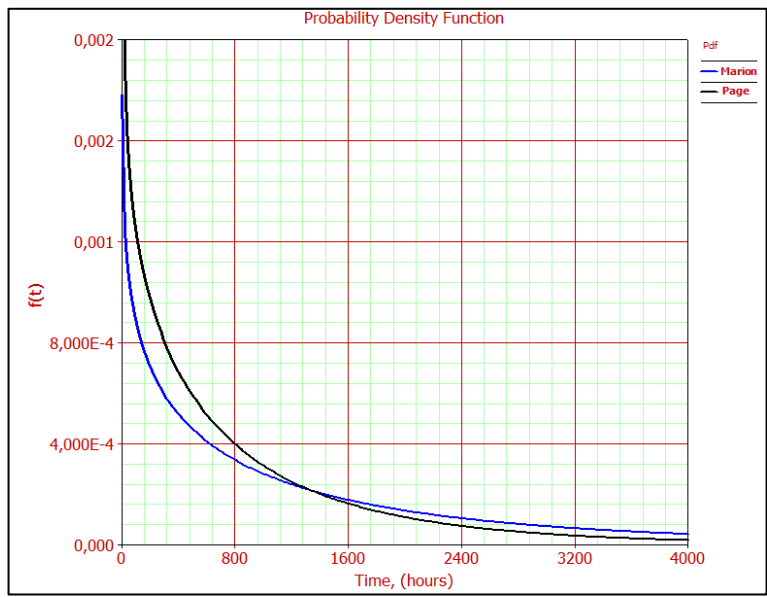
Figure A.19 PDF curves of Dragging – Chain
