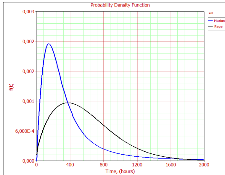
Figure A.31 PDF curves of Rigging - Rope
