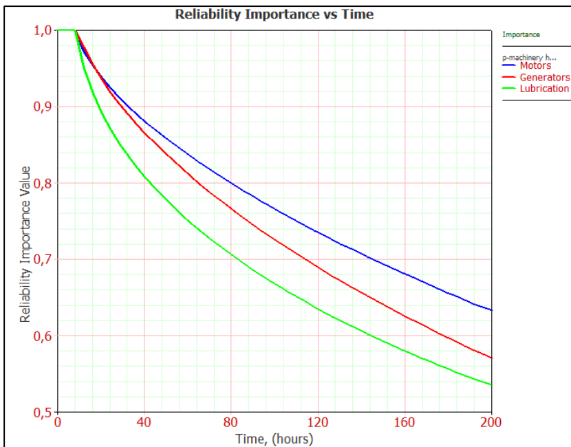
Figure A.62 Changes in importance values with time (Page-Machinery House)
