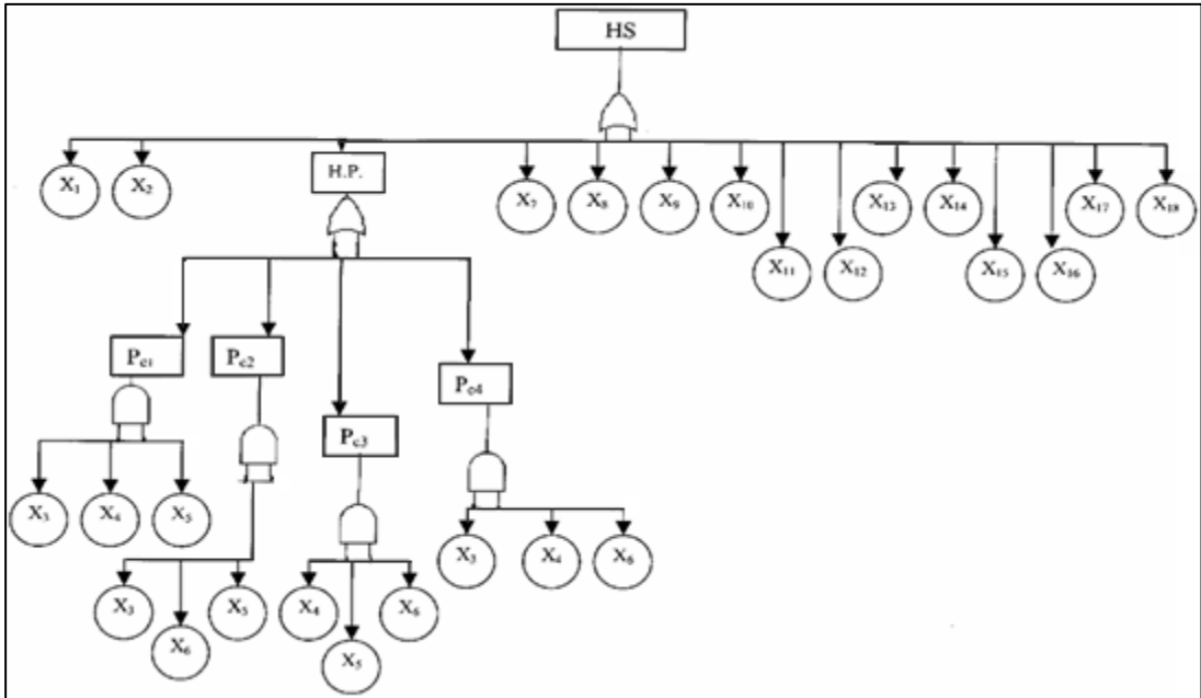
Figure 2.5 Simplified fault tree of the system (Samanta et al. , 2002)
