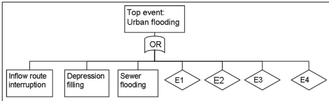
Figure 2.12 Fault tree representation for the urban flooding (Veldhius et al , 2011)
