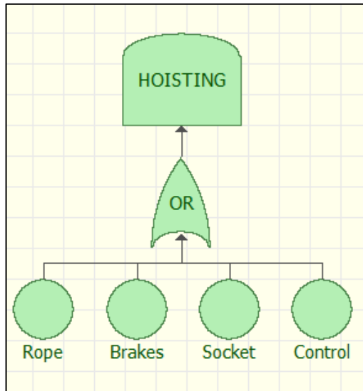
Figure 4.6 Fault tree representation of hoisting units
