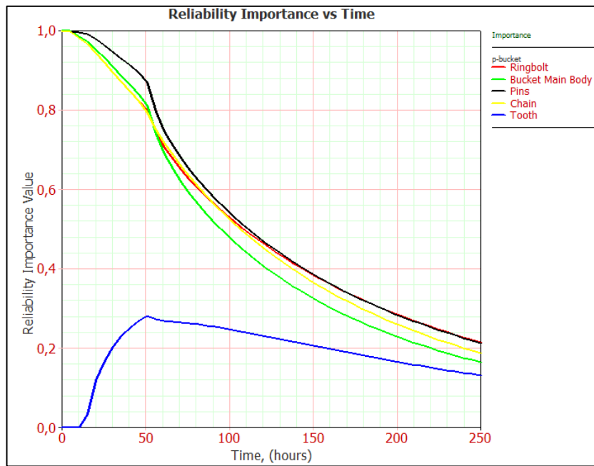
Figure A.47 Changes in importance values with time (Page-Bucket)
