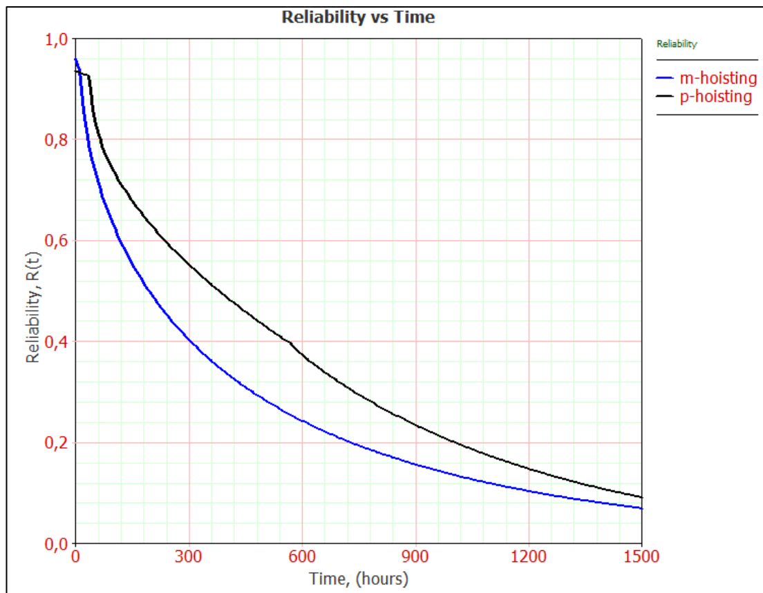
Figure 4.7 Reliability graph of hoisting units
