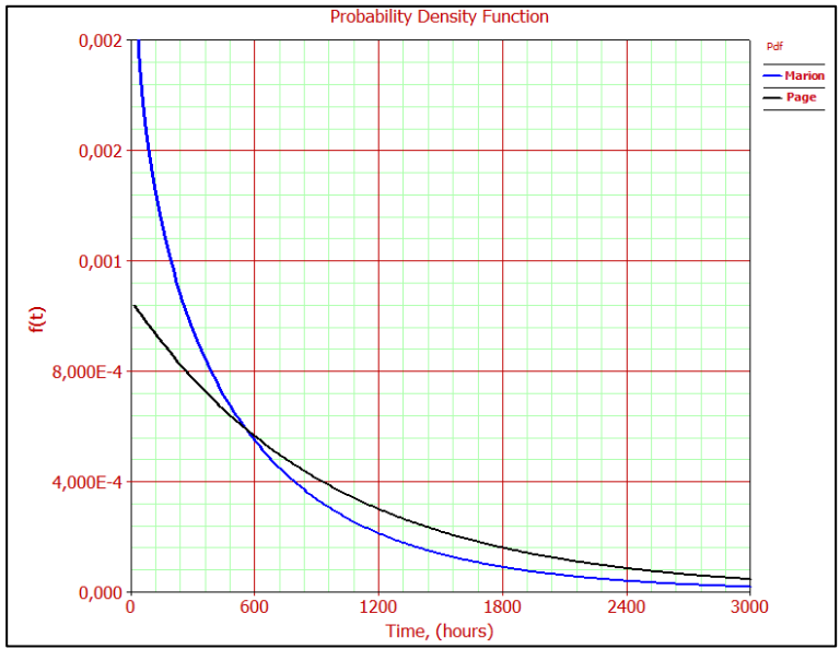
Figure A.57 PDF curves of Machinery House – Lubrication
