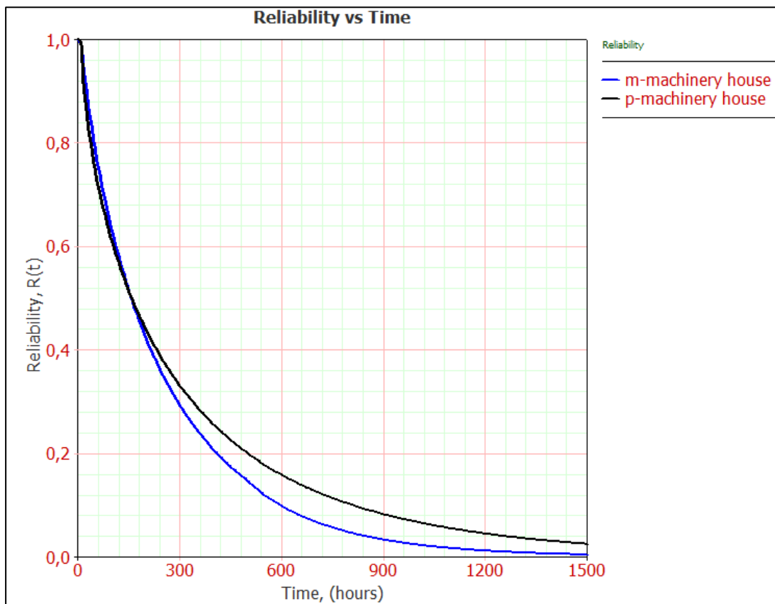
Figure 4.15 Reliability graph of machinery houses
