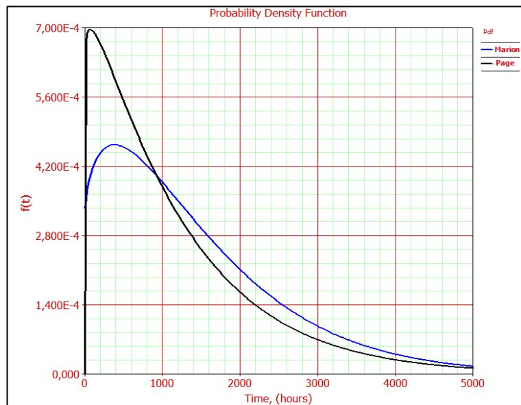
Figure A.32 PDF curves of Rigging - Pulley
