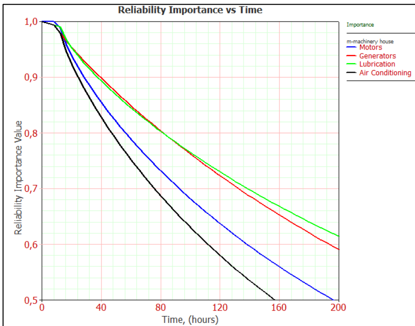
Figure A.61 Changes in importance values with time (Marion-Machinery House)
