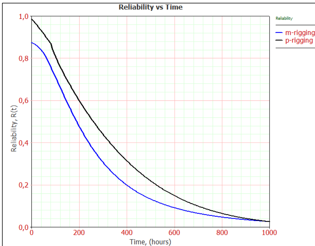
Figure 4.9 Reliability graph of rigging units
