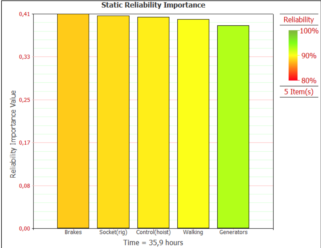
Figure 4.19 5 components with highest RI values at Marion’s mean life
