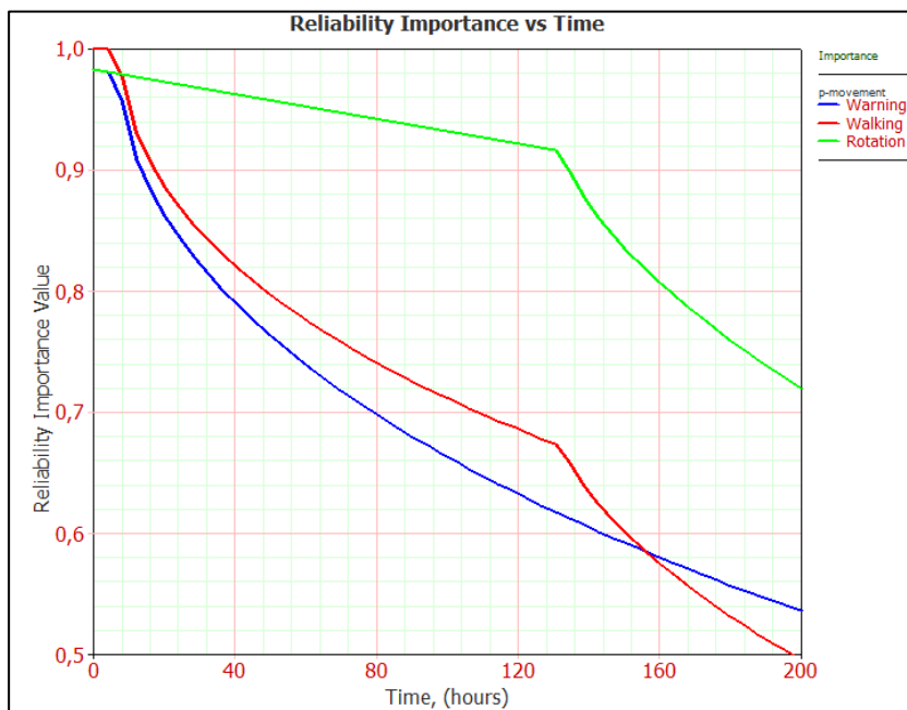
Figure A.54 Changes in importance values with time (Page-Movement)
