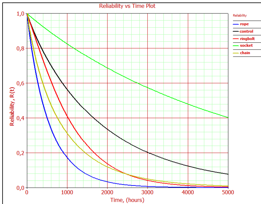
Figure A.21 Reliability curves of components (Page-Dragging)
