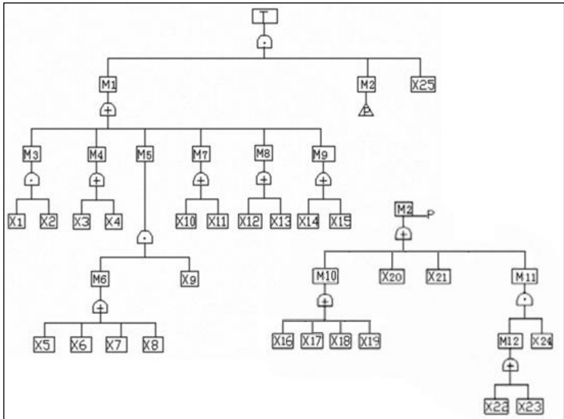
Figure 2.7 Fault tree representation of the system (Wang, 2010)
