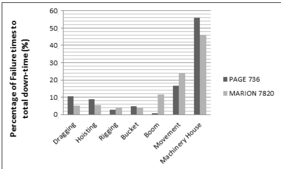
Figure 4.3 The contribution of each component to the total downtime
