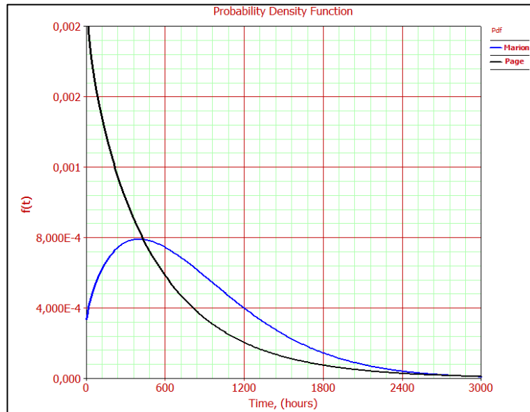
Figure A.15 PDF curves of Dragging - Rope
