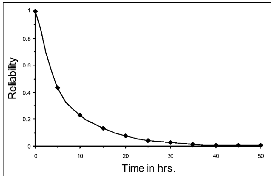
Figure 2.11 Reliability vs. Time graph of the shearer (Gupta et al. , 2006)
