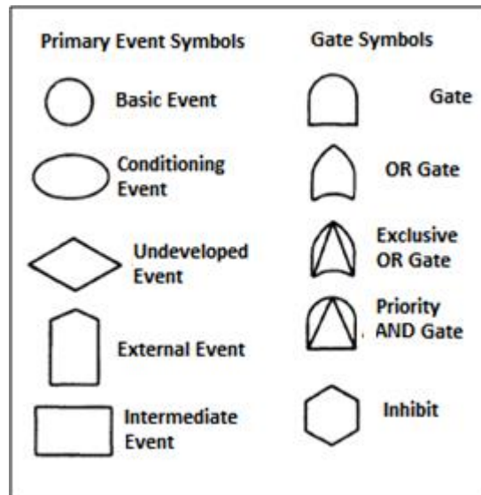
Figure 2.1 Symbols used for operators in Fault Tree Analysis (Vesely et al. , 1981)
