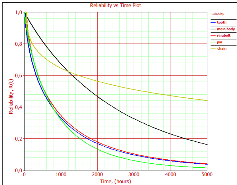
Figure A.45 Reliability curves of components (Page-Bucket)
