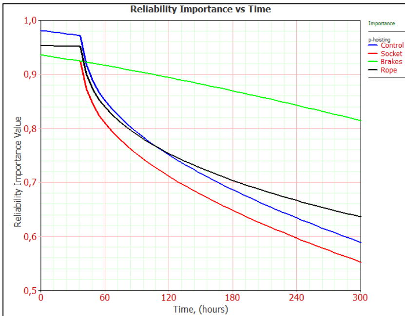
Figure A.30 Changes in importance values with time (Page-Hoisting)
