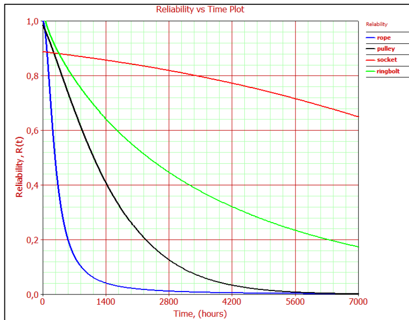
Figure A.35 Reliability curves of components (Marion-Rigging)
