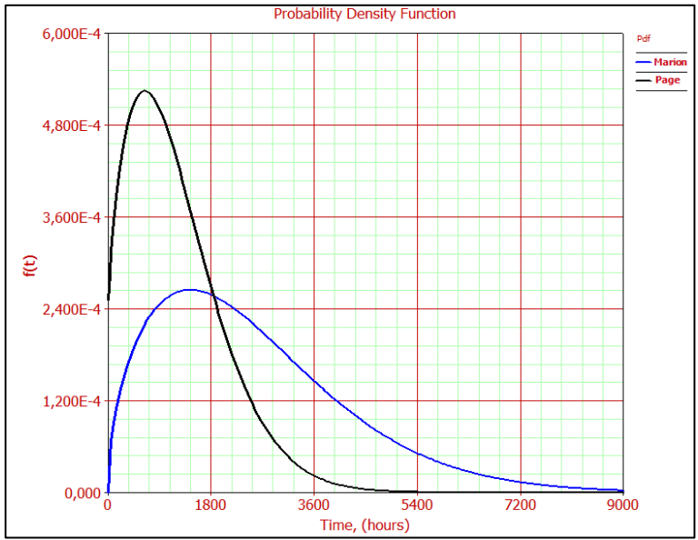
Figure A.25 PDF curves of Hoisting - Rope
