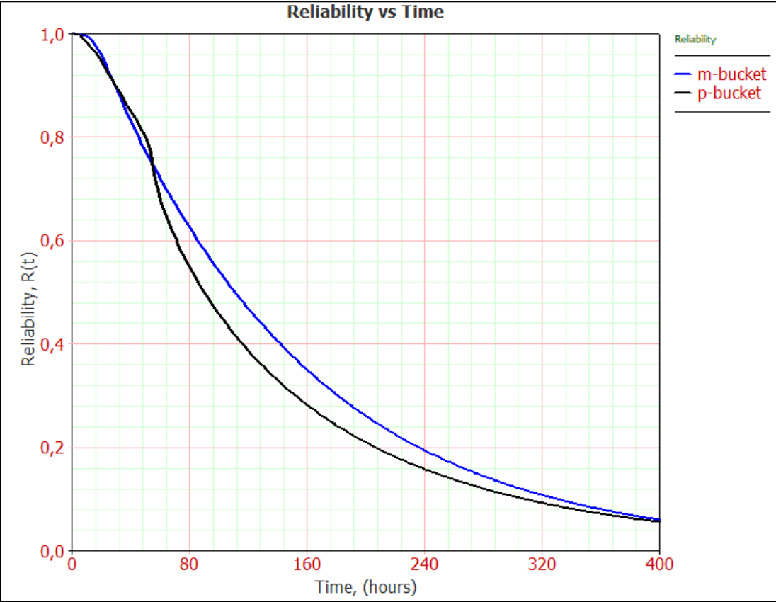
Figure 4.11 Reliability graph of bucket units
