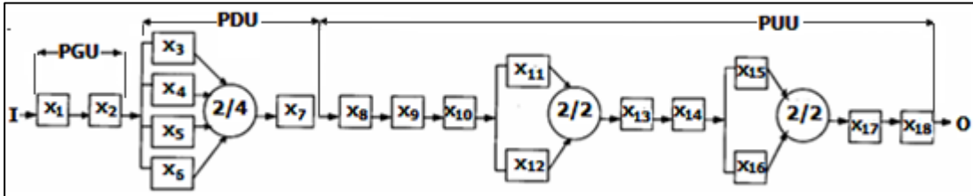
Figure 2.3 System reliability block diagram (Samanta et al. , 2002)
