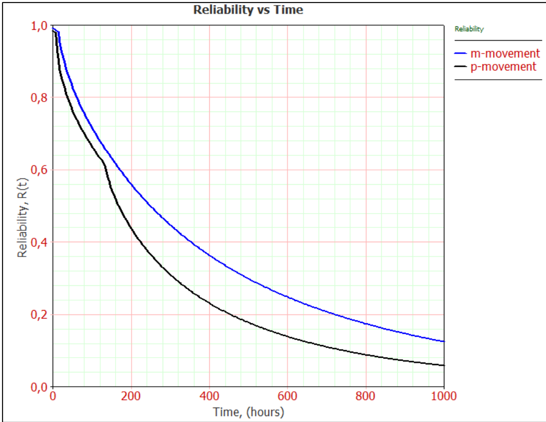
Figure 4.13 Reliability graph of movement units
