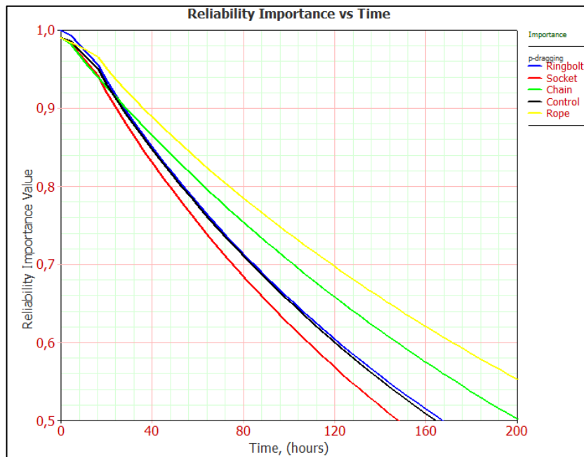
Figure A.23 Changes in importance values with time (Page-Drugging)
