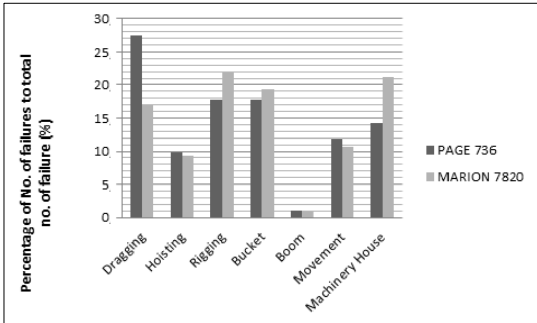
Figure 4.2 The contribution of each component to the total number of failures
