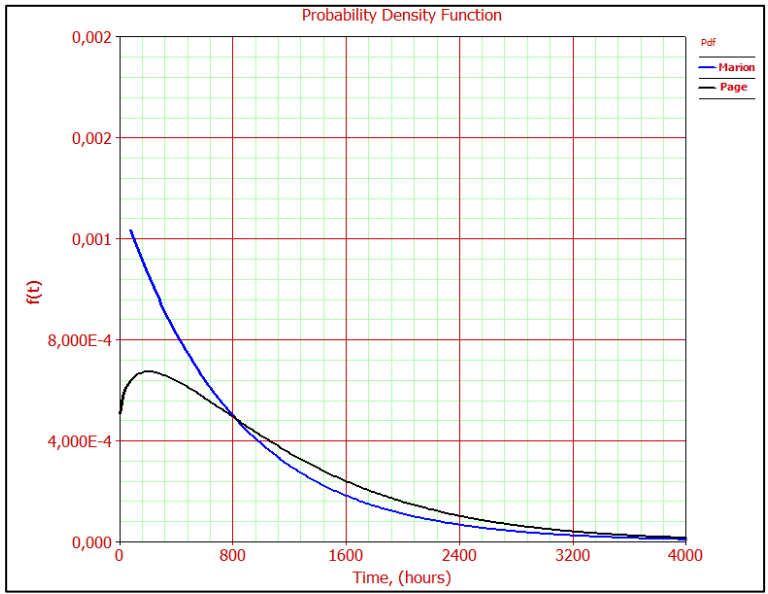
Figure A.17 PDF curves of Dragging – Ringbolt
