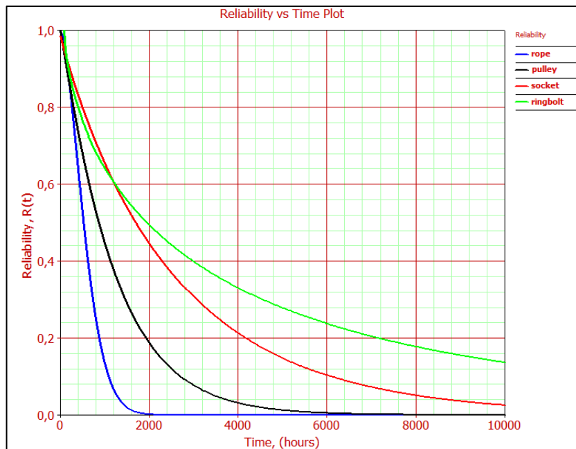
Figure A.36 Reliability curves of components (Page-Rigging)
