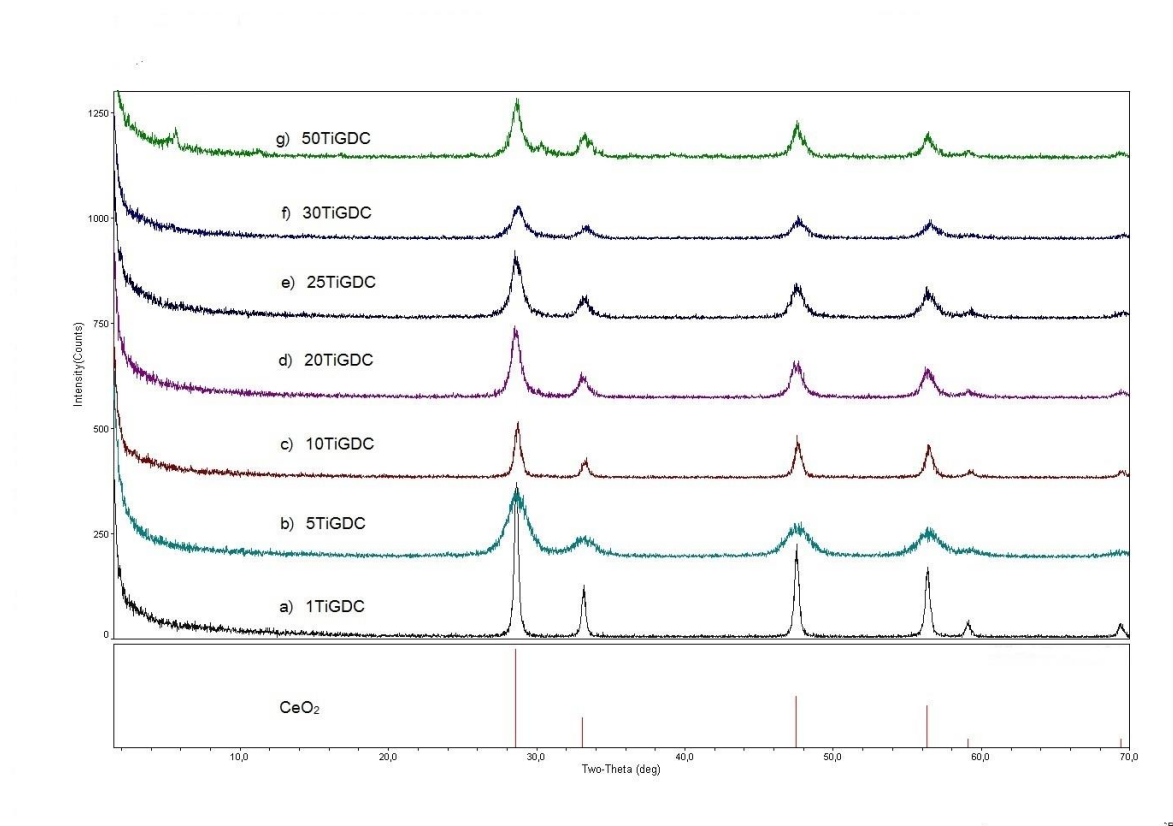
Figure 3.4. XRD results of TiGDC.
