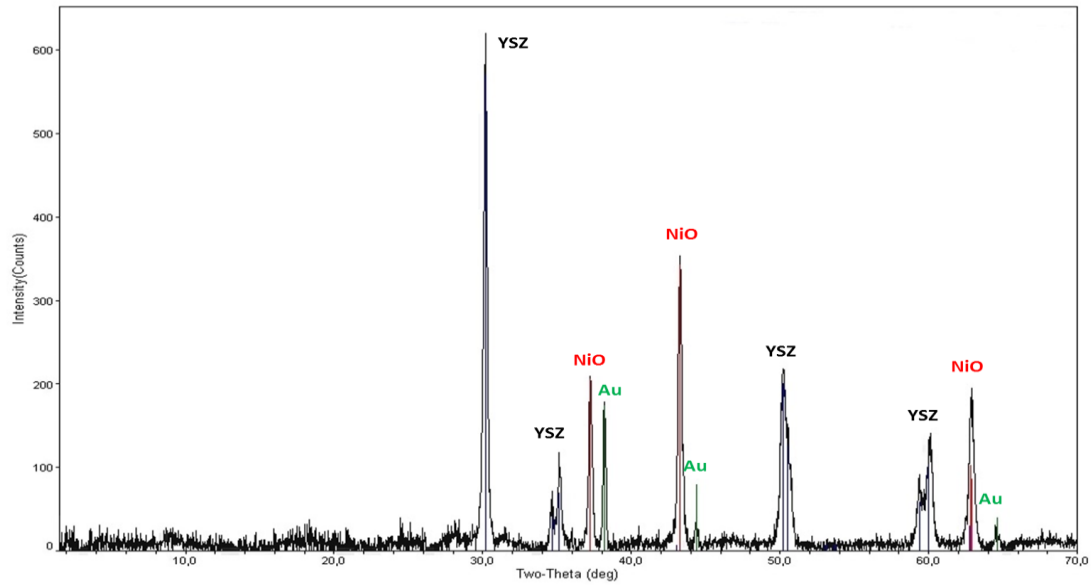
Figure 3.6. XRD results of Manganese impregnated anode cell.
