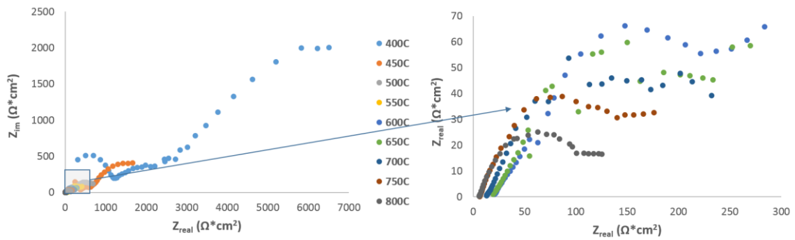
Figure 3.26. Comparison of EIS data: 1VDC fed with O2O at different temperatures between 400°C -800°C.
