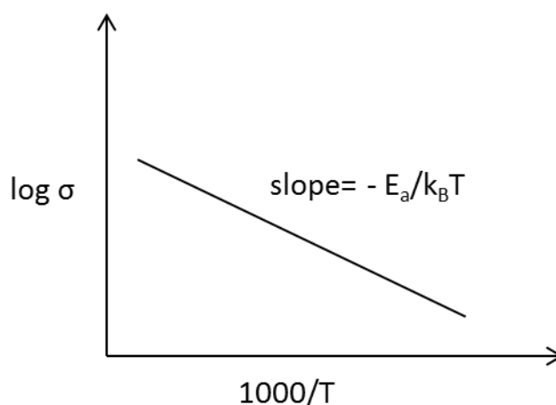
Figure 1.4. Arrhenius plot.
