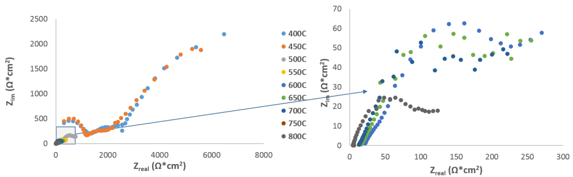
Figure 3.24. Comparison of EIS data: 1VDC fed with O3 at different temperatures between 400°C -800°C.
