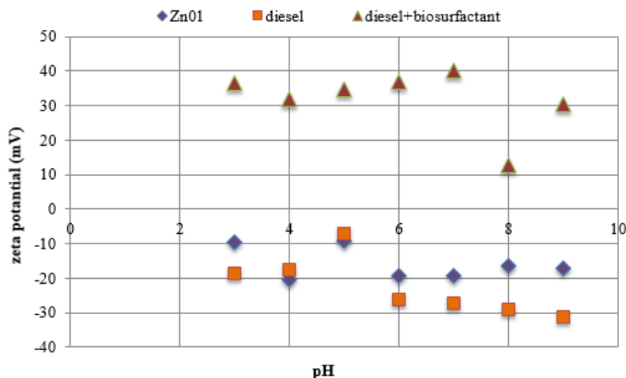
Figure 29. Zeta potential measurement for the isolate Zn01
