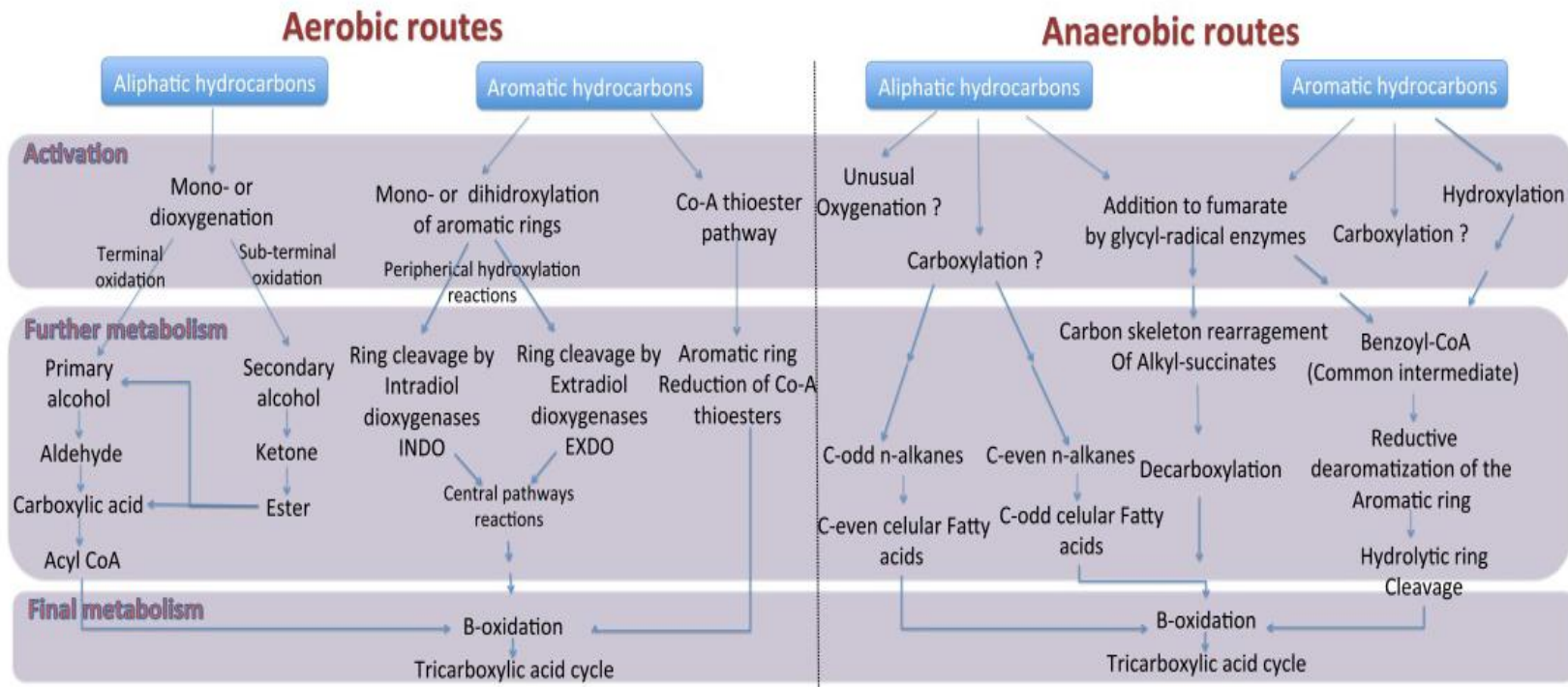
Figure 1. Aerobic and anaerobic bacterial degradation pathways of hydrocarbon compounds (Sierra-Garcia and Oliveira, 2013)
