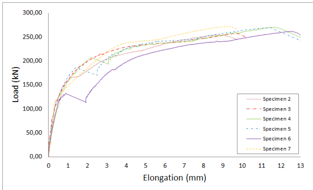
Figure 2.101. Load-displacement behavior comparison of all specimens
