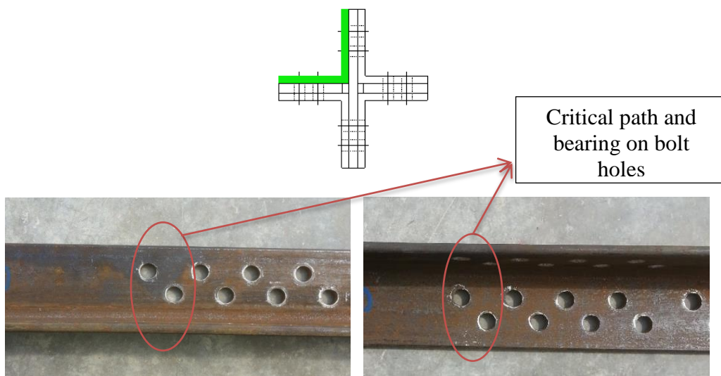
Figure 2.54. Bearing on lower main member 1 (Specimen-3)
