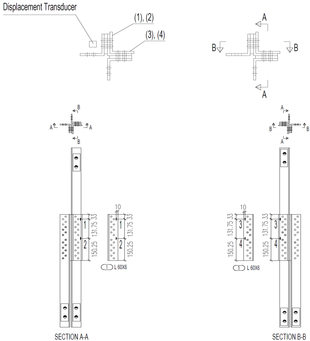
Figure 2.64. Strain gage and displacement transducer locations in side and cross-sectional view of Specimen-4 (dimensions in mm unit)
