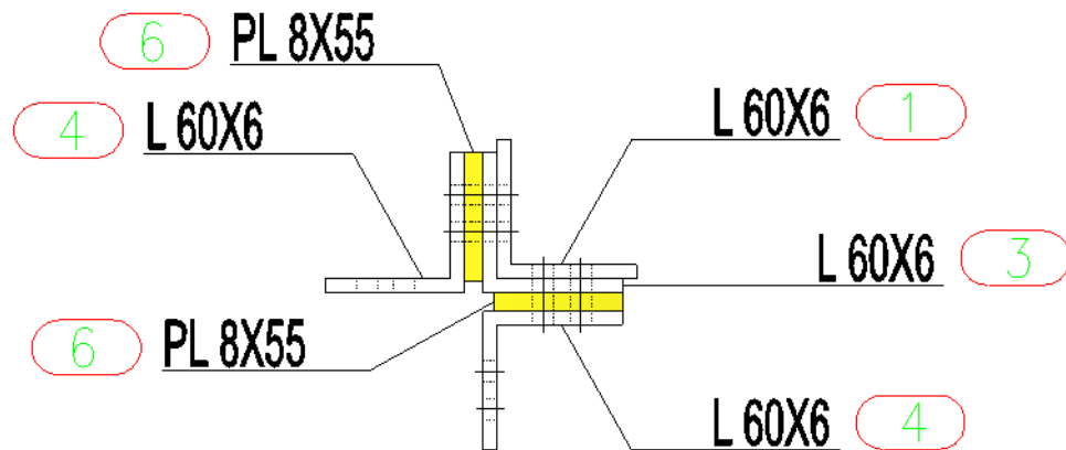
Figure 2.55. Cross-sectional view of Specimen-4
