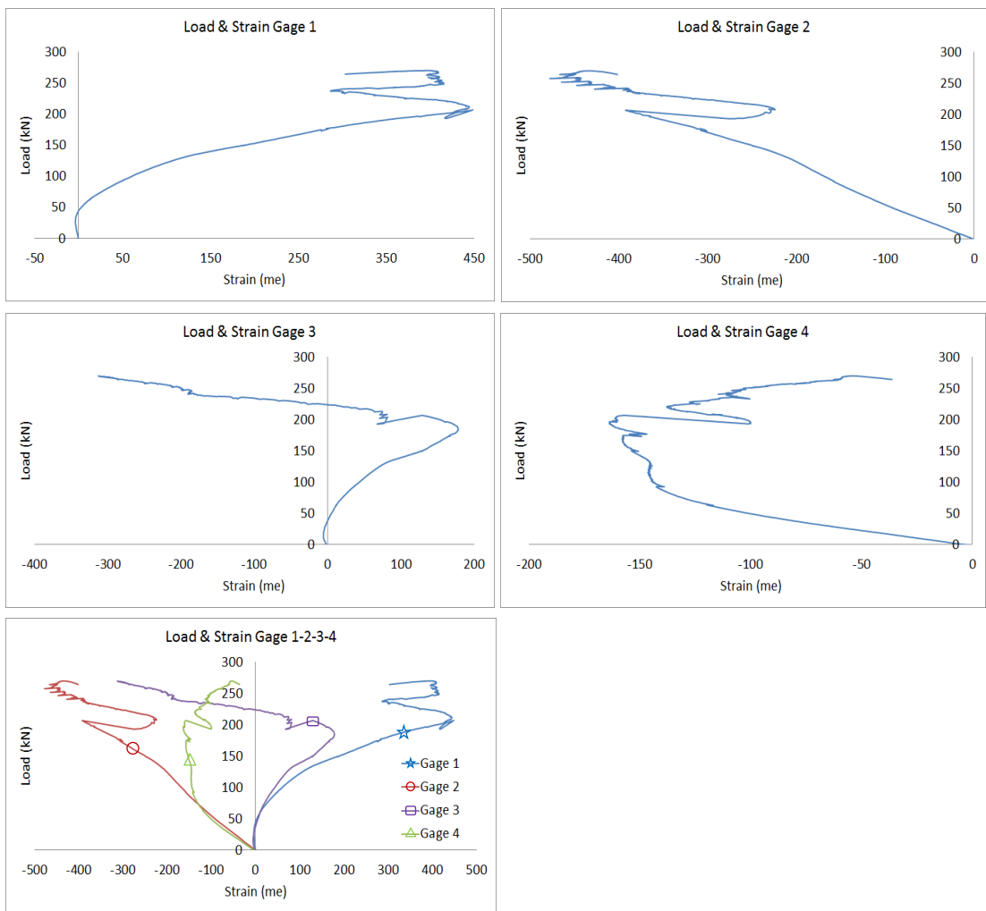
Figure 2.66. Strain distribution in interior reinforcement angle of Specimen-4
