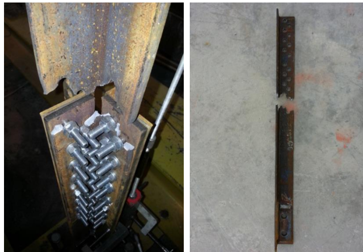
Figure 2.71. Rupture on critical path of Specimen-5
