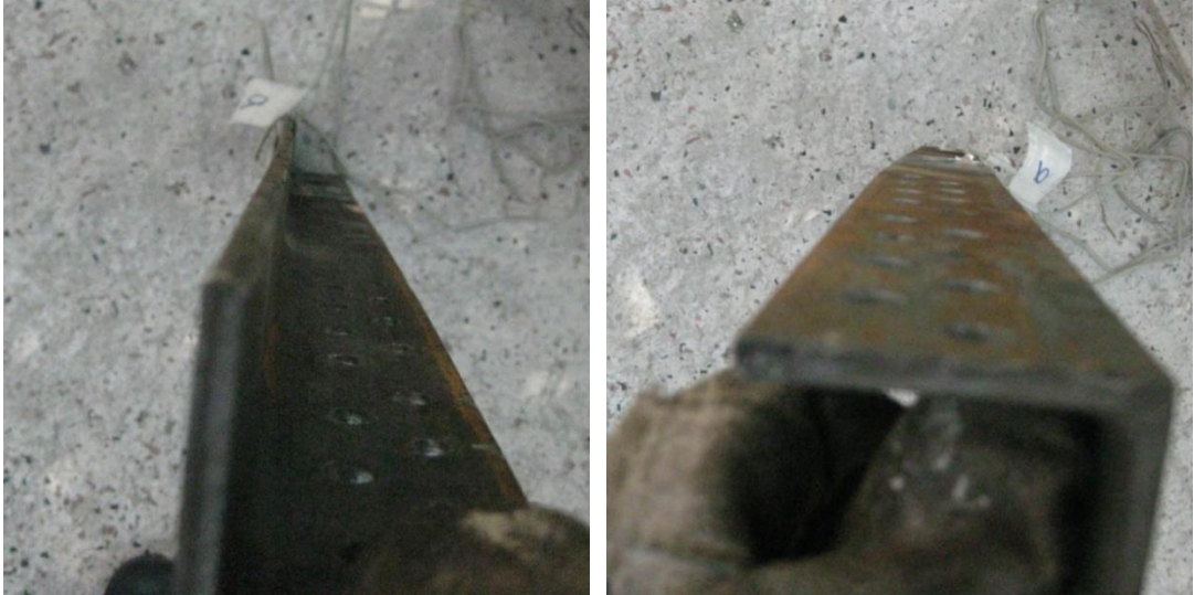
Figure 2.34. Bending on lower main member 1 (Specimen-2)
