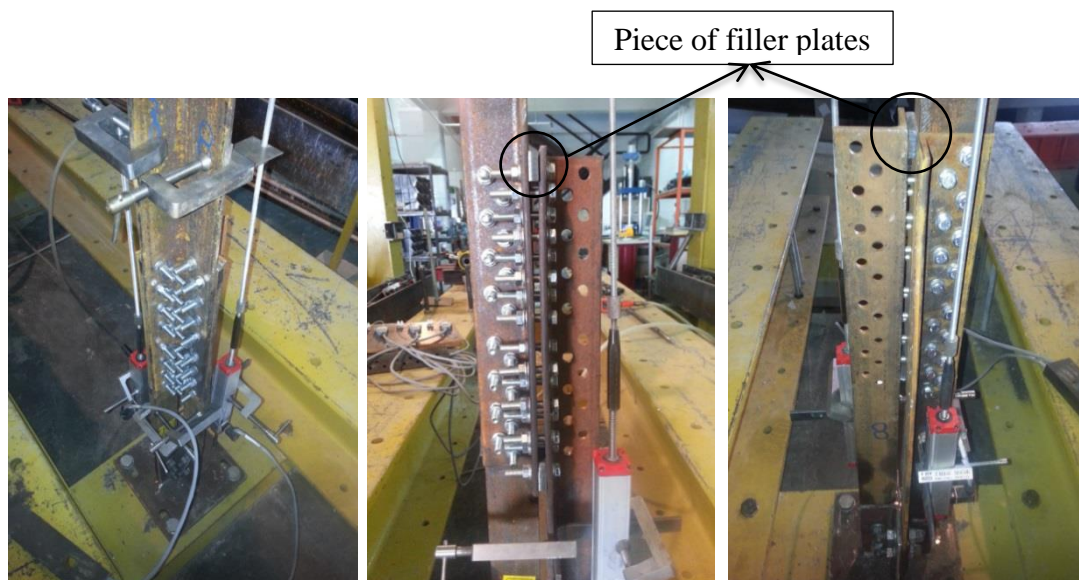
Figure 2.92. General view of Specimen-7
