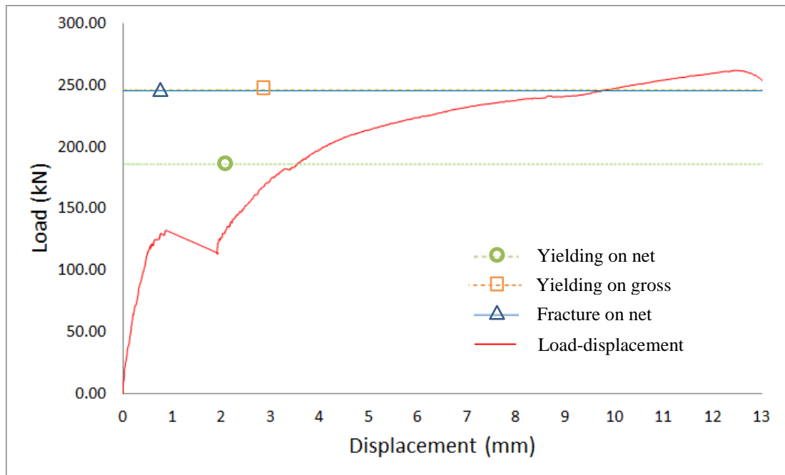
Figure 2.84. Load-displacement behavior for Specimen-6
