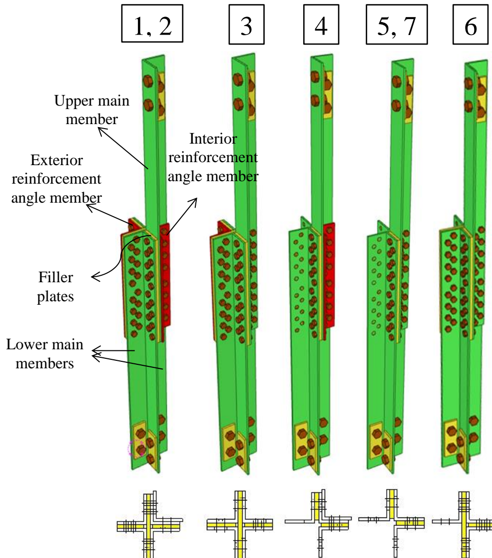
Figure 2.2. Overall geometry of test specimens
