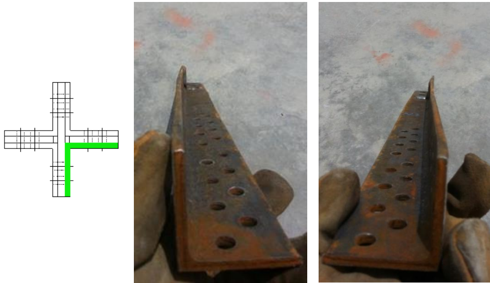
Figure 2.53. Bending on lower main member 2 (Specimen-3)
