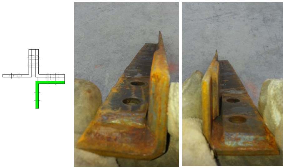
Figure 2.76. Bending on lower main member 2 (Specimen-5)
