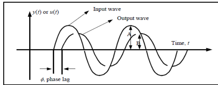
Figure 3.2. Frequency response [45].
