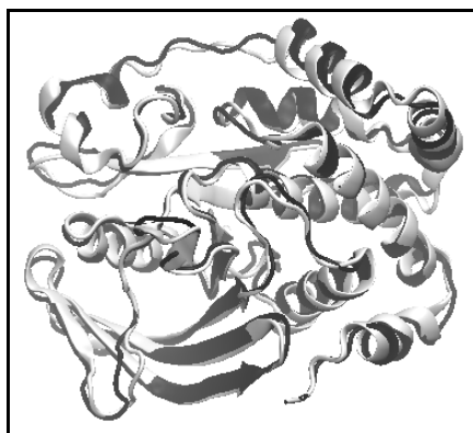
Figure 4.5. The cartoon representation of the average conformation of the MD closed simulation shown in black and the crystal structure (PDB IDs: 1SUG) shown in white.
