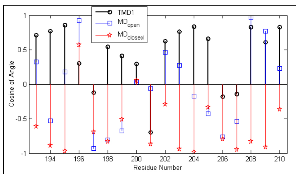
Figure 5.20. Angle cosines of S-loop between crystal structure displacements and those obtained from the first eigenvector in TMD1 (black), MD open (blue) and MD closed (red) simulations at 0.2 GHz.
