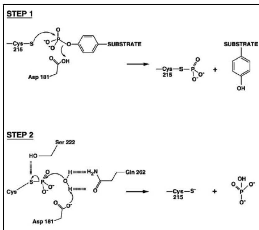
Figure 2.8. Schematic representation of the catalytic mechanism of PTP1B [9].
