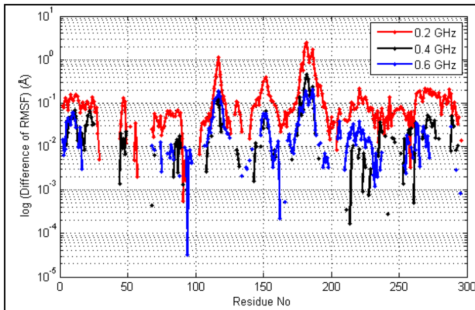
Figure B.1. Difference of RMSF values of TMD1 simulation from equilibrium MD open and MD closed at 0.2 GHz (red), at 0.4 GHz (black), at 0.6 GHz (blue) in logarithmic scale.
