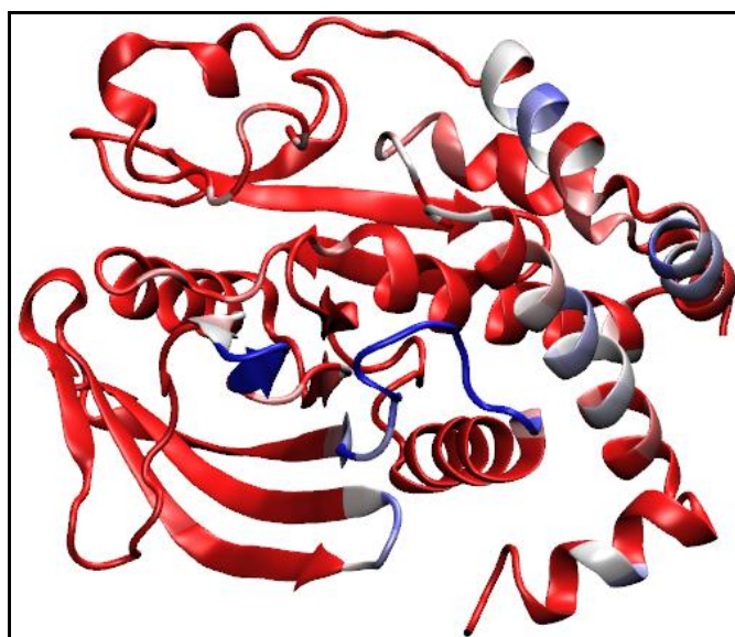
Figure 5.13. Distribution of residues with increased mobility on the three-dimensional structure of PTP1B at 0.4 GHz. Residues, which show an increase greater than 0.1 Å in RMSF is shown in blue, and those smaller than 0.01 Å in shown red, and the mapping of the increase in RMSF to blue-red coloring is logarithmic.
