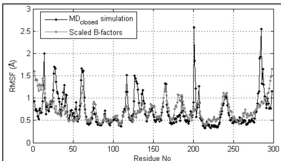
Figure 4.6. RMSF of the residues during the 40 ns MD closed simulation.
