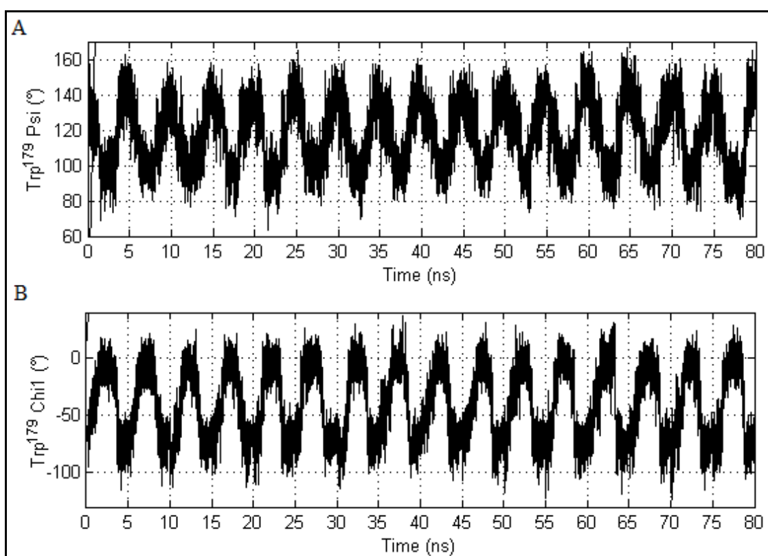
Figure 4.12. (a) Backbone \psi , and (b) sidechain \chi_1 angles of Trp179 in TMD1 simulation.
