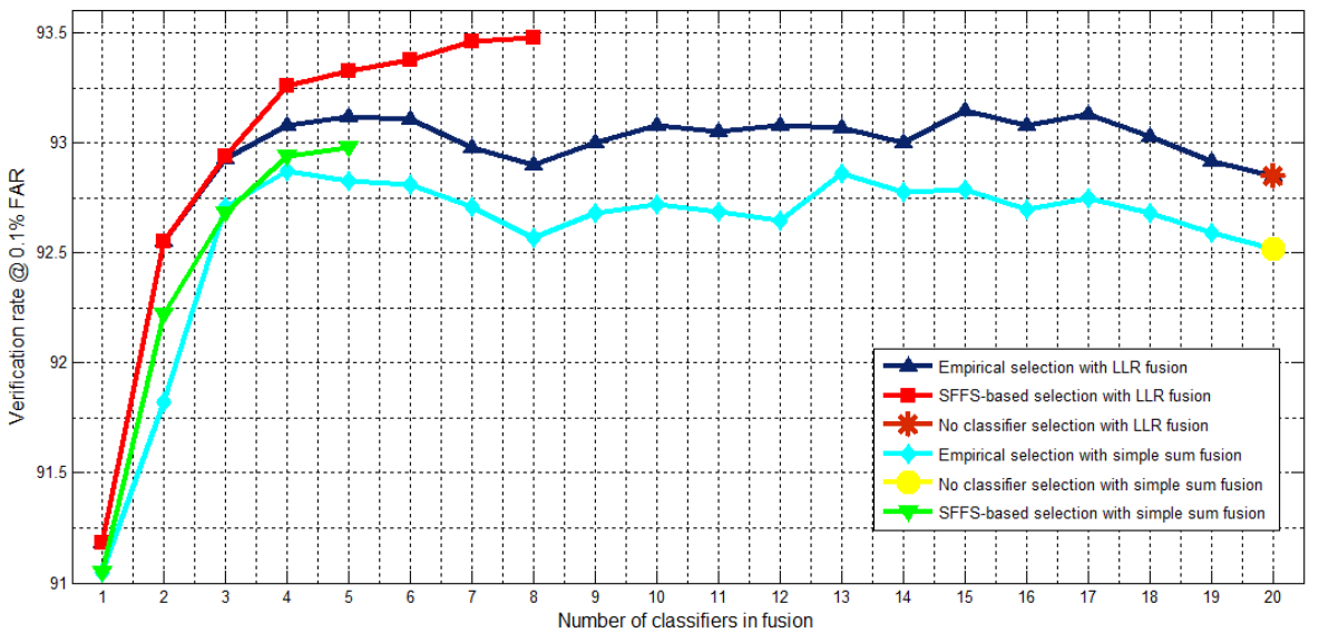
Figure 4.6. Comparison of different classifier selection and fusion methods with changing number of selected classifiers for the fusion.
