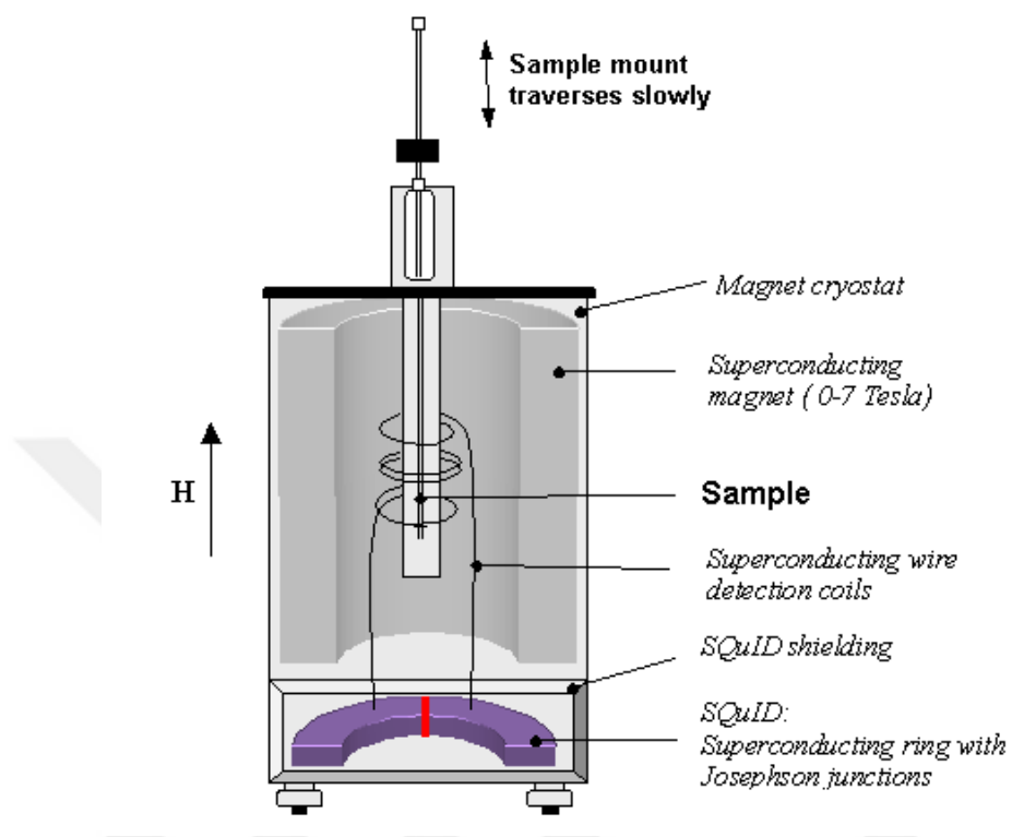
Figure 4.3. Schematic diagram of a SQUID magnetometer
