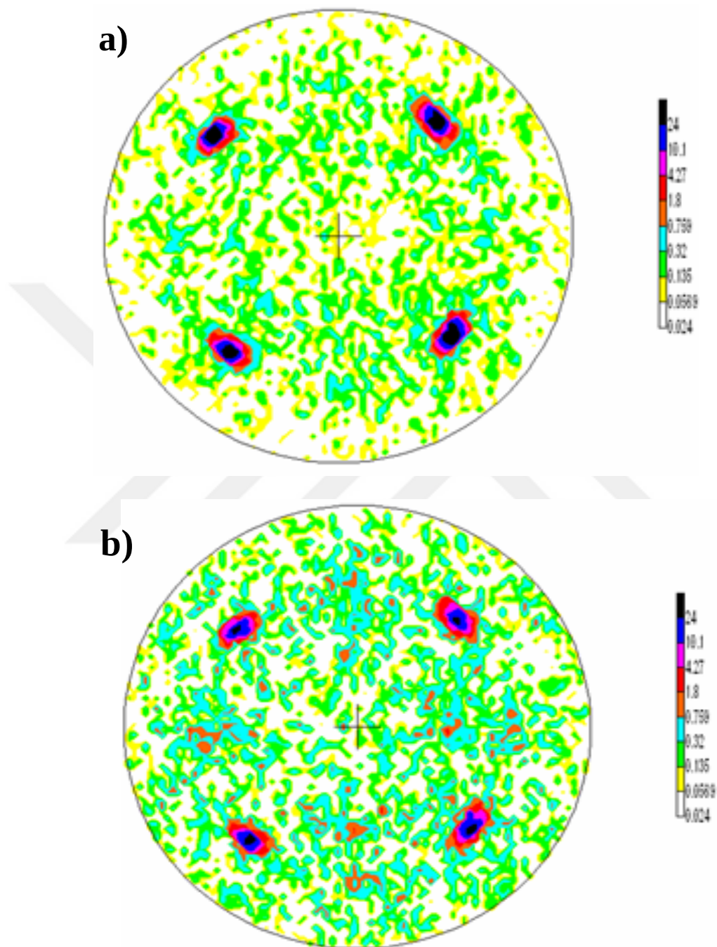
Figure 6.16: The background subtracted logarithmic scale (111) pole figures of LMO:MgO composite films fabricated on IBAD-MgO templates. Films modified with MgO volume percentages of a) 5% and b) 50%.
