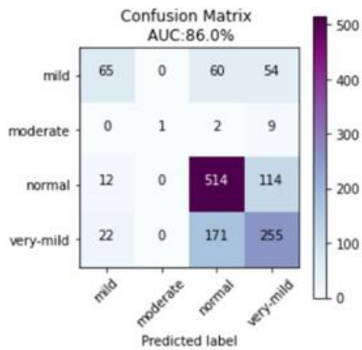
Figure 4.9: InceptionV3 + Additional Capacity
