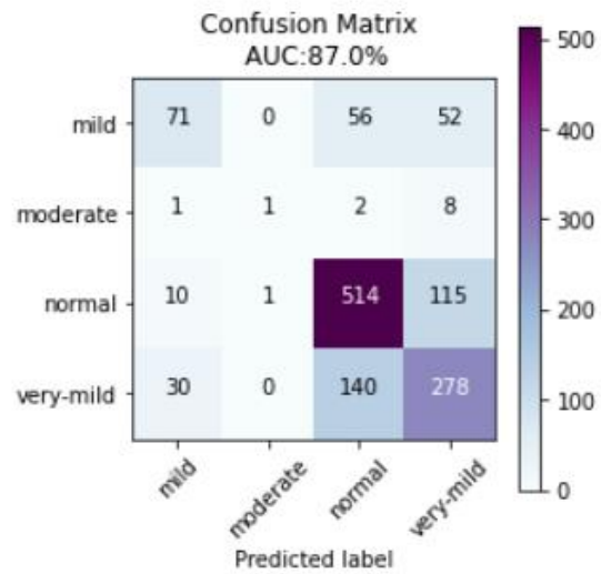
Figure 4.10: InceptionV3 + Additional Capacity + Data Augmentation
