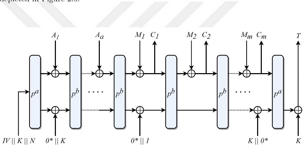
Figure 2.5. Ascon Encryption.
