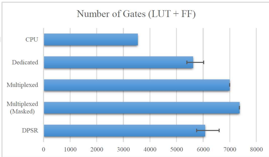
Figure 5.4. Resource utilization comparison between DA, MUX, and DPSR implementations.
