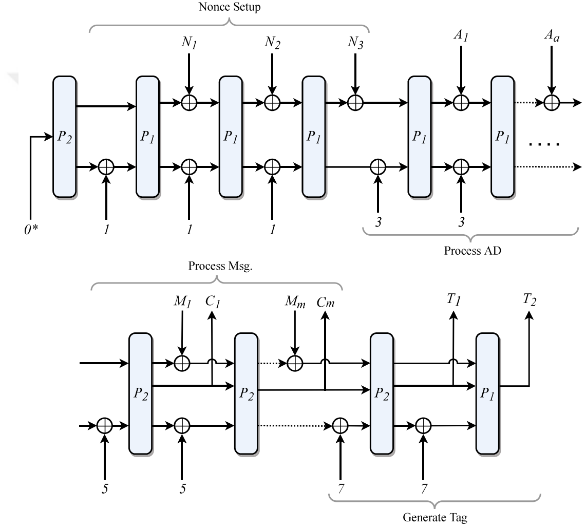
Figure 2.6. TinyJAMBU AEAD Mode of Operation.
