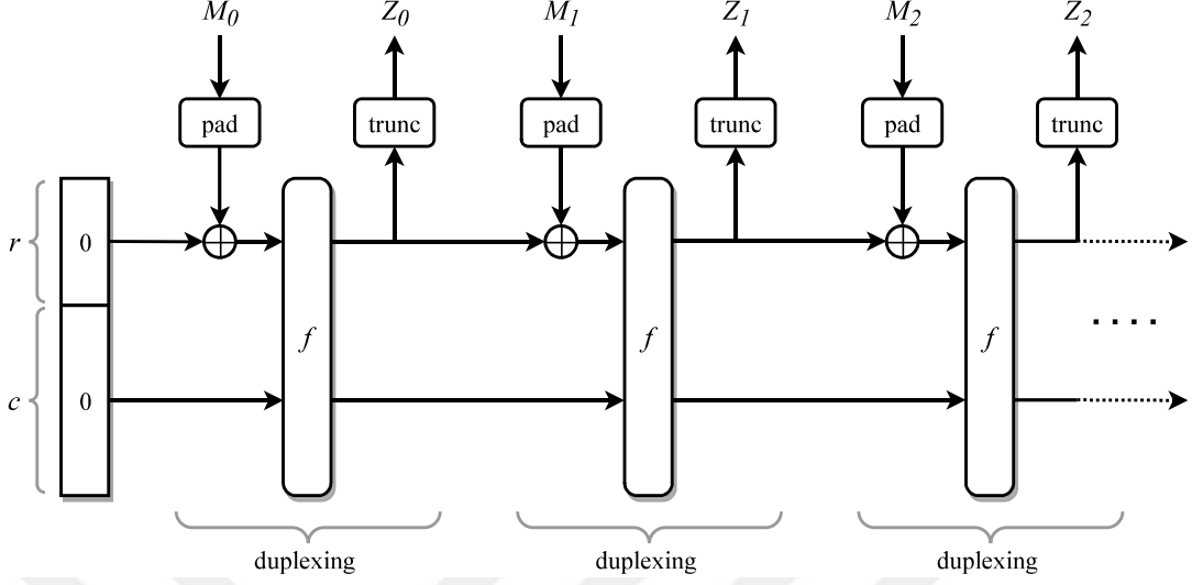
Figure 2.4. Duplex Construction.
