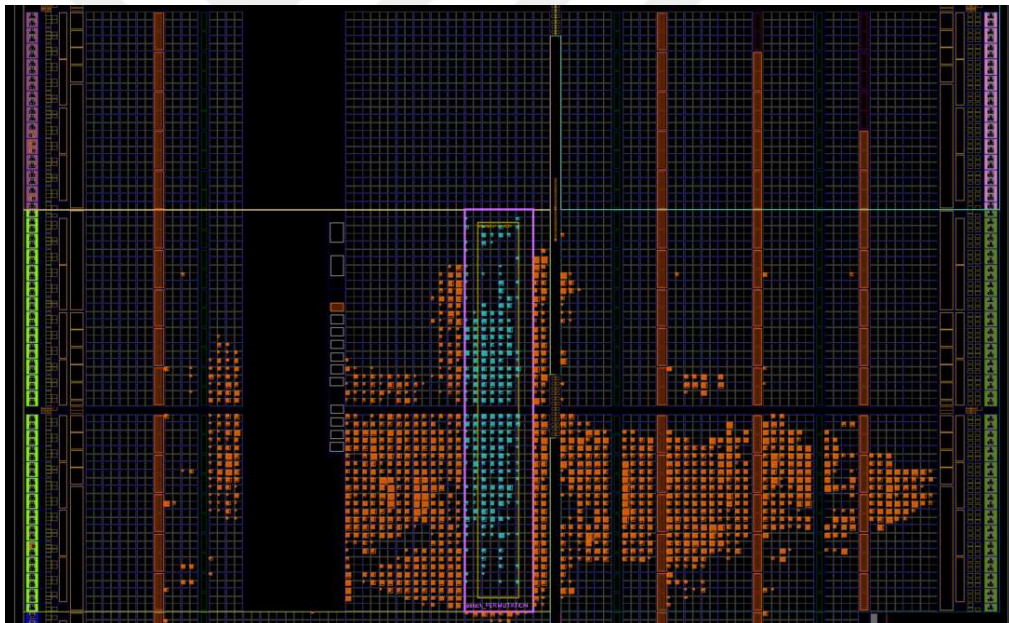
Figure 4.2. Post-Implementation FPGA Layout.
