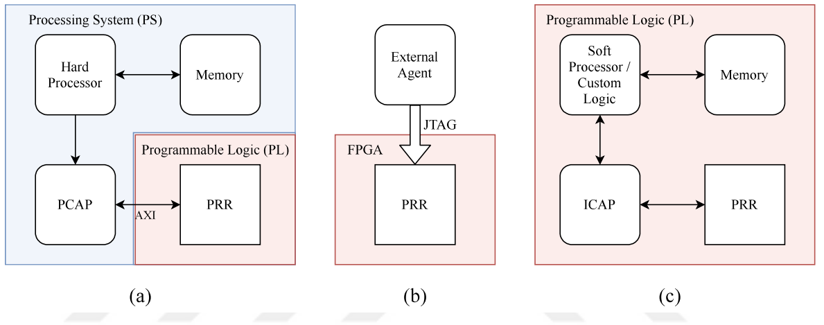
Figure 2.11. Partial Reconfiguration Using (a) PCAP, (b) External Agent, (c) ICAP.
