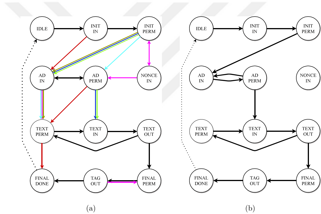
Figure 3.2. FSM Transitions for (a) Seven NIST LWC Algorithms, (b) Ascon.
