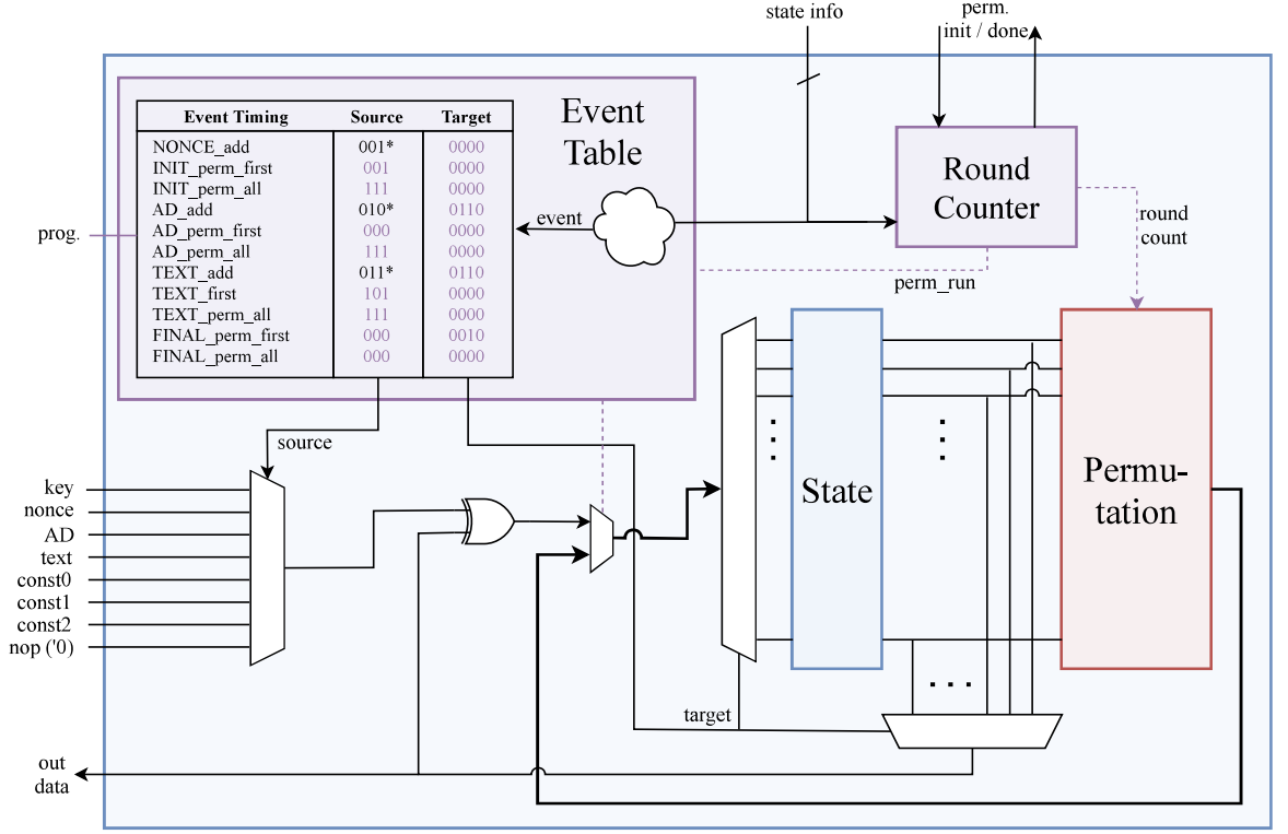
Figure 3.4. Cipher Module Block Diagram.
