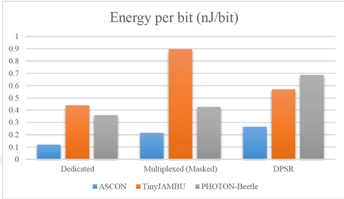
Figure 5.3. Energy efficiency comparison between DA, MUX, and DPSR implementations.
