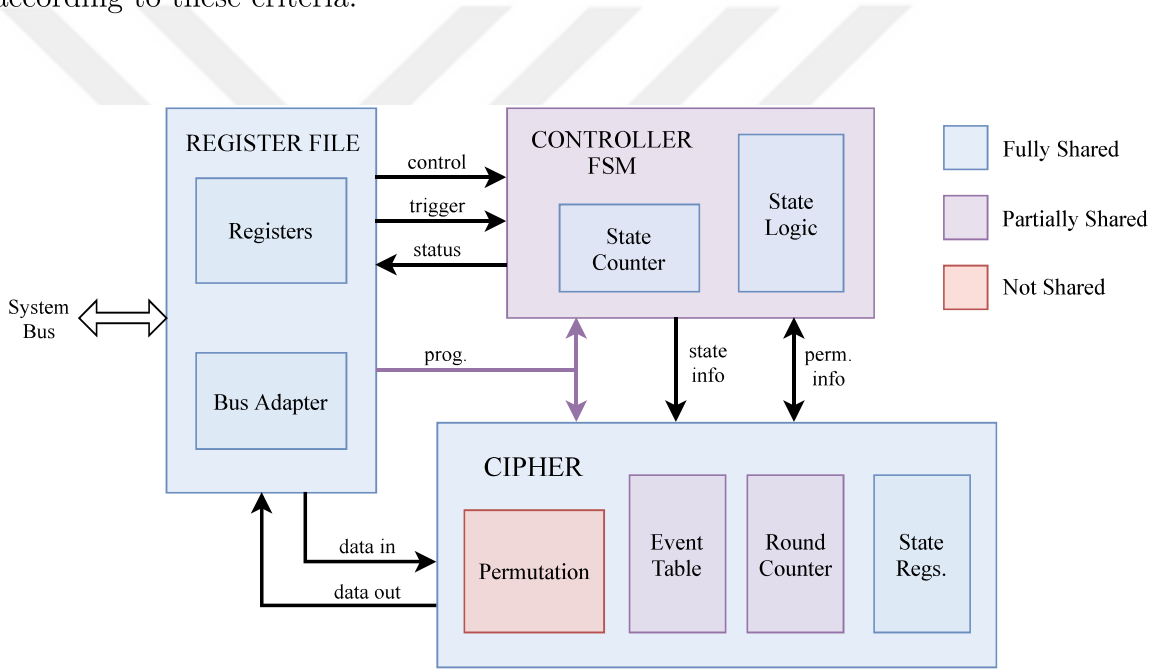
Figure 3.1. Top-Level Block Diagram of the Accelerator.
