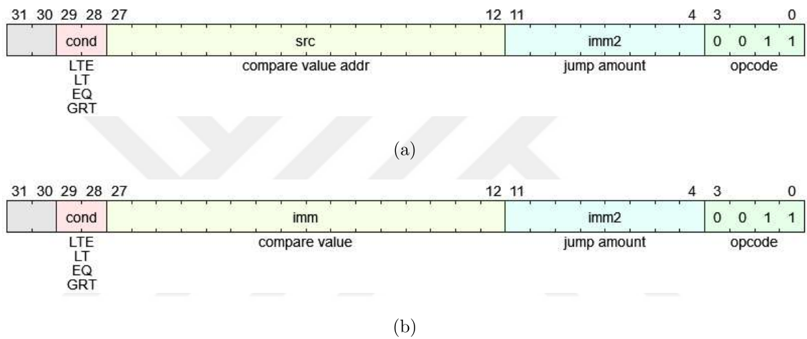
Figure 3.10. (a) Branch (BRN). (b) Branch-Immediate (BRNI).
