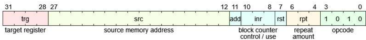
Figure 3.7. Write Load Value (WRT) Instruction.
