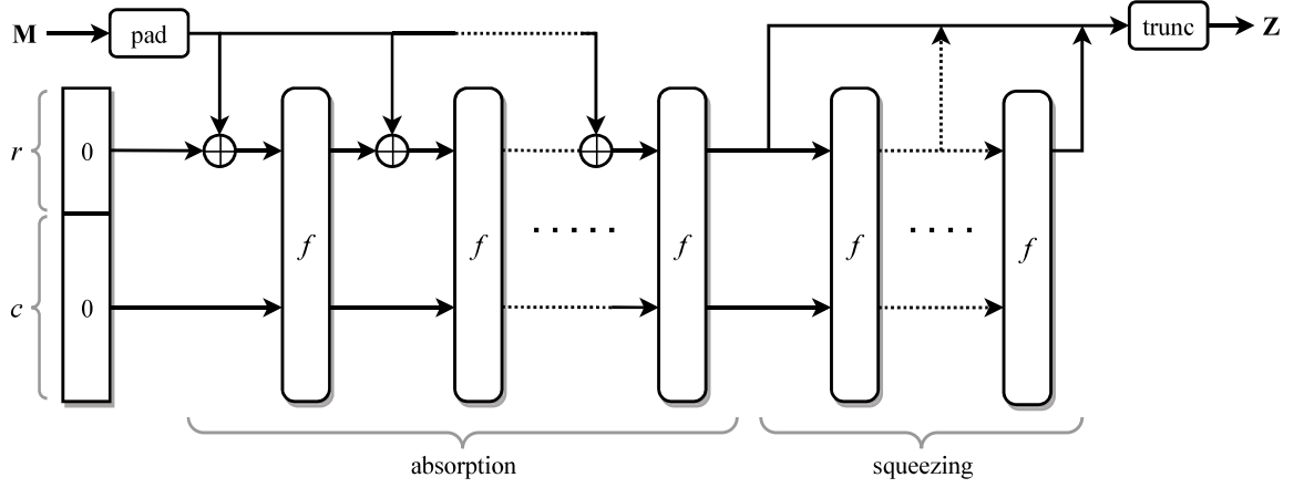
Figure 2.3. Generic Sponge Function.
