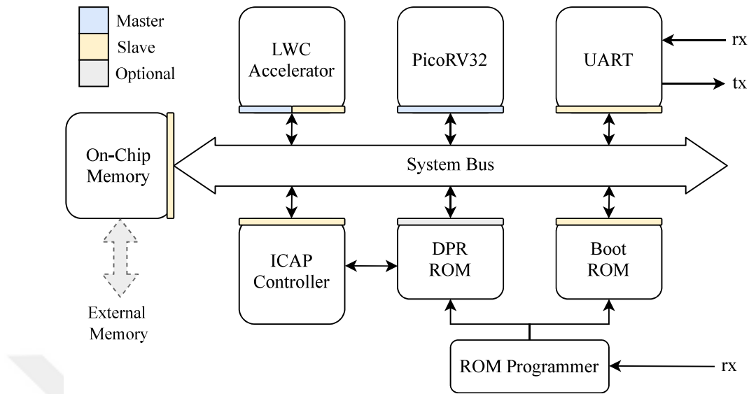
Figure 3.13. Top Level Connections.
