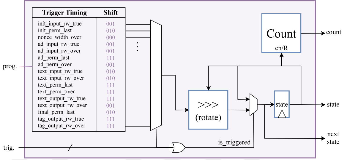
Figure 3.3. Controller Block Diagram.
