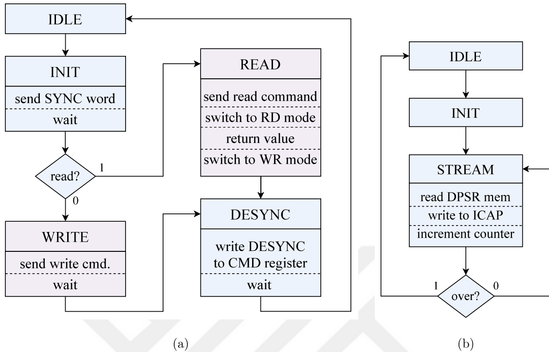
Figure 3.14. ICAP Controller Diagram (a) Single Mode, (b) Stream Mode.
