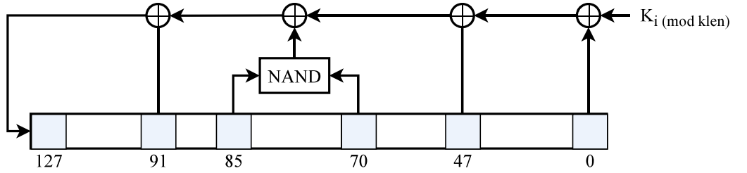
Figure 2.7. The NLFSR Used in TinyJAMBU’s 128-bit Permutation.
