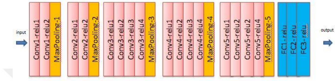
Figure 3.2. Architecture of the Pre-Trained VGG19 model
