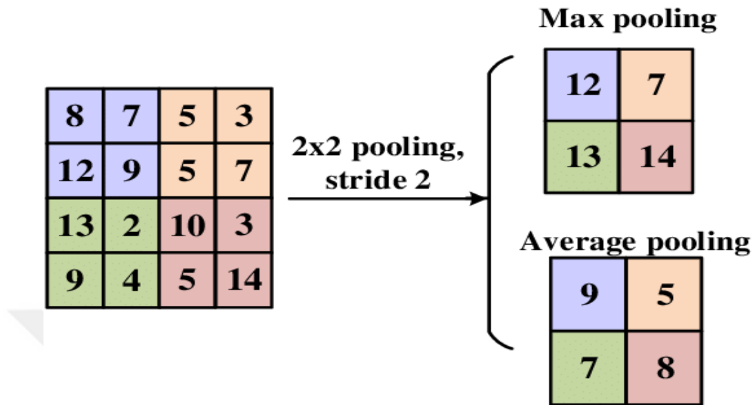
Figure 2.5 Pooling operations [59]
