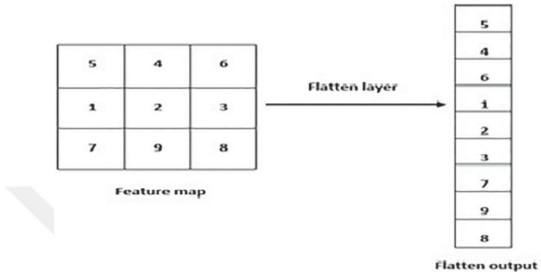
Figure 2.7 Flatten Operation [61]
