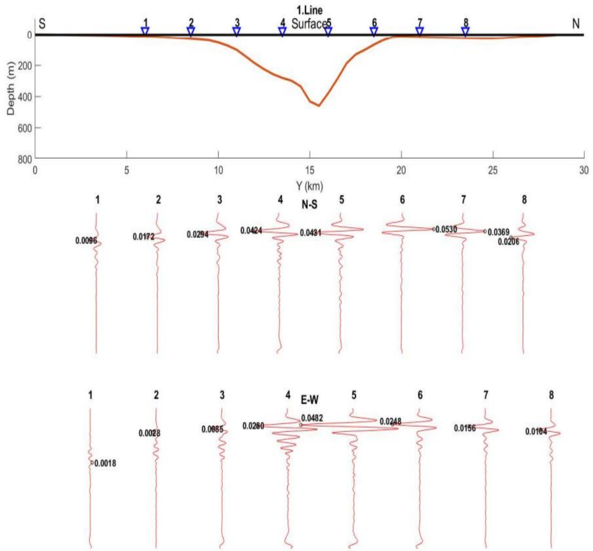
Figure 5.37. The generated velocity time histories of 18.09.2015 Mw 3.7 using Mindavelli model with basin bandpass filtered at 0.3-1 Hz (unit of cm/s).
