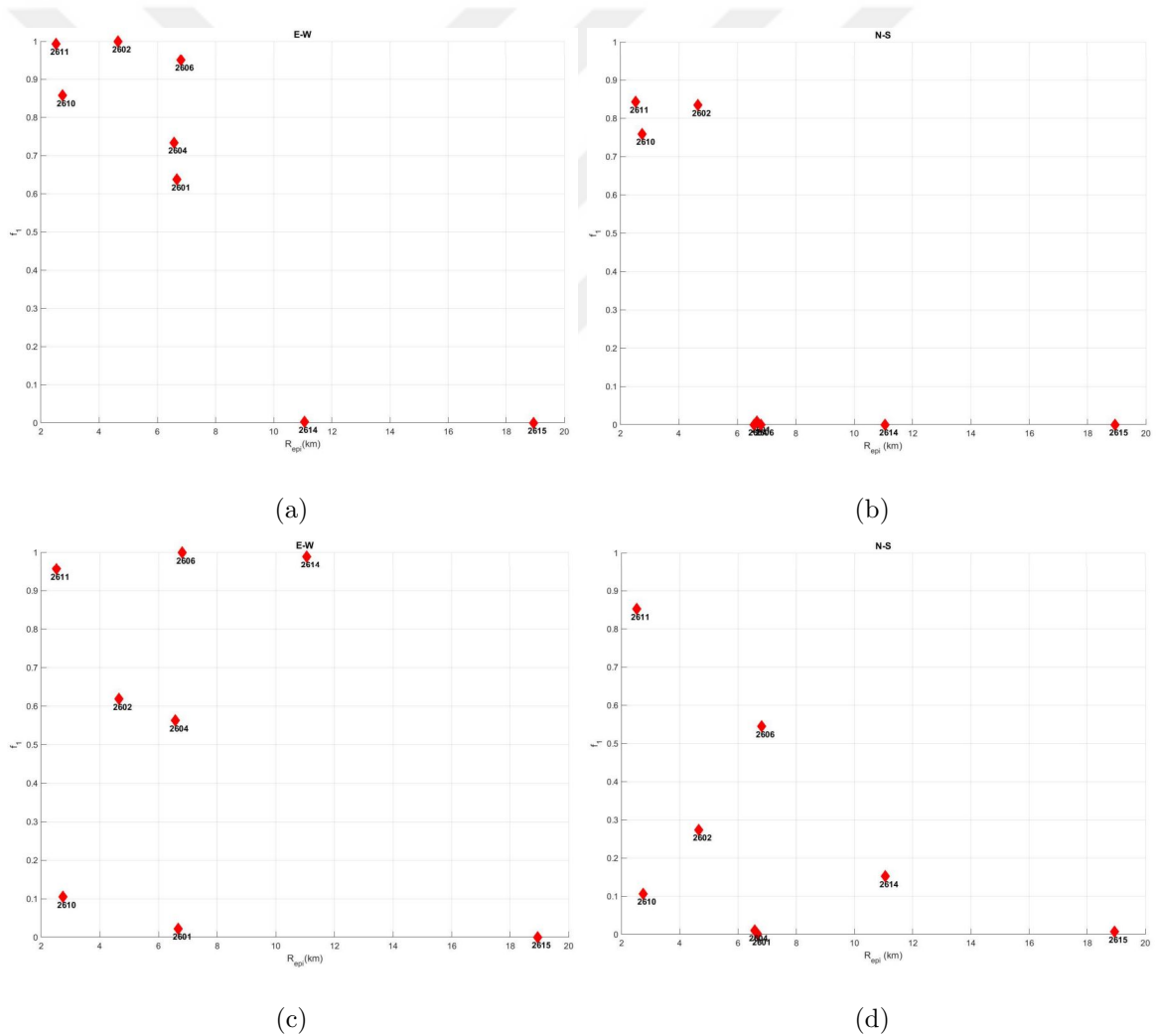
Figure 5.14. f_1 factor for 17.01.2015 Mw 3.7 using velocity model with basin (a) and (b), without basin (c) and (d) at frequency ranges of 0.3 and 1 Hz.
