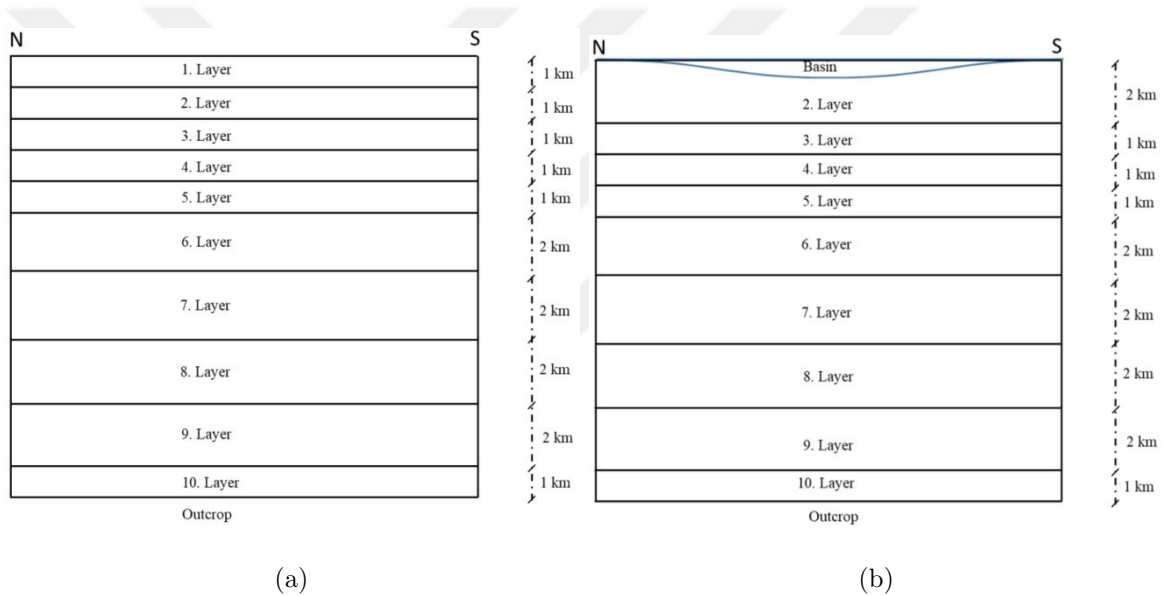
Figure 3.16. Illustration of velocity structure model for Eskişehir used in simulation.
