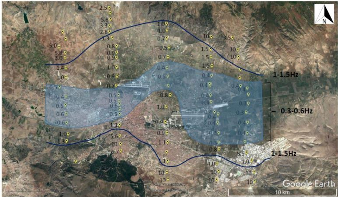
Figure 3.7. The distribution of resonance frequency on the Eskişehir basin. Shaded field indicate the frequency range of 0.3 to 0.6 Hz. The Blue line display the frequency range of 1 to 1.5 Hz (obtained from TUBITAK Project-116Y524).
