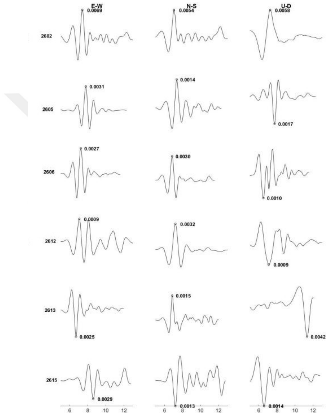
Figure 4.23. Velocity time series of the 24.07.2020 Mw 4.1 Earthquake bandpass filtered at 0.3-1 Hz.
