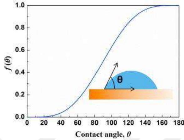
Figure 2.32 Variation of the contact angle and geometric factor [145].
