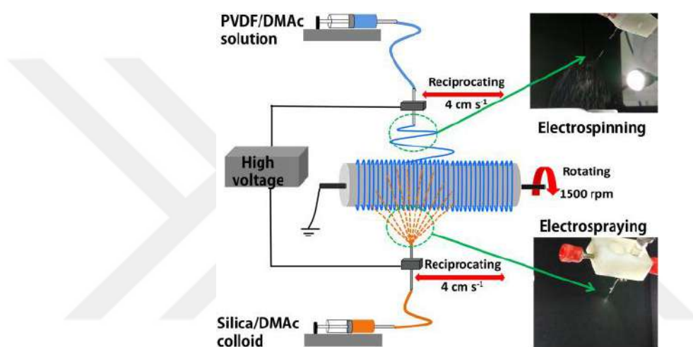
Figure 2. 28 Schematic representation of simultaneous electrospinning-electrospraying process [127].
