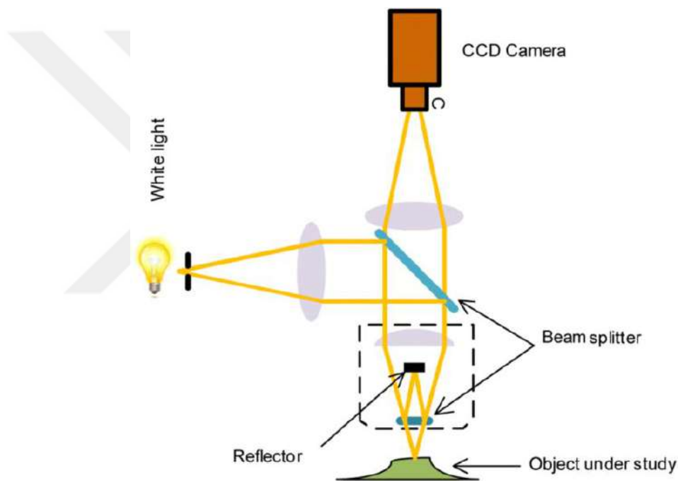
Figure 3. 12 Working principle of a 3D profilometer [167].
