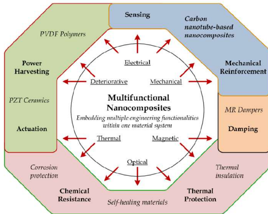
Figure 1. 3 The concept of multifunctional nanocomposites, the properties imparted, and applications areas [11].
