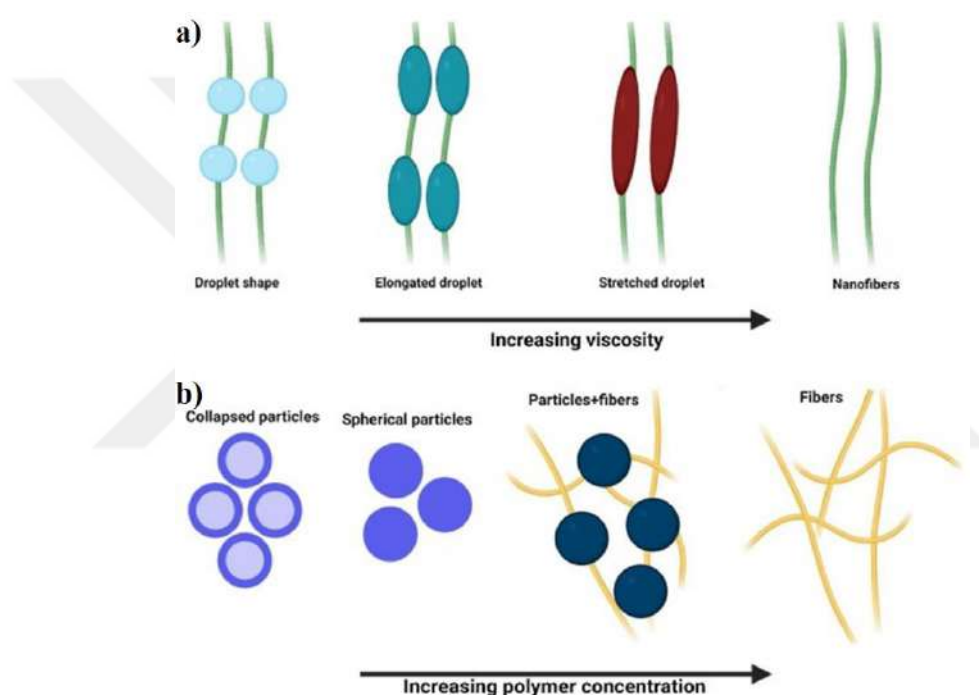
Figure 4. 13 The effect of (a) increasing viscosity and (b) increasing polymer concentration on bead formation [192].
