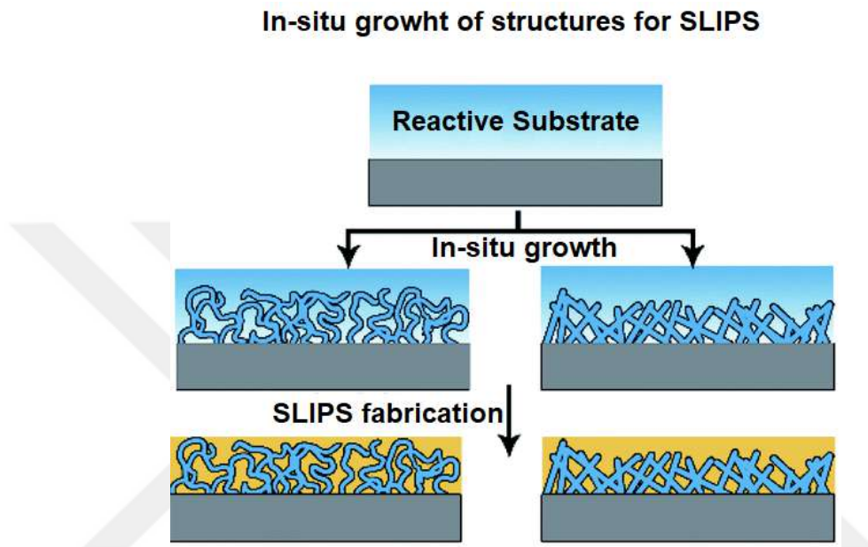
Figure 2. 35 In-situ growth fabrication techniques used for SLIPS [151].
