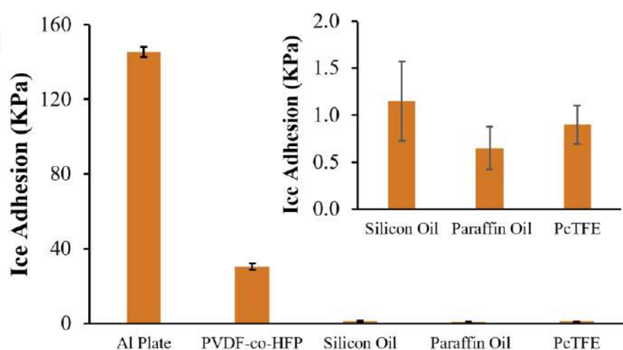
Figure 5.8 Ice adhesion strengths of samples (Inset: ice adhesion test result of SLIPS with silicone oil, paraffin oil, and PctFE, respectively).
