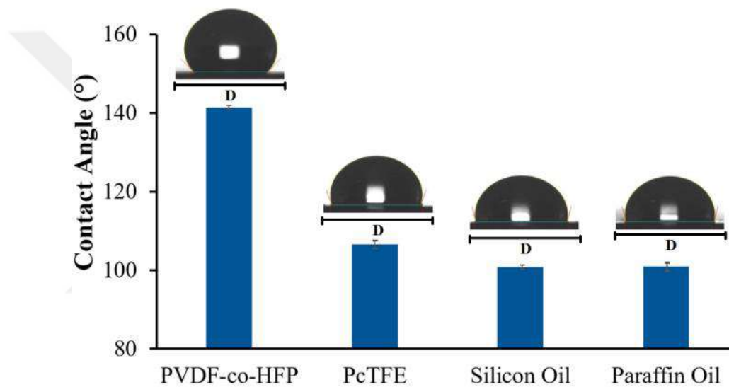
Figure 5.5 Static contact angles results of the as-produced membrane and SLIPS ( D=3.0 mm).
