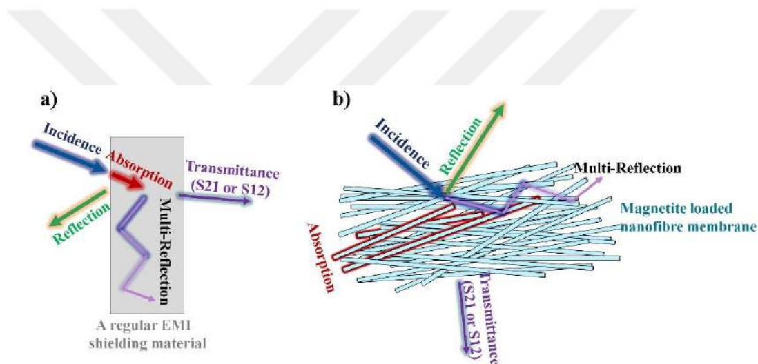
Figure 6. 13 The schematic representation of the EMI shielding mechanism on (a) bulky materials and (b) electrospun membranes.
