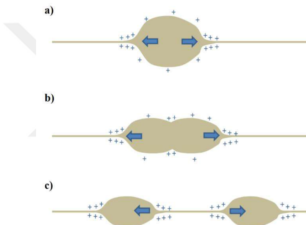
Figure 4. 12 Schematic representation of the formation of beads during electrospinning process (a) repulsive force at both ends of the bead, (b) splitting apart of the bead and the increasing charge density at the centre (c) moving further apart of the beads because of the charge concentration at the ends.
