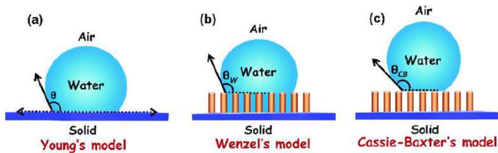
Figure 2.15 Schematic illustration of Young's (a), Wenzel (b) and Cassie-Baxter (c) Models [75].
