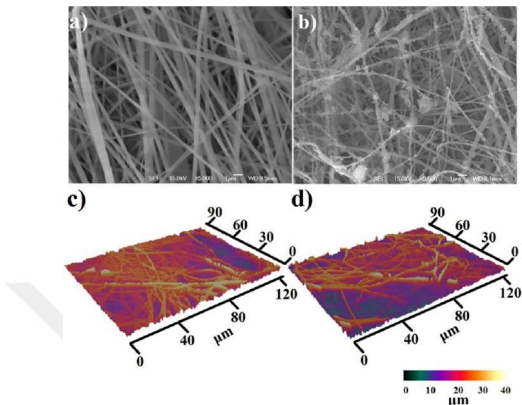
Figure 6. 4 SEM and 3D topographical images of (a and c) r-PET/magnetite nanocomposite fibre membrane and (b and d) FSFS treated r-PET/magnetite nanocomposite fibre membrane.
