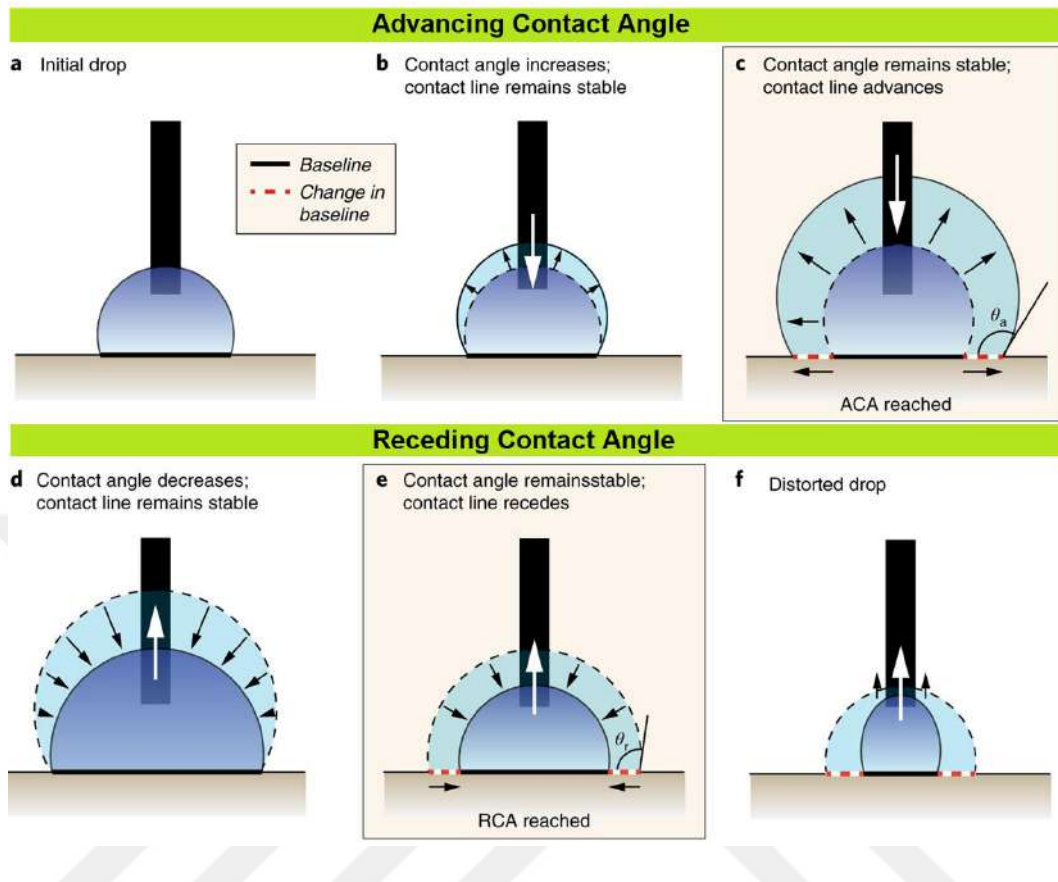
Figure 2. 16 Measurement of Advancing(a-c) and receding (d-f) contact angles and their different stages [76].
