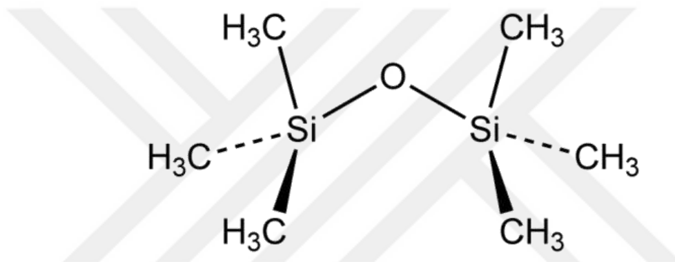
Figure 2. 17 Chemical structure of PDMS [98].
