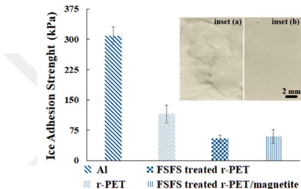
Figure 6. 8 Ice adhesion strength values of the aluminium reference versus r-PET, FSFS treated r-PET and FSFS treated r-PET/magnetite electrospun membranes (Surface appearance after ice adhesion test for (inset: a) untreated and (inset: b) FSFS treated samples).
