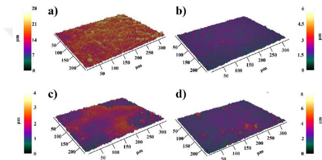
Figure 5.4 3D topographic images of (a) PVDF-co-HFP electrospun membrane (b) SLIPS with PctFE, (c) SLIPS with silicone oil, and (d) SLIPS with liquid paraffin.
