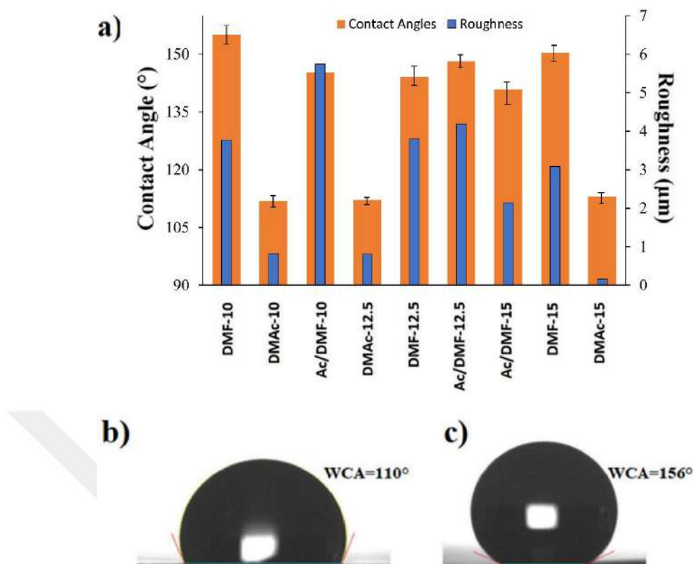
Figure 4. 3 Contact angle and roughness comparison of the produced samples (a), contact angles of DMac-15 (b) and DMF-10 (c).
