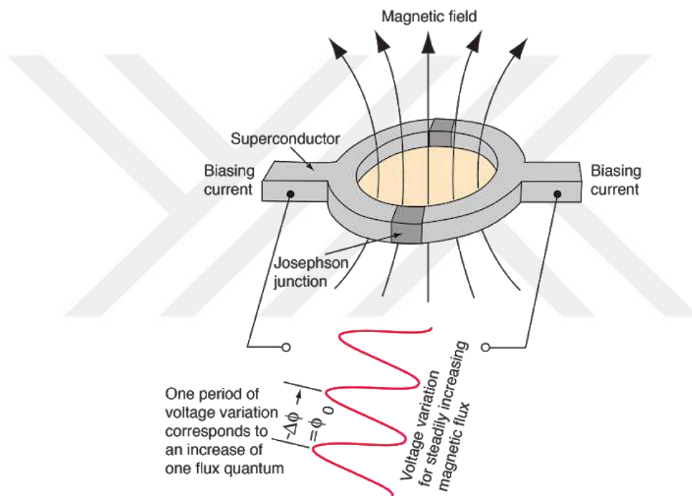
Figure 3. 16 Working principle of SQUID magnetometer [172].
