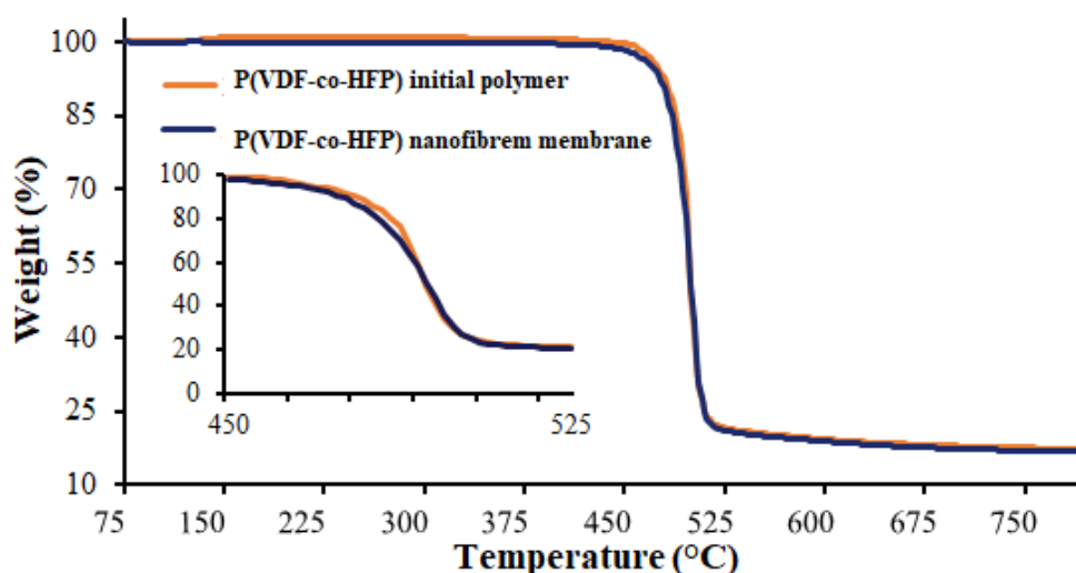
Figure 4. 9 Weight loss (wt.%) versus temperature for nanofibre membrane and initial polymer.
