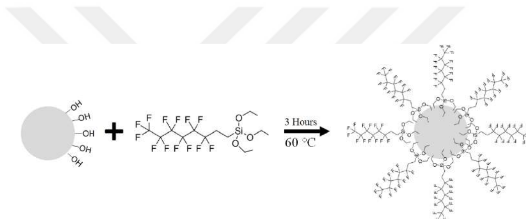
Figure 3. 5 Surface modification of \text{SiO}_2 nanoparticles with PFTOES.
