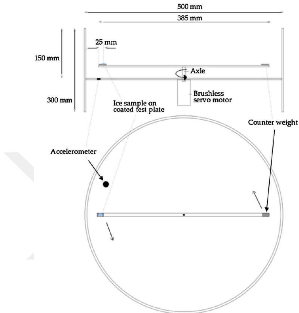
Figure 3. 13 Schematic diagrams of the centrifuge ice adhesion test device [143] consist of a carbon fibre rotor driven by a brushless servo motor and housed in a stainless-steel casing.
