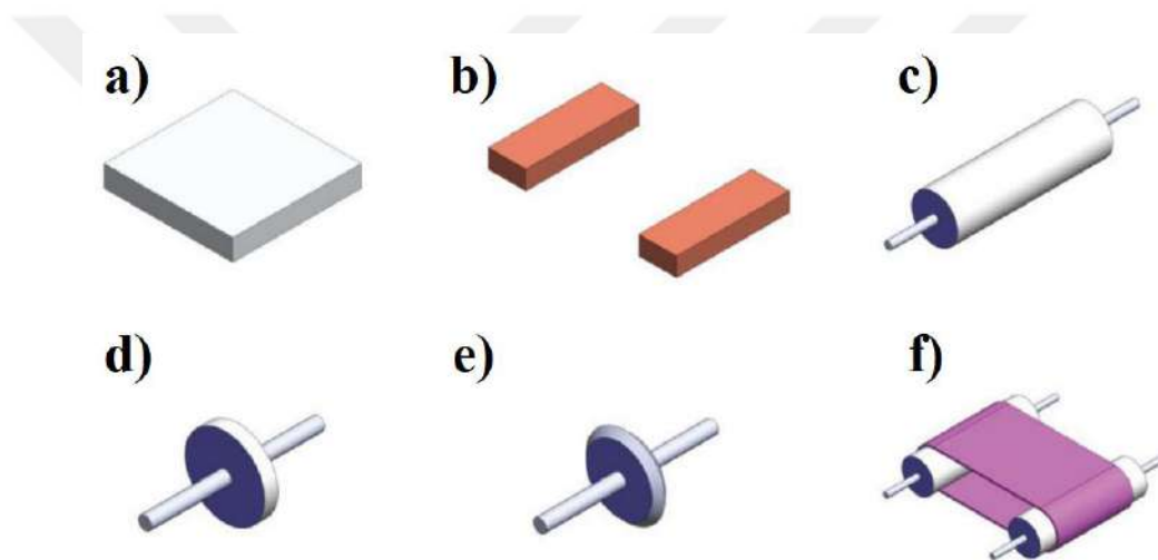
Figure 2.10 Some types of electrospinning collectors (a) flat plate, (b) parallel plates, (c) rotating drum, (d) rotating disc with a flat edge, (e) rotating disc with a sharp edge and (f) conveyor [46].
