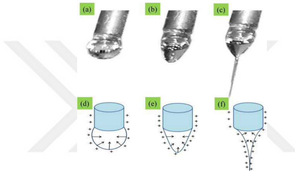
Figure 2.12 Effect of increasing voltage to the droplet shape (a-c) and schematic representation of droplet deformation with increasing voltage (d-f) [65].
