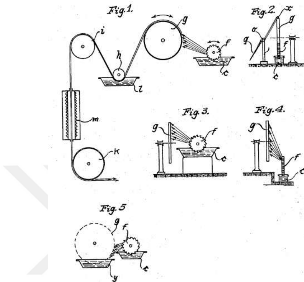
Figure 2.1 Schematic illustration of the patented apparatus by Anton Formhals [19, 20].
