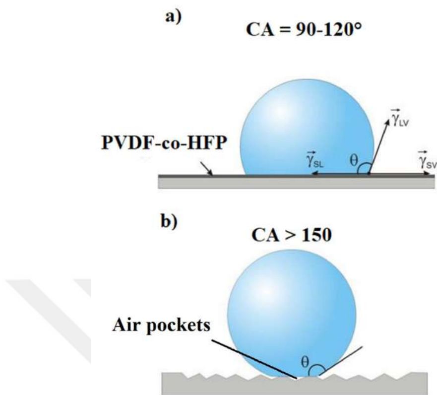
Figure 4. 18 Schematic representation of the effect of surface structure on contact angle (a) flat PVDF-co-HFP (90~120°) and (b) high-roughness surface PVDF-co-HFP (>150°).
