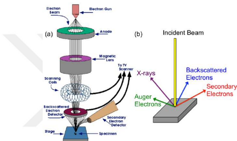
Figure 3. 11 (a) Schematic representation of and working principle of SEM (b) the sample-beam interactions and electronic signals generated [166].
