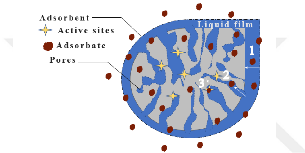
Figure 2.11 Mass transfer kinetics steps in adsorption (Wang & Guo, 2020)
