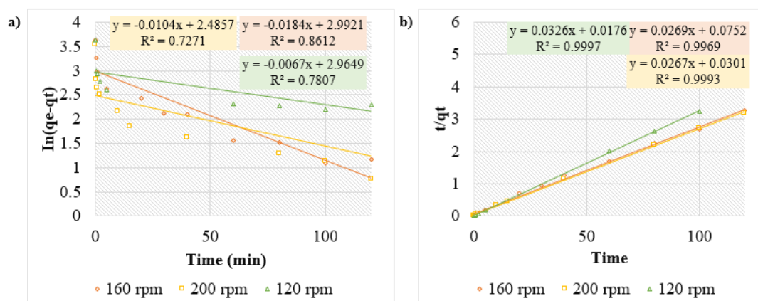
Figure 4.18 Kinetic models for different shaking speeds a) PFO, b) PSO
