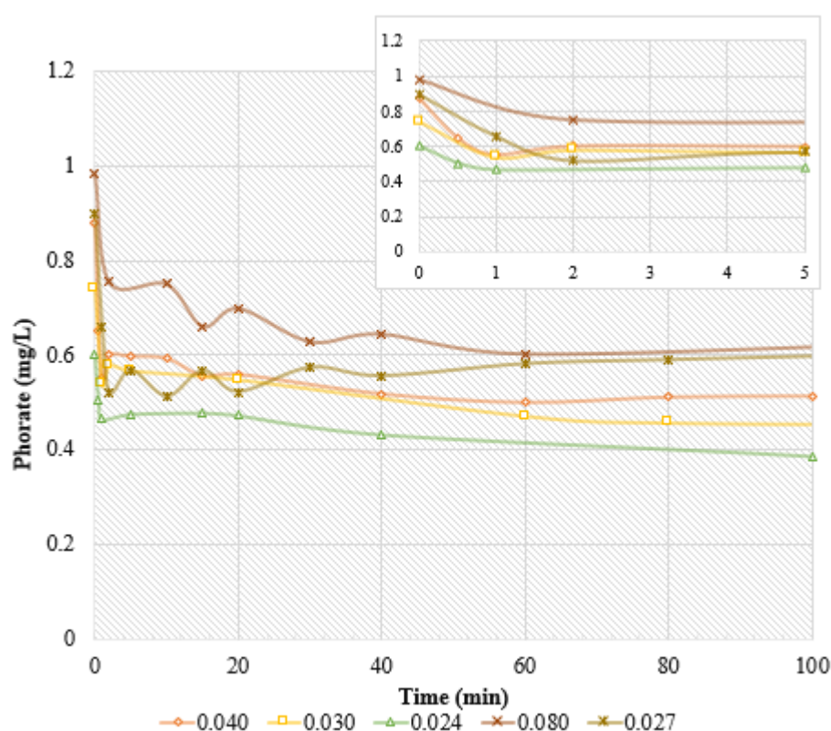
Figure 4.15 The effect of adsorbate to adsorbent ratio on the adsorption kinetic of phorate on CHA (160 rpm, pH 7, 25 °C)
