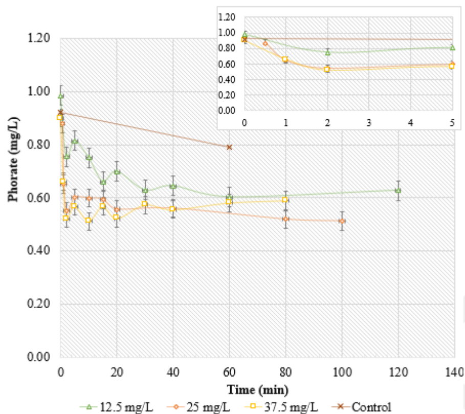
Figure 4.11 The effect of CHA dosage on the kinetics of adsorption of phorate onto CHA ( C_0=1 mg/L at 25 °C, 160 rpm, pH 7)
