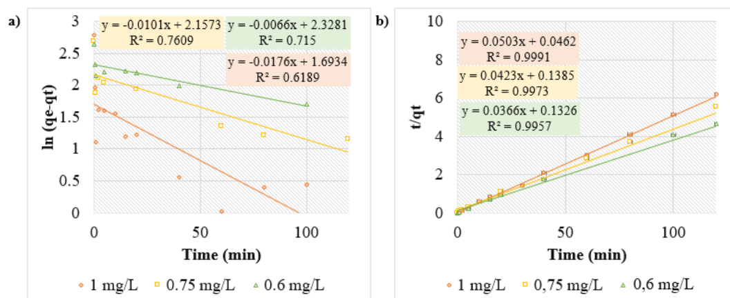
Figure 4.8 Kinetic models for different initial concentrations a) PFO, b) PSO
