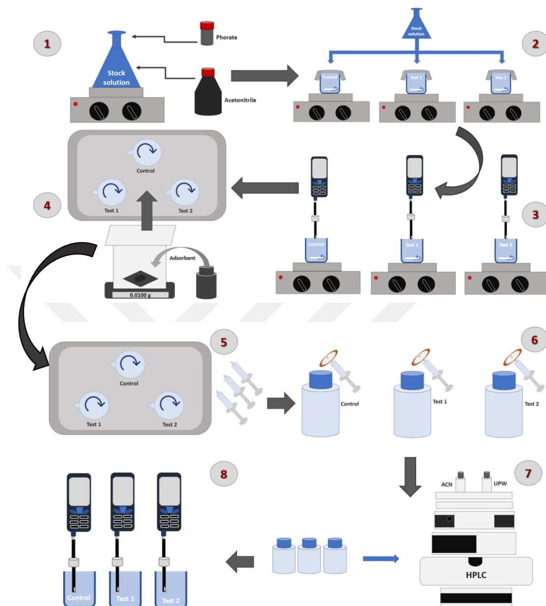
Figure 3.2 The flow diagram for the experimental procedure followed
