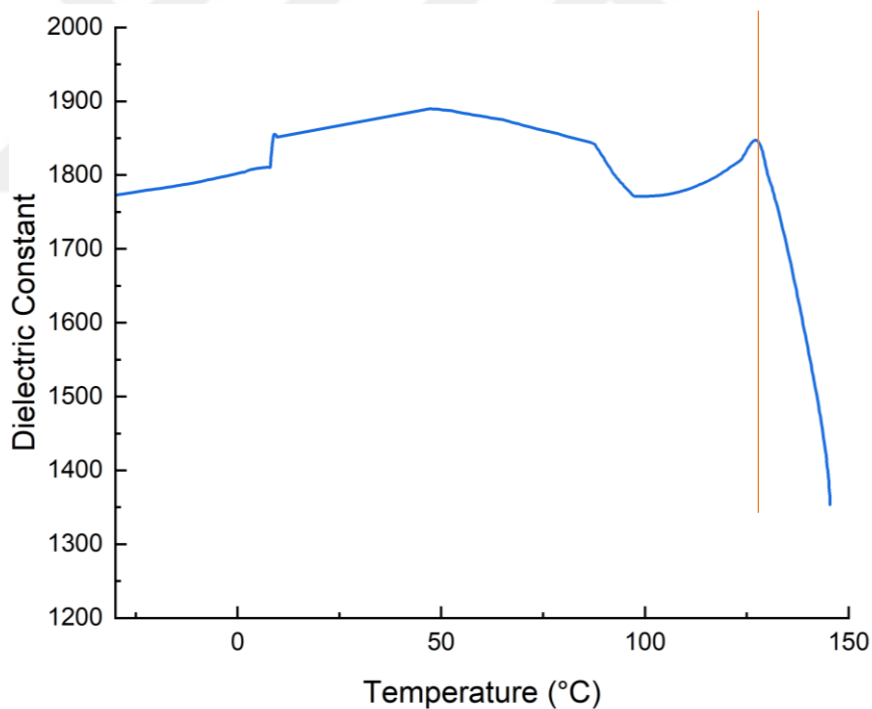
Figure 48. \epsilon_r vs temperature graph of Nb doped \text{BaTiO}_3 ceramic sintered at 1270 °C for 1 h.
