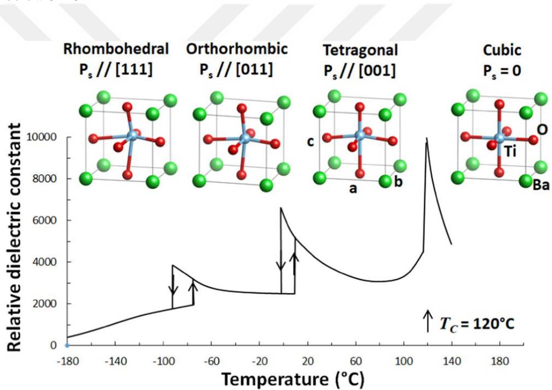
Figure 8. Temperature dependence of BaTiO 3 crystal structure [40].
