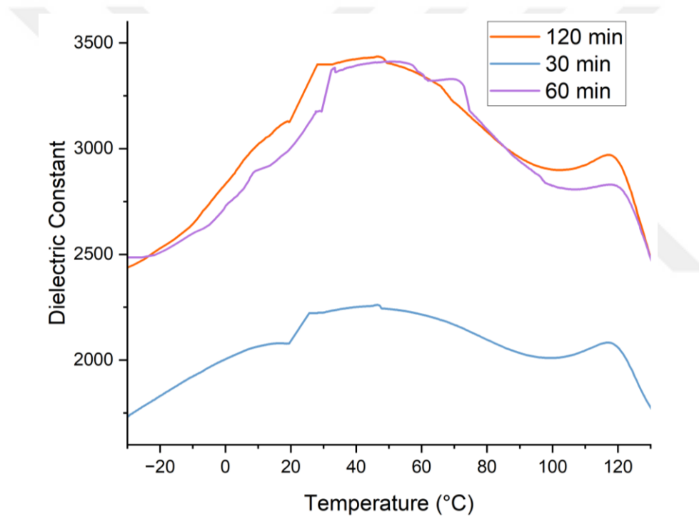
Figure 59. \epsilon_r vs temperature graph of Nb 3 Co 1 ceramics sintered at 1270 °C for different sintering times.
