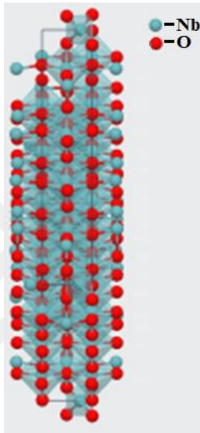
Figure 16. Crystal structure of \text{Nb}_2\text{O}_5 [47].
