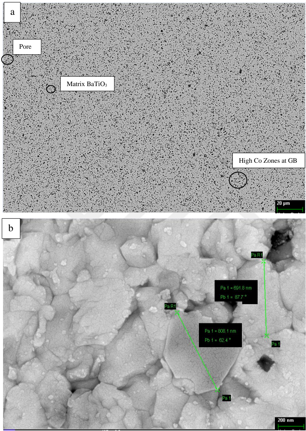
Figure 38. SEM images of 1 mole% \text{Co}_3\text{O}_4 added \text{BaTiO}_3 ceramic sintered at 1270 °C for 1 h. (a) Low magnification. (b) High magnification for grain size measurement.
