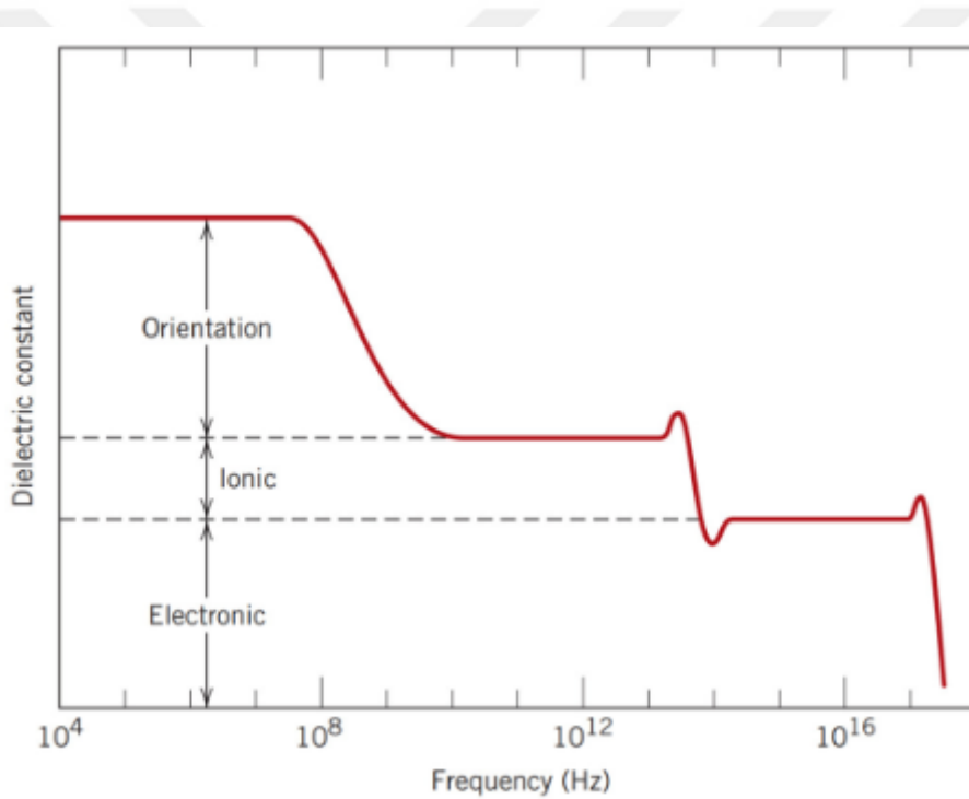
Figure 4. Variation of \epsilon_r with frequency. Contributions of polarization types to \epsilon_r [24].
