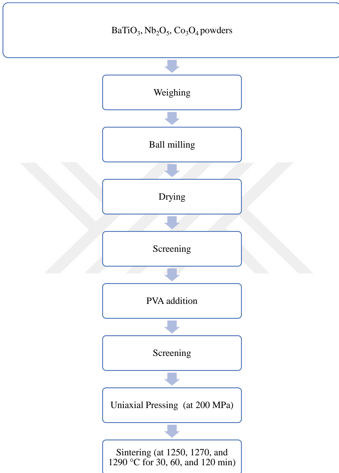
Figure 19. Flowsheet showing the steps applied for the preparation of the BaTiO 3 based ceramic capacitors.
