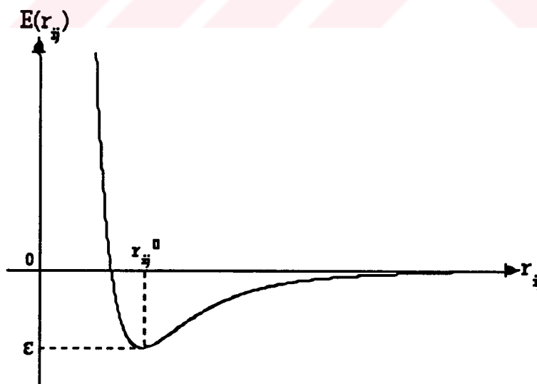
FIGURE 4.2. Lennard-Jones potential vs. r_{ij}
