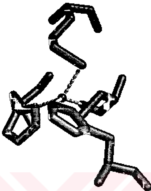
FIGURE 2.4. An example of group 1 copper ligands. Ligands of the first copper of methylamine dehydrogenase, 1mda
