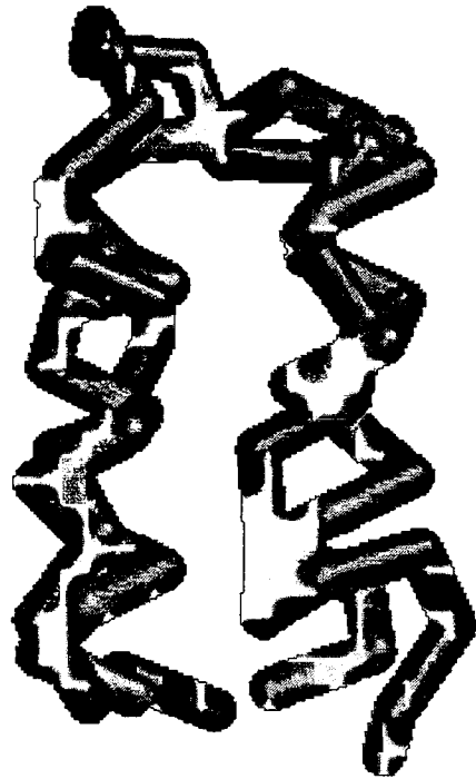
FIGURE 7.11. The superimposed structure of predicted and 30-residue segment of 1rop. The light-grey structure is the native structure and the darker one is the predicted tertiary structure. The 3-D structure of the backbone is shown.
