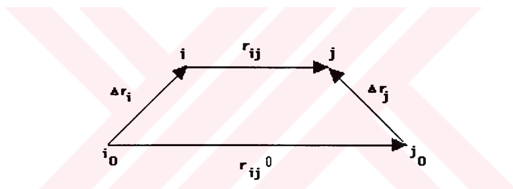
FIGURE 5.1. Representation of r_{ij}
