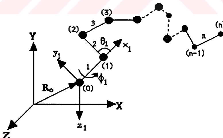
FIGURE 4.1. A random configuration of a protein chain. The C^{\alpha} atoms are numbered from 0 to n in the laboratory-fixed frame, OXYZ, as shown in parentheses. The first bond-based coordinate system x_1y_1z_1 is shown.
