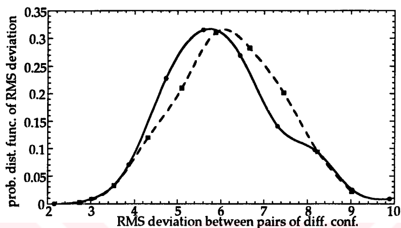
FIGURE 7.4. Probability distribution function of RMS deviations between pairs of conformations satisfying the end-to-end constraint (solid curve) and the constraint applied to the middle of the chain (dashed curve).
