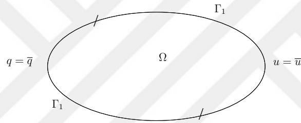
Figure 2.1: The geometry of the domain and boundary conditions
