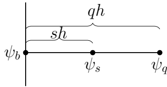
Figure 1.1: \psi_b boundary value \psi_s and \psi_q interior values
