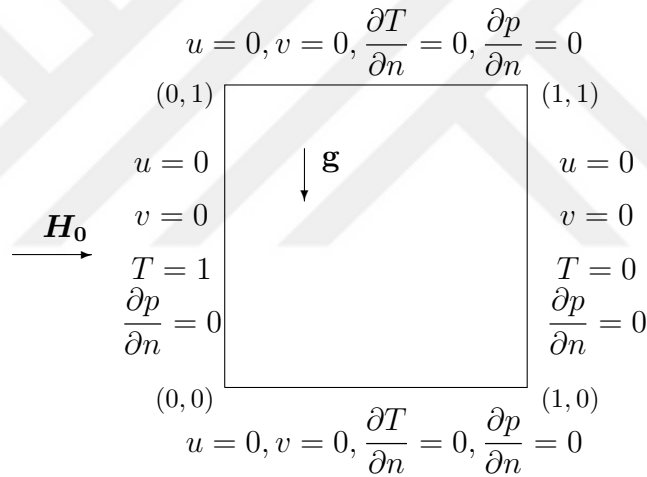
Figure 4.3: Problem 4.3.1: Square cavity and boundary conditions.
