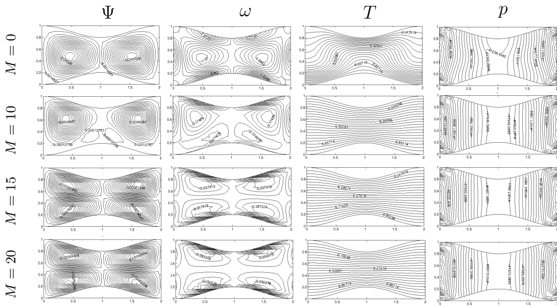
Figure 3.61: Problem 3.6.5: The effect of M on the flow, temperature and pressure for Gr = 10^4 , CR = 40\% and L = 2 , \mathbf{H}_0 = (0, 1) .
