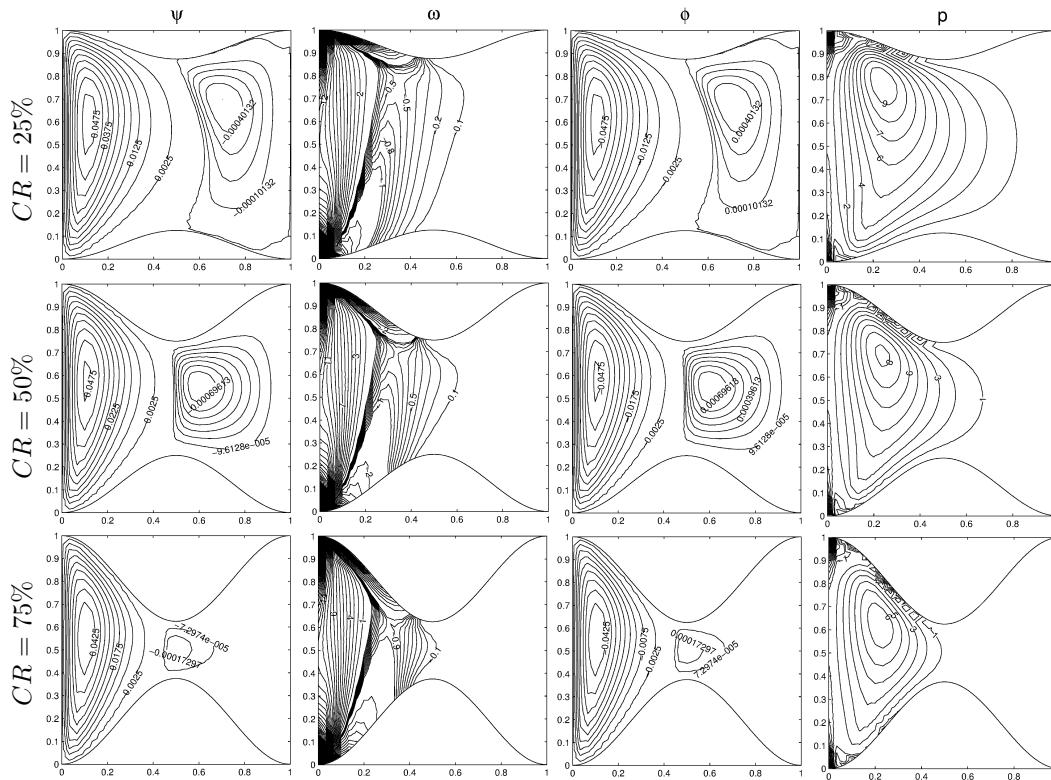
Figure 3.37: Problem 3.5.2: MHD flow with electric potential for M = 40 , \mathbf{H}_0 = (0, 0, 1) .
