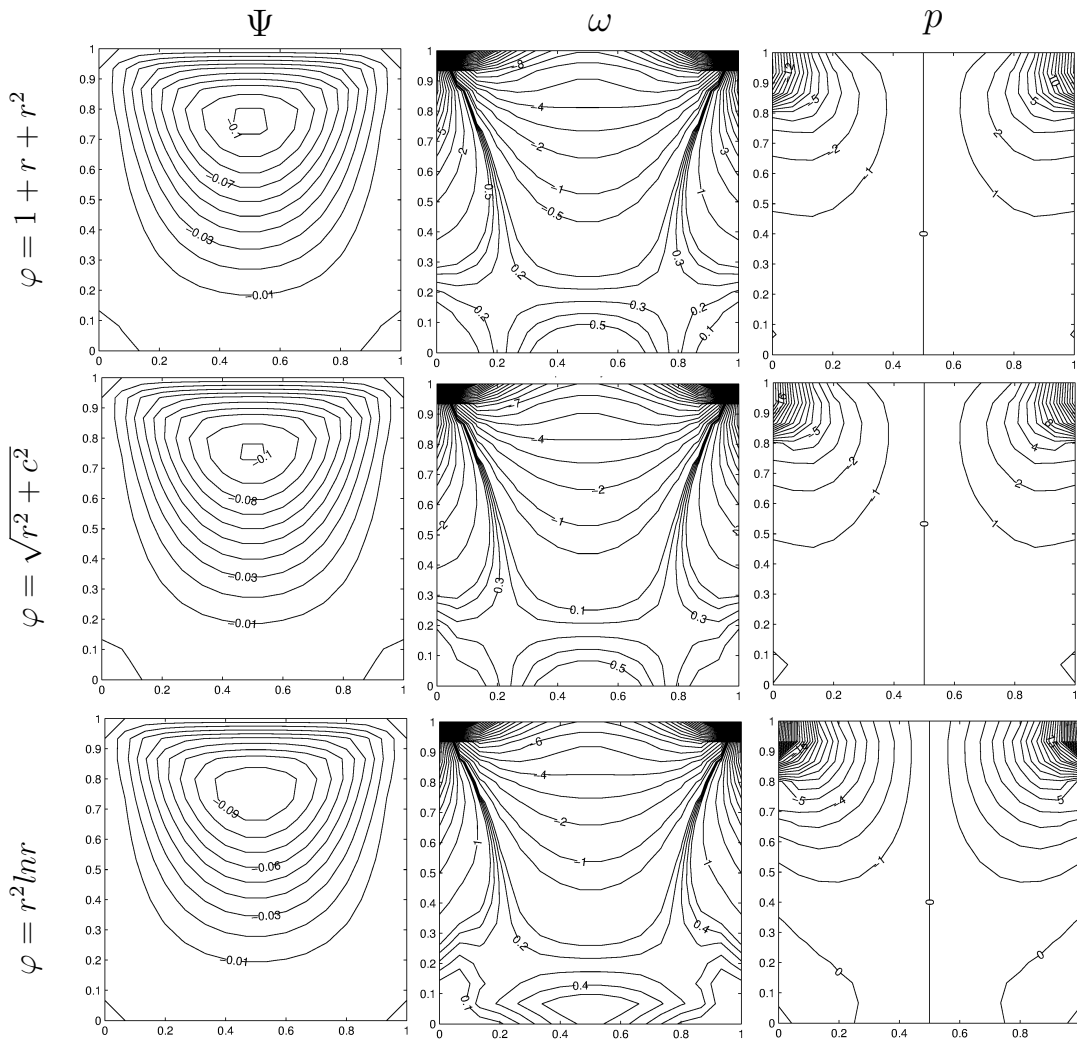
Figure 3.5: Problem 3.1: RBF solution of the MHD Stokes flow for M = 0 using \varphi = 1 + r + r^2 , \varphi = \sqrt{r^2 + c^2} and \varphi = r^2 \ln r .
