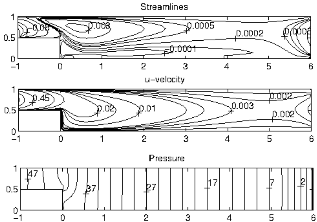
Figure 3.19: Problem 3.3: MHD Stokes flow with M = 0 , \mathbf{H}_0 = (1, 0, 0) .
