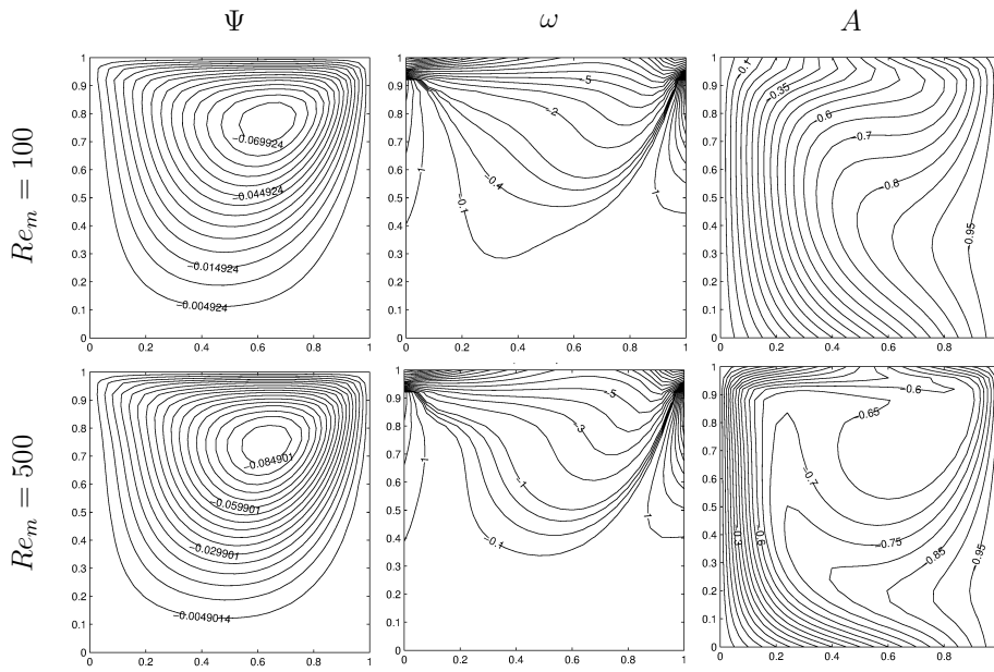
Figure 4.7: Problem 4.4.1: Streamlines, vorticity contours, magnetic potential lines for Re_m = 100, 500 using \Delta t = 0.2, Re = 100, M = 10 .
