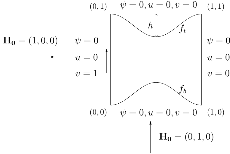
Figure 3.11: Problem 3.2: Schematic of the square cavity with constriction and the boundary conditions
