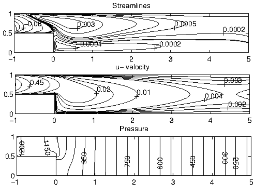
Figure 3.24: Problem 3.3: MHD Stokes flow with M = 0 , \mathbf{H}_0 = (0, 1, 0) .
