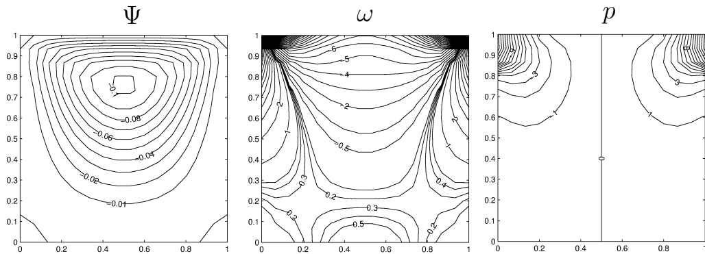
Figure 3.2: Problem 3.1: RBF solution of the MHD Stokes flow for M = 0 .
