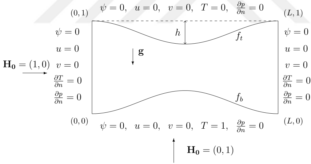
Figure 3.54: Problem 3.6.5: Schematic of the rectangular cavity with constriction and the boundary conditions
