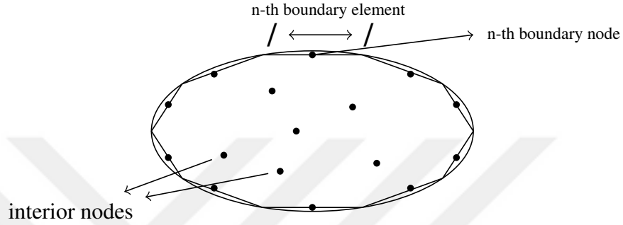
Figure 2.2: Constant boundary element case
