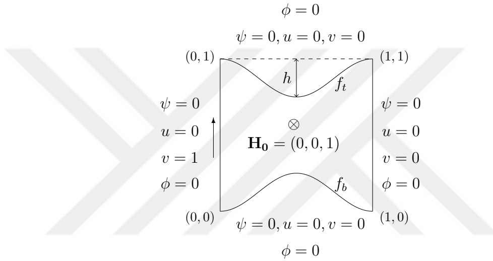
Figure 3.34: Problem 3.5.2: Constricted cavity and boundary conditions.
