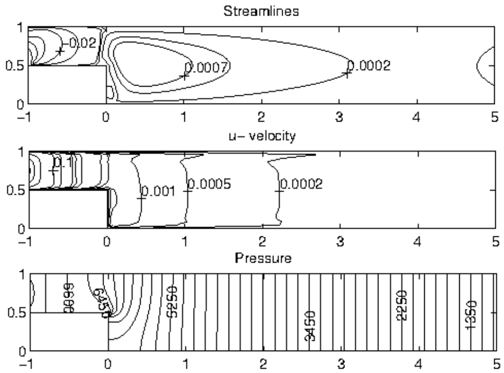
Figure 3.26: Problem 3.3: MHD Stokes flow with M = 30 , \mathbf{H}_0 = (0, 1, 0) .
