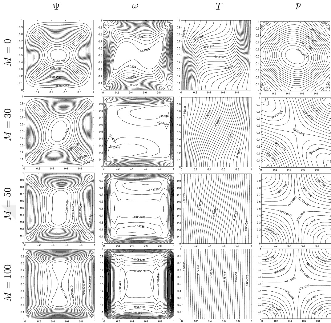
Figure 4.4: Problem 4.3.1: Streamlines, vorticity contours, isotherms and pressure contours for Gr = 10^4 and M = 0, 30, 50, 100 with \Delta t = 0.1, 0.1, 0.05, 0.01 , respectively.
