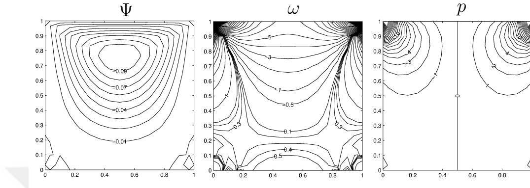
Figure 3.7: Problem 3.1: DRBEM solution of the MHD Stokes flow for M = 0 .
