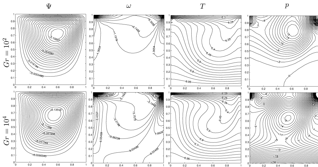
Figure 3.52: Problem 3.6.4: MHD convection flow for M = 0 , Ec = 1 .
