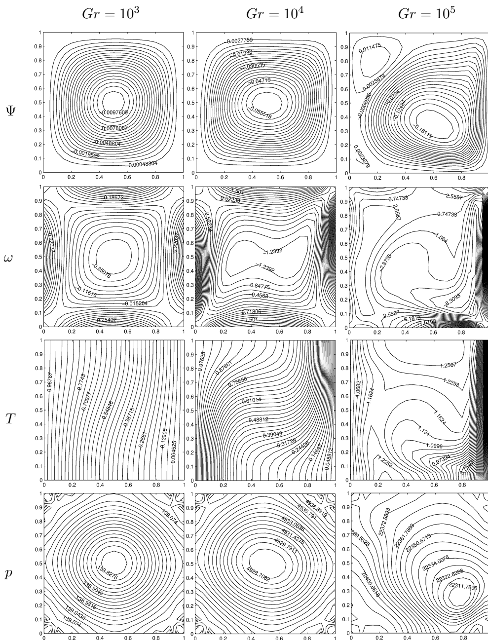
Figure 3.47: Problem 3.6.3: MHD convection flow for M = 0 , Ec = 1 .
