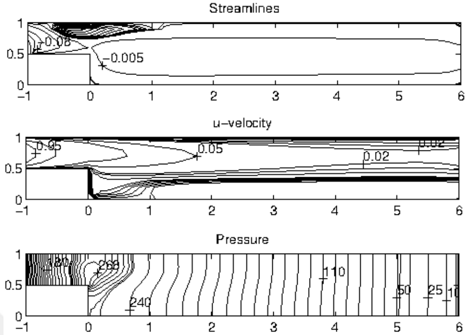
Figure 3.23: Problem 3.3: MHD Stokes flow with M = 90 , \mathbf{H}_0 = (1, 0, 0) .
