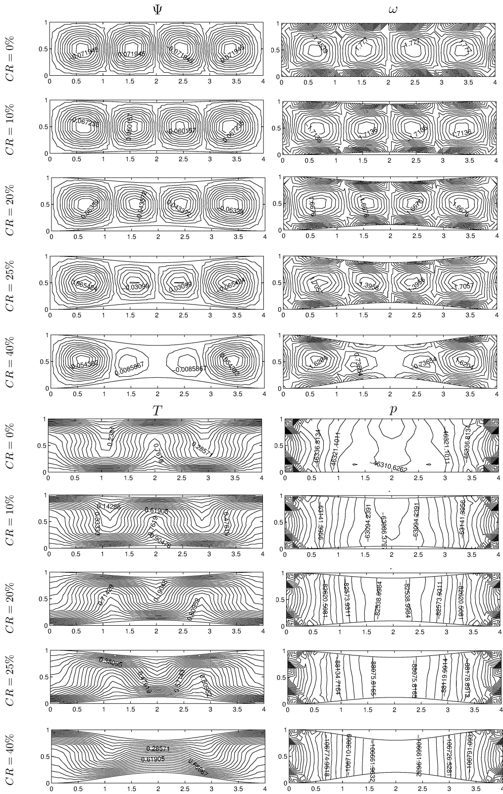
Figure 3.59: Problem 3.6.5: The effect of CR on the flow, temperature and pressure for Gr = 10^4 , M = 4 and L = 4 , \mathbf{H}_0 = (0, 1) .
