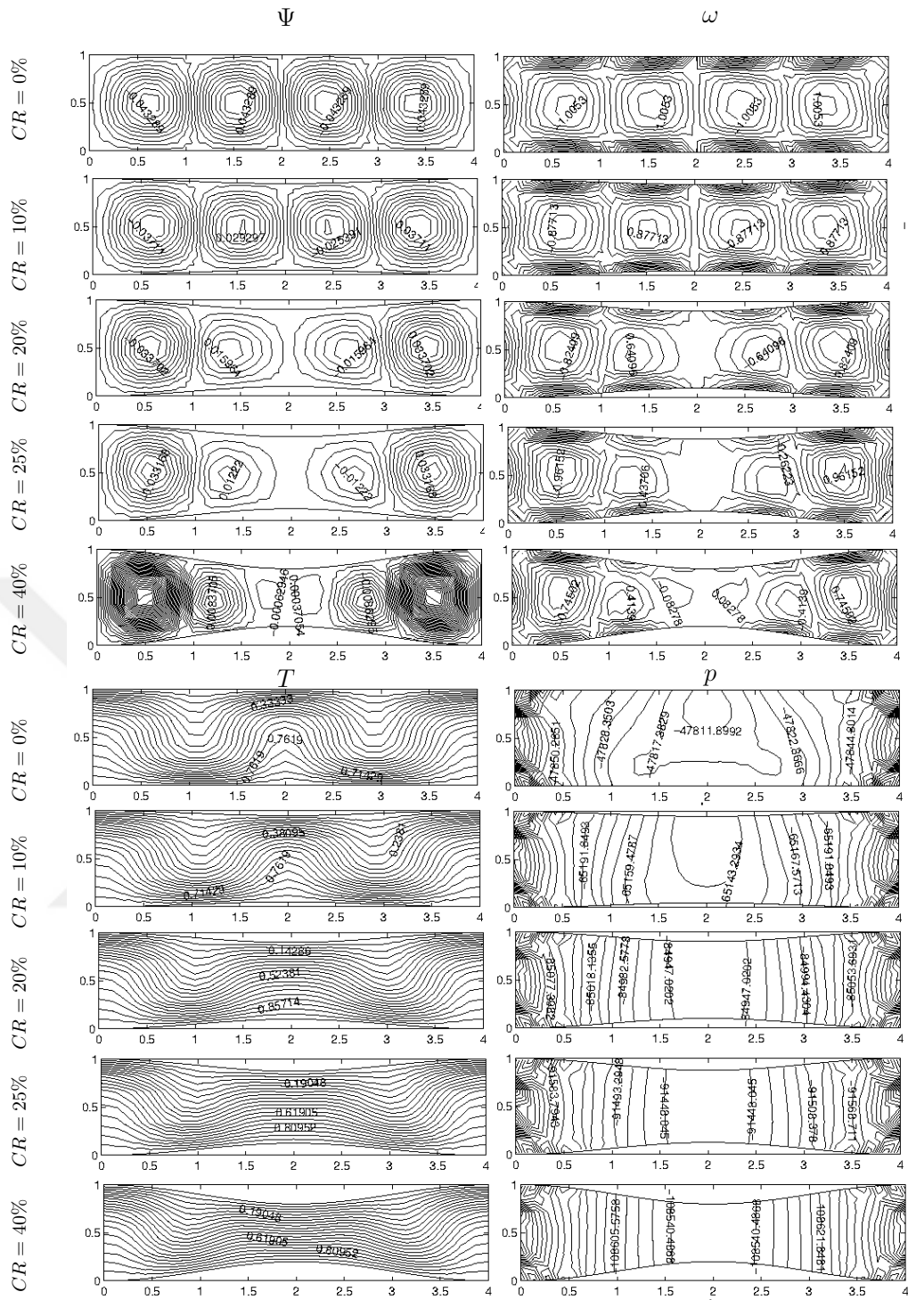
Figure 3.60: Problem 3.6.5: The effect of CR on the flow, temperature and pressure for Gr = 10^4 , M = 10 and L = 4 , \mathbf{H}_0 = (0, 1) .
