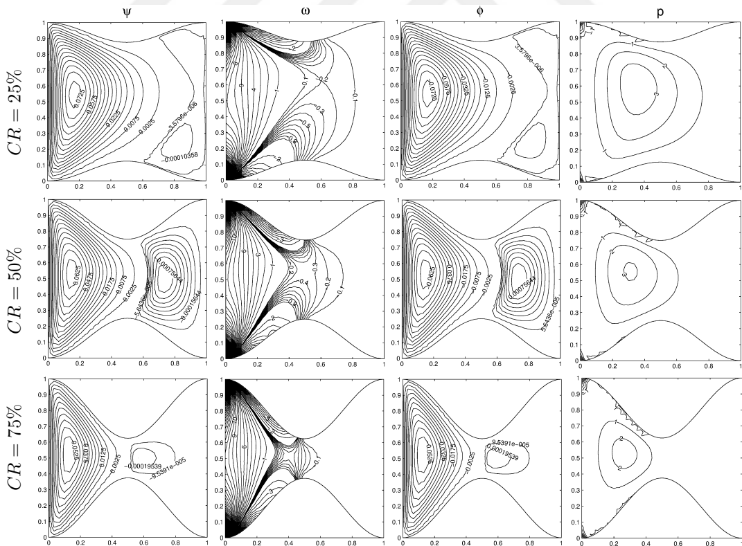
Figure 3.36: Problem 3.5.2: MHD flow with electric potential for M = 20 , \mathbf{H}_0 = (0, 0, 1) .
