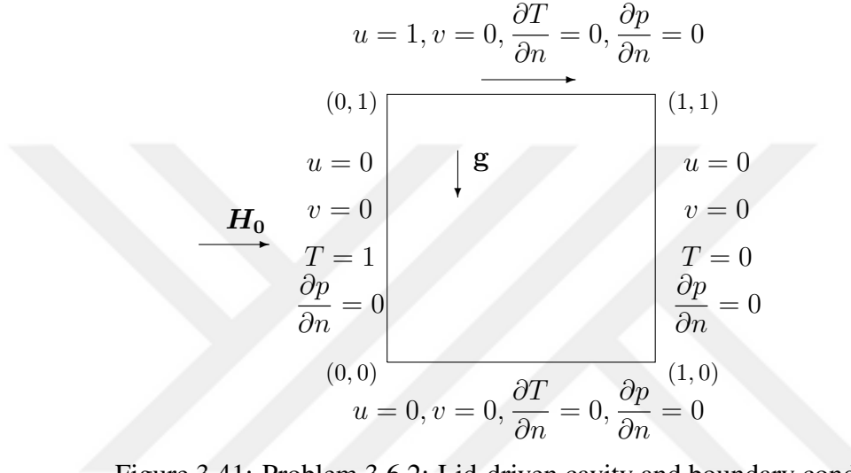
Figure 3.41: Problem 3.6.2: Lid-driven cavity and boundary conditions.
