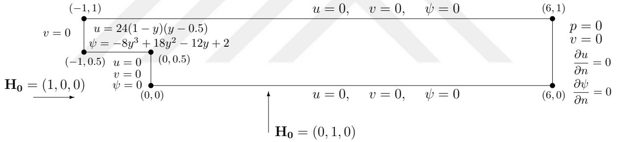
Figure 3.18: Problem 3.3: Backward-Facing step channel and boundary conditions
