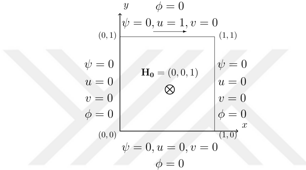
Figure 3.32: Problem 3.5.1: Lid-driven cavity and boundary conditions.
