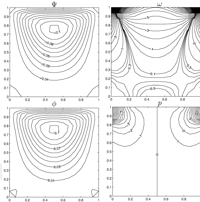
Figure 3.29: Problem 3.4: Stokes flow with electric potential ( \phi|_{wall} = 0 ), M = 0 .
