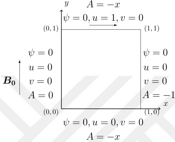
Figure 4.5: Problem 4.4.1: Lid-driven cavity and boundary conditions.
