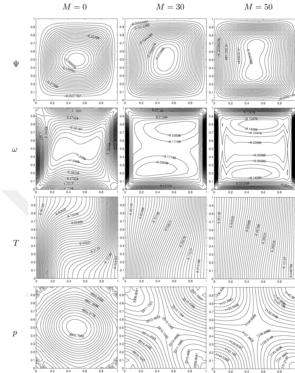
Figure 3.46: Problem 3.6.3: MHD convection flow for Gr = 10^4 , Ec = 0 .
