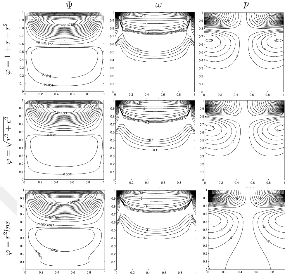
Figure 3.6: Problem 3.1: RBF solution of the MHD Stokes flow for M = 30 using \varphi = 1 + r + r^2 , \varphi = \sqrt{r^2 + c^2} and \varphi = r^2 \ln r .
