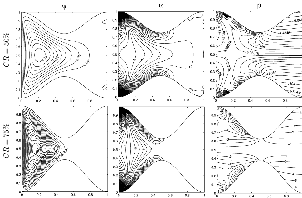
Figure 3.14: Problem 3.2: MHD Stokes flow with M = 10 , \mathbf{H}_0 = (1, 0, 0) .
