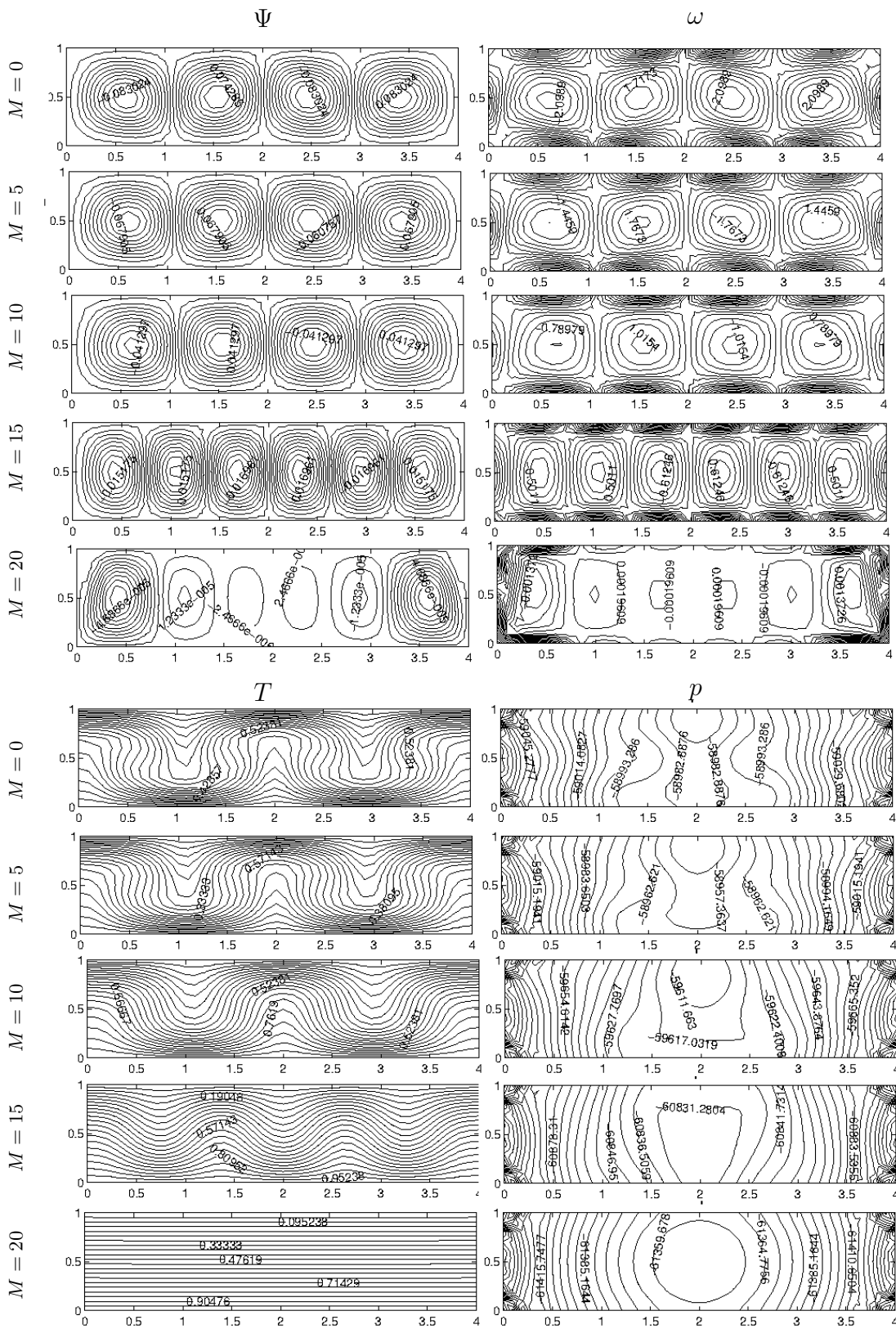
Figure 3.58: Problem 3.6.5: The effect of M on the flow, temperature and pressure for Gr = 10^4 and L = 4 , \mathbf{H}_0 = (0, 1) .
