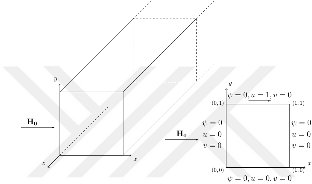
Figure 3.1: Problem 3.1: Lid-driven cavity and boundary conditions.
