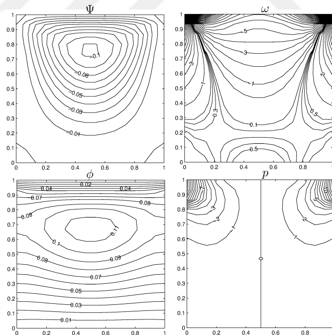
Figure 3.30: Problem 3.4: Stokes flow with electric potential ( \frac{\partial \phi}{\partial n}|_{x=0,1}, \phi|_{y=0,1} = 0 ), M = 0 .
