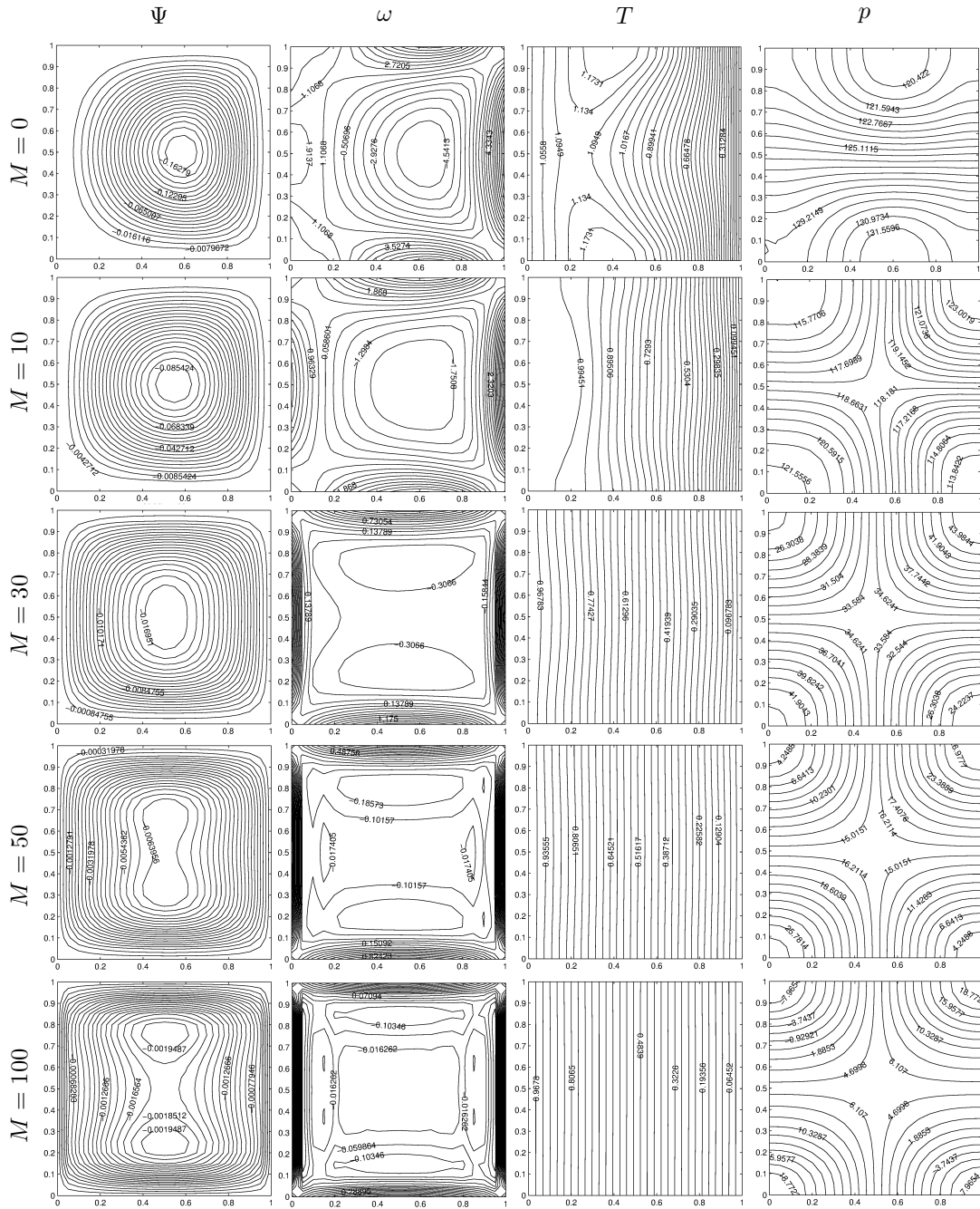
Figure 3.40: Problem 3.6.1: MHD convection Stokes flow for Gr = 90 , Ec = 1 .
