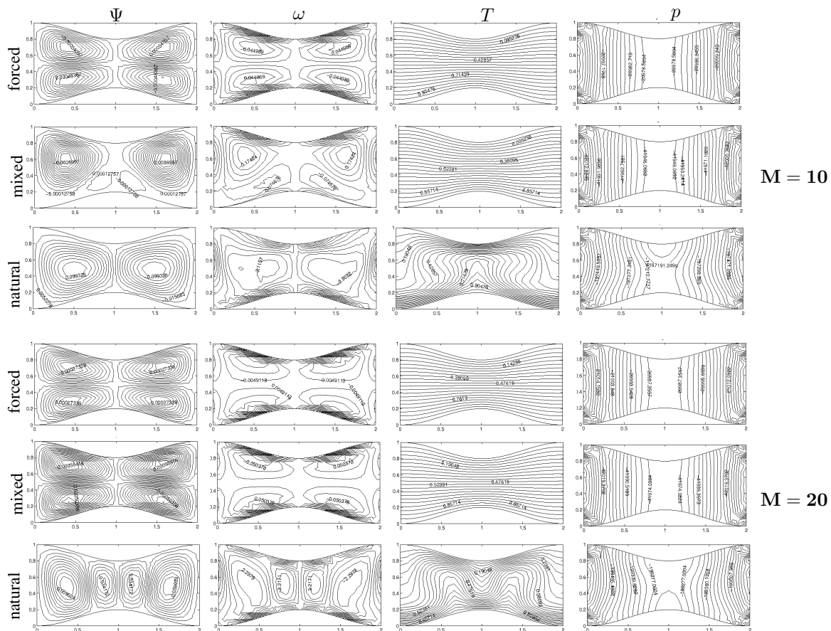
Figure 3.63: Problem 3.6.5: The effect of magnetic field on convection flow for CR = 40\% and L = 2 , \mathbf{H}_0 = (0, 1) .
