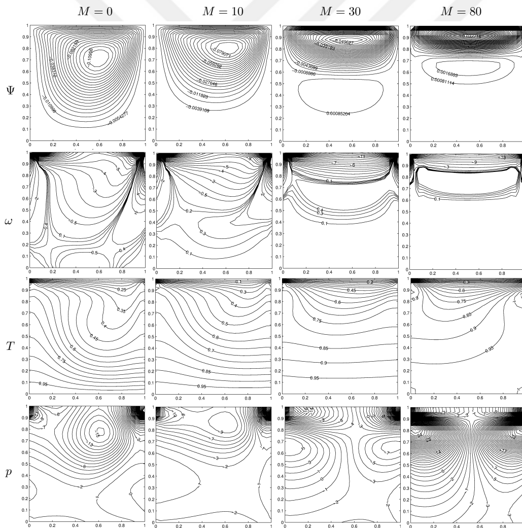
Figure 3.53: Problem 3.6.4: MHD convection flow for Gr = 10^3 , Ec = 1 .
