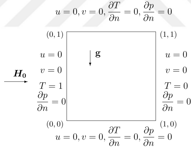
Figure 3.44: Problem 3.6.3: Square cavity and boundary conditions.
