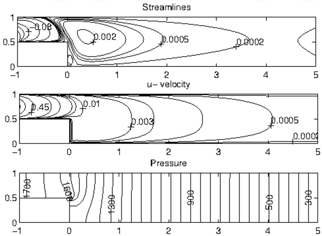
Figure 3.25: Problem 3.3: MHD Stokes flow with M = 10 , \mathbf{H}_0 = (0, 1, 0) .
