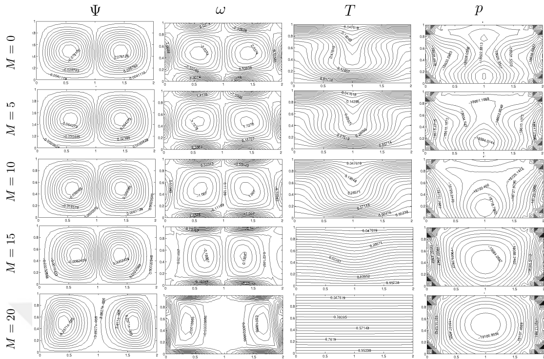
Figure 3.57: Problem 3.6.5: The effect of M on the flow, temperature and pressure for Gr = 10^4 and L = 2 , \mathbf{H}_0 = (0, 1) .
