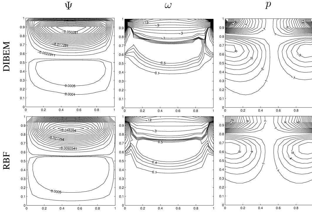
Figure 3.10: Problem 3.1: DIBEM and RBF solutions of the MHD Stokes flow for M = 30 .
