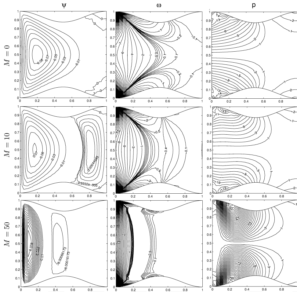
Figure 3.16: Problem 3.2: MHD Stokes flow with CR = 25\% , \mathbf{H}_0 = (0, 1, 0) .
