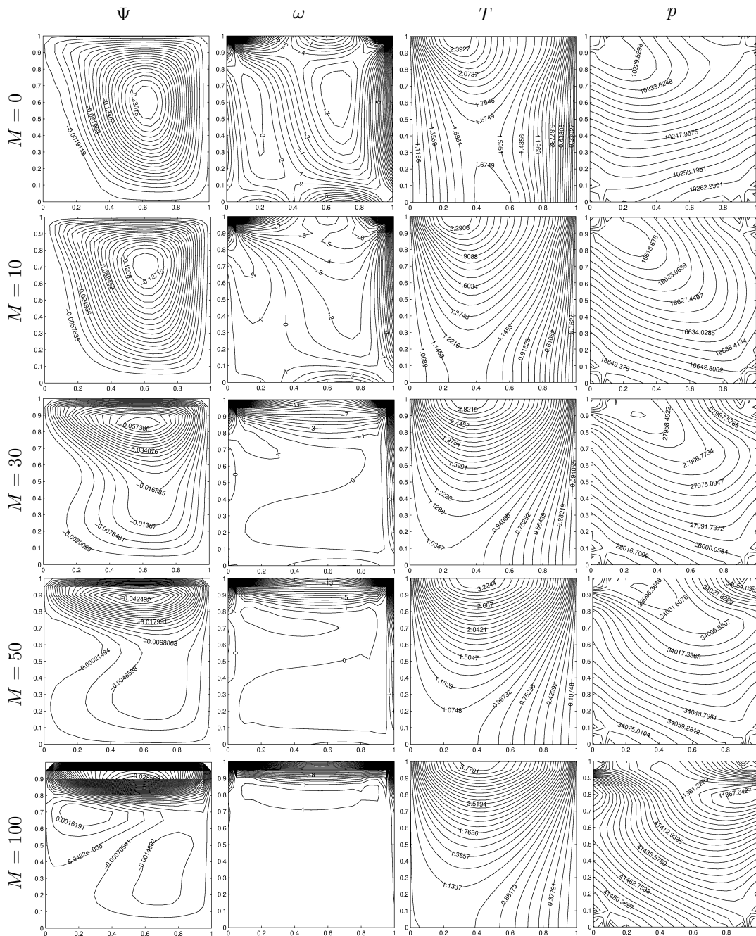
Figure 3.43: Problem 3.6.2: MHD convection Stokes flow for Gr = 90 , Ec = 1 .
