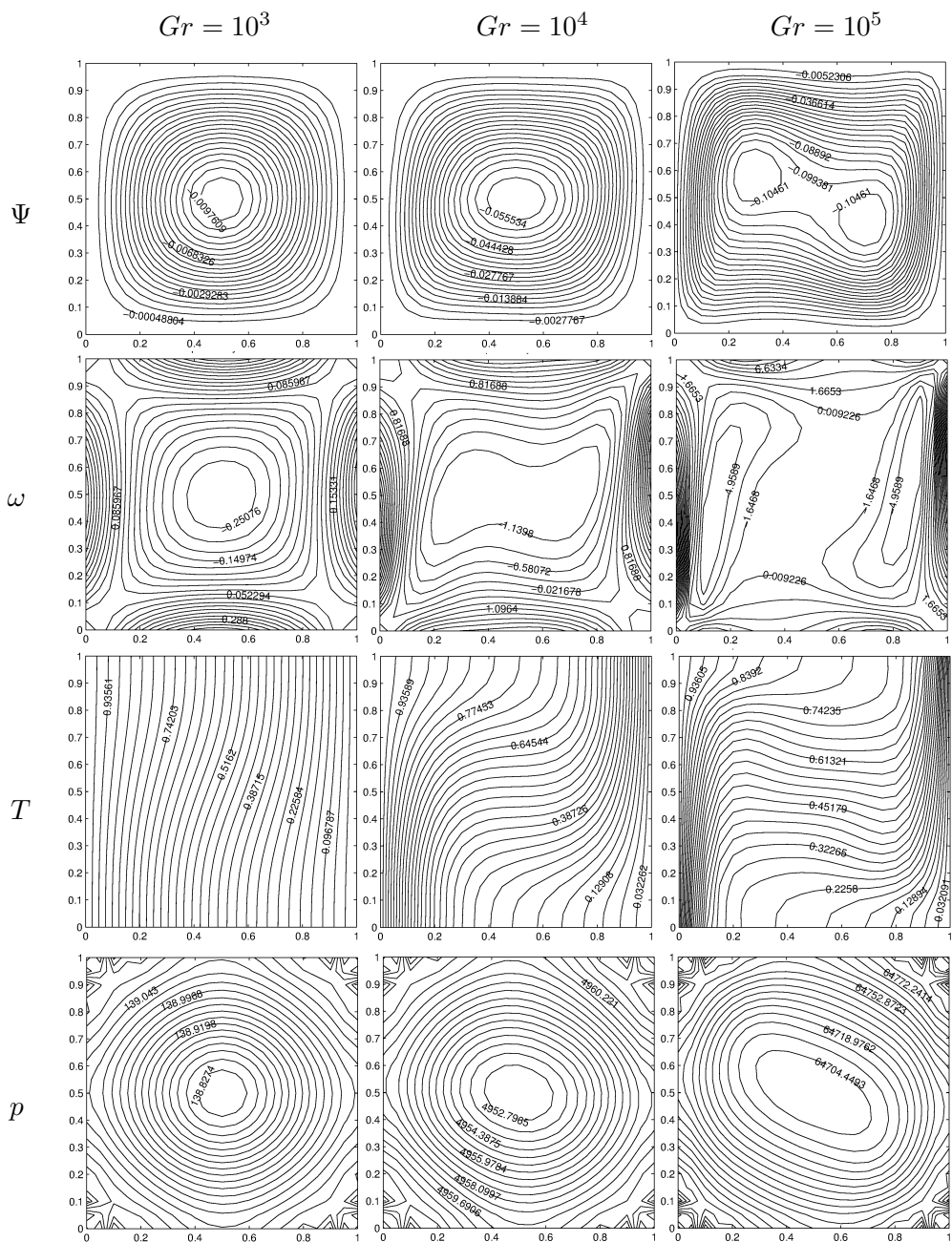
Figure 3.45: Problem 3.6.3: MHD convection flow for M = 0 , Ec = 0 .
