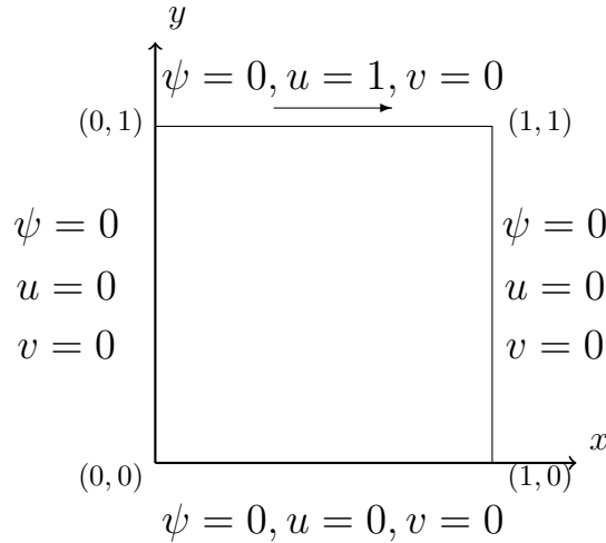
Figure 4.1: Problem 4.2.1: Lid-driven cavity and boundary conditions.
