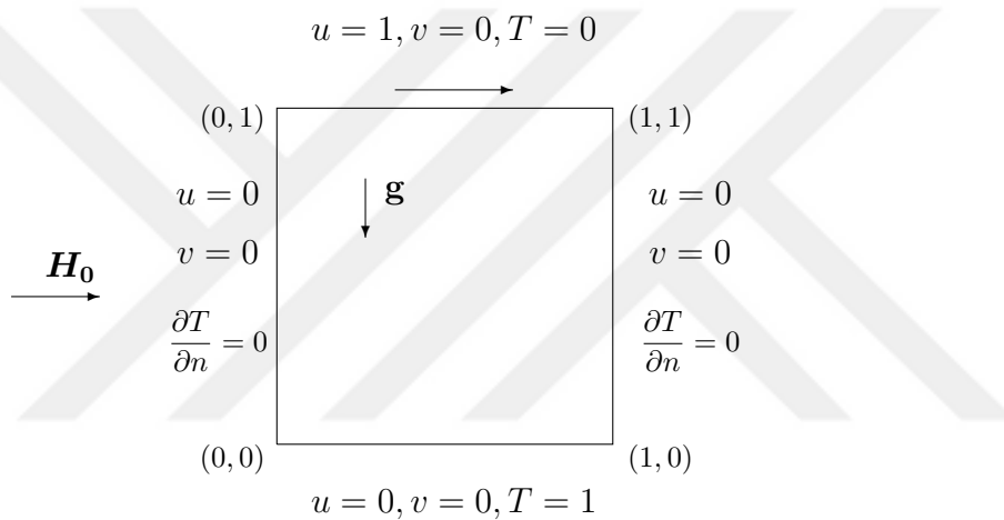
Figure 3.49: Problem 3.6.4: Lid-driven cavity and boundary conditions.
