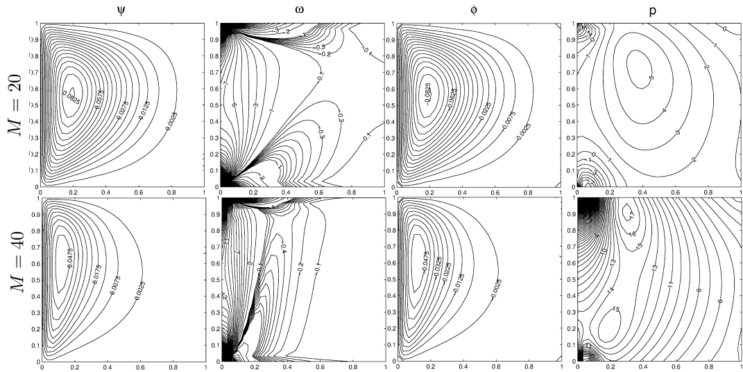
Figure 3.35: Problem 3.5.2: MHD flow with electric potential for CR = 0\% , \mathbf{H}_0 = (0, 0, 1) .
