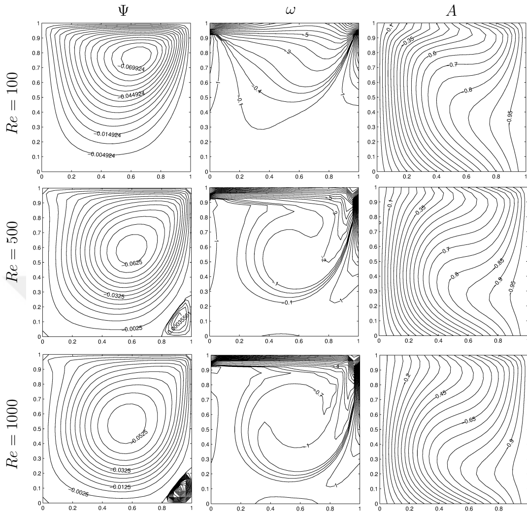
Figure 4.6: Problem 4.4.1: Streamlines, vorticity contours, magnetic potential lines for Re = 100, 500, 1000 using \Delta t = 0.2, M = 10, Re_m = 100 .
