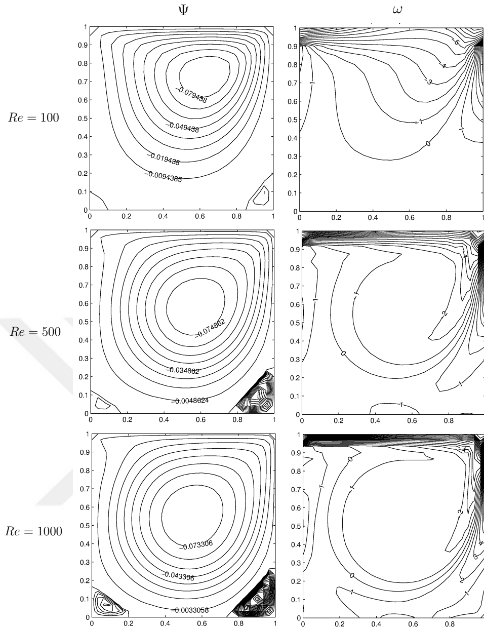
Figure 4.2: Problem 4.2.1: Flow behaviors for Re = 100, 500, 1000 using \Delta t = 0.8, 0.5, 0.1 , respectively.
