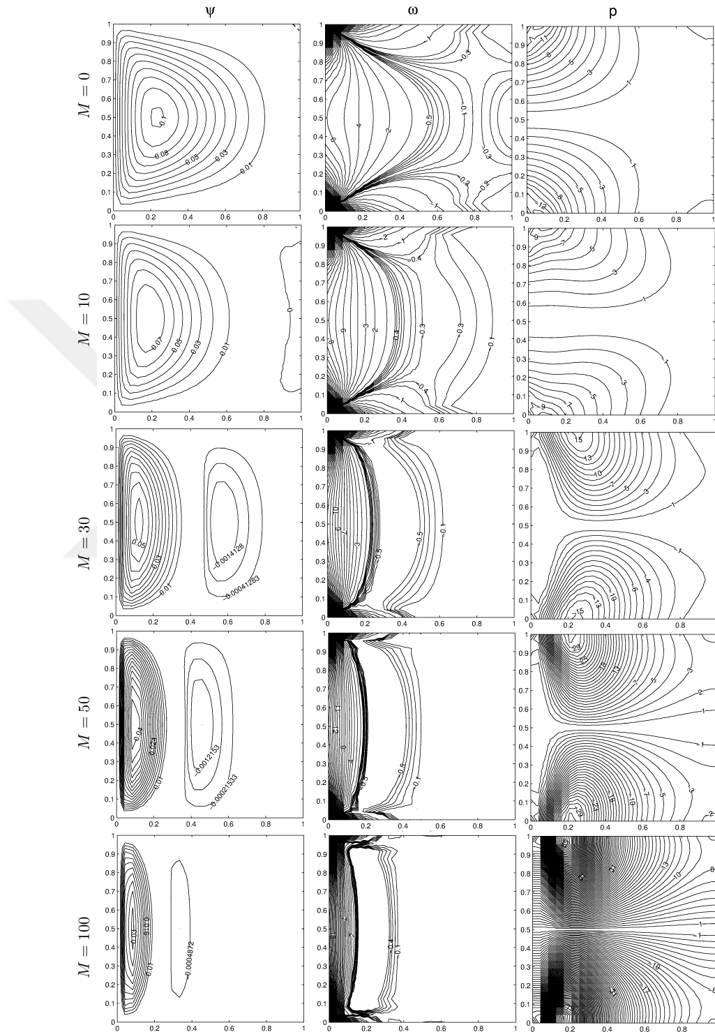
Figure 3.15: Problem 3.2: MHD Stokes flow with CR = 0\% , \mathbf{H}_0 = (0, 1, 0) .
