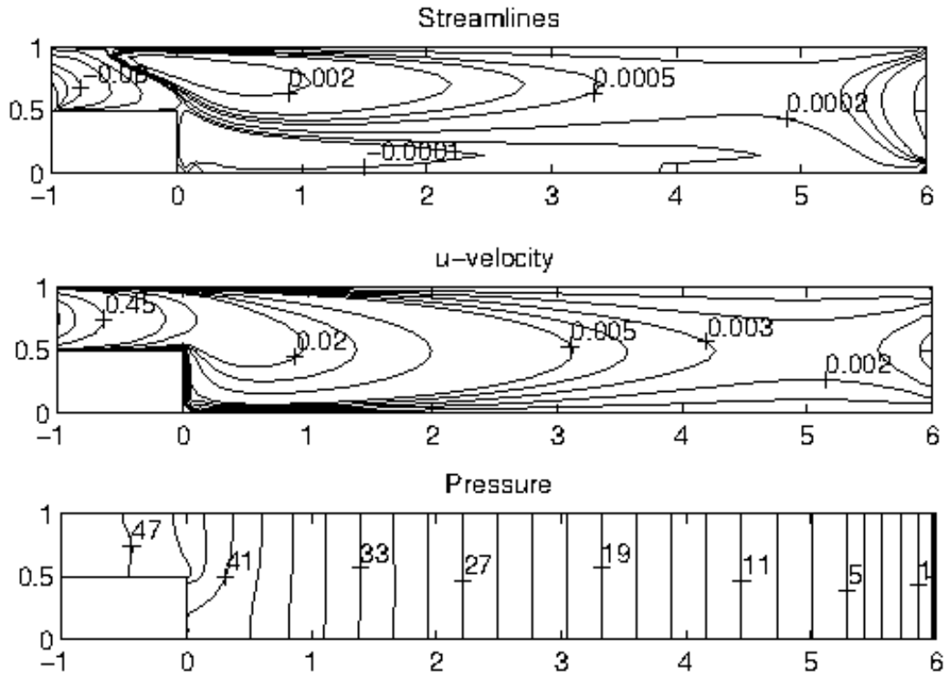
Figure 3.21: Problem 3.3: MHD Stokes flow with M = 10 , \mathbf{H}_0 = (1, 0, 0) .
