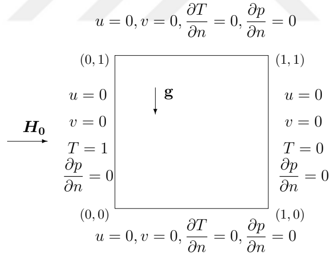
Figure 3.38: Problem 3.6.1: Square cavity and boundary conditions.
