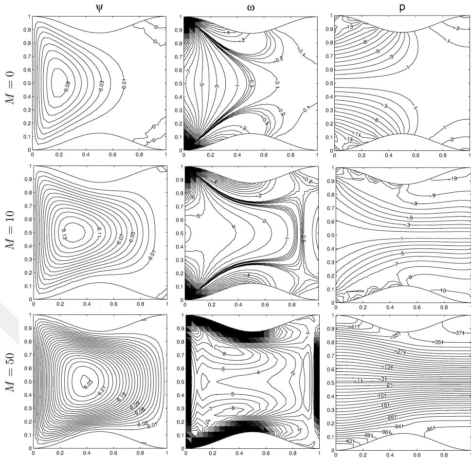
Figure 3.13: Problem 3.2: MHD Stokes flow with CR = 25\% , \mathbf{H}_0 = (1, 0, 0) .
