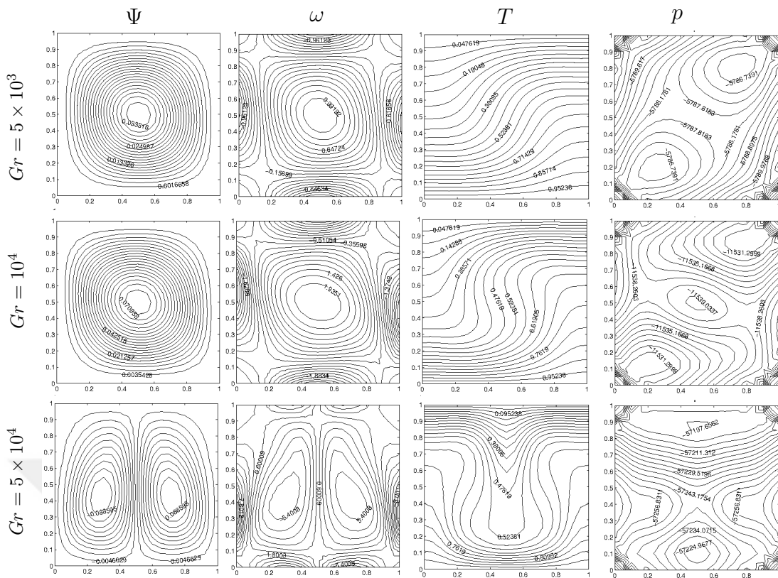
Figure 3.55: Problem 3.6.5: The effect of Gr on the flow, temperature and pressure for M = 0 and L = 1 , \mathbf{H}_0 = (0, 1) .
