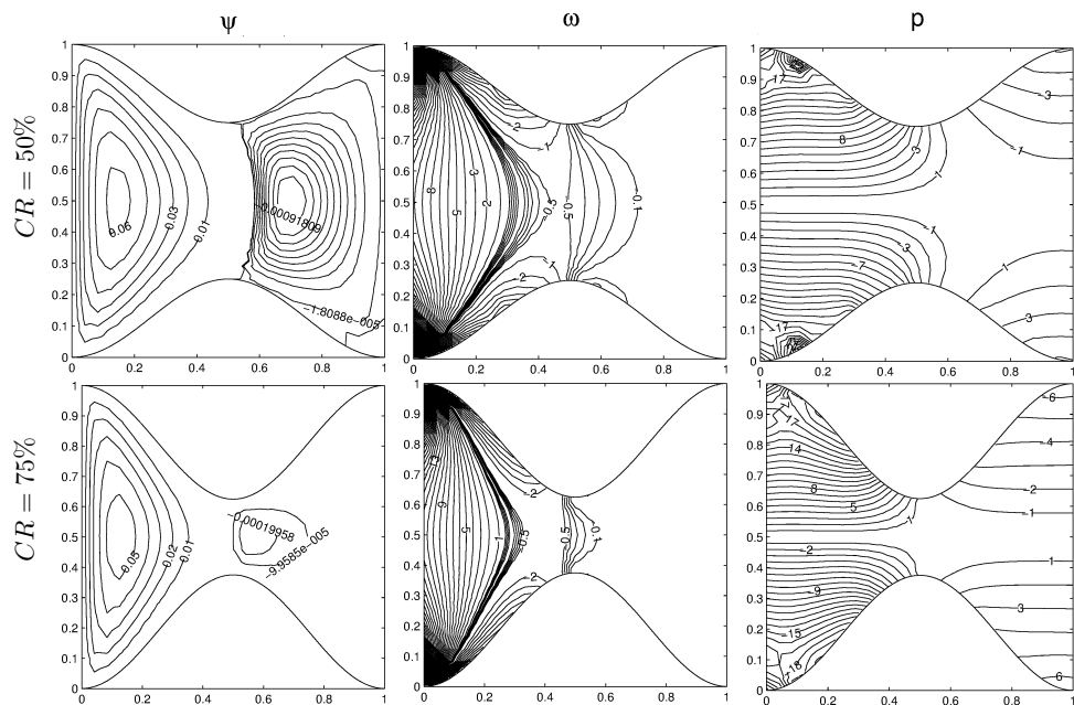
Figure 3.17: Problem 3.2: MHD Stokes flow with M = 10 , \mathbf{H}_0 = (0, 1, 0) .
