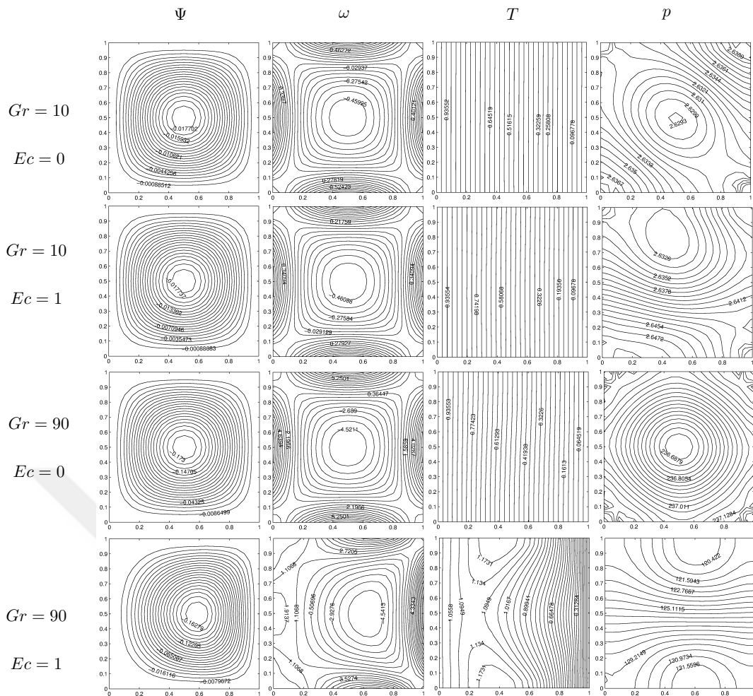
Figure 3.39: Problem 3.6.1: MHD convection Stokes flow for M = 0 .
