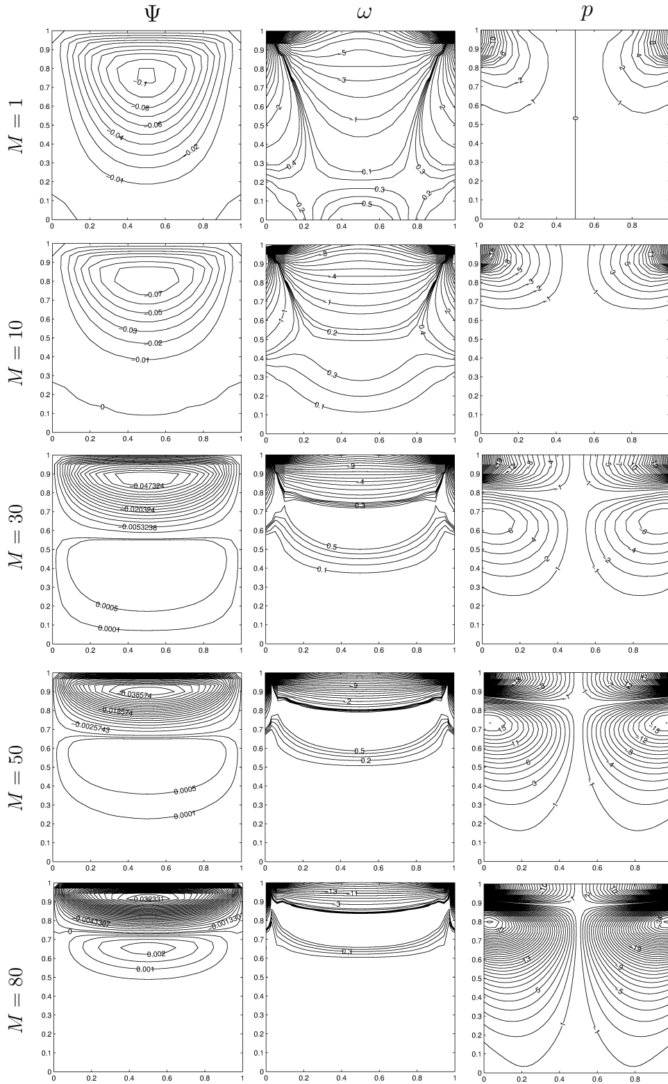
Figure 3.3: Problem 3.1: RBF solution of the MHD Stokes flow for 1 \leq M \leq 80 .
