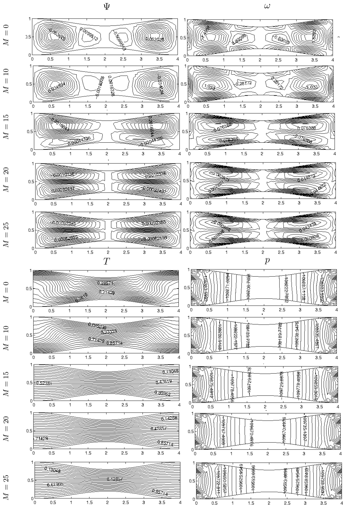
Figure 3.65: Problem 3.6.5: The effect of M on the flow, temperature and pressure for Gr = 10^4 , CR = 40\% and L = 4 , \mathbf{H}_0 = (1, 0) .
