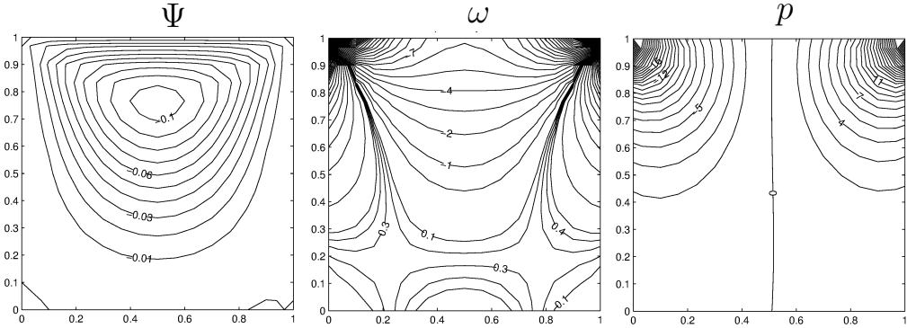
Figure 3.9: Problem 3.1: DIBEM solution of the MHD Stokes flow for M = 0 .
