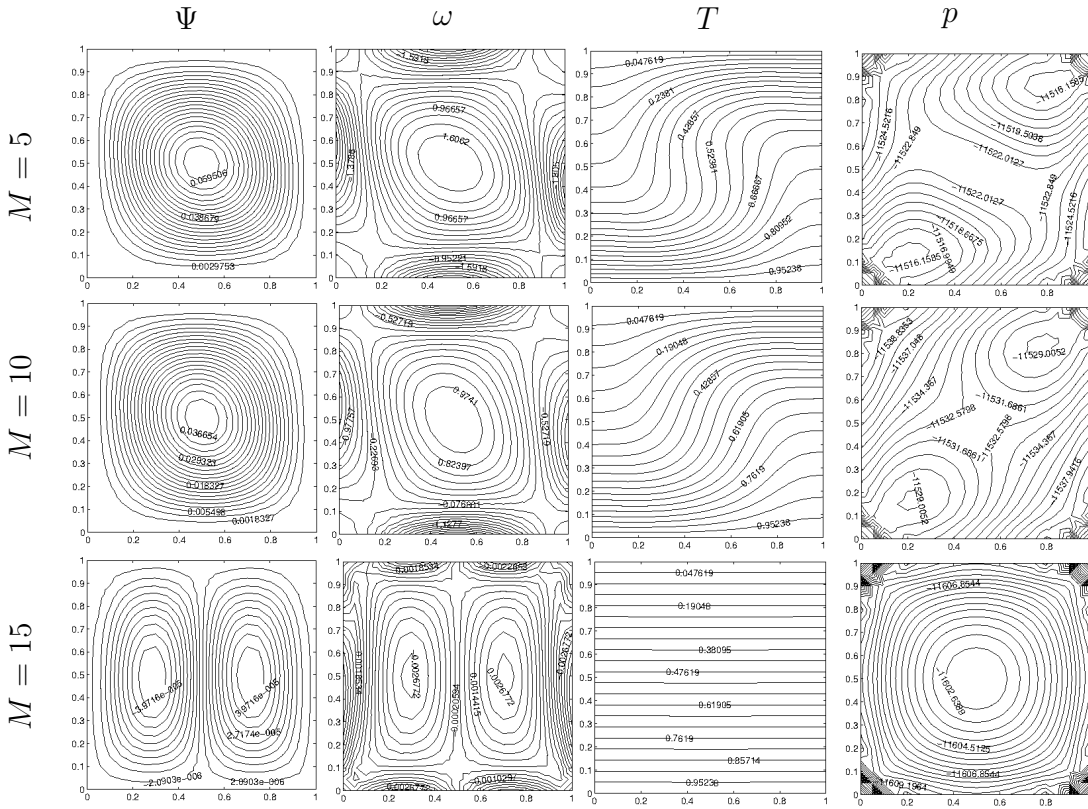
Figure 3.56: Problem 3.6.5: The effect of M on the flow, temperature and pressure for Gr = 10^4 and L = 1 , \mathbf{H}_0 = (0, 1) .
