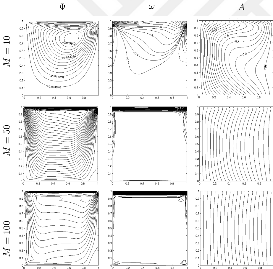
Figure 4.8: Problem 4.4.1: Streamlines, vorticity contours, magnetic potential lines for M = 10, 50, 100 using \Delta t = 0.2, 0.1, 0.05 , respectively, Re = Re_m = 100 .
