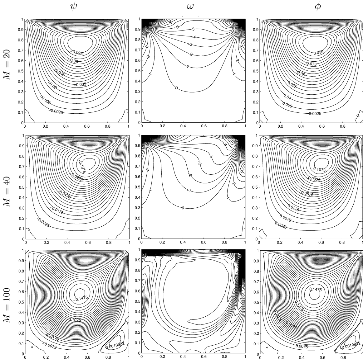
Figure 3.33: Problem 3.5.1: MHD flow with electric potential, \mathbf{H}_0 = (0, 0, 1) .
