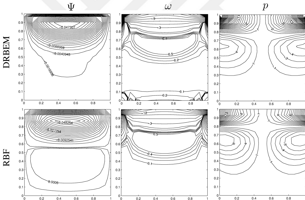
Figure 3.7: Problem 3.1: DRBEM solution of the MHD Stokes flow for M = 0 .
