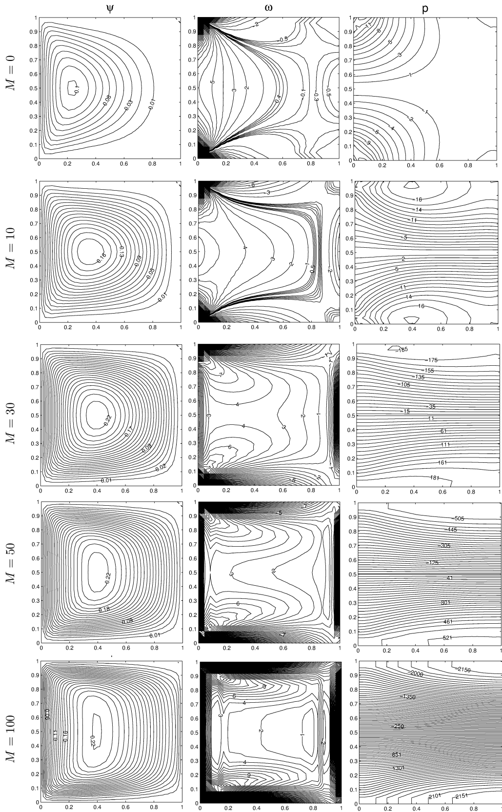
Figure 3.12: Problem 3.2: MHD Stokes flow with CR = 0\% , \mathbf{H}_0 = (1, 0, 0) .
