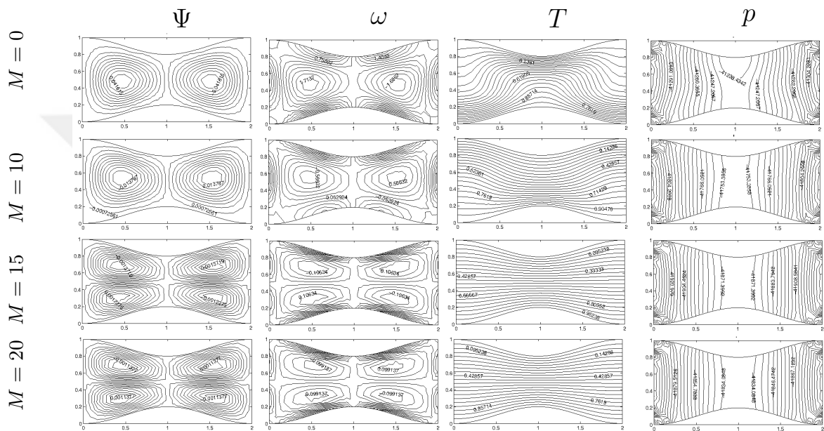
Figure 3.64: Problem 3.6.5: The effect of M on the flow, temperature and pressure for Gr = 10^4 , CR = 40\% and L = 2 , \mathbf{H}_0 = (1, 0) .
