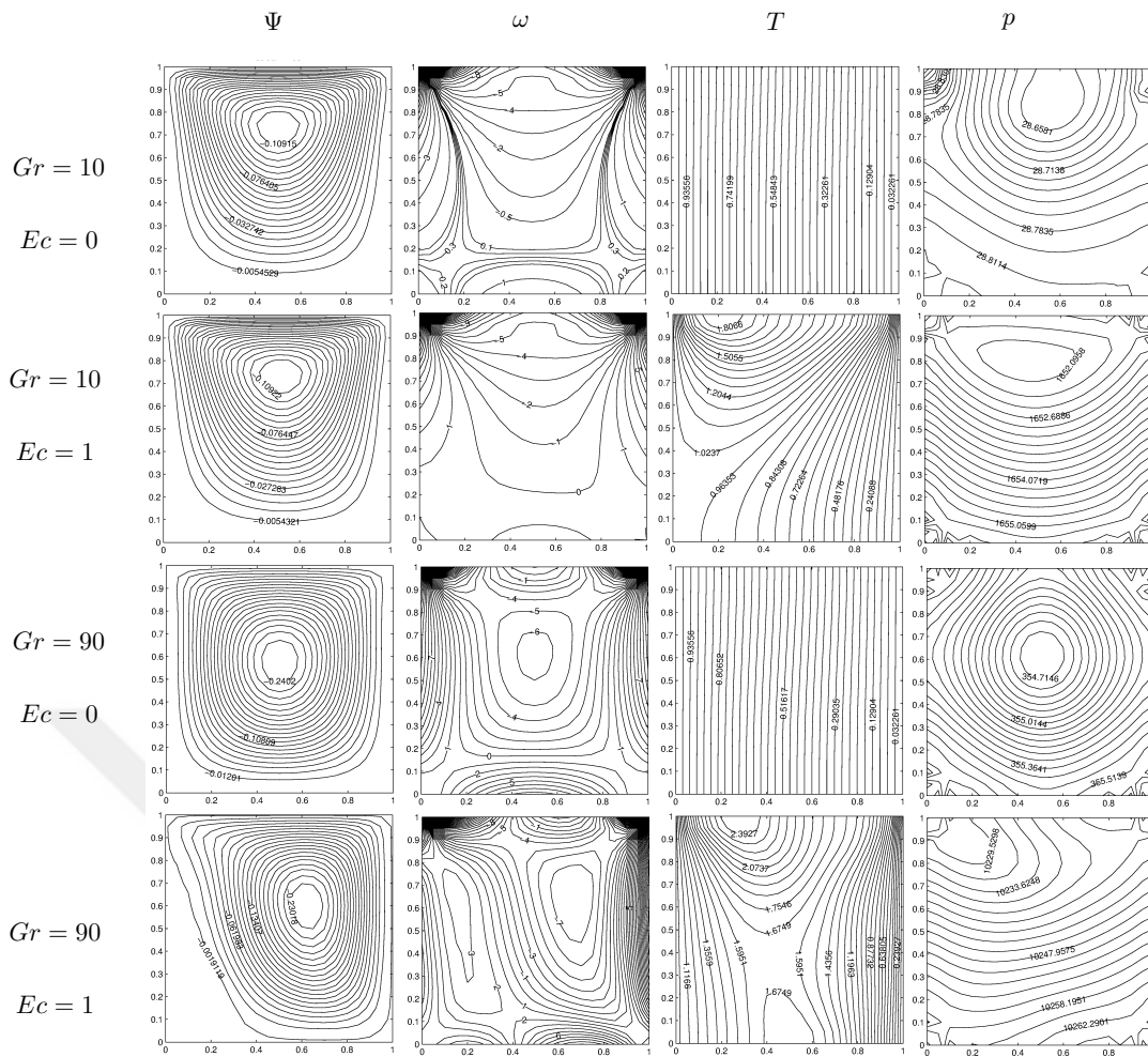
Figure 3.42: Problem 3.6.2: MHD convection Stokes flow for M = 0 .
