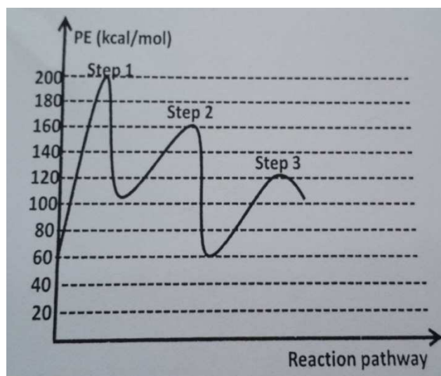
Figure 4.3 Potential energy vs reaction pathway graph
