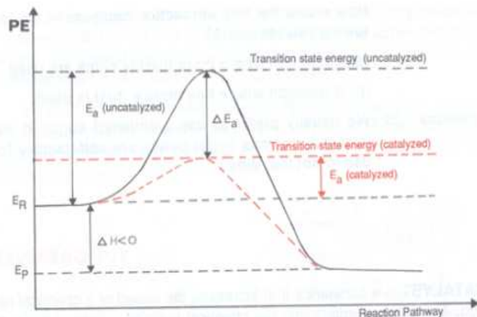
Figure 4.8 Energy profiles for a catalyzed and uncatalyzed reaction
