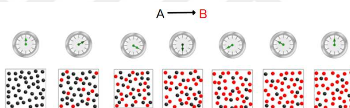
Figure 4.12 The reaction in which A is converted to B ( A \rightarrow B ) at sub-microscopic level
