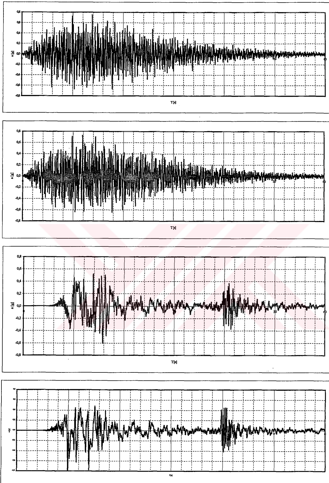
Figure 6-20 The Records SIMULATION 1, 2, YPT E-W and YPT N-S
