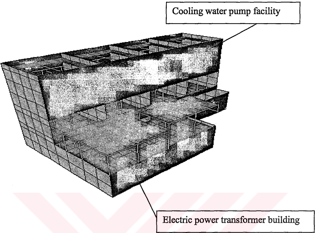
Figure 5-14 3-D View of the SAP2000 Model
