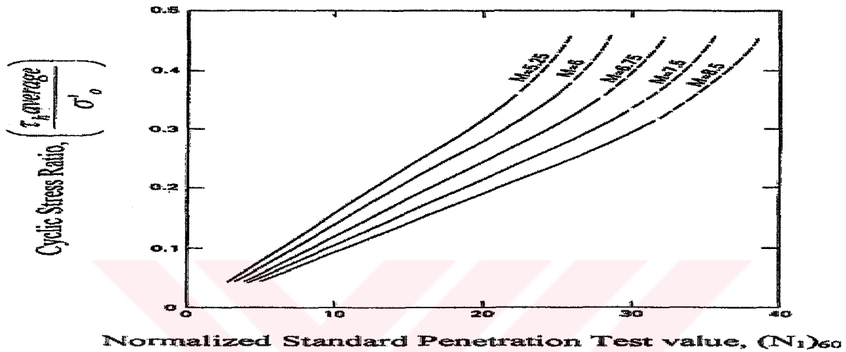
Figure 2-10 Seed & Idriss (1971) Curves for Various Values of Earthquake Magnitude The Curves Differ Very Little for the Same Value of Moment Magnitude
