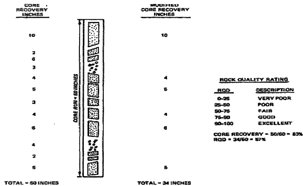
Figure 4-10 Illustration of RQD Sampling (U.S. Army Corps of Engineers, 1986)
