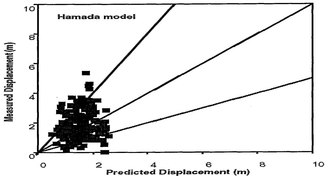
Figure 6-5 Hamada (1986) Model for Ground Slope
