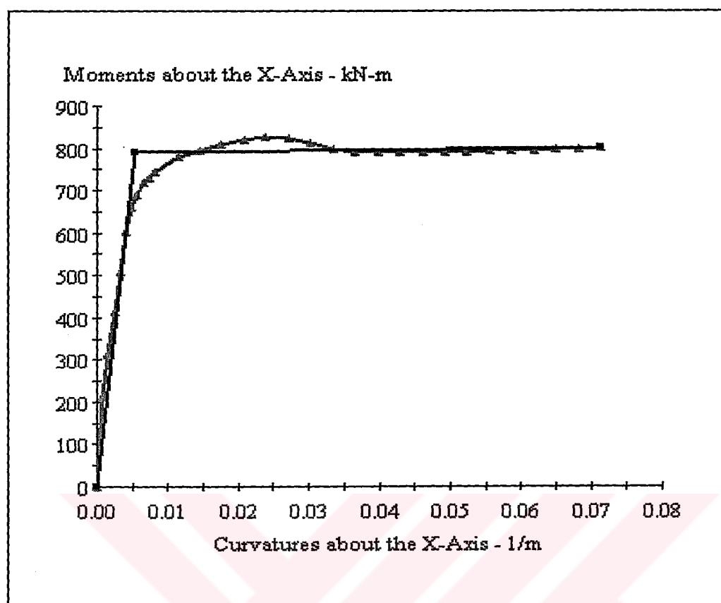
Figure 5-11 M-Kappa Diagram of the Middle Region
