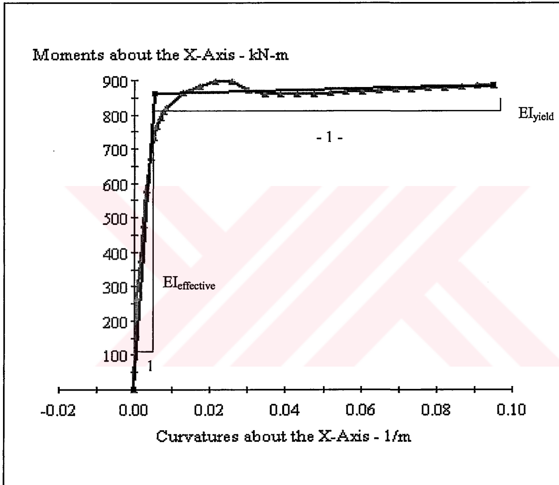
Figure 5-22 M- Kappa diagram of the hinge ( P(g) = 871 \text{ kN} )
