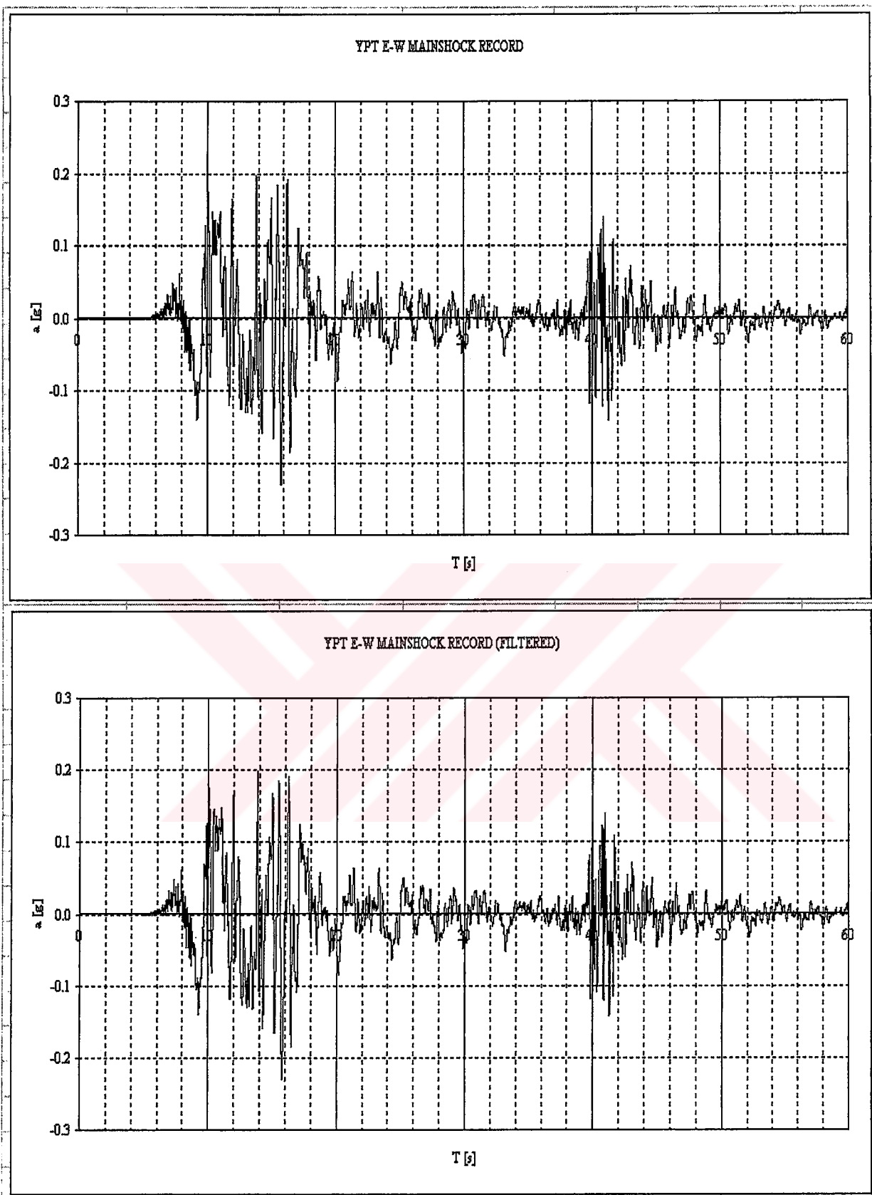
Figure 6-16 Before and After the Filtering of the Data YPT E-W (PGA = -0.23 g)
