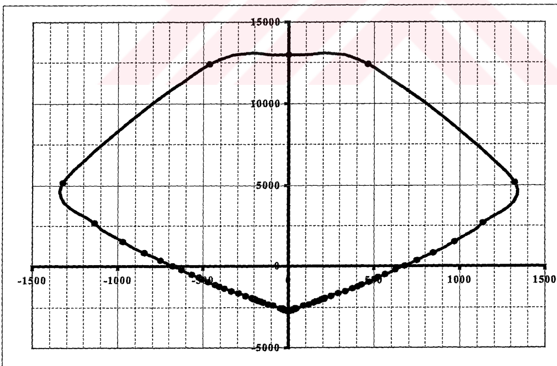
Figure 5-13 P-M Interaction Curve of the Middle Sections
