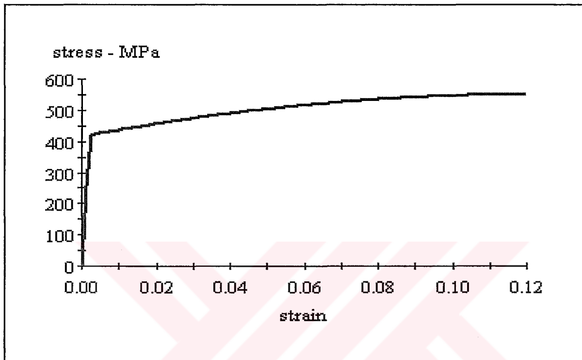
Figure 5-5 The Stress – Strain Diagram of the Steel
