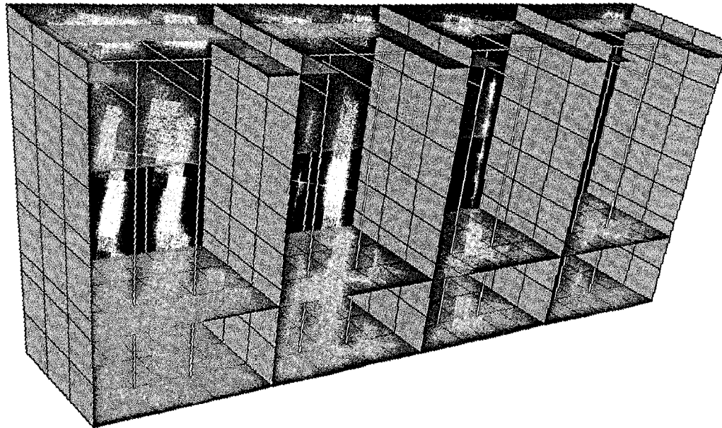
Figure 5-17 3-D Cross-Section of the Cooling Water Pump Facility
