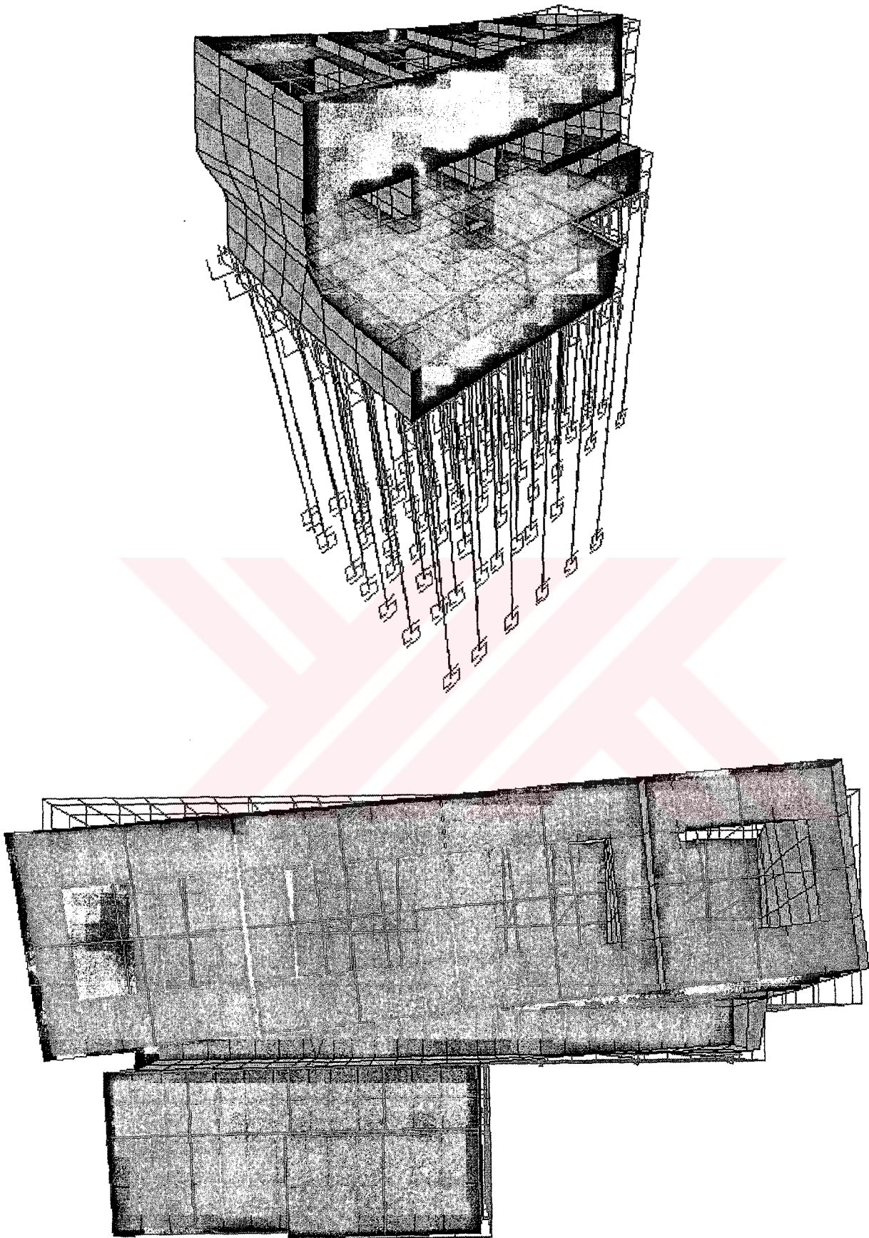
Figure 6-8 3 rd Mode, T = 0.26s , MPR = 7\% - 4\% - 0.16\% "U(X,Y,Z)"
