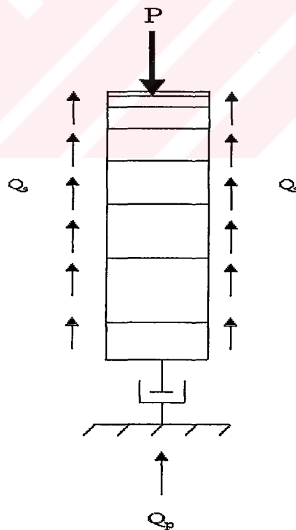
Figure 5-23 Illustration of Vertical Deformation of a Pile and Normal Force Hinge
