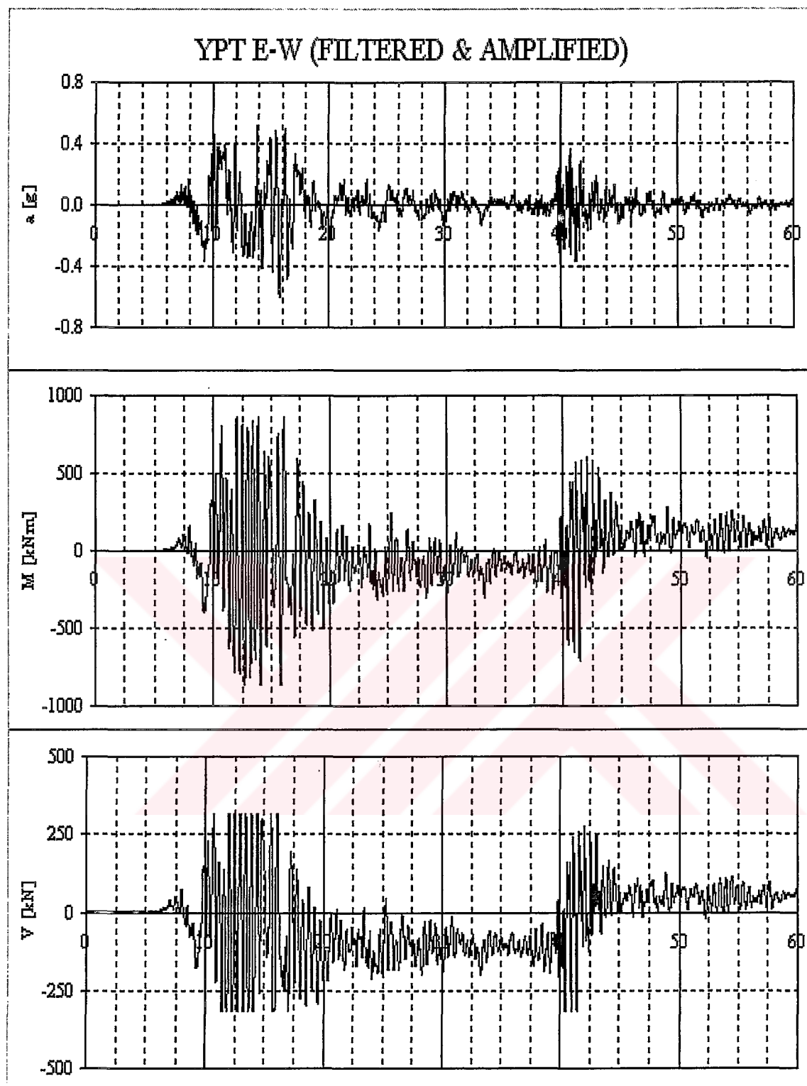
Figure 7-12 (1) YPT E-W (2) M33 (3) V22 (Element ID: 21)
