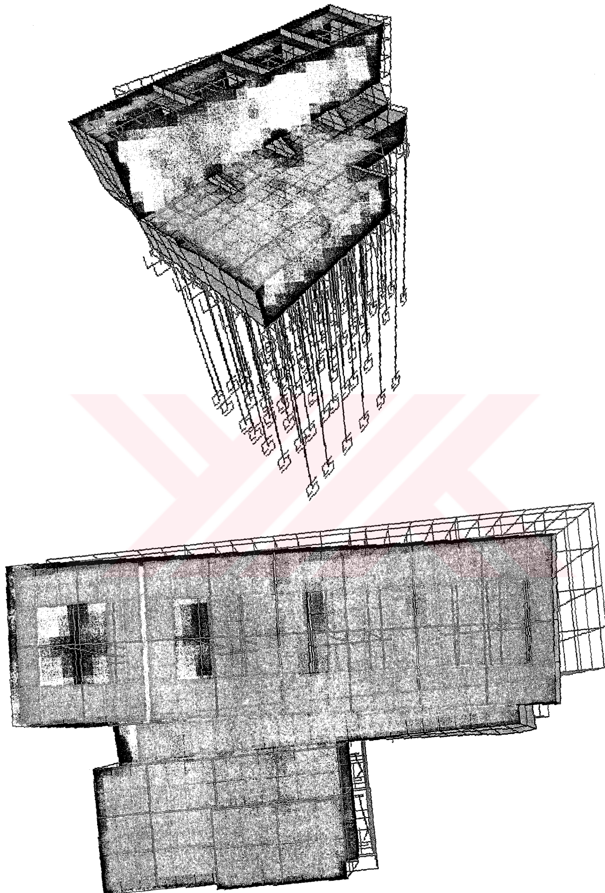
Figure 6-7 2 nd Mode, T = 0.49s , MPR = \%52 - \%3 - \%0.15 "U(X,Y,Z)"
