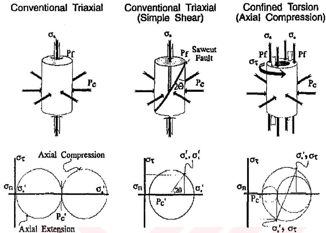
Figure 4-8 Tests of Conventional Triaxial, Simple Shear and Confined Torsion
