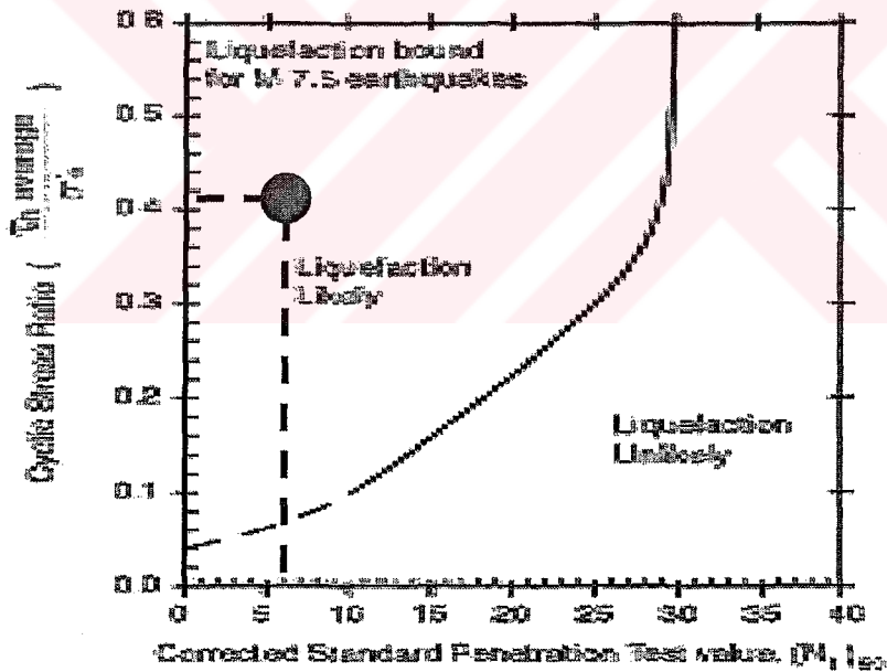
Figure 5-27 Liquefaction Pot. Anly. According to the Empirical Evaluation Method of Seed
