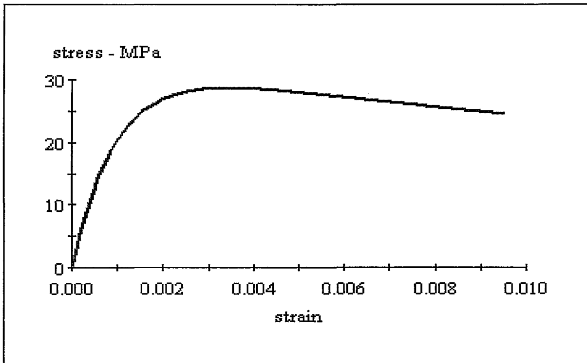
Figure 5-7 The Stress – Strain Diagram of the Confined Concrete (Mid Region)
