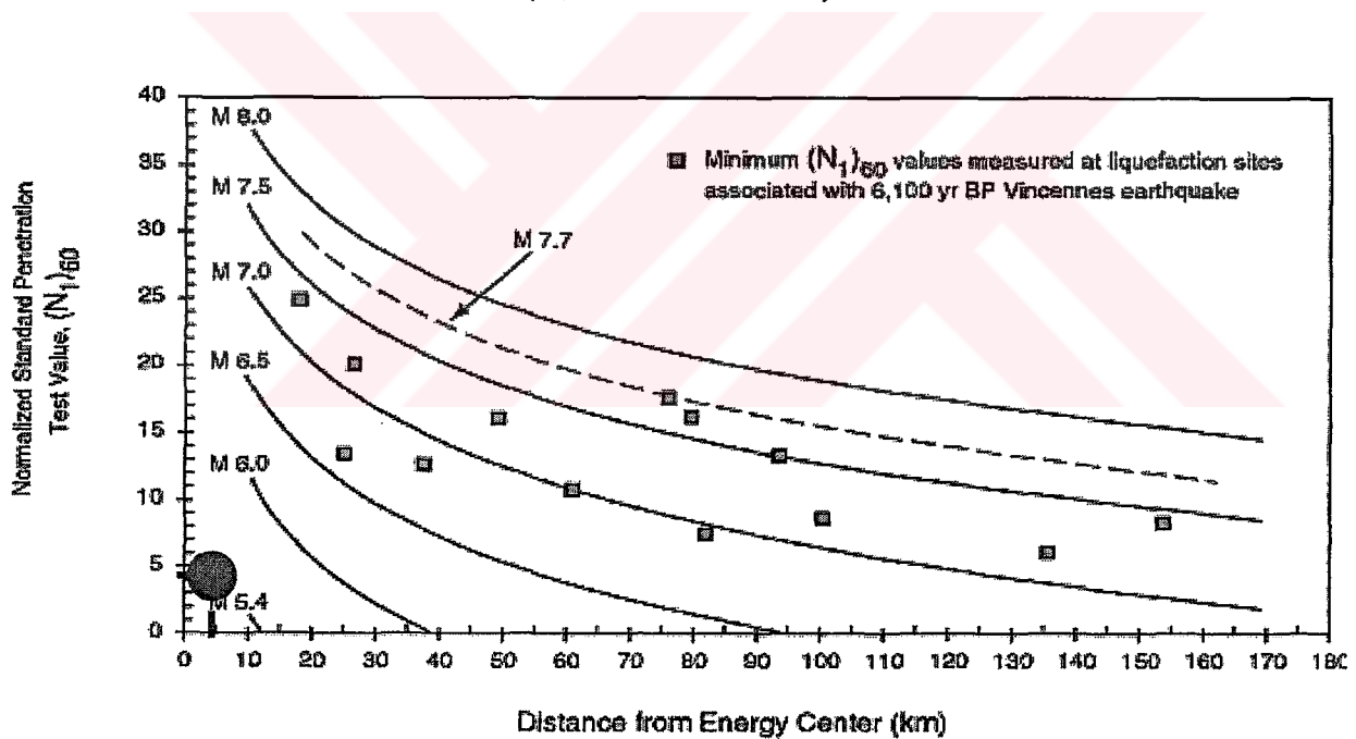
Figure 5-29 Minimum Field-Measured Values of Normalized SPT N_{60} as a Function of R
