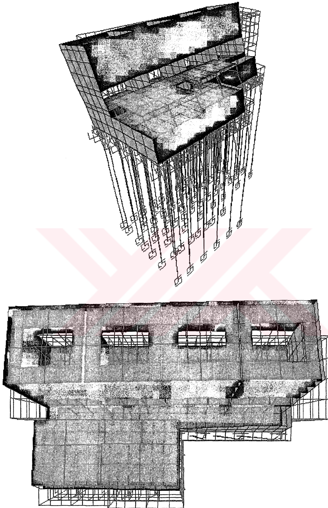
Figure 6-6 1 st Mode, T = 0.53s , MPR = 2 - 49 - 0.01 "U(X,Y,Z)"
