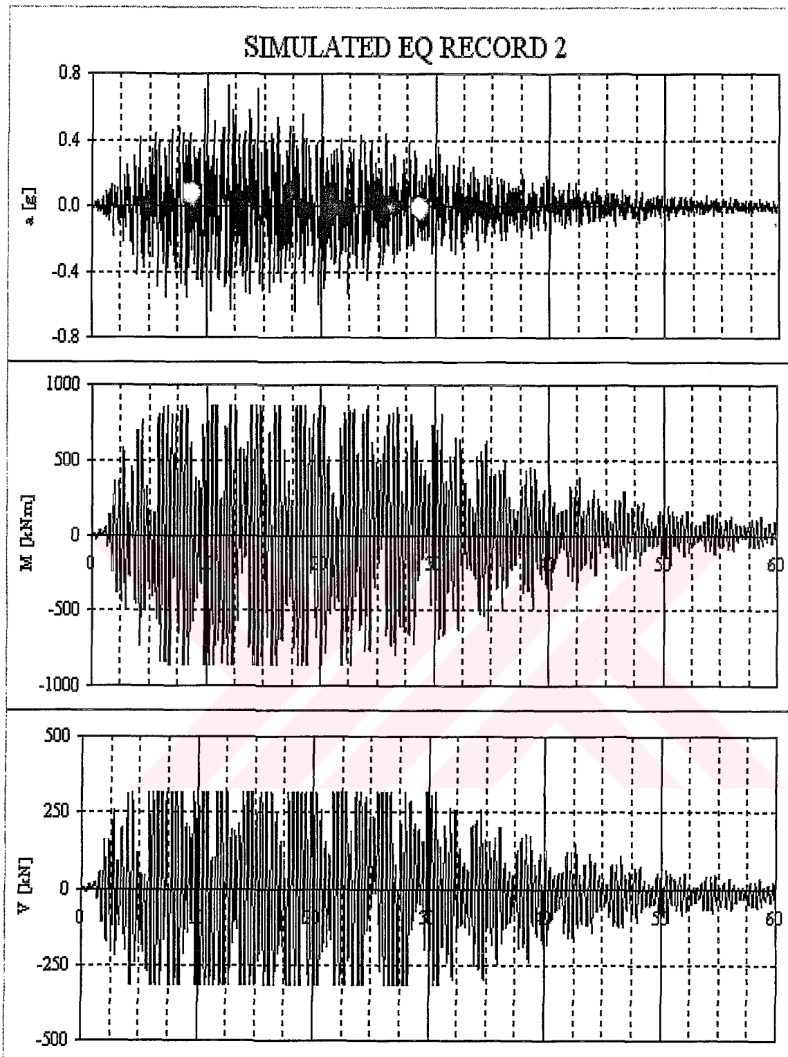
Figure 7-11 (1) Simulated Earthquake 2 (2) M33 (3) V22 (Element ID: 18)
