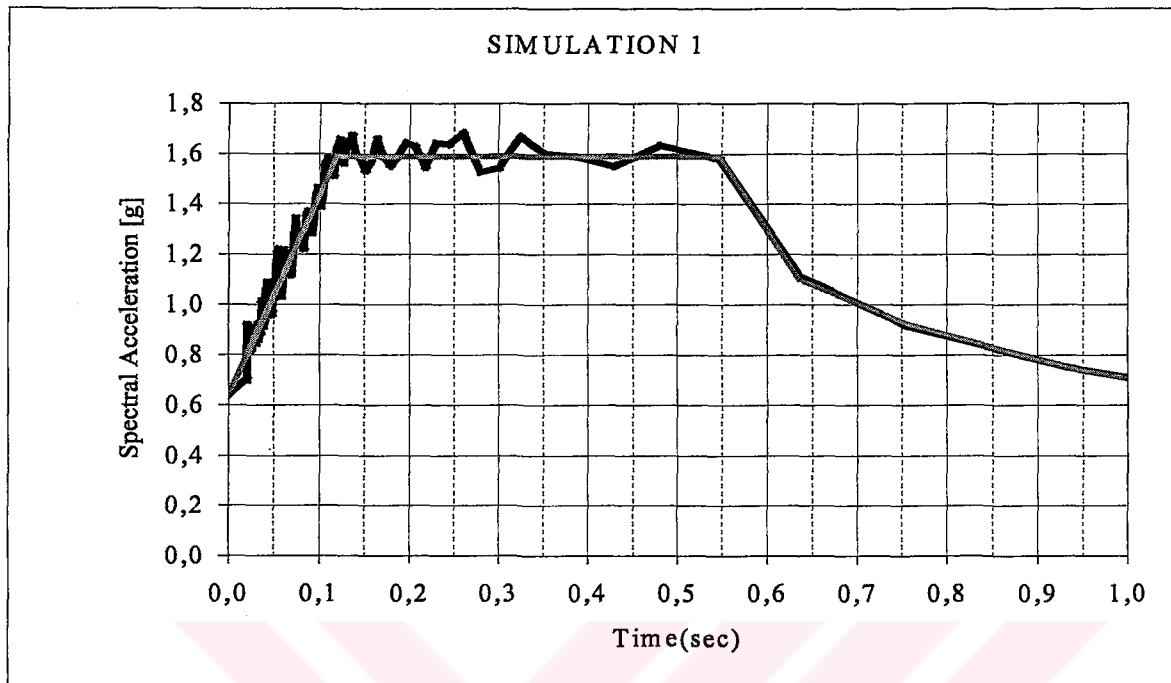
Figure 6-13 The Target and the Simulated SPA 1
