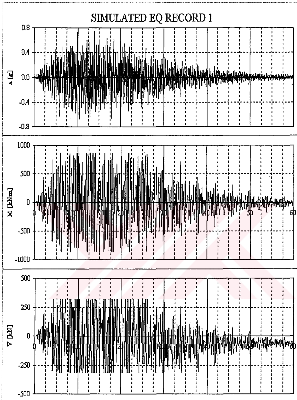
Figure 7-9 (1) Simulated Earthquake 1 (2) M33 (3) V22 (Element ID: 18)
