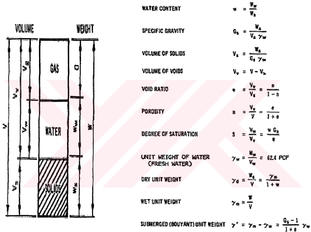
Figure 4-3 Weight - Volume relationships (U.S. Army Corps of Engineers, 1986)
