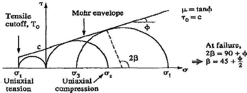
Figure 4-6 Mohr – Coulomb Failure Criterion
