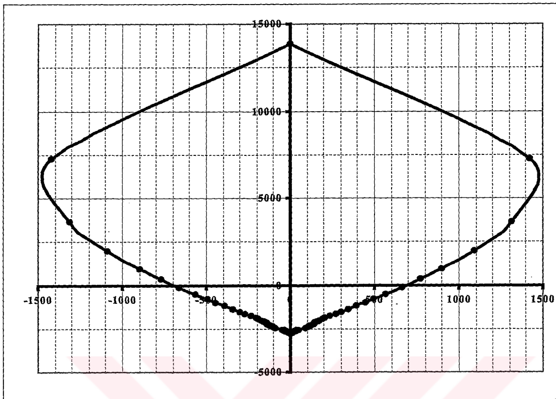
Figure 5-12 P-M Interaction Curve of the Confinement Zones
