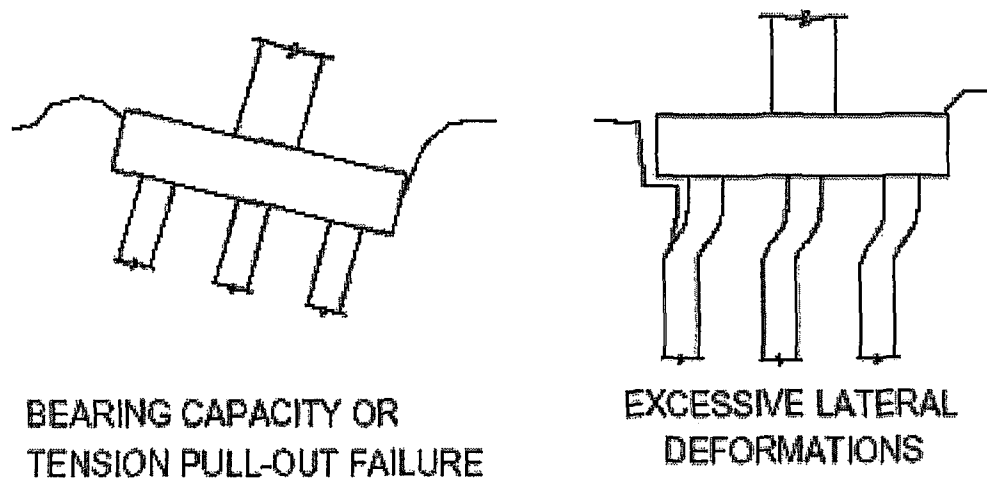
Figure 3-1 Failure Types of Pile Groups Subjected to Seismic Loading
