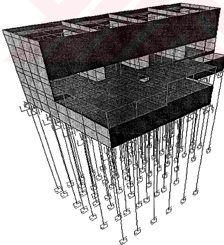
Figure 5-26 The 3-D View of the Entire Structure
