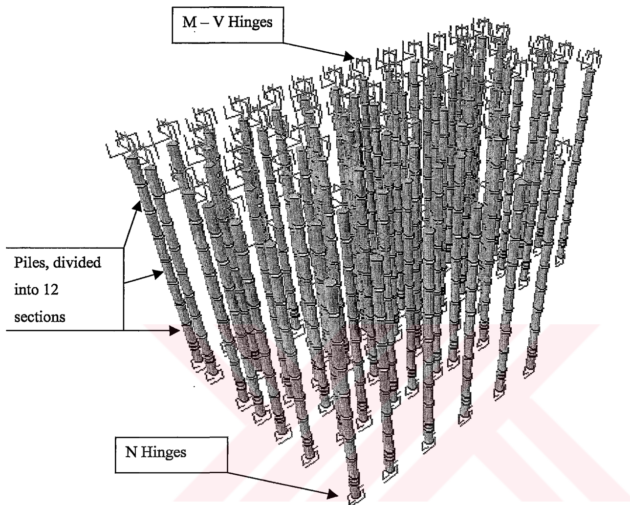
Figure 5-24 3-D View of the Substructure (77 x 12)
