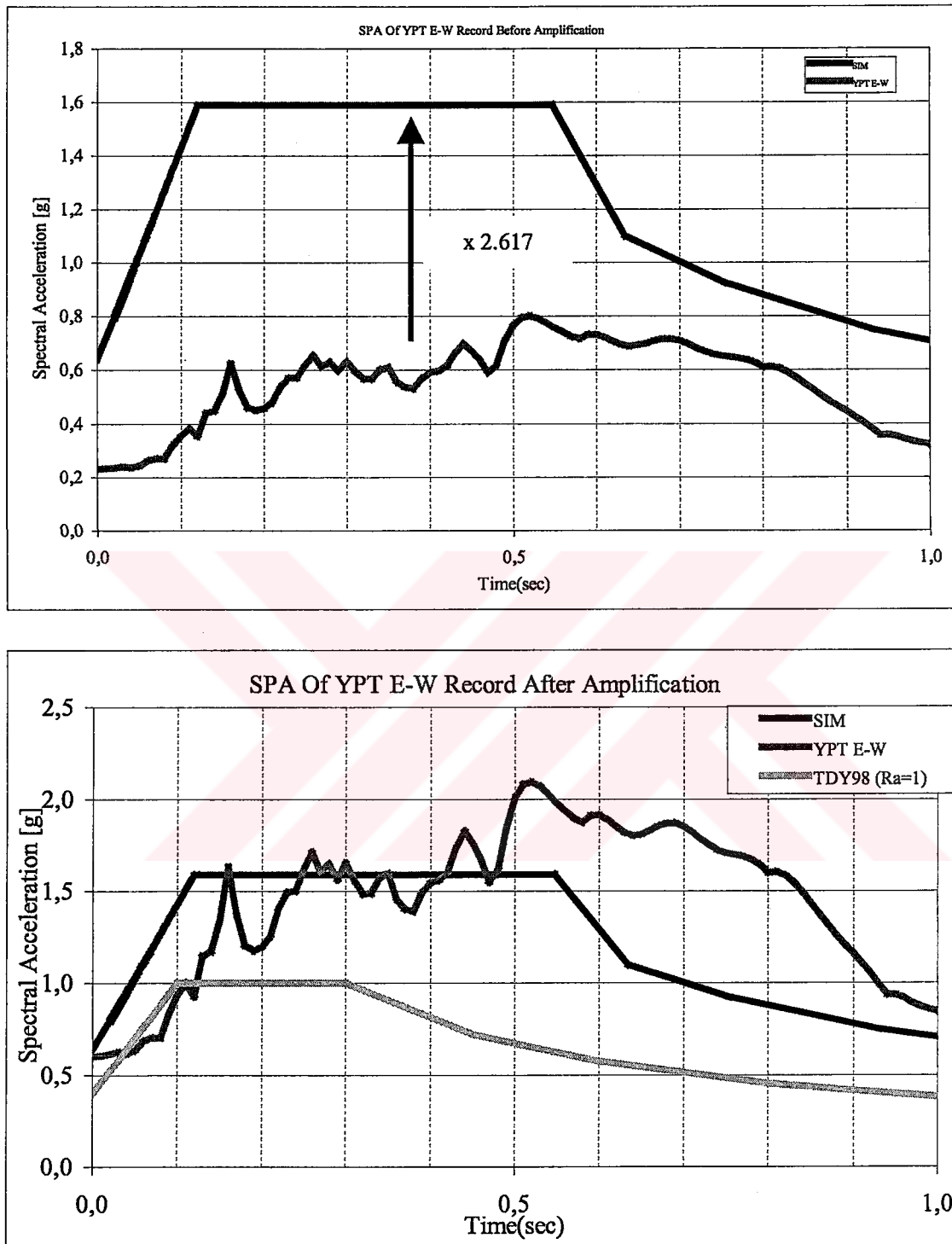
Figure 6-18 Before & After the Amplification (x2.617) of SPA of YPT E-W Data
