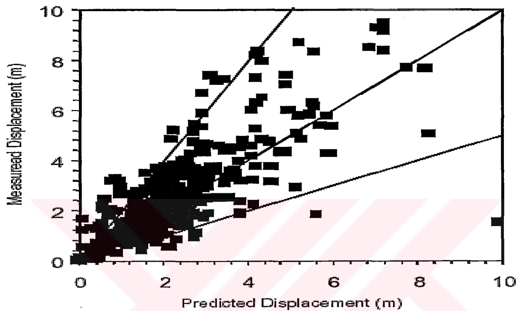
Figure 6-3 MLR Model
