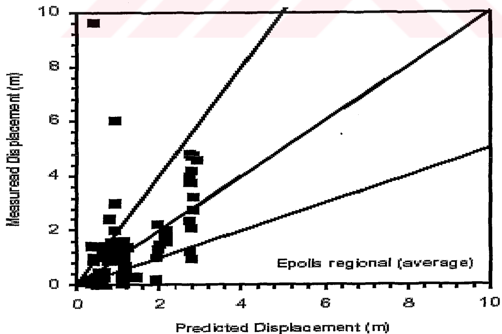
Figure 6-4 Rauch Model
