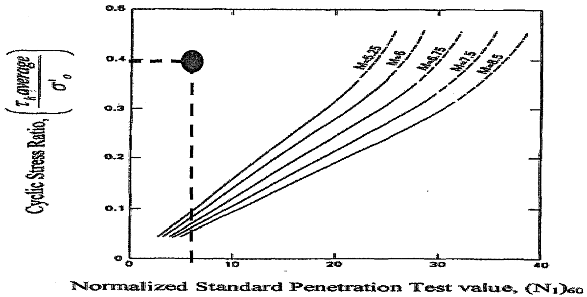
Figure 5-28 Seed & Idriss (1983-1985) Curves for CSR & Various Values of M_w
