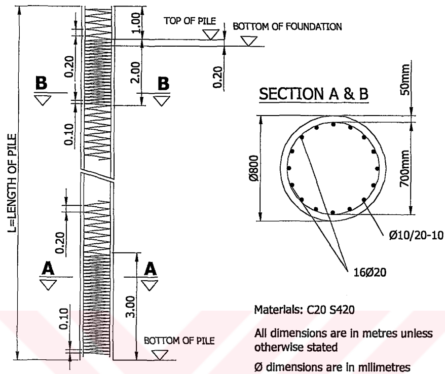
Figure 5-1 Reinforcement Details of the Piles
