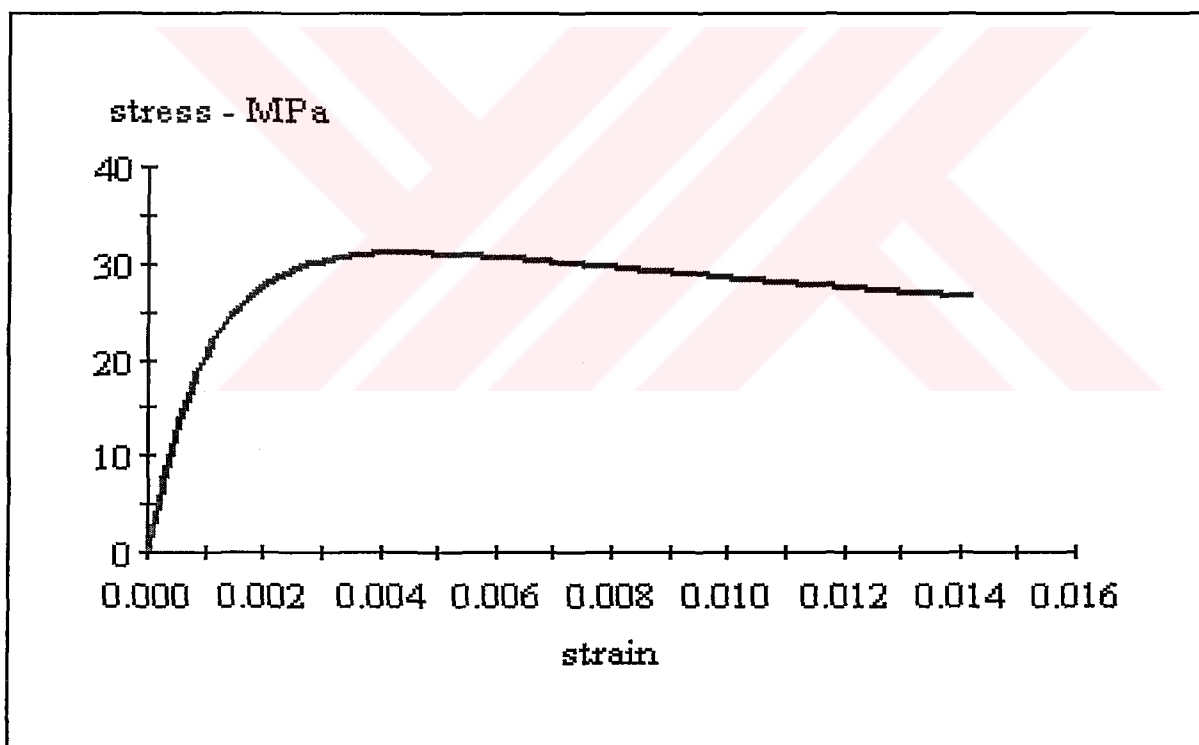
Figure 5-6 The Stress – Strain Diagram of the Confined Concrete (Confinement Zone)
