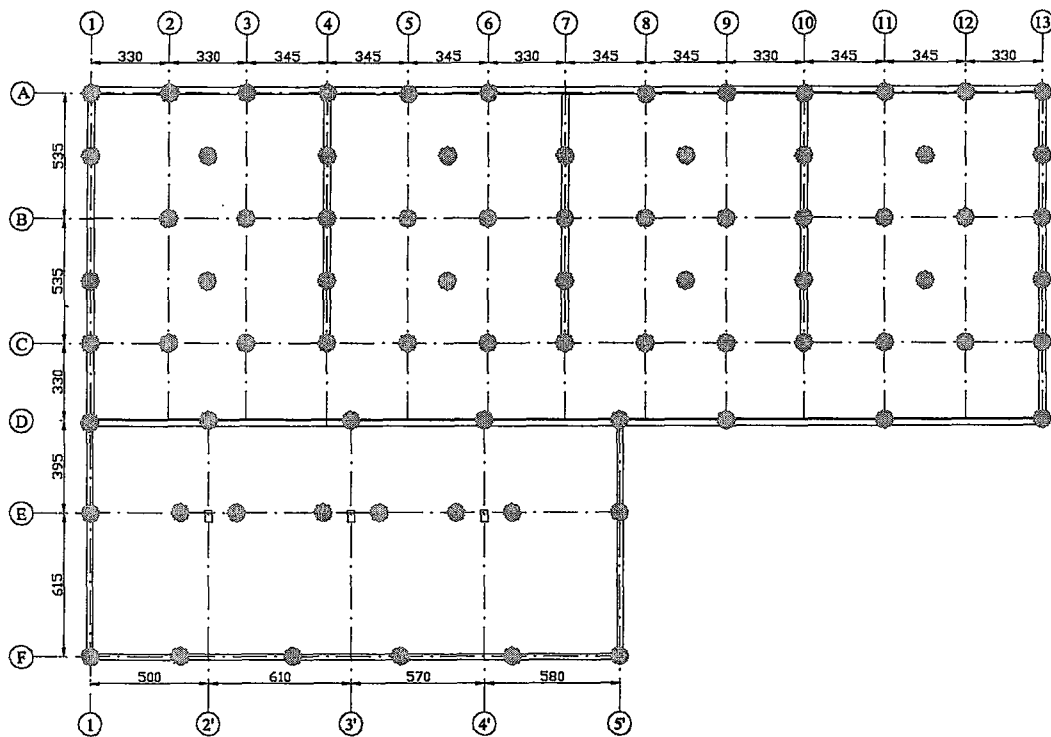
Figure 5-3 Plan View of the Pile Applications
