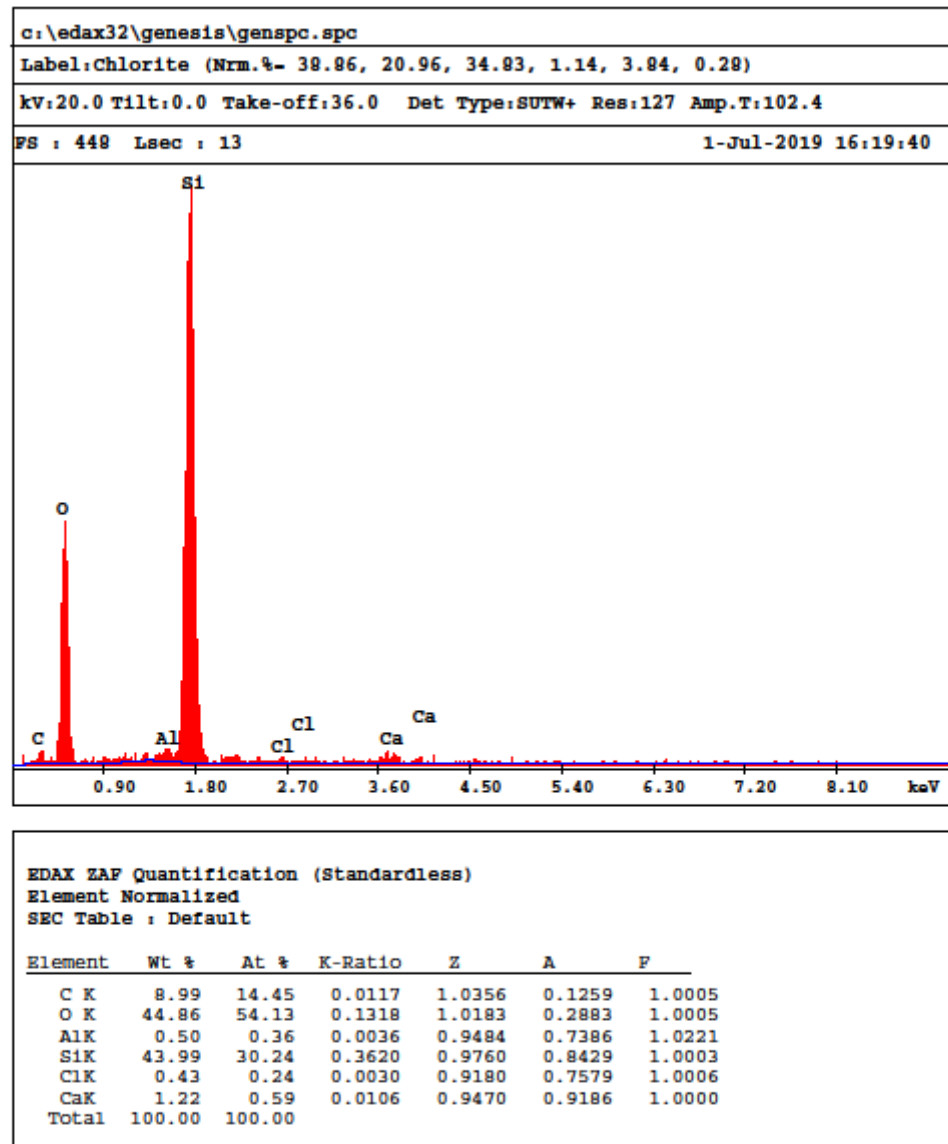
Figure 4.20. Element profile of sand grains taken from sample treated without bacteria introduction
