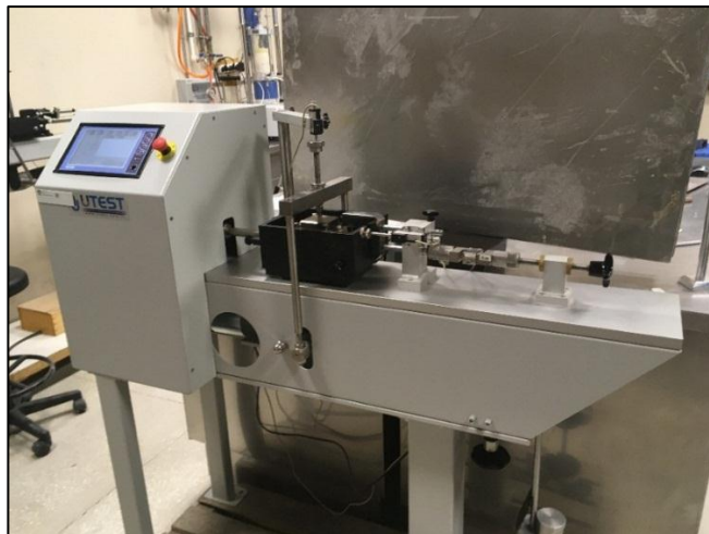
Figure 3.11. Direct shear test setup
