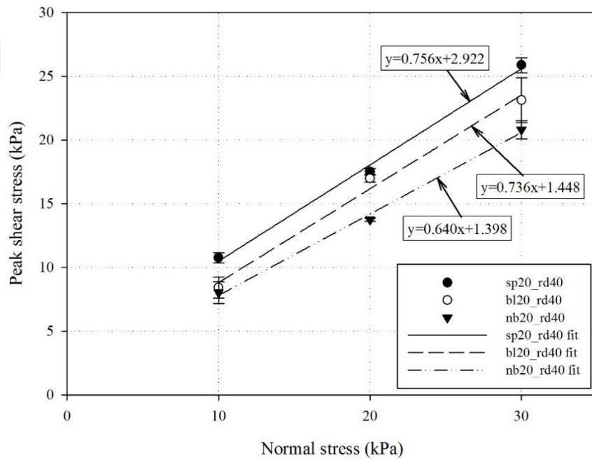
Figure 4.4. Effect of bacteria on friction angle and cohesion of sand prepared at a relative density of 40% and treated with 20 injections of cementation solution
