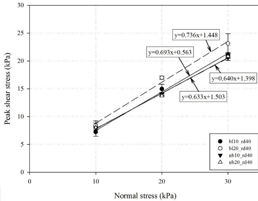
Figure 4.11. Effect of the number of injections of cementation solution of friction angle and cohesion of sand prepared at a relative density of 40% and treated using Bacillus licheniformis
