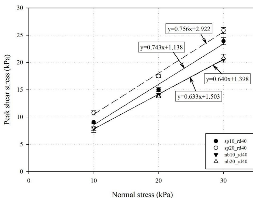
Figure 4.10. Effect of the number of injections of cementation solution of friction angle and cohesion of sand prepared at a relative density of 40% and treated using Sporosarcina pasteurii
