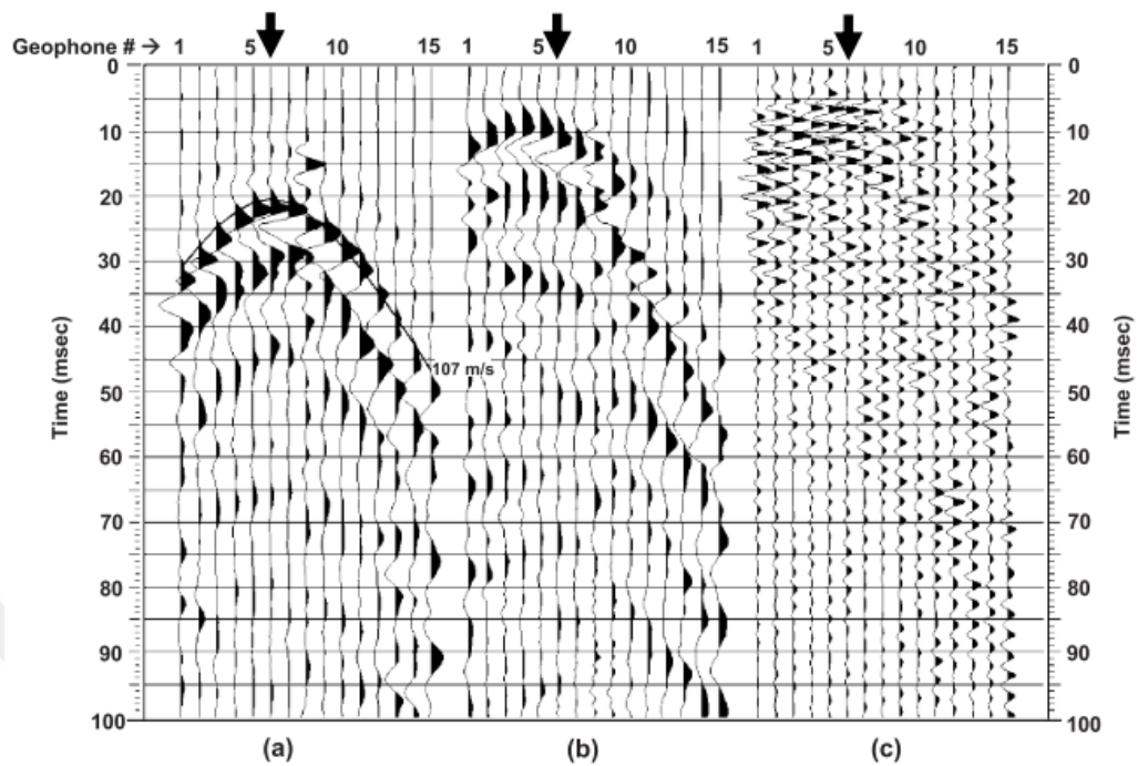
Figure 2.9. Shear wave data (a) before treatment, (b) after 1 day of injection, (c) at the end of the treatment process (van Paassen et al., 2010)
