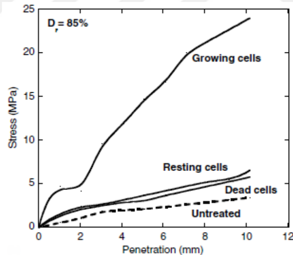
Figure 2.2. Effect of living state of microorganism on California Bearing Ratio Test results (Chou et al., 2011)
