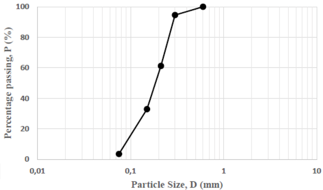
Figure 3.1. The grain size distribution of the sand (Ahmadi-Adli, 2014)
