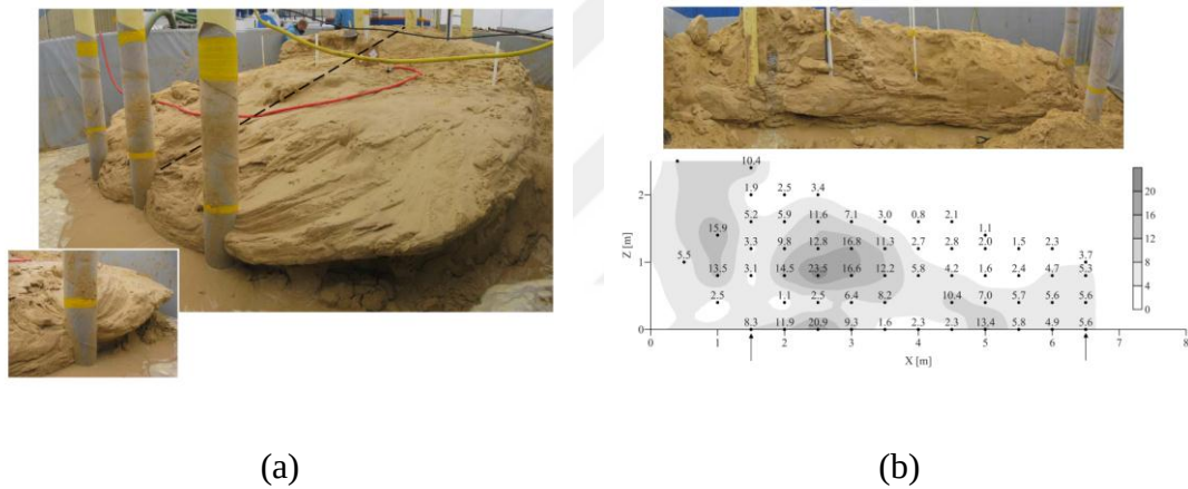
Figure 2.7. (a) the cemented sand body, (b) CaCO 3 content along the vertical cross-section passes through the middle of the cemented body (van Paassen et al., 2010)
