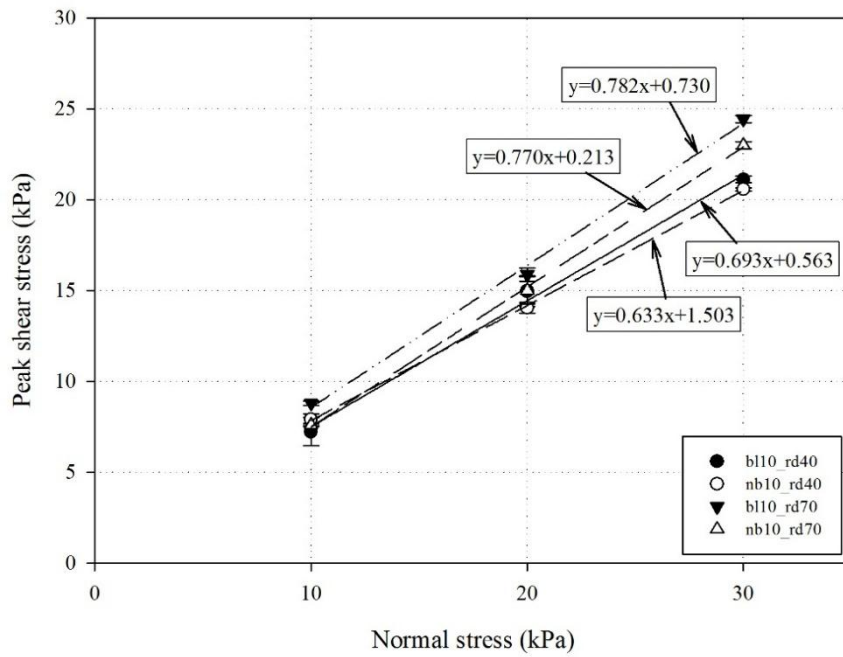
Figure 4.7. Effect of relative density on friction angle and cohesion of sand treated using Bacillus licheniformis and with the application of 10 injections of cementation solution
