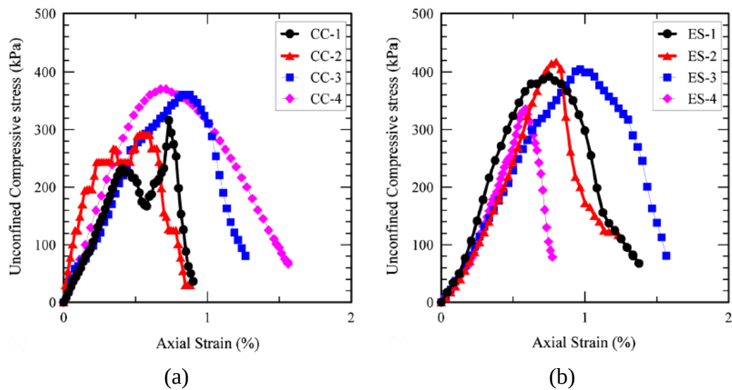
Figure 2.4. Unconfined compression strength test results of soils treated using (a) calcium chloride, (b) eggshell as calcium source (Choi et al., 2016)
