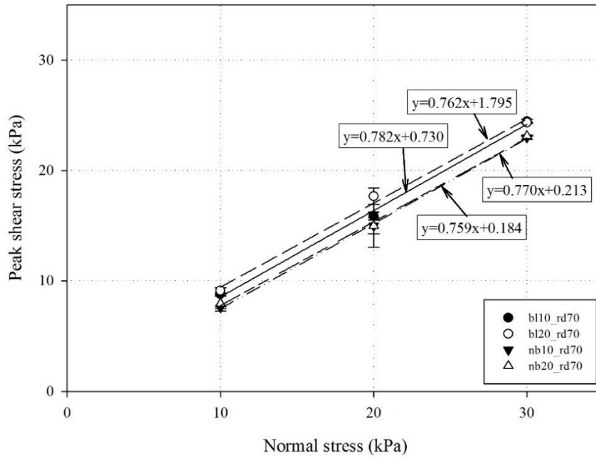
Figure 4.13. Effect of the number of injections of cementation solution of friction angle and cohesion of sand prepared at a relative density of 70% and treated using Bacillus licheniformis
