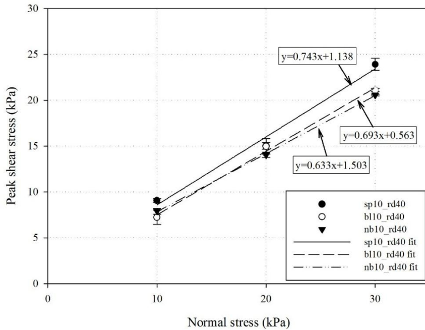
Figure 4.2. Effect of bacteria on friction angle and cohesion of sand prepared at a relative density of 40% and treated with 10 injections of cementation solution
