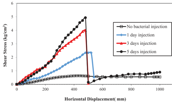
Figure 2.17. Effect of injection duration on shear strength (Cheshomi et al., 2018)
