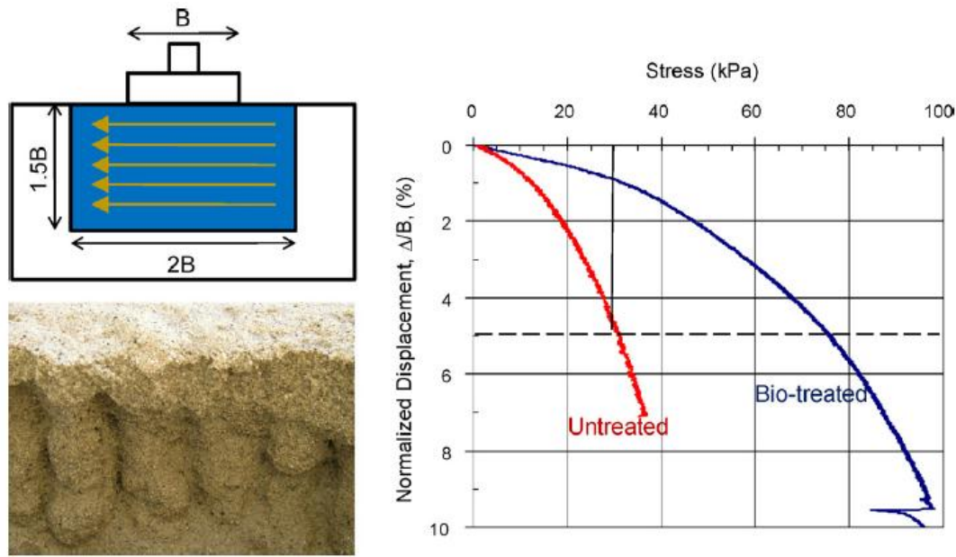
Figure 2.12. Results of bio-treatment experiments under a shallow foundation model (Martinez and DeJong, 2009)
