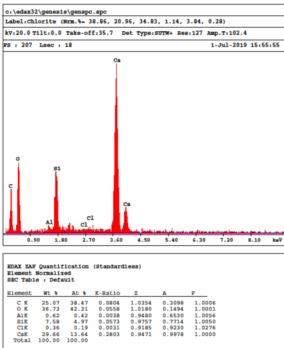
Figure 4.21. Element profile of sand grains taken from sample treated with Sporosarcina pasteurii
