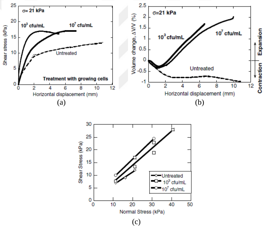
Figure 2.14. Direct shear test results for untreated and bio-treated sands (Chou et al., 2011)
