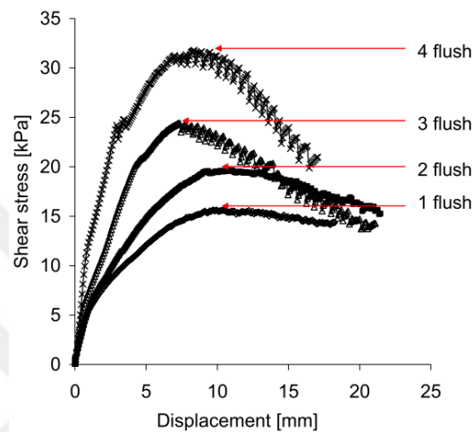
Figure 2.15. Correlation between shear strength and number of flushes obtained from treatment on gravel (van Paassen, 2011)
