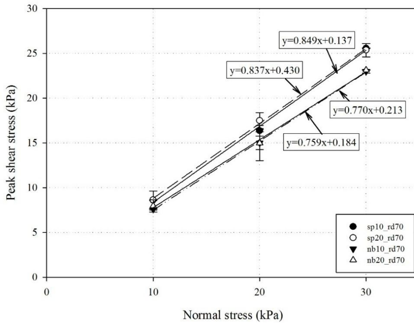
Figure 4.12. Effect of the number of injections of cementation solution of friction angle and cohesion of sand prepared at a relative density of 70% and treated using Sporosarcina pasteurii
