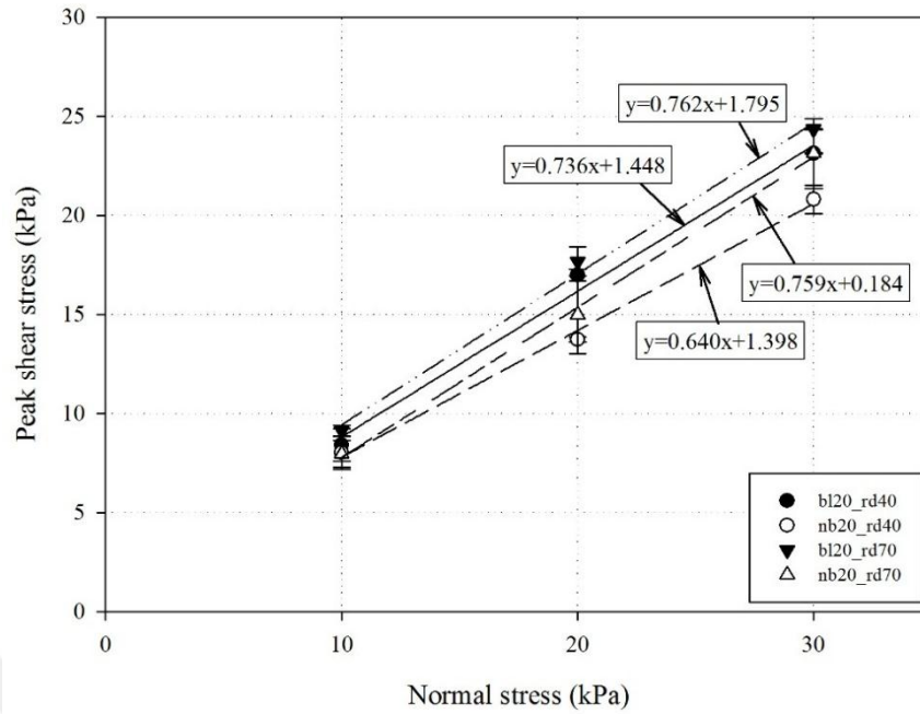
Figure 4.9. Effect of relative density on friction angle and cohesion of sand treated using Bacillus licheniformis and with the application of 20 injections of cementation solution
