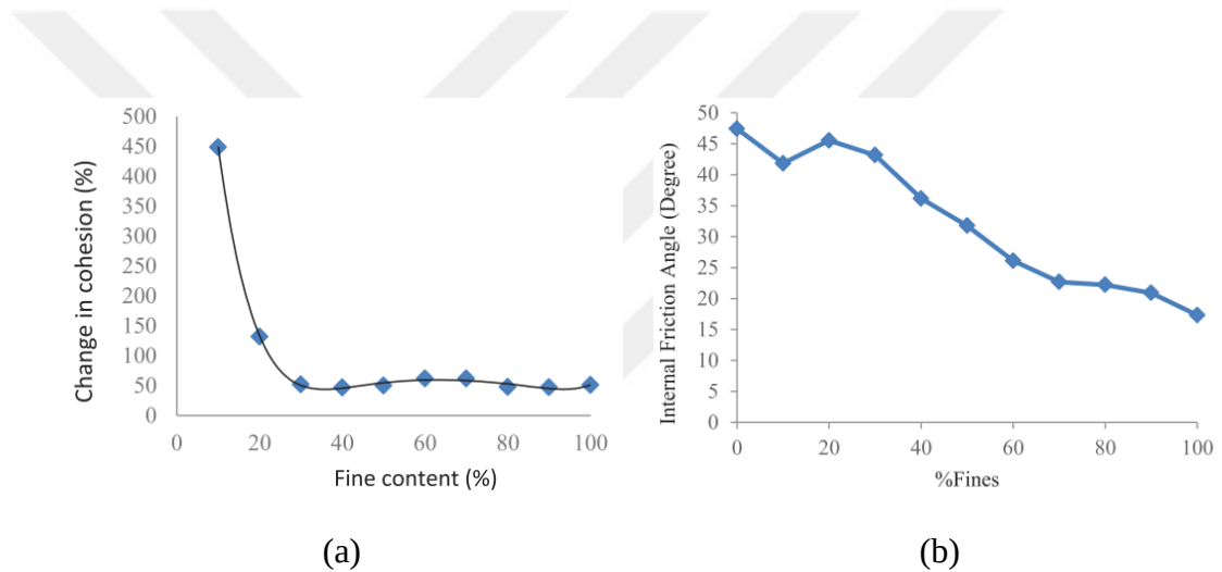
Figure 2.16. Change of (a) cohesion, (b) internal friction angle of treated soil with respect to fines content (Hataf and Jamali, 2018)
