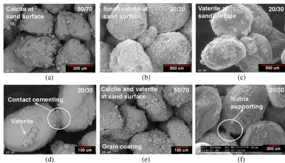
Figure 2.8. Scanning Electron Microscopy images showing examples of distribution alternatives and different \text{CaCO}_3 morphologies (Lin et al., 2016)
