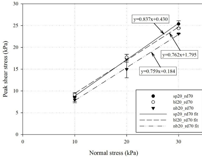
Figure 4.5. Effect of bacteria on friction angle and cohesion of sand prepared at a relative density of 70% and treated with 20 injections of cementation solution
