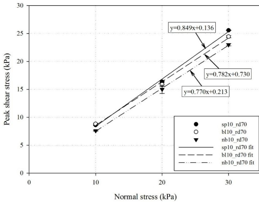
Figure 4.3. Effect of bacteria on friction angle and cohesion of sand prepared at a relative density of 70% and treated with 10 injections of cementation solution
