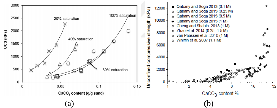
Figure 2.13. (a) Unconfined compressive strength variation of samples having different saturation degrees (Cheng et al., 2013), (b) relation between \text{CaCO}_3 content and unconfined compressive strength (Wang et al., 2017)
