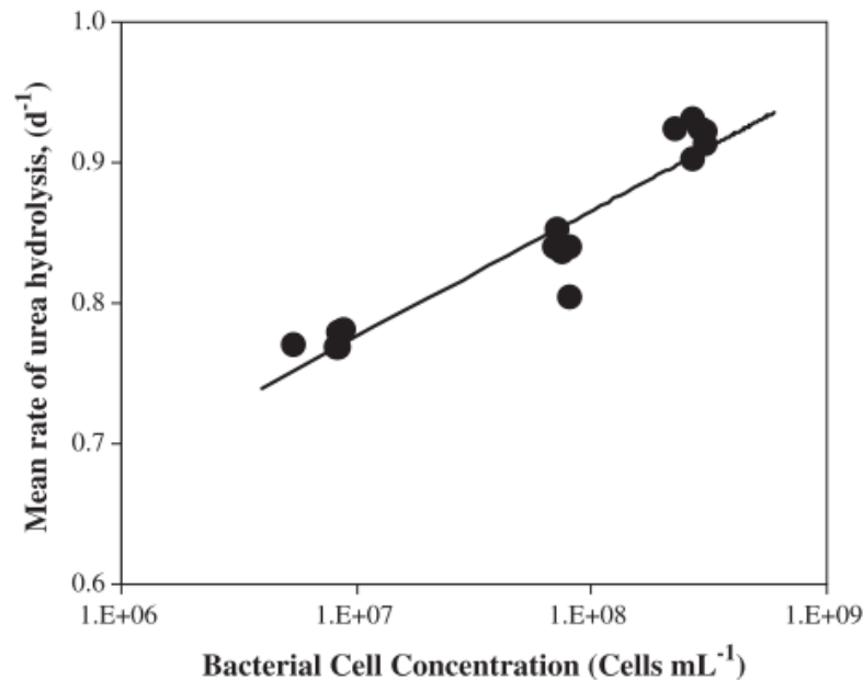
Figure 2.5. The relation between bacterial cell concentration and the mean rate of urea hydrolysis (Okwadha and Li, 2010)
