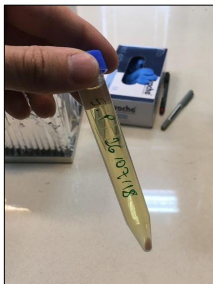
Figure 3.2. (a) pouring ammonium-yeast extract into the flasks, (b) inoculation of Bacillus licheniformis from stock culture, (c) orbital shaker equipment, (d) centrifugation stage, (e) bacterial pellet at the bottom of the tube after centrifugation
