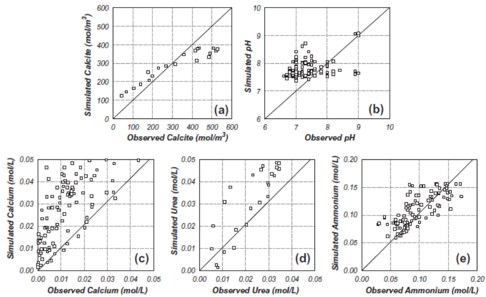
Figure 2.6. Simulated vs observed data (Martinez et al., 2014)
