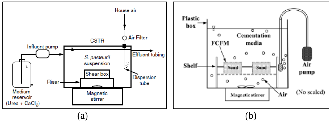
Figure 3.4. Schematic drawings of the system used to prepare direct shear specimens by (a) Chou et al. (2011), (b) Zhao et al. (2014)
