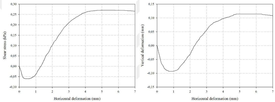
Figure A.5. (a) Horizontal deformation versus shear stress, (b) horizontal deformation versus vertical deformation relationships under 20 kPa normal stress of sand prepared at relative density of 40% and treated with Sporosarcina pasteurii through 10 injections
