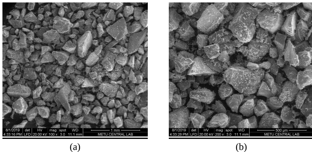
Figure 4.14. Scanning electron microscopy micrographs of sand sample prepared at a relative density of 40% and treated without bacteria introduction through 10 injections (a) 100x; (b) 200x
