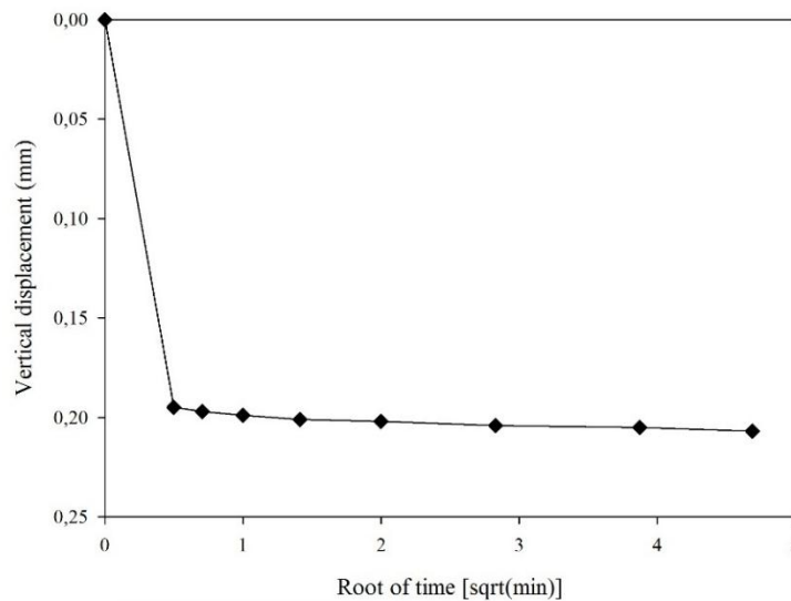
Figure 3.12. Typical root time versus vertical displacement plot of treated specimens
