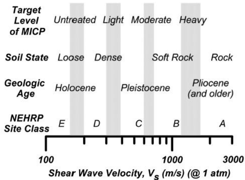
Figure 2.10. The relation between the level of cementation and shear wave velocity (Montoya and DeJong, 2015)
