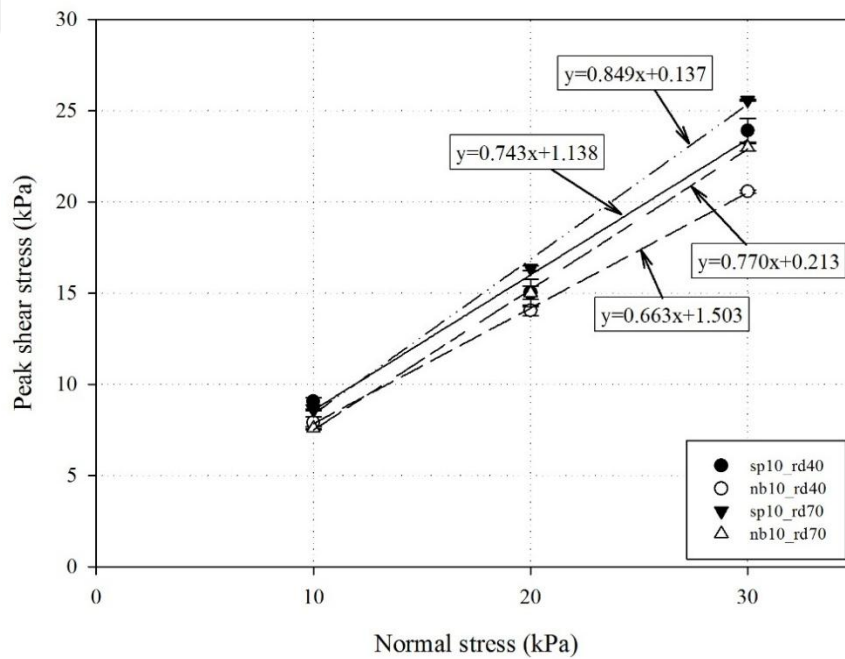
Figure 4.6. Effect of relative density on friction angle and cohesion of sand treated using Sporosarcina pasteurii and with the application of 10 injections of cementation solution
