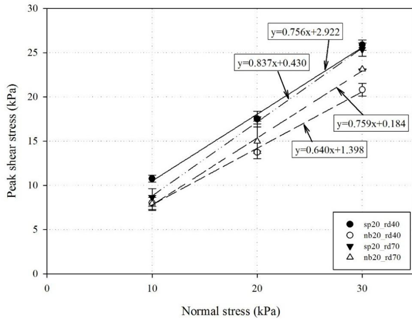
Figure 4.8. Effect of relative density on friction angle and cohesion of sand treated using Sporosarcina pasteurii and with the application of 20 injections of cementation solution
