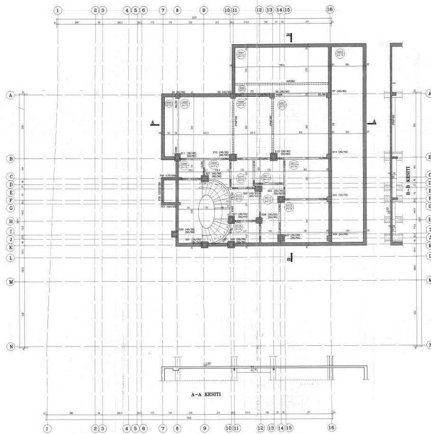
(a) partial basement floor (-3.85)
