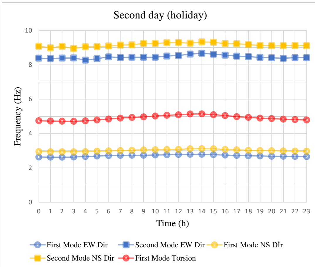
Figure 4.10. Hourly variation of frequencies (29/04/2017)
