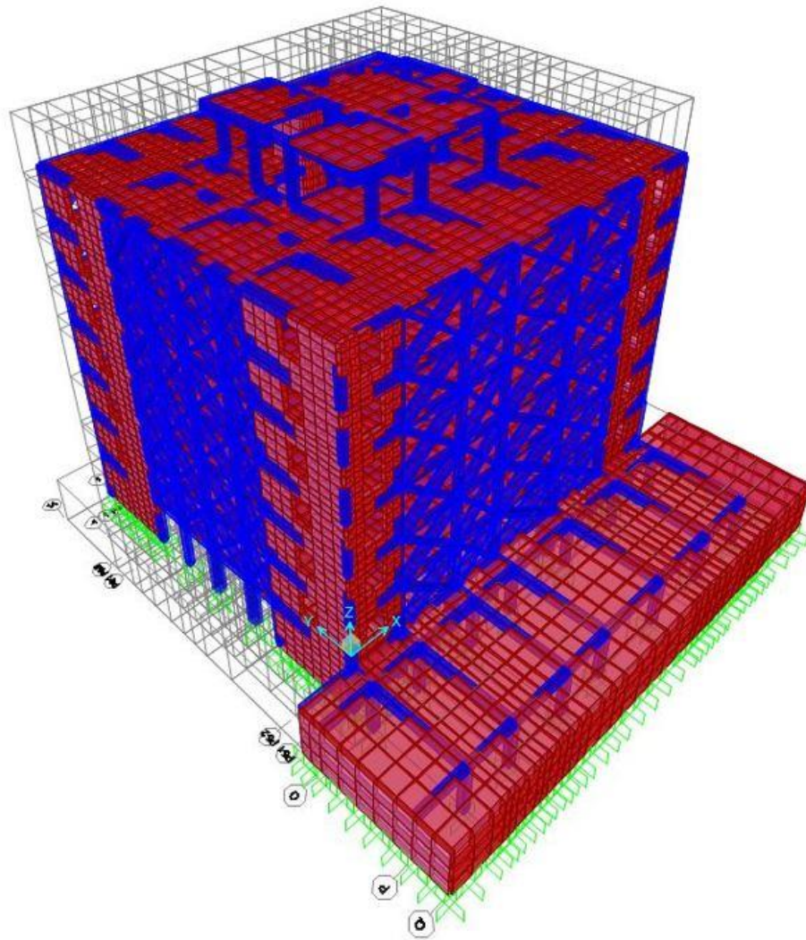
Figure 4.15. Finite element model with strut members
