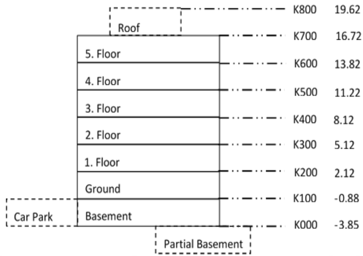
Figure 3.2. Floor labels and elevations (in m)
