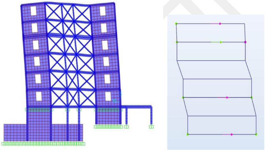
(b) Second mode
