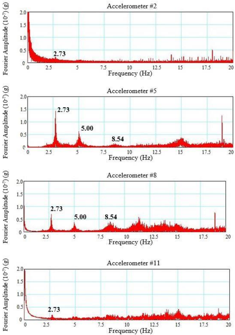
Figure 4.2. Fourier amplitude spectra for the EW direction (continued)
