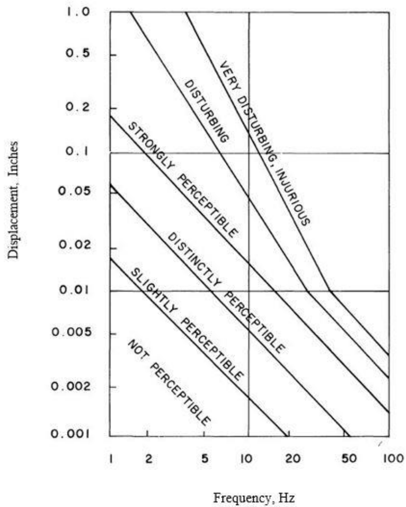
Figure 2.1. Modified Reiher-Meister Scale (Lenzen, 1966)
