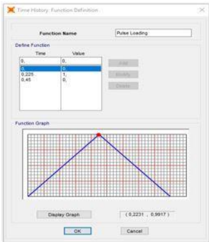
Figure 5.7. Pulse loading (for every footstep (0.75m every 0.5s))
