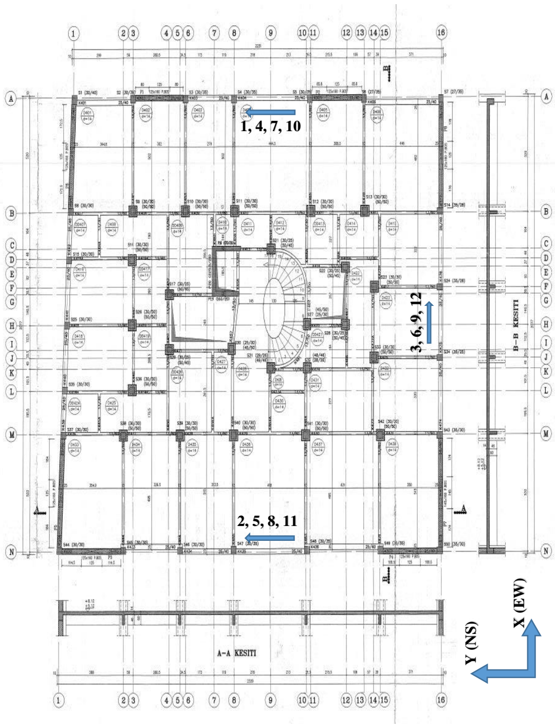
Figure 3.6. Instrumentation scheme and the location of the accelerometers on the plan
