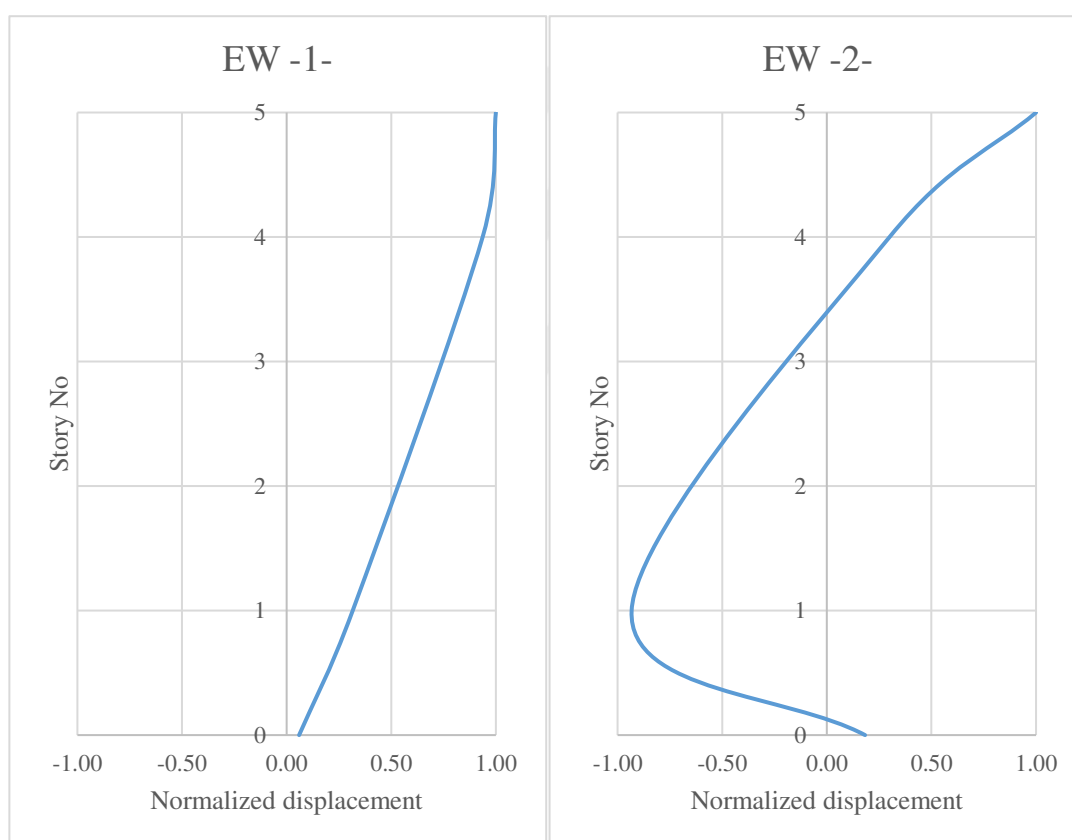
Figure 4.5. The first and second translational mode shapes for the EW direction
