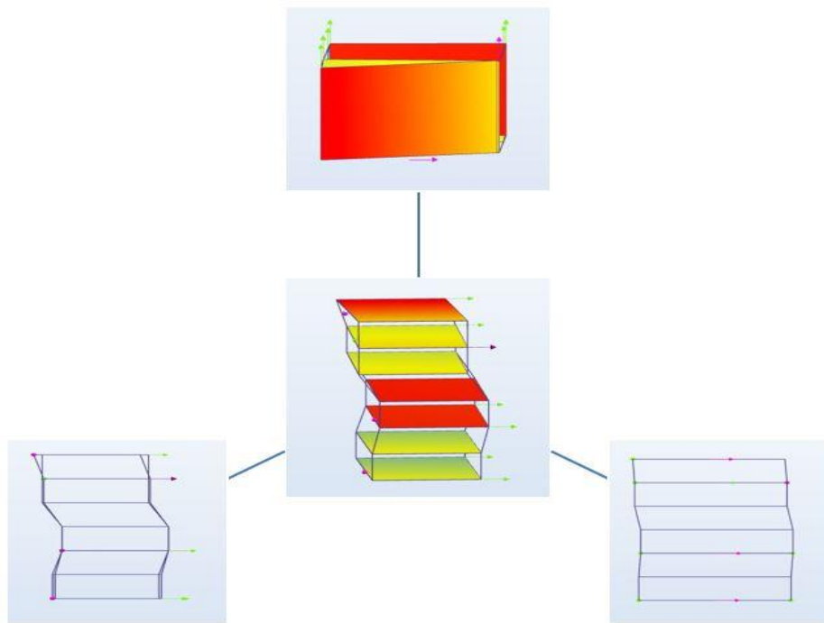
(c) Second translational mode in the EW direction
