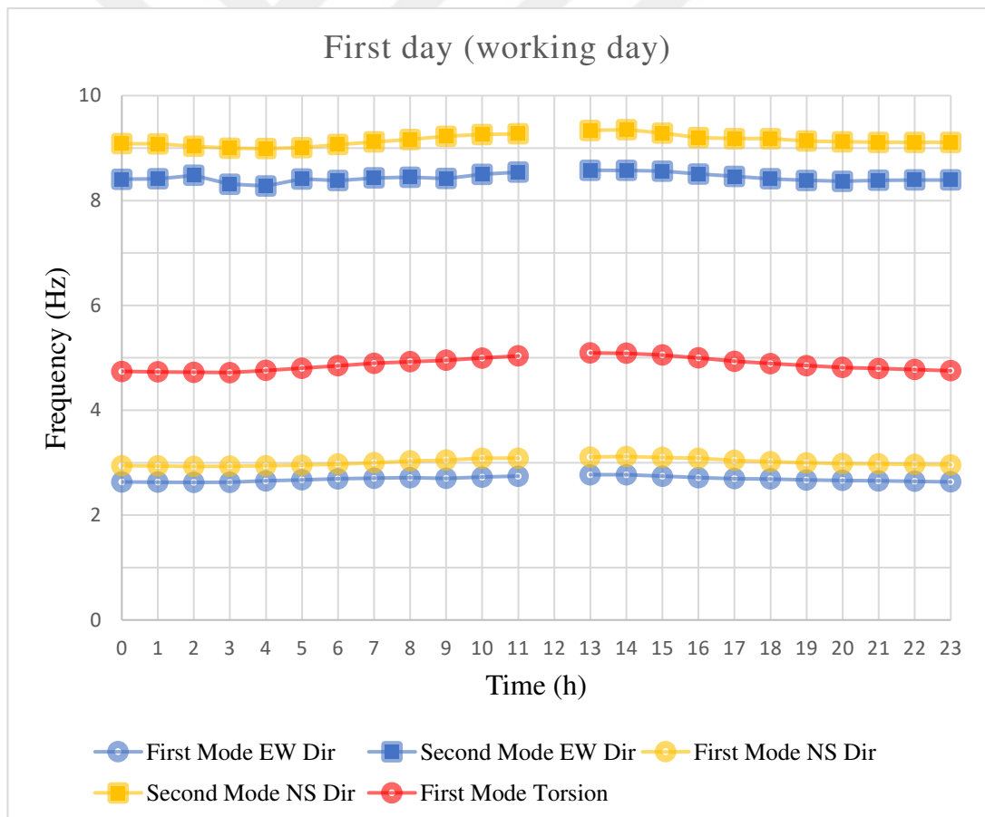
Figure 4.9. Hourly variation of frequencies (28/04/2017)
