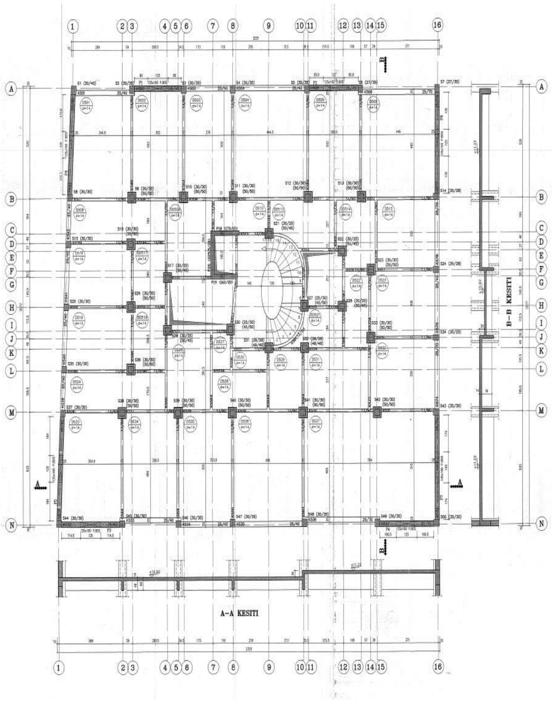
(e) third floor (+11.22)
