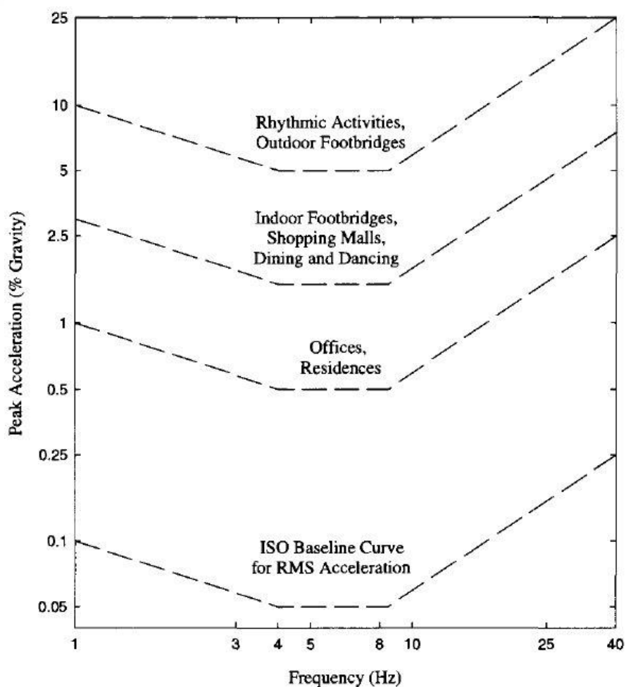
Figure 2.2. Recommended peak acceleration for human tolerance (ISO 2631-2)
