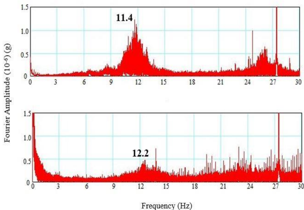
Figure 5.6. Floor frequency for the ground and second floors
