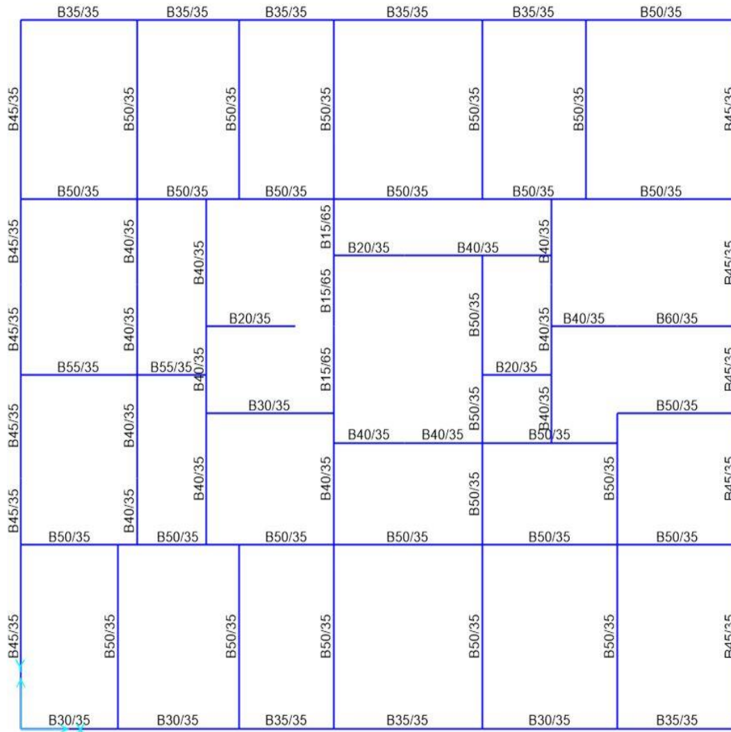
(b) fourth and fifth floors
