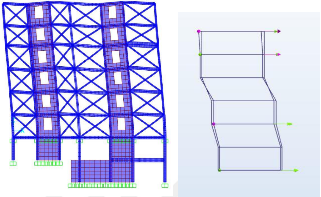
(a) First mode
