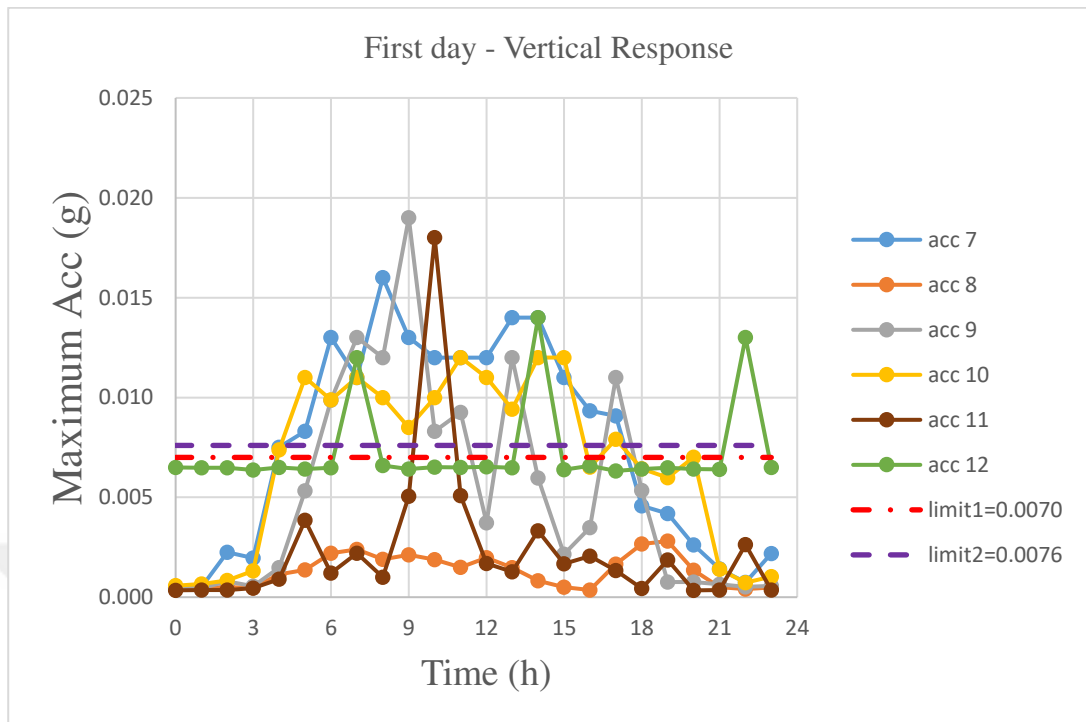
Figure 5.4. Hourly variation of maximum acceleration (03/05/2017)
