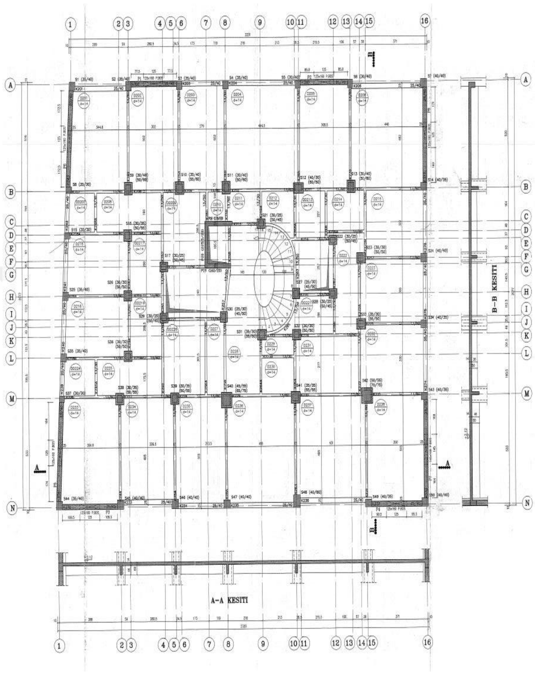
(c) ground floor (+2.12)
