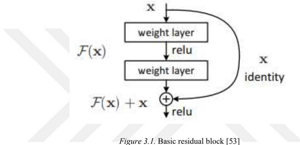
Figure 3.1. Basic residual block [53]
