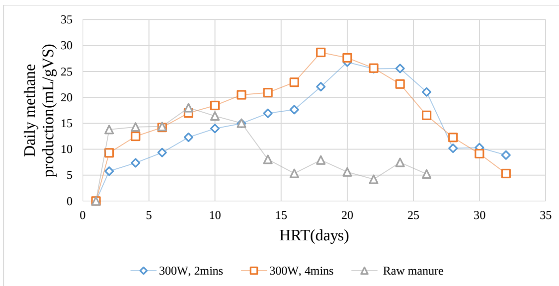
Figure 3.24 Daily methane production from microwave pretreatment of cattle manure.
