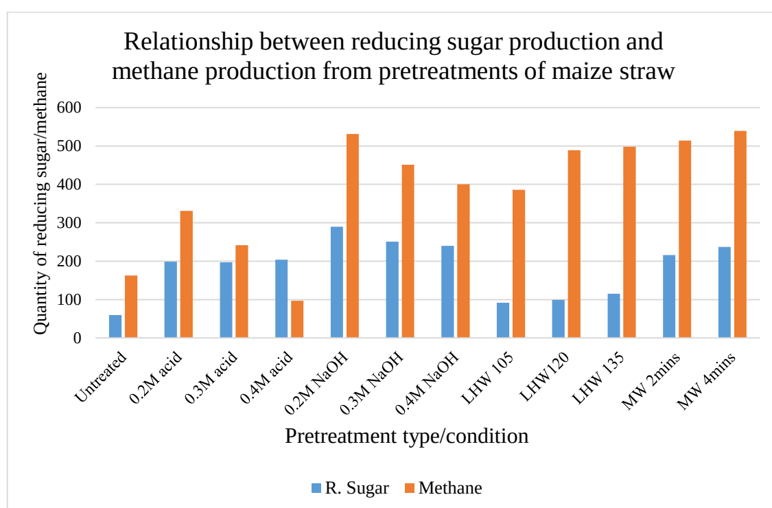
Figure 3. 3 Relationship between measured reducing sugar and methane production from maize straw.
