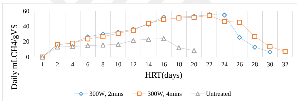
Figure 3. 11 Daily Methane production from microwave pretreatment of maize straw.
