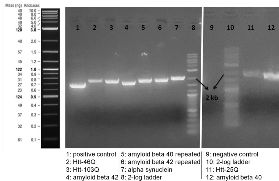
Figure 3.14: Agarose gel image showing the result of colony PCR on yeast colonies transformed with the indicated constructs above. Since two primers flanking Aga2p and gene of interest were used, amplicon lengths changed accordingly.
