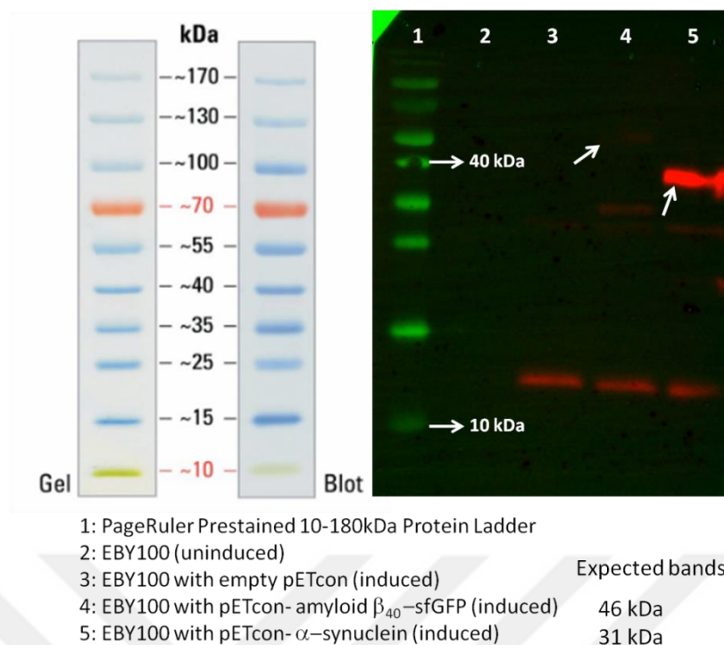
Figure 3.19: Result of western blot analysis of proteins with c-myc tag produced by listed cells.
