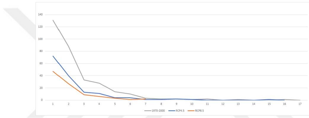
Figure 3.21. 1970-2000, RCP 4.5 and RCP 8.5 wind chill index consecutive cold day distributions in Amman.
