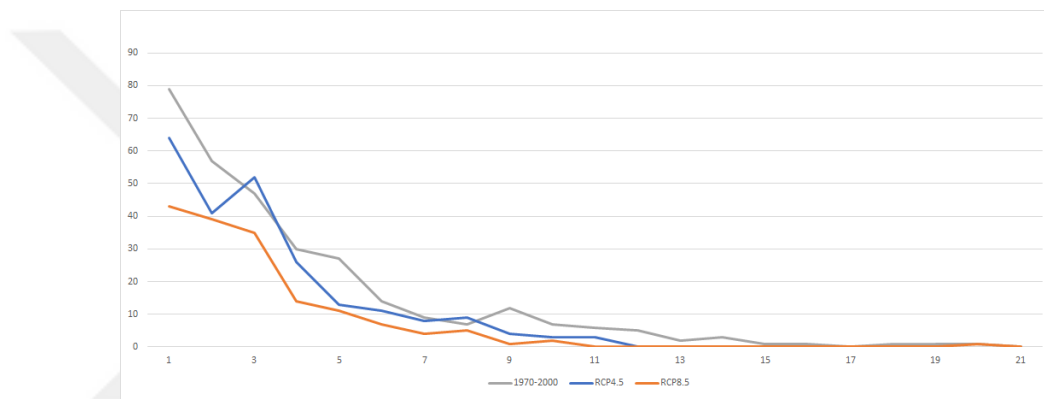
Figure 3.91. 1970-2000, RCP 4.5 and RCP 8.5 wind chill index consecutive cold day distributions in Riyadh.
