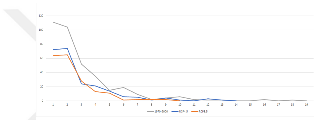
Figure 3.101. 1970-2000, RCP 4.5 and RCP 8.5 wind chill index consecutive cold day distributions in Tehran.
