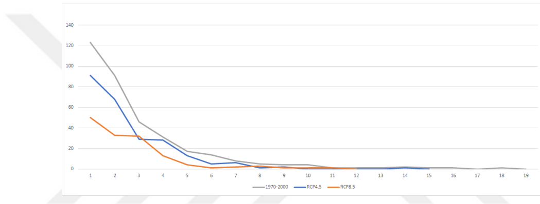
Figure 3.31. 1970-2000, RCP 4.5 and RCP 8.5 wind chill index consecutive cold day distributions in Ankara.
