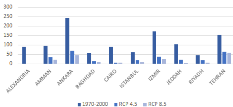
Figure 3.8. 1970-2000, RCP 4.5 and RCP 8.5 wind chill index extremely cold day counts.
