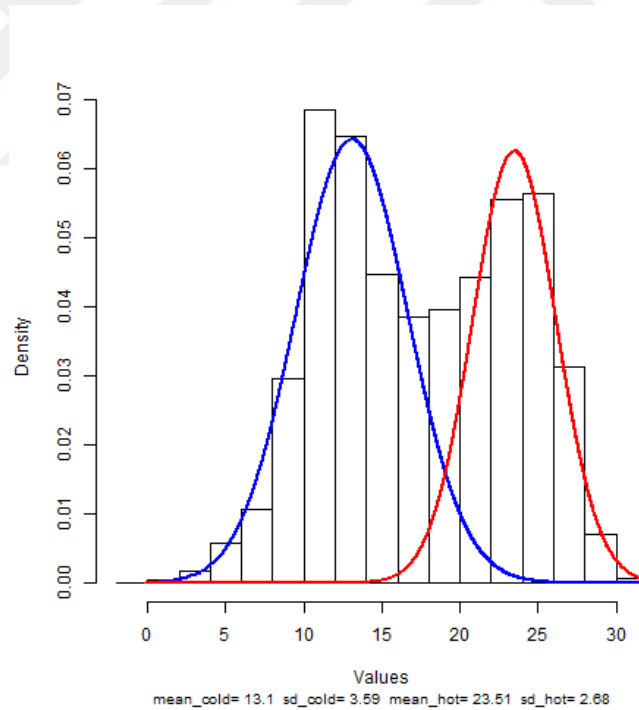
Figure 3.73. Distribution of 1970-2000 heat index values in Izmir.
