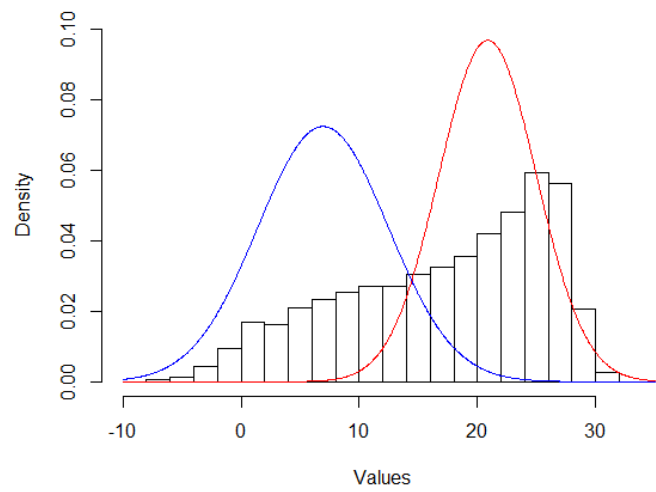
Figure 3.105. Distribution of 2070-2100 RCP 8.5 heat index values in Tehran.
