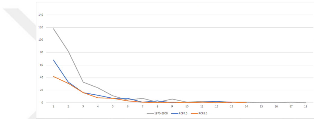
Figure 3.61. 1970-2000, RCP 4.5 and RCP 8.5 wind chill index consecutive cold day distributions in Istanbul.
