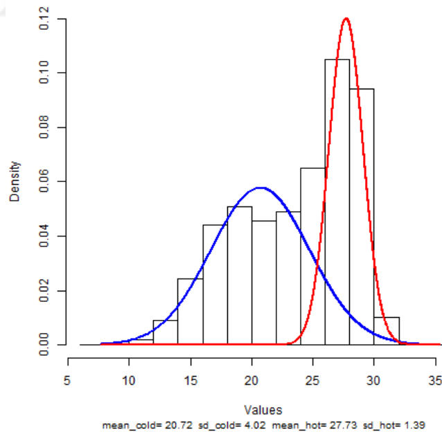
Figure 3.93. Distribution of 1970-2000 heat index values in Riyadh.
