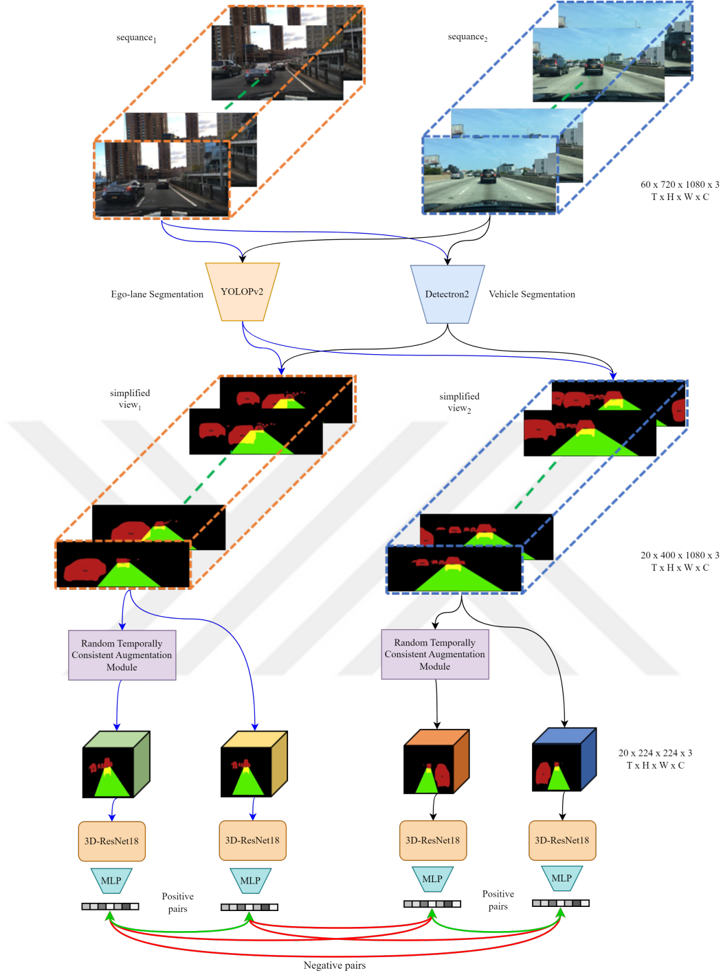
Figure 5.3. Contrastive Maneuver Representation Learning. First, we create simplified video clips by extracting the vehicle and ego-lane masks from raw videos. Then, different temporally consistent augmentations (e.g. crop, flip, shear, rotation) are applied to the simplified video clips randomly before giving them as input to our video encoder (3D-ResNet18). For self-supervised learning, extracted feature tensors of each sample in mini-batch are compared with InfoNCE loss such that representations of positive pairs (green arrows) are brought together, and representations of negative pairs (red arrows) are put far apart.
