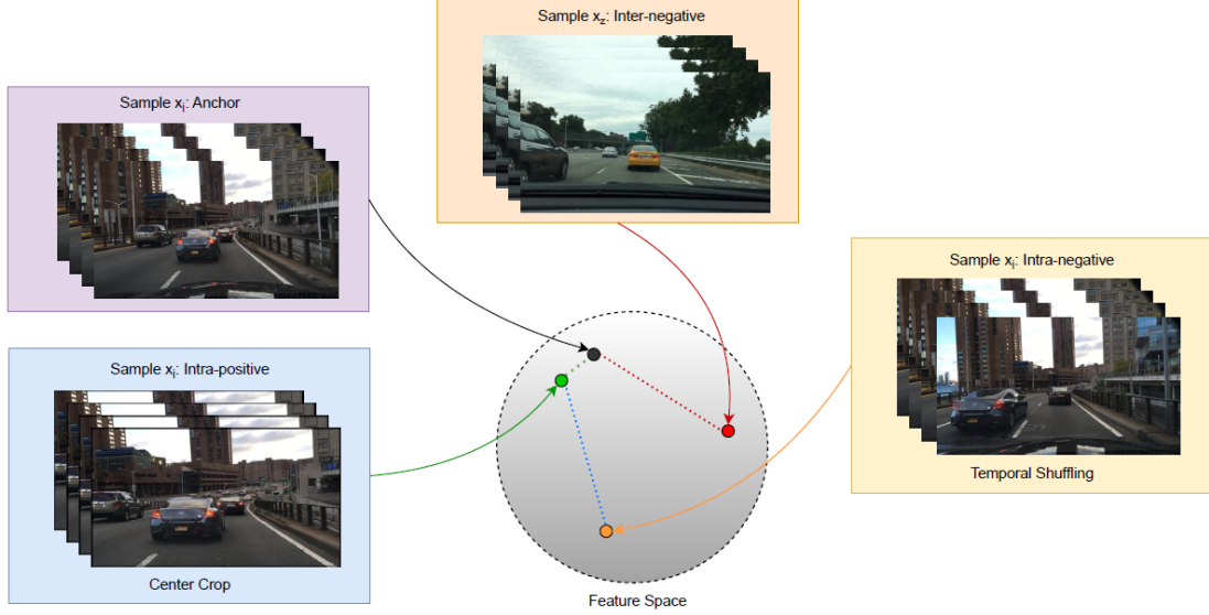
Figure 5.6. Feature space representation of intra-positive, intra-negative, and inter-negative samples. (Source: Tao et al. (2020))
