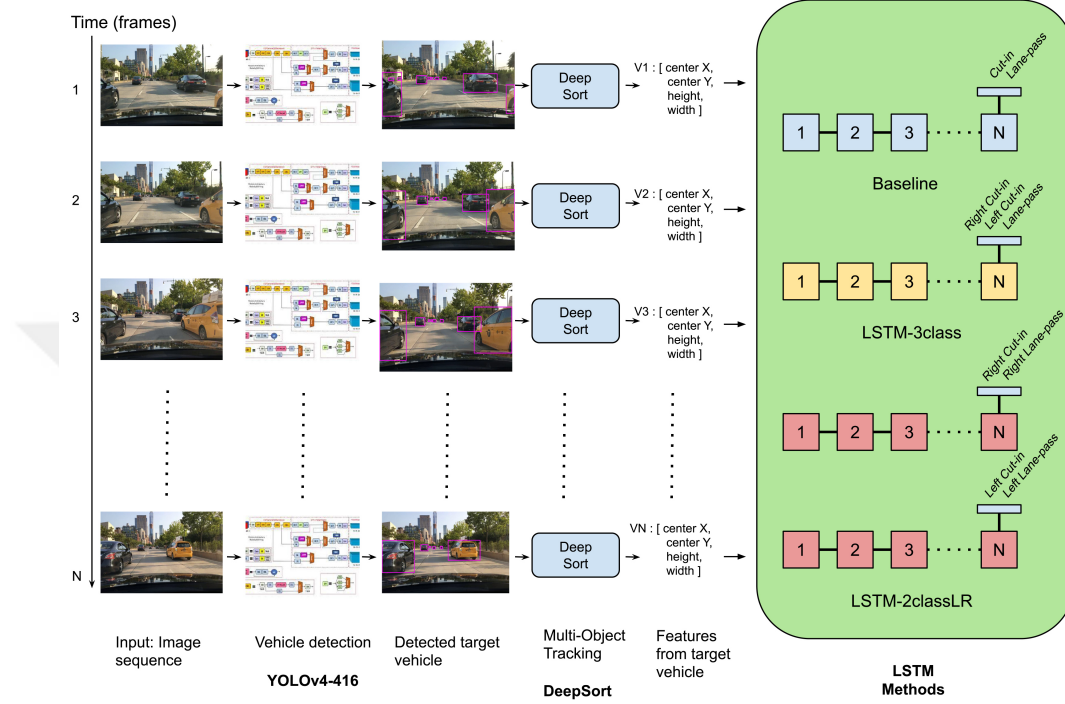
Figure 4.1. Pipeline of the proposed approach. Following the steps for extracting the bounding boxes of target vehicles (TVs), the baseline LSTM method uses feature vectors of TVs and classifies maneuvers as cut-in or lane-pass. LSTM-3class method classifies into 3: right cut-in, left cut-in, or lane-pass classes. As a third alternative, LSTM-2classLR has two separate LSTMs for left-hand side and right-hand side TVs. We conducted experiments with varying sequence lengths (15, 30, 45, and 60 frames) all representing two seconds of the video.
