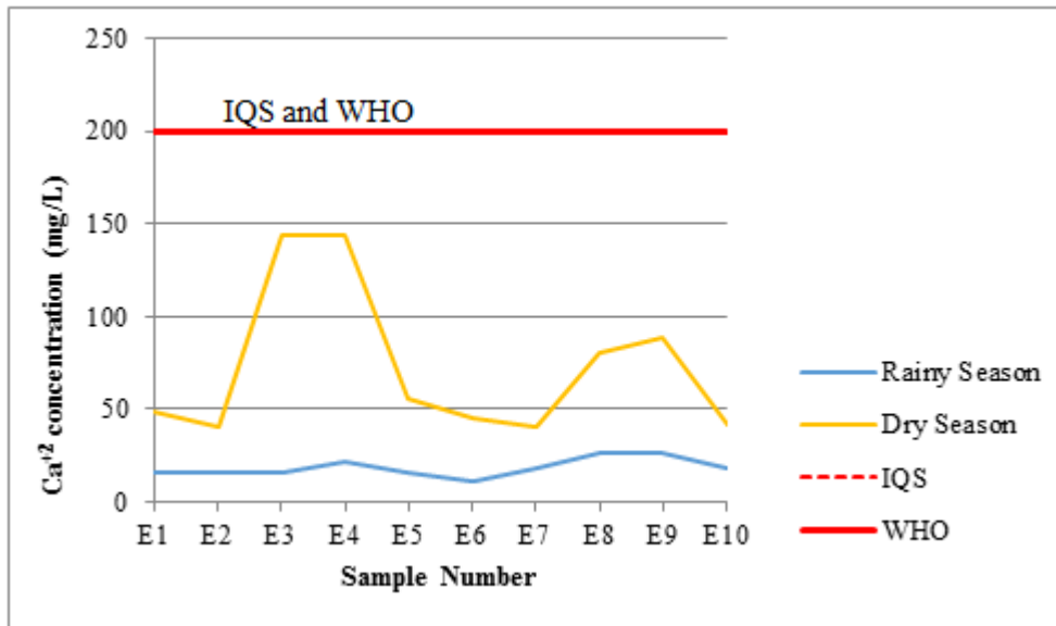
Figure 4.10. Seasonal variations of calcium contents in investigated groundwaters
