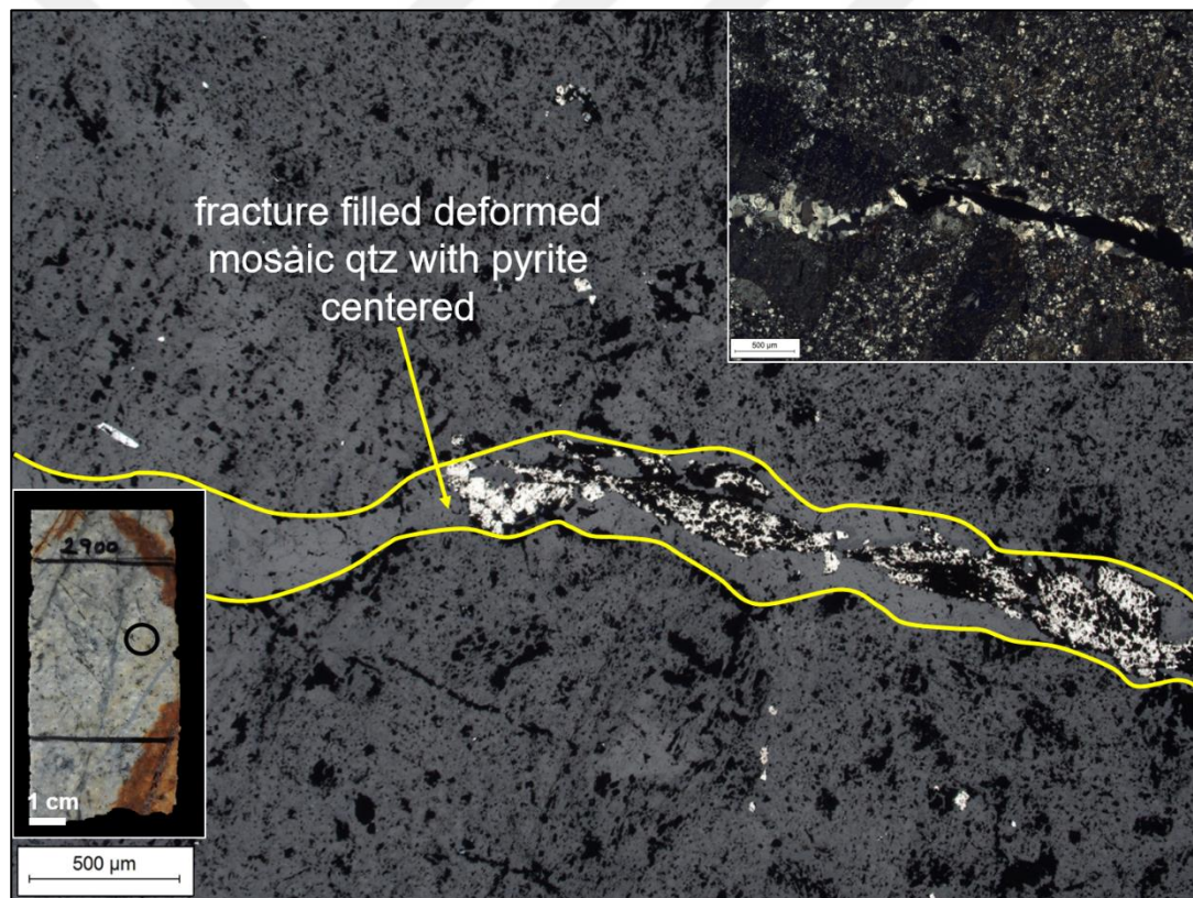
Figure 4.58. Microphotographs of sample (drill hole SHD-154, 29.00 m depth) showing weak stockwork veinlets with comb to mosaic quartz and pyrite inclusions (main image RL, PPL; inset TL, XPL). (Abbreviations: qtz = quartz).
