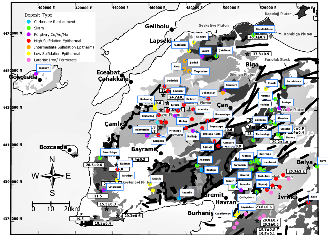
Figure 3.7. Distribution of major magmatic-hydrothermal deposits and prospects in Biga Peninsula (adapted from Yiğit 2012)
