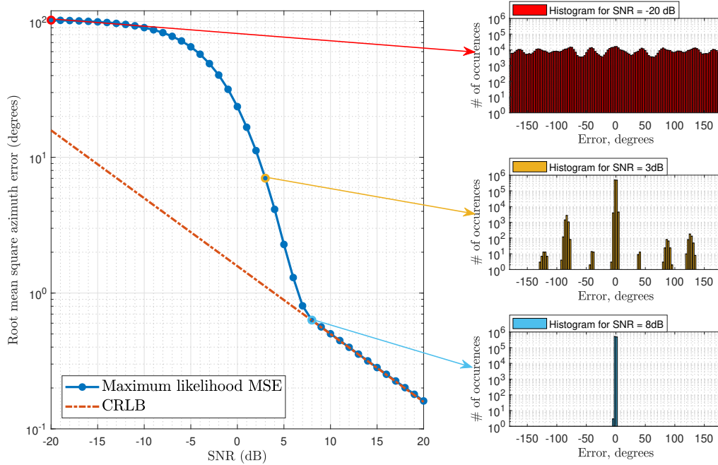
Figure 1.2: Histograms of error signals at different regions of operation.
