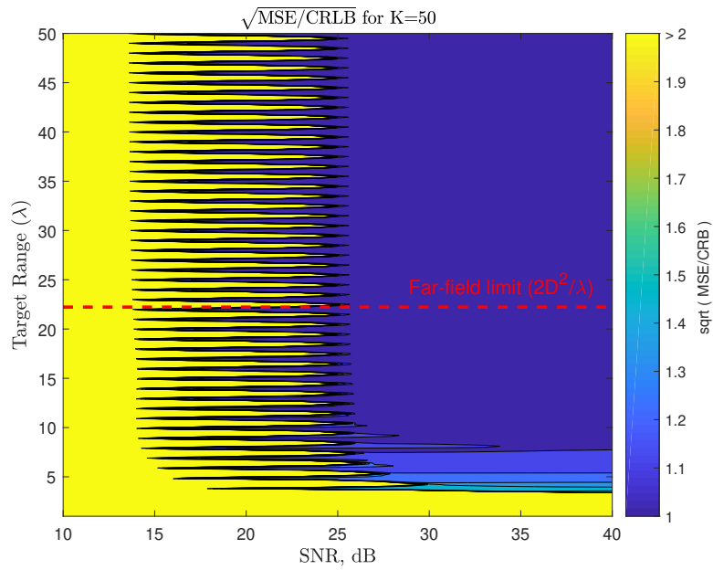
Figure 4.6: Ratio of predicted MSE values for ML estimator to CRLB for various SNR and target range values, for a Rician factor of 50. Note that the color scale is set between 1 and > 2 .
